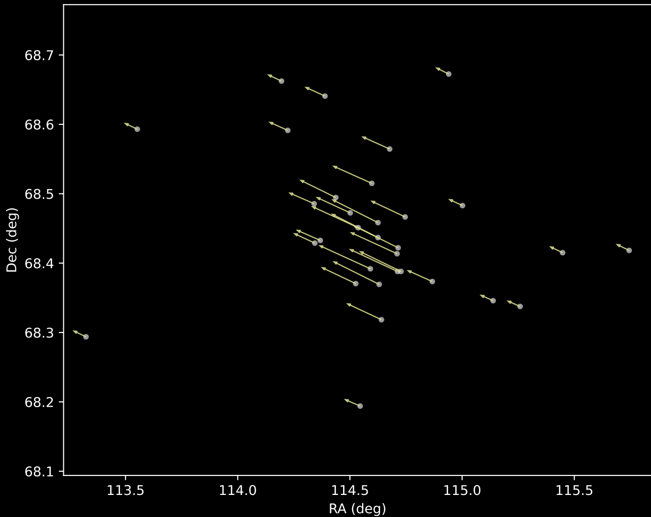
Gaia DR3 Cluster 57 Proper Motion Vectors (n=32)
