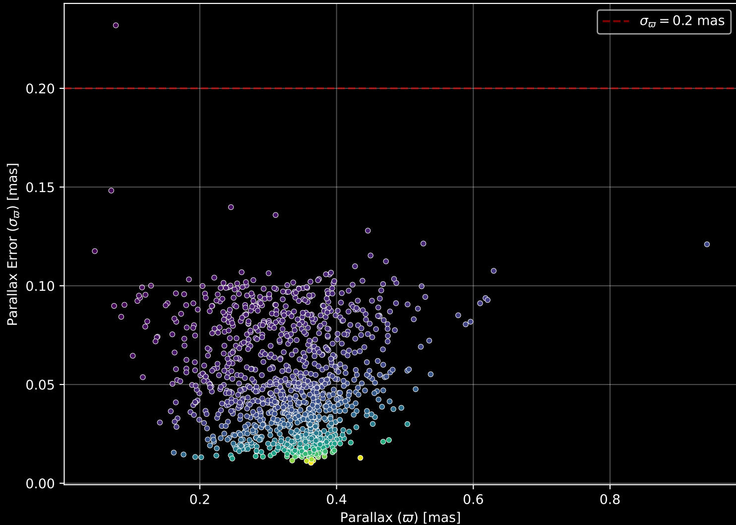
Gaia Cluster: [Skiff_J0058+68.4] Parallax Quality (n= 1085)
