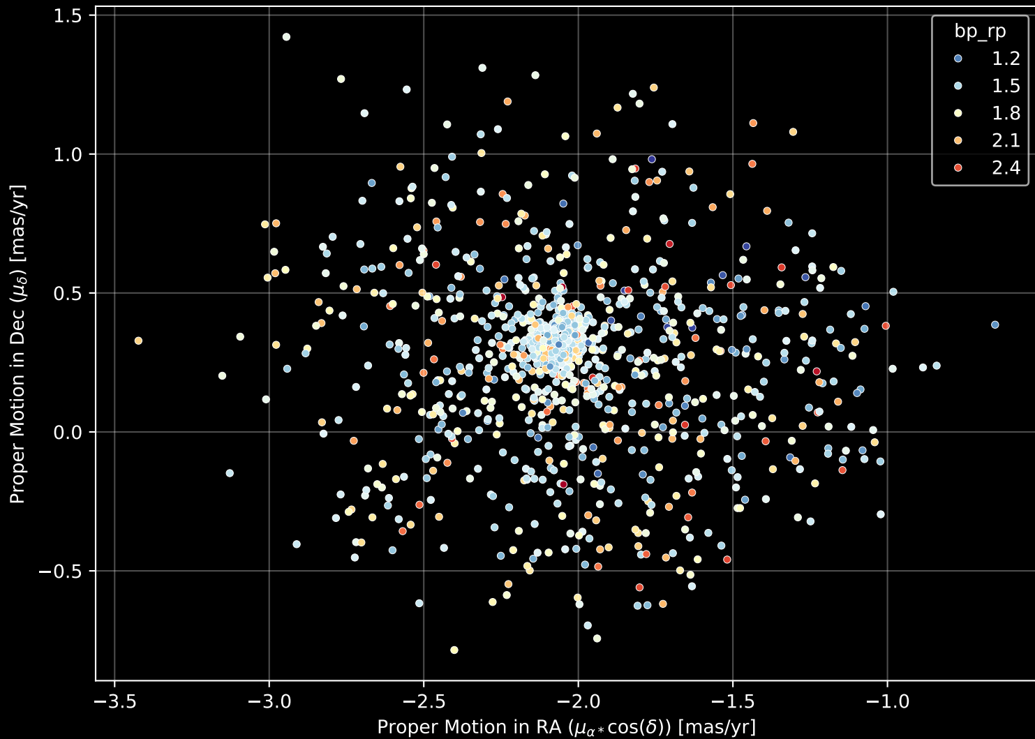
Gaia Cluster: [Skiff_J0058+68.4] Proper Motion Diagram (n= 1085)
