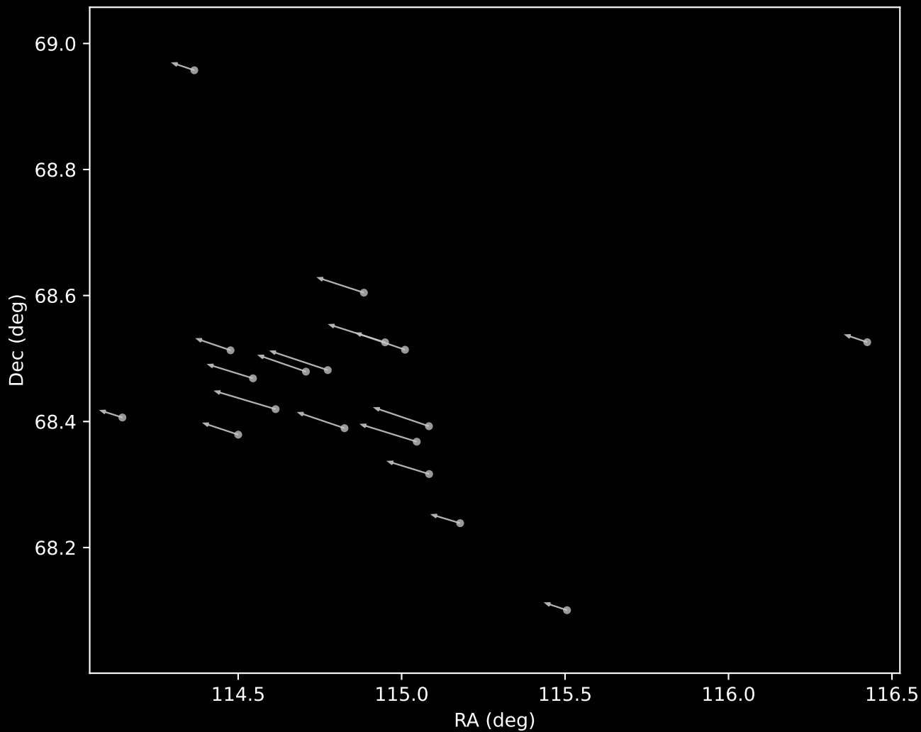
Gaia DR3 Cluster 55 Proper Motion Vectors (n=18)
