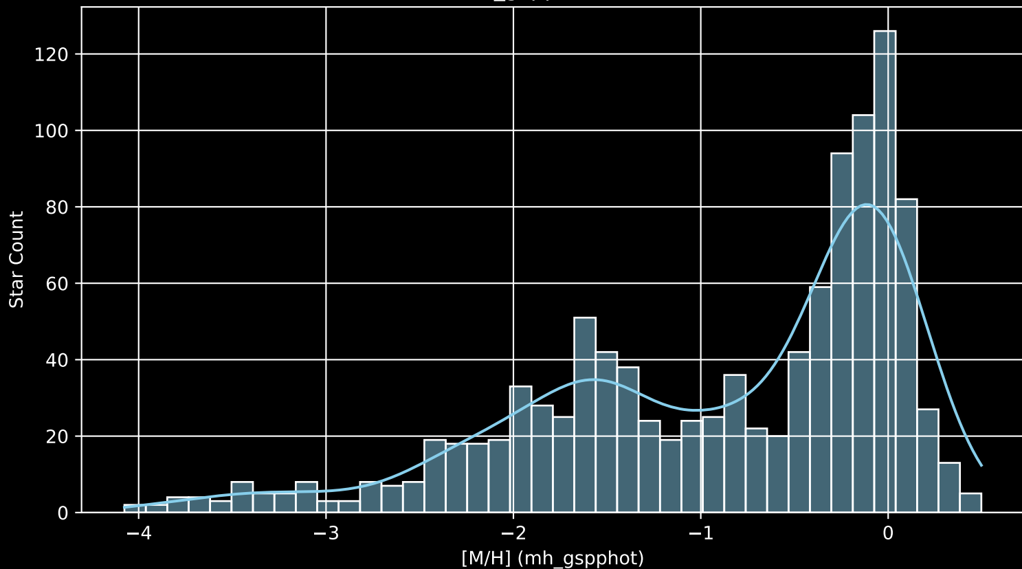
Gaia Cluster: [Skiff_J0058+68.4 [M/H] (mh_gspphot) (n= 1083)
