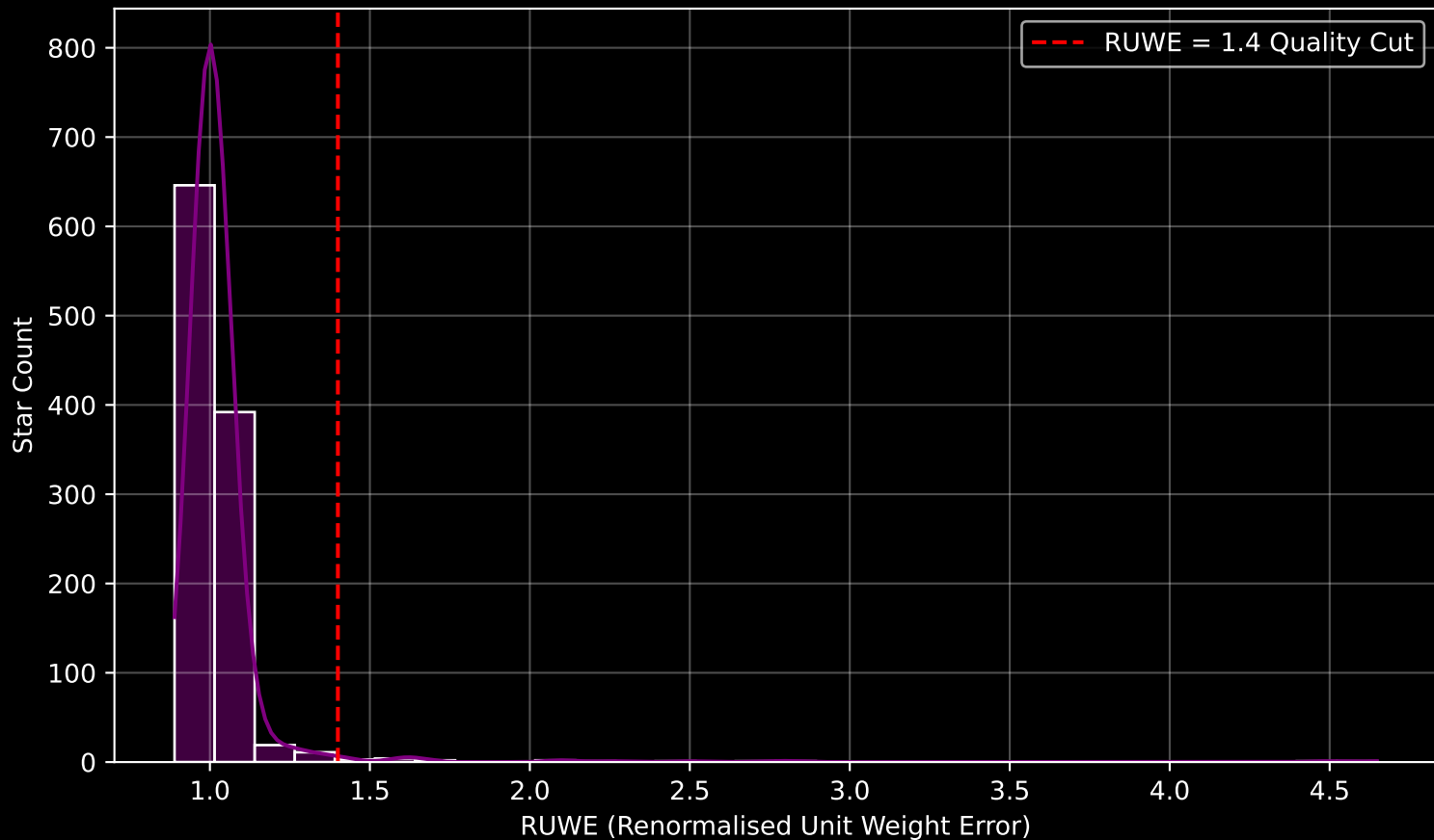
Gaia Cluster: [Skiff_J0058+68.4] RUWE Distribution (n= 1085)
