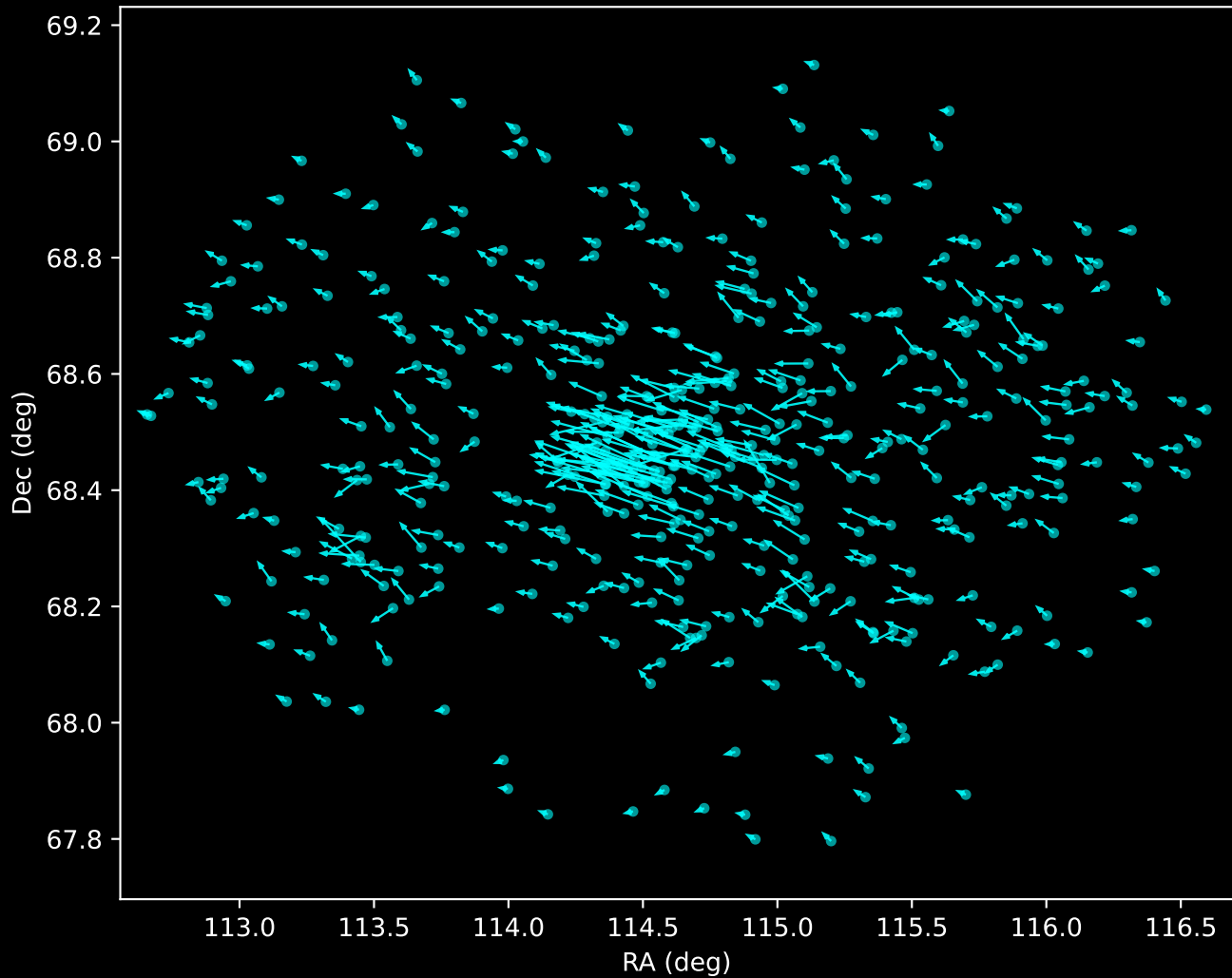
Gaia DR3 Noise Stream Proper Motion Vectors (n=467)
