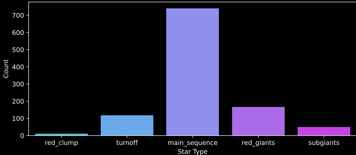
Gaia Cluster: [Skiff_J0058+68.4] Count plot of Star Type
