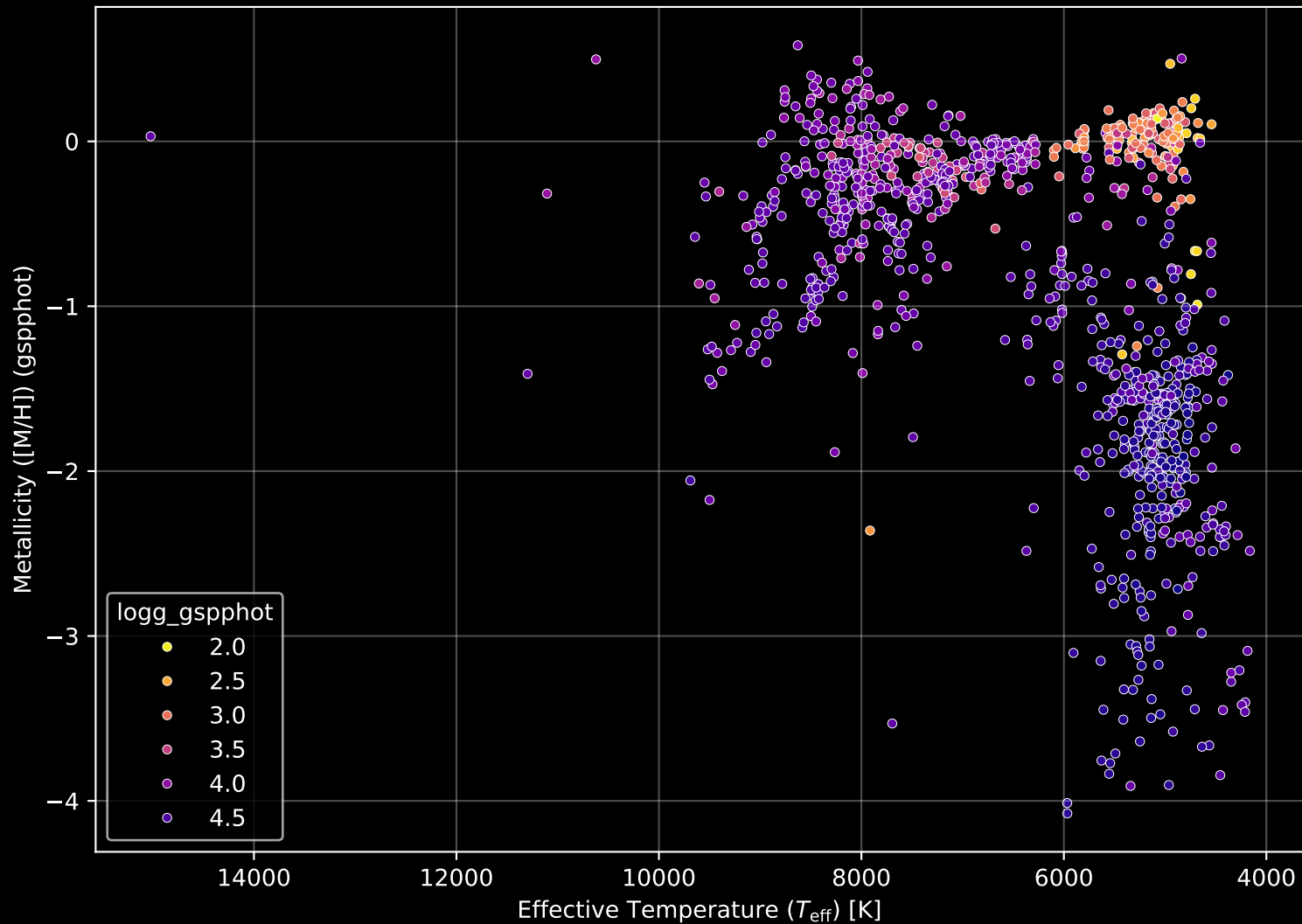
Gaia Cluster: [Skiff_J0058+68.4] Stellar Population Parameters (n= 1085)
