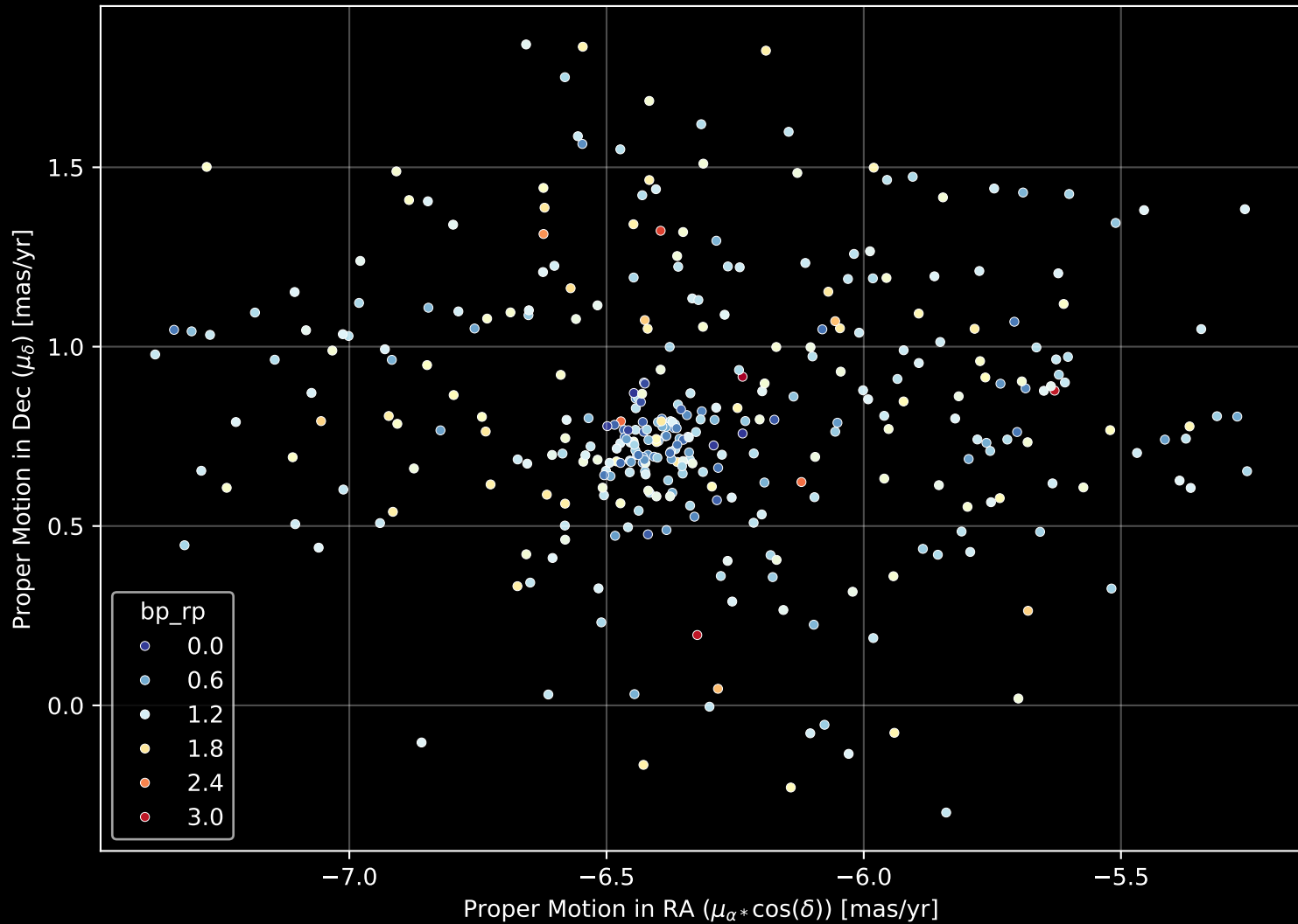
Gaia Cluster: [Stock_14] Proper Motion Diagram (n= 351)
