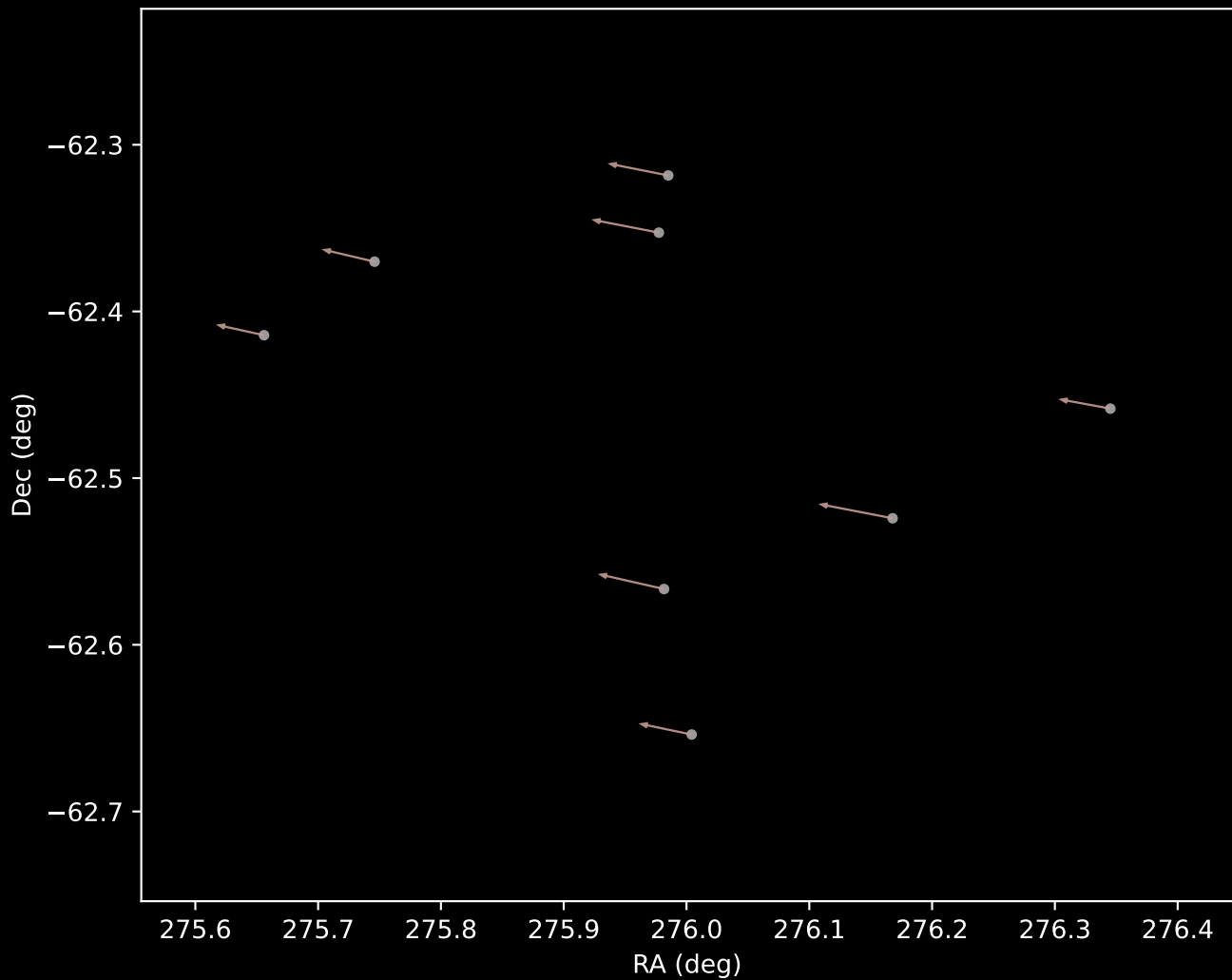
Gaia DR3 Cluster 11 Proper Motion Vectors (n=8)
