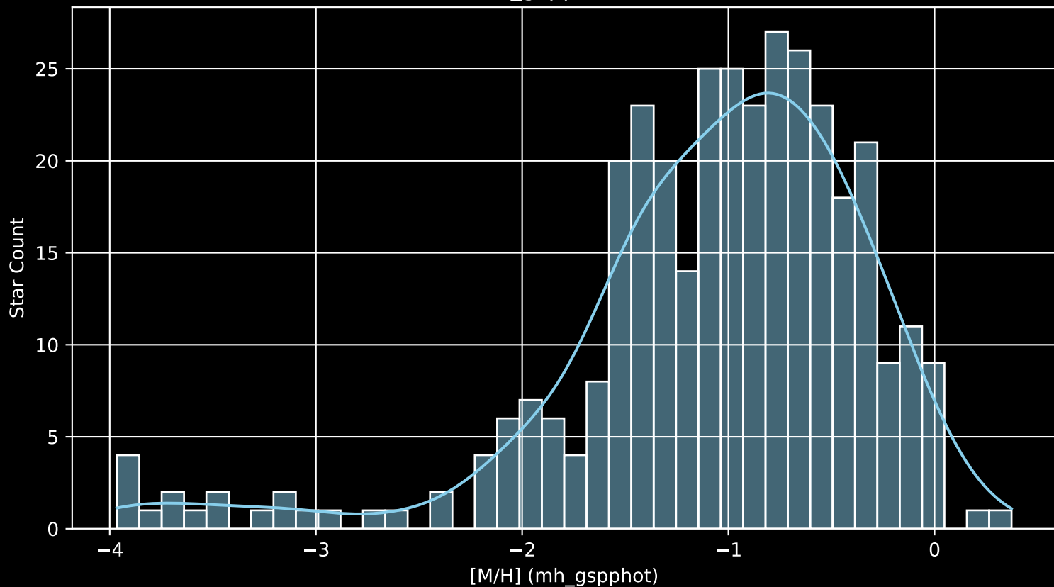
Gaia Cluster: [Stock_14 [M/H] (mh_gspphot) (n= 350)
