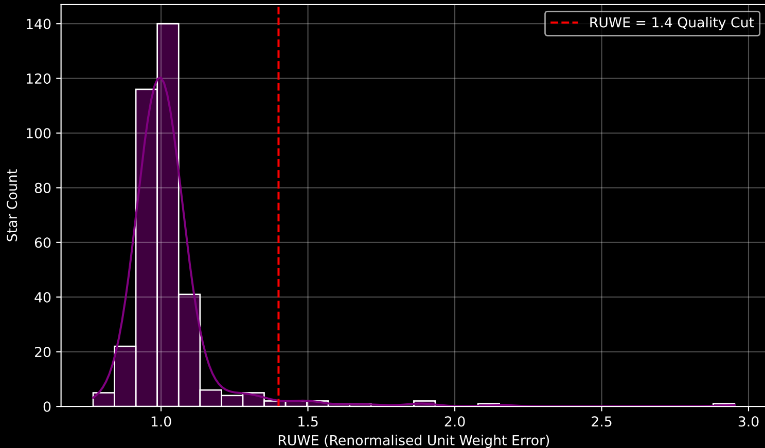
Gaia Cluster: [Stock_14] RUWE Distribution (n= 351)
