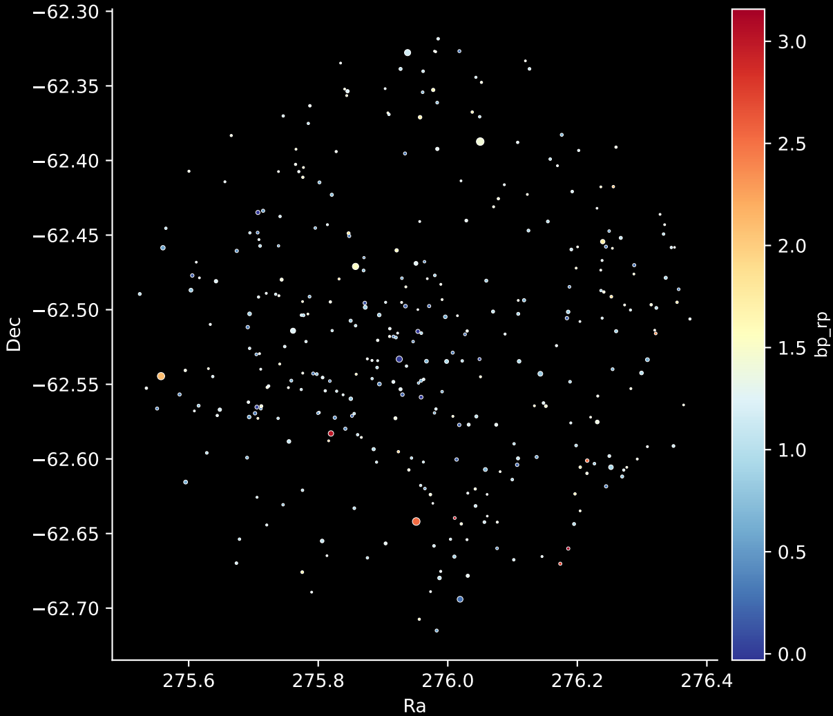
Gaia Cluster: [Stock_14] Stars: 351
