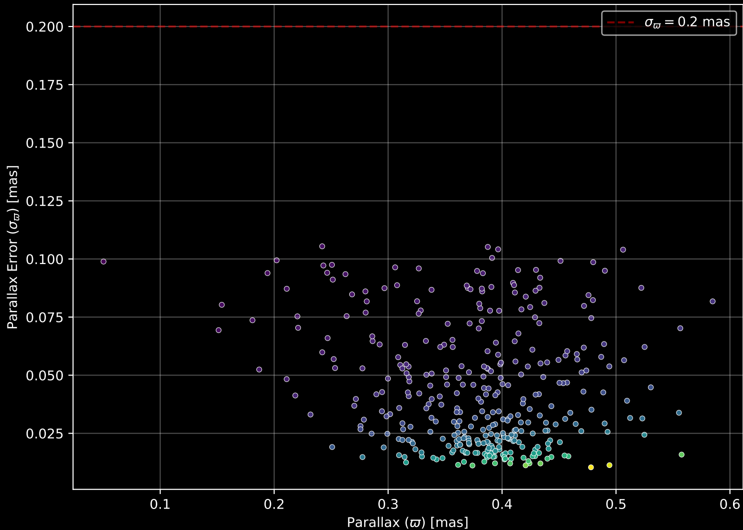
Gaia Cluster: [Stock_14] Parallax Quality (n= 351)
