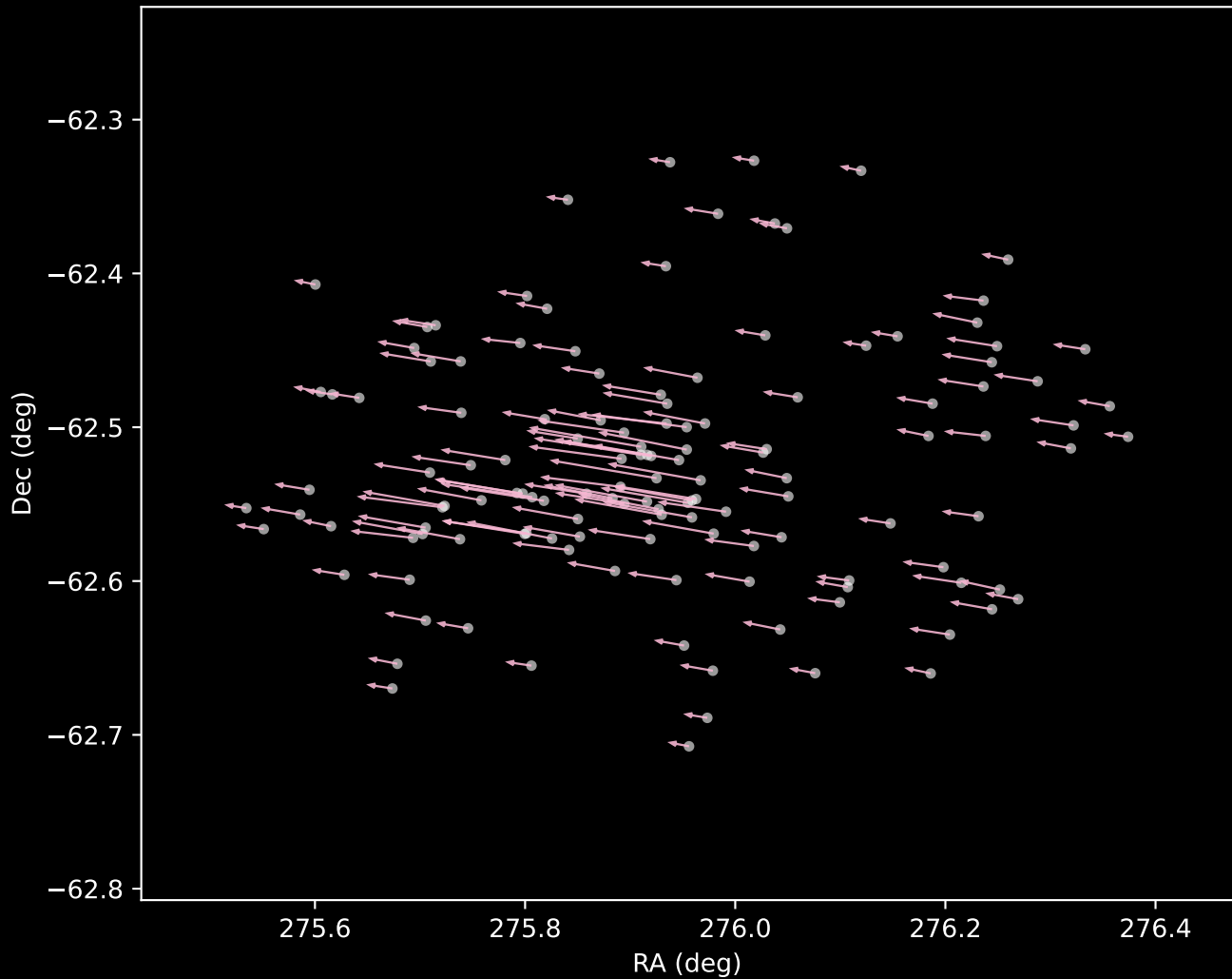
Gaia DR3 Cluster 13 Proper Motion Vectors (n=134)
