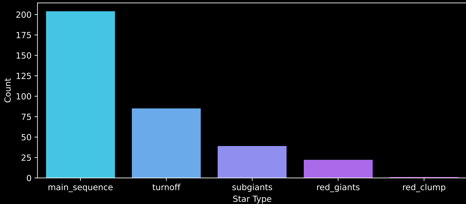
Gaia Cluster: [Stock_14] Count plot of Star Type
