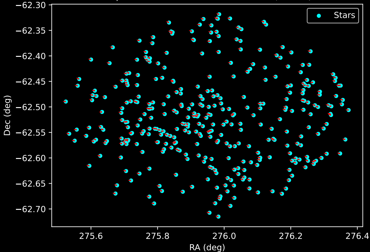
Gaia Cluster: [Stock_14] Proper Motion Vectors for Gaia Star Field (n= 351)
