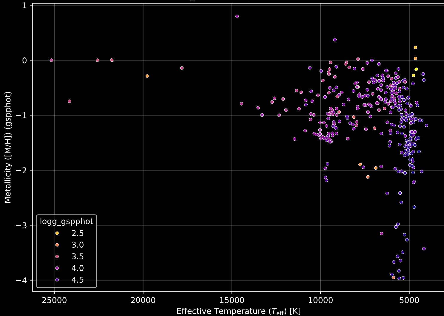
Gaia Cluster: [Stock_14] Stellar Population Parameters (n= 351)
