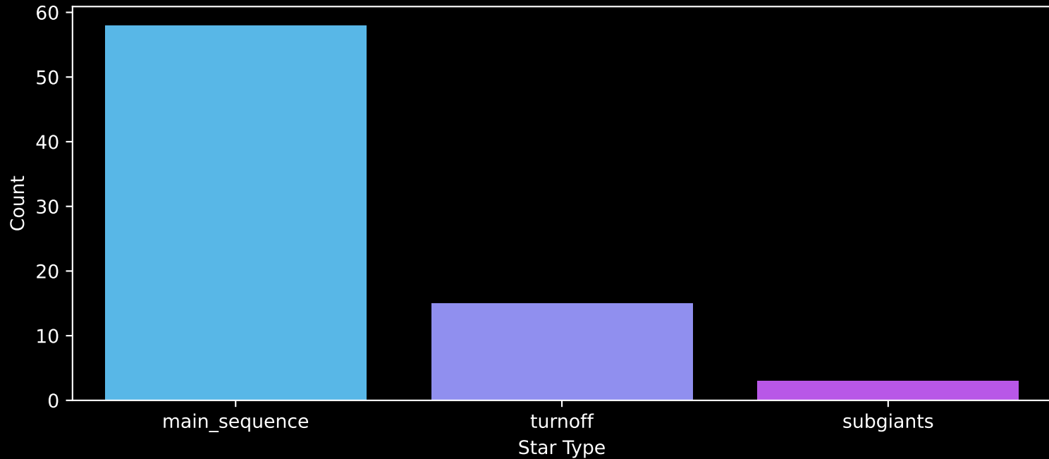
Gaia Cluster: [Stock_21] Count plot of Star Type
