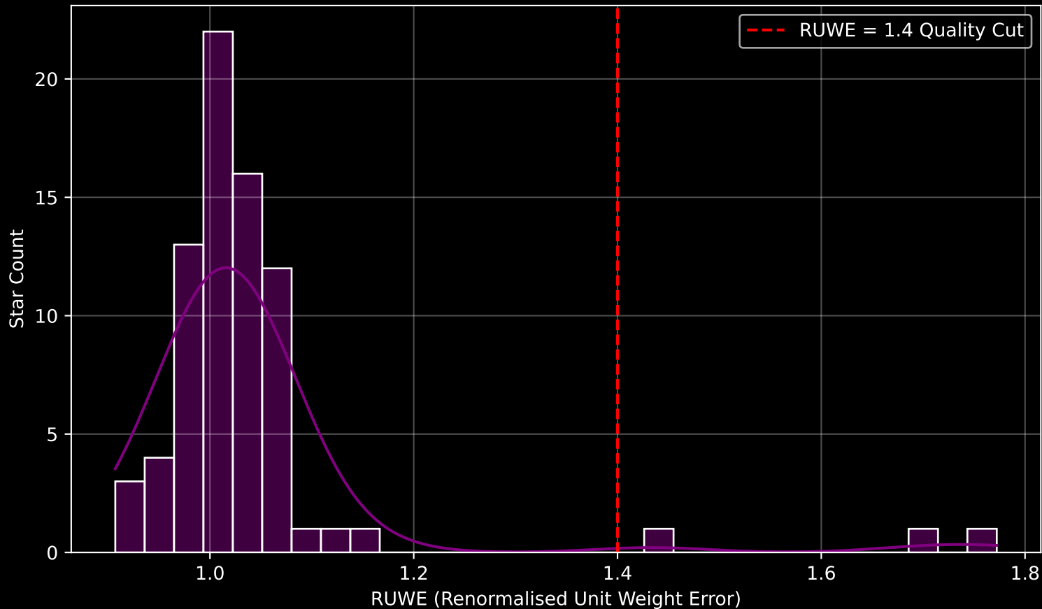
Gaia Cluster: [Stock_21] RUWE Distribution (n= 76)
