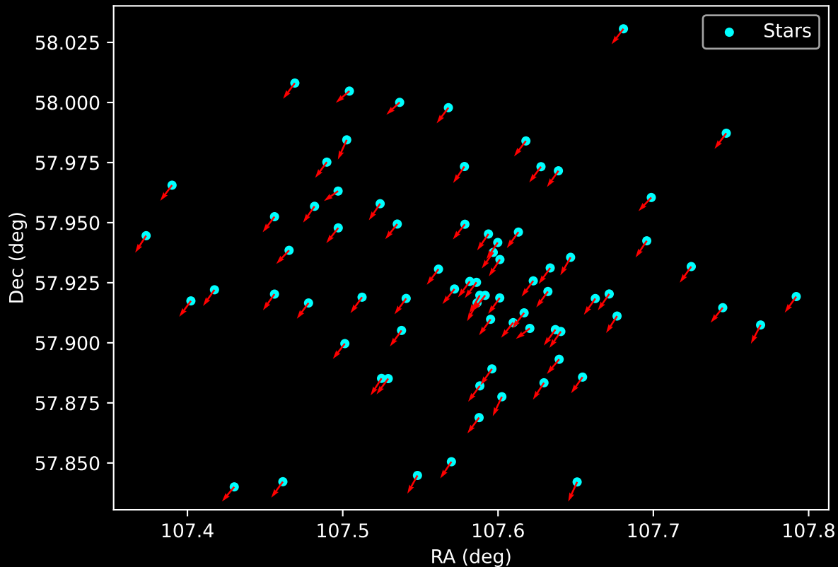
Gaia Cluster: [Stock_21] Proper Motion Vectors for Gaia Star Field (n= 76)
