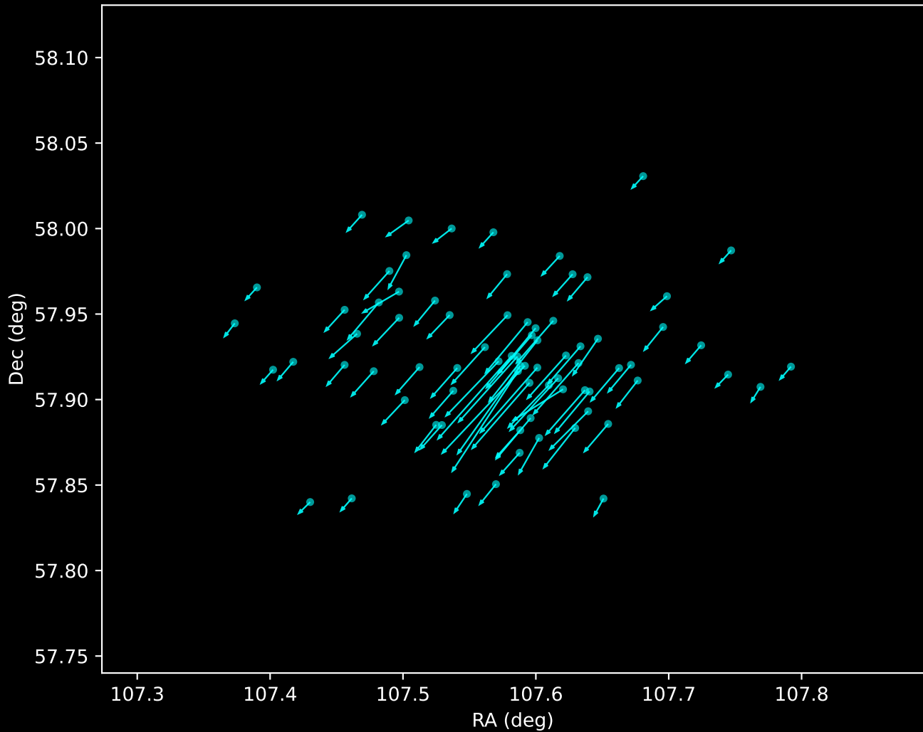
Gaia DR3 Noise Stream Proper Motion Vectors (n=76)
