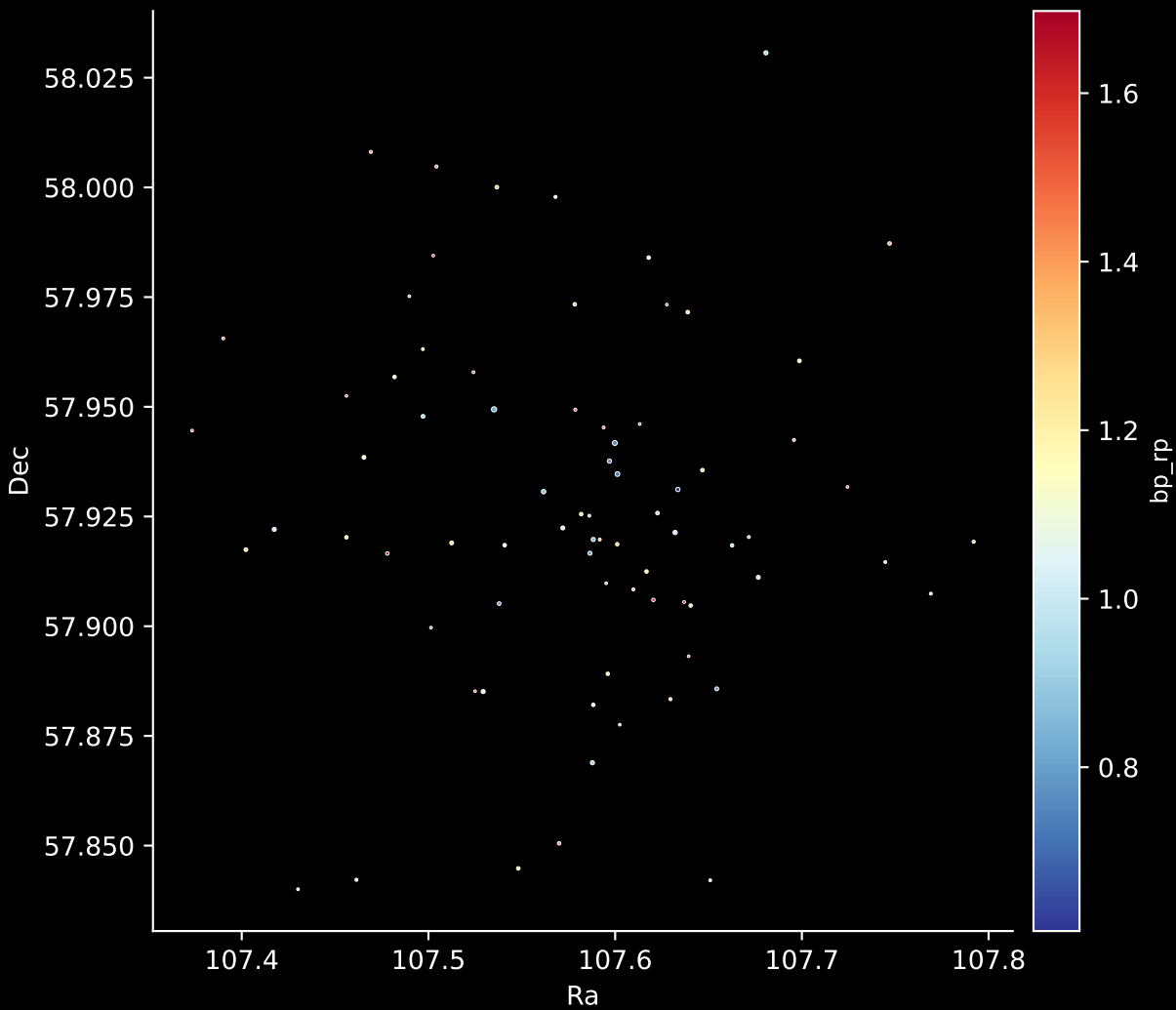
Gaia Cluster: [Stock_21] Stars: 76
