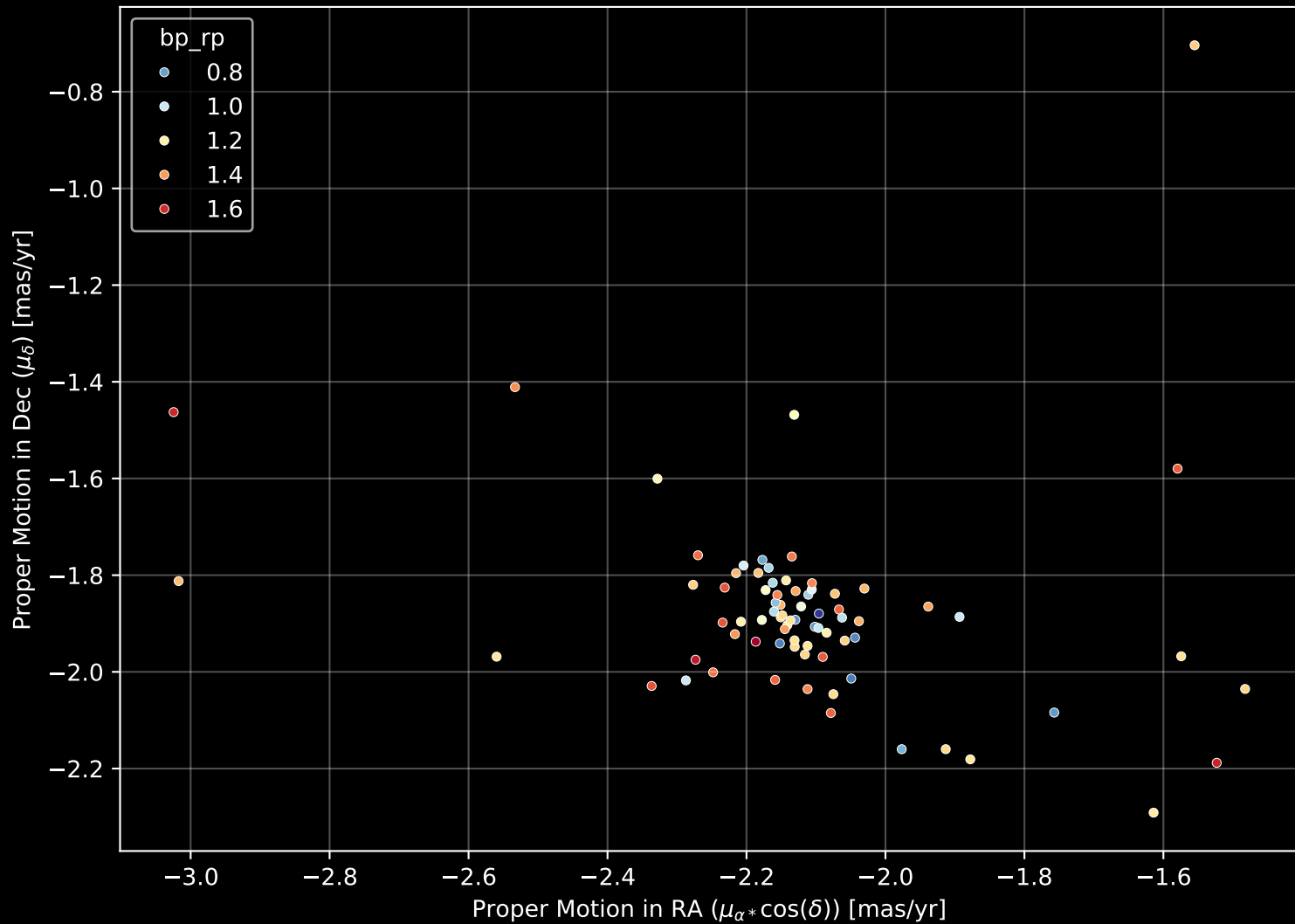
Gaia Cluster: [Stock_21] Proper Motion Diagram (n= 76)
