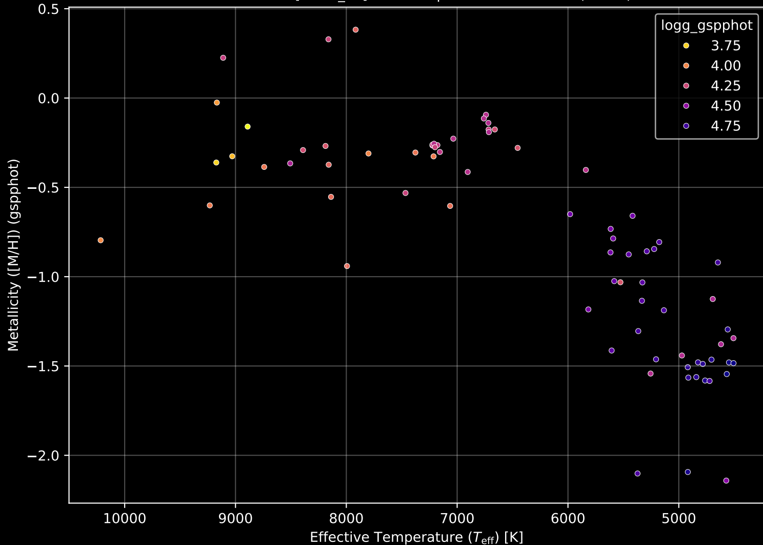
Gaia Cluster: [Stock_21] Stellar Population Parameters (n= 76)
