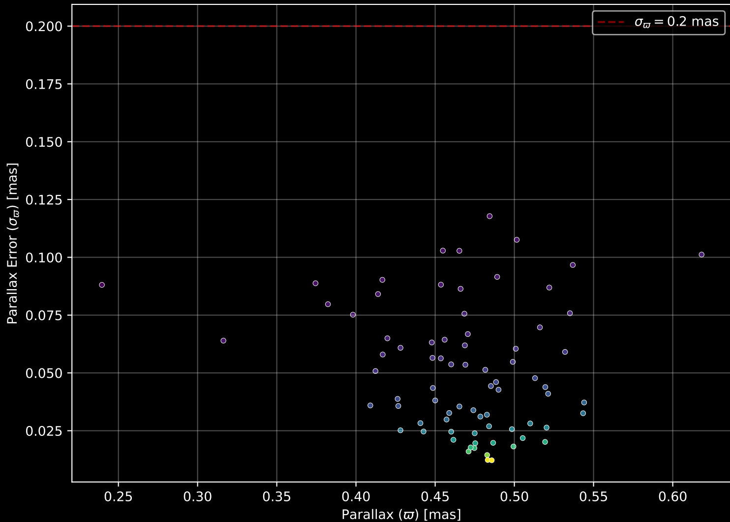
Gaia Cluster: [Stock_21] Parallax Quality (n= 76)
