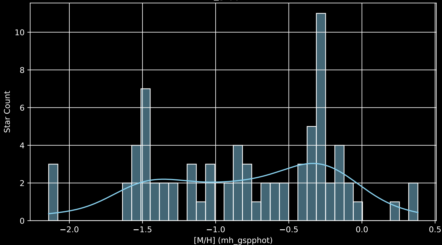
Gaia Cluster: [Stock_21 [M/H] (mh_gspphot) (n= 76)
