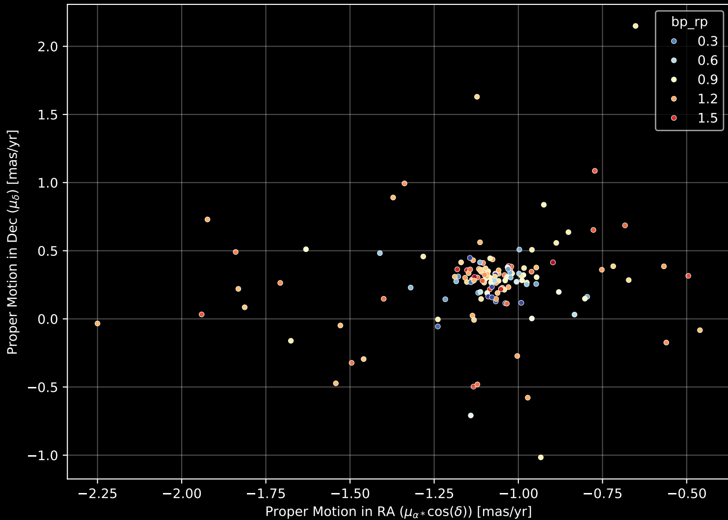
Gaia Cluster: [Stock_4] Proper Motion Diagram (n= 143)
