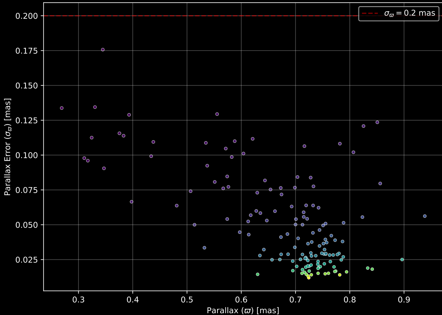
Gaia Cluster: [Stock_4] Parallax Quality (n= 143)
