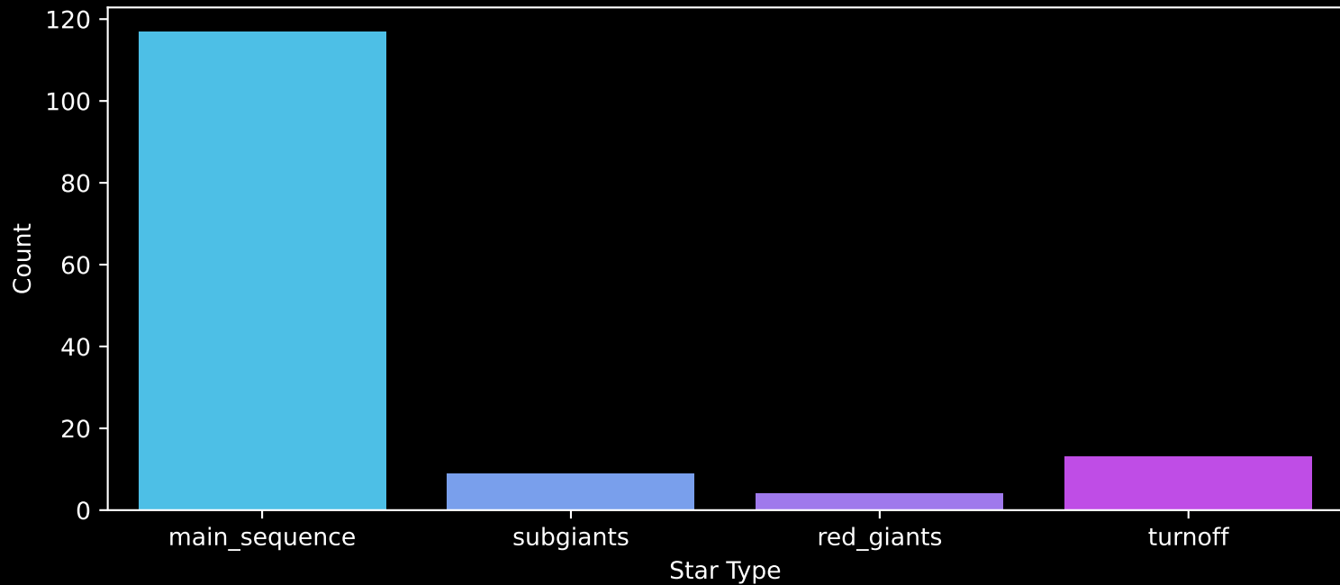
Gaia Cluster: [Stock_4] Count plot of Star Type
