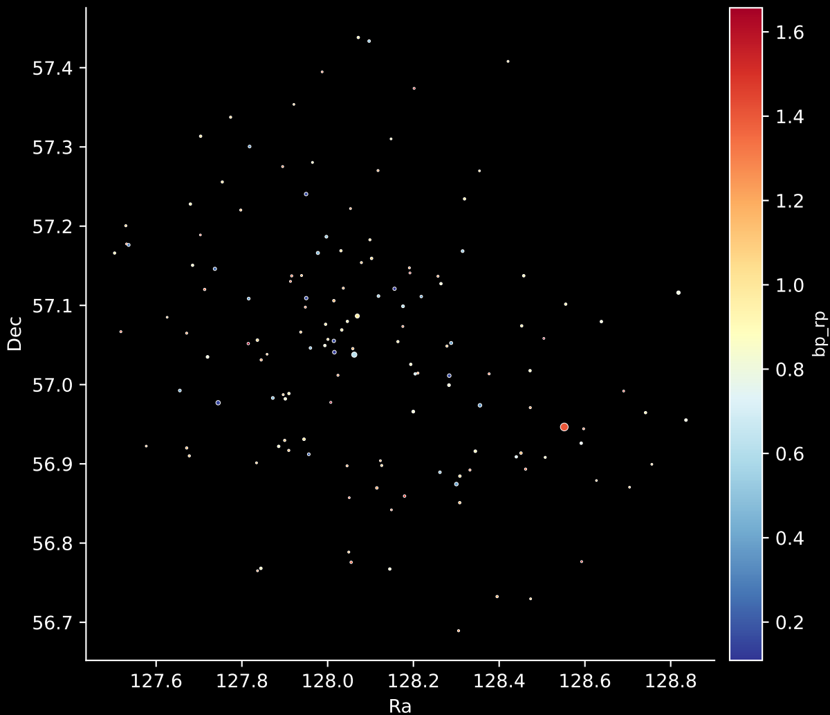
Gaia Cluster: [Stock_4] Stars: 143
