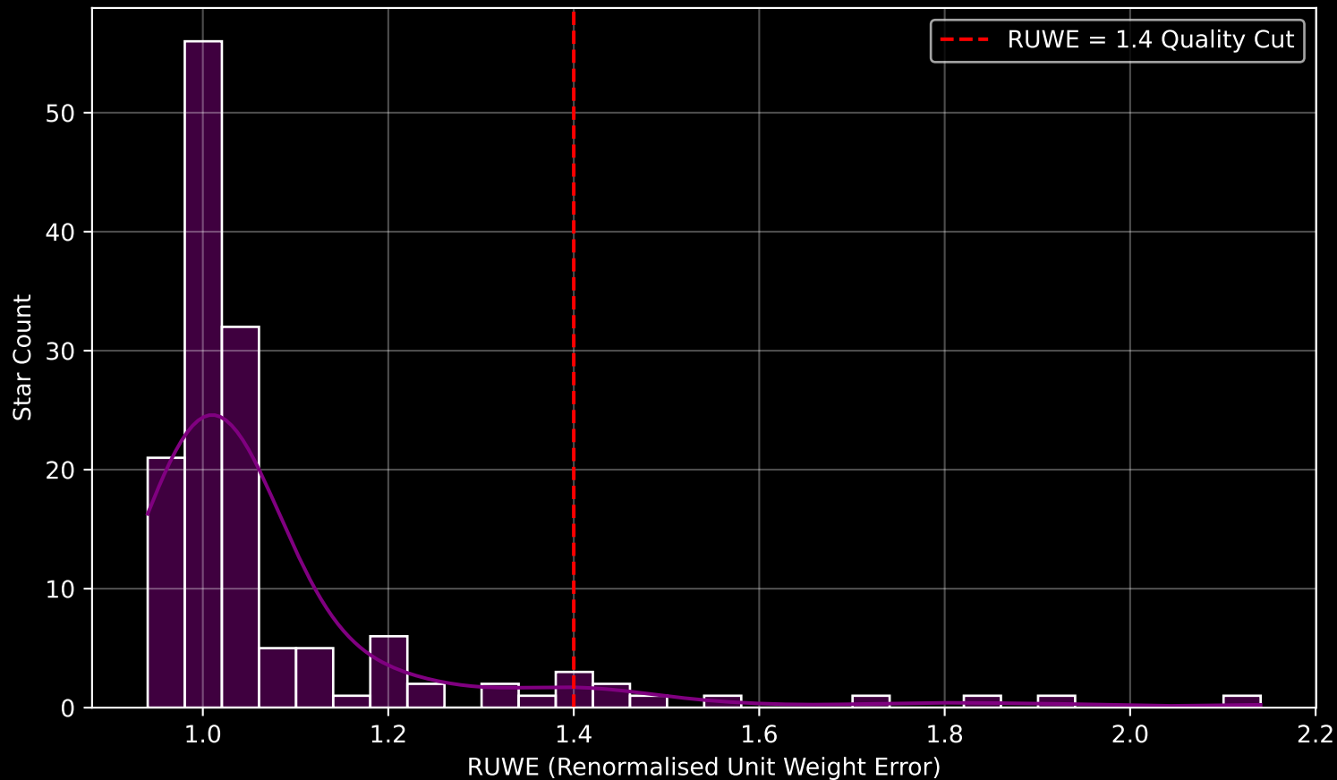
Gaia Cluster: [Stock_4] RUWE Distribution (n= 142)
