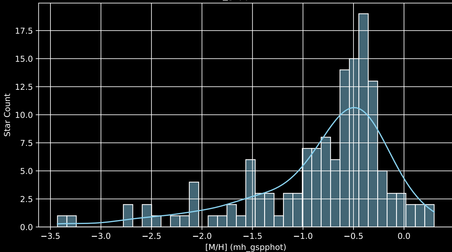
Gaia Cluster: [Stock_4 [M/H] (mh_gspphot) (n= 143)
