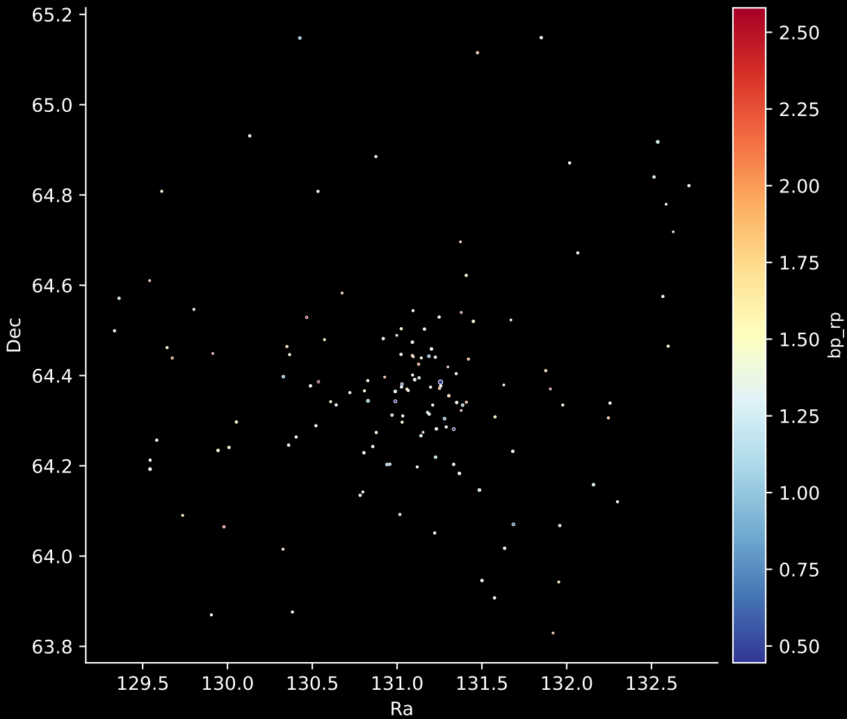
Gaia Cluster: [Stock_5] Stars: 136
