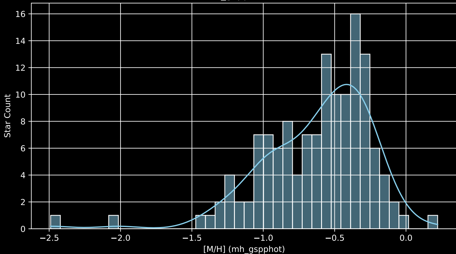
Gaia Cluster: [Stock_5 [M/H] (mh_gspphot) (n= 136)
