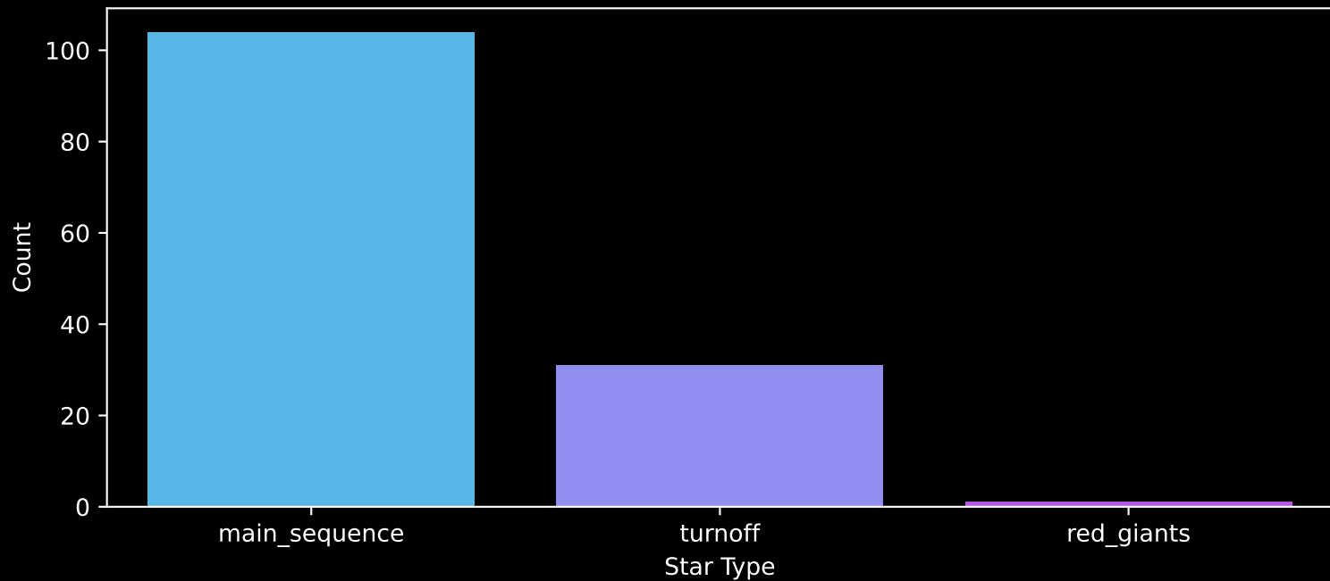
Gaia Cluster: [Stock_5] Count plot of Star Type
