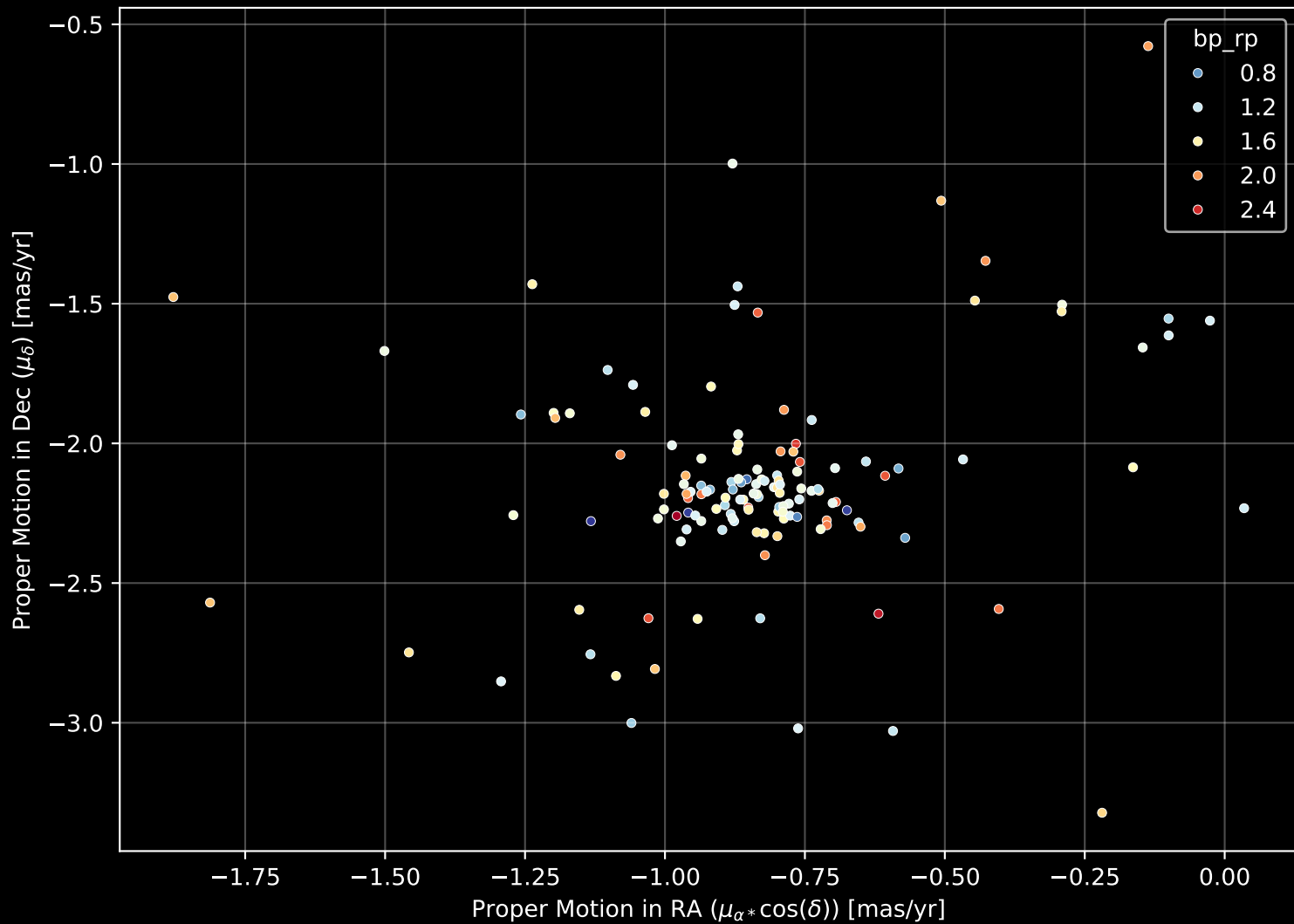
Gaia Cluster: [Stock_5] Proper Motion Diagram (n= 136)
