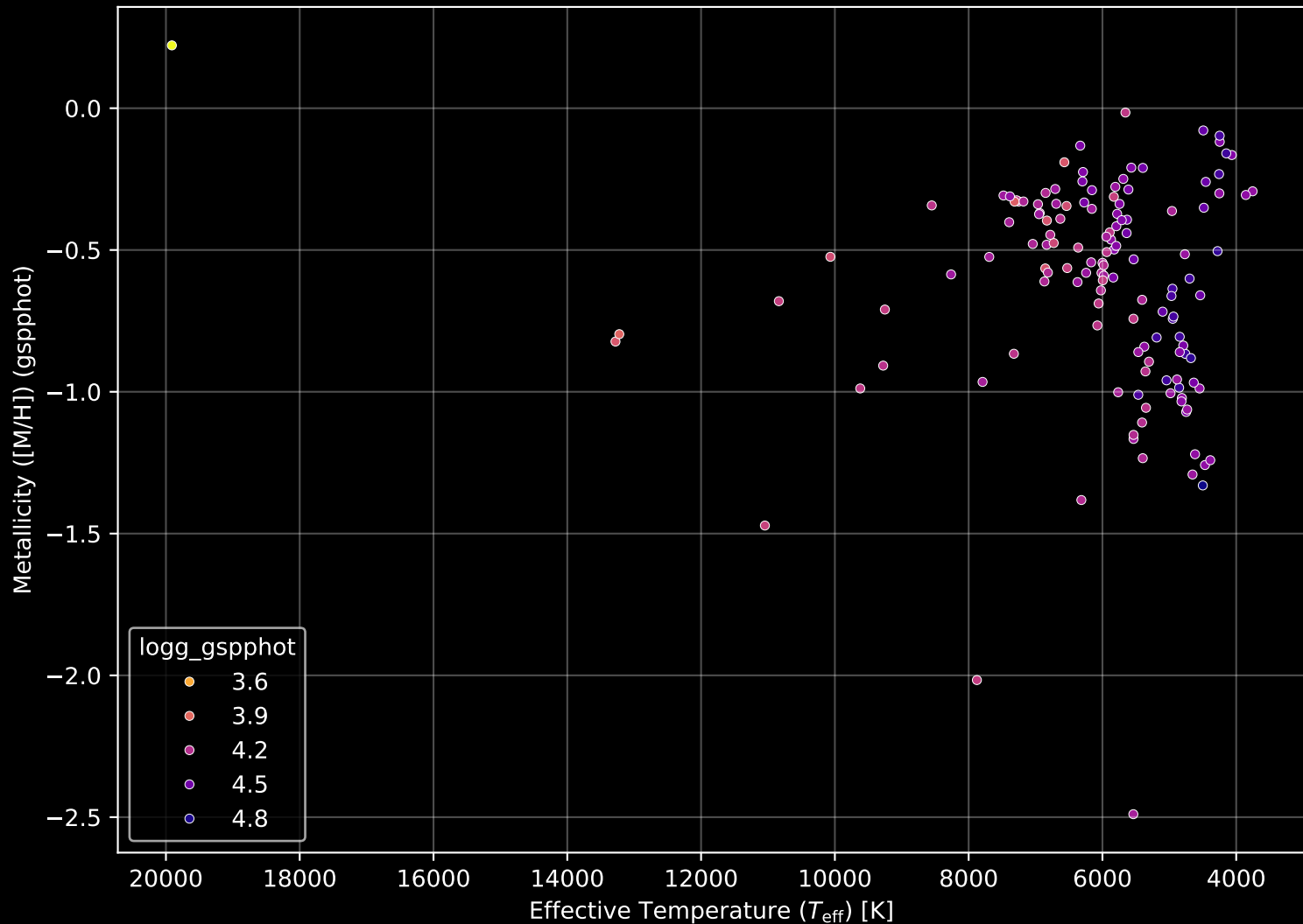
Gaia Cluster: [Stock_5] Stellar Population Parameters (n= 136)
