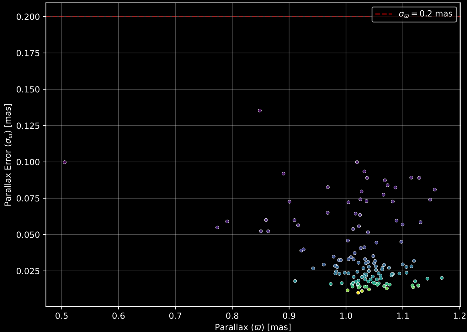
Gaia Cluster: [Stock_5] Parallax Quality (n= 136)
