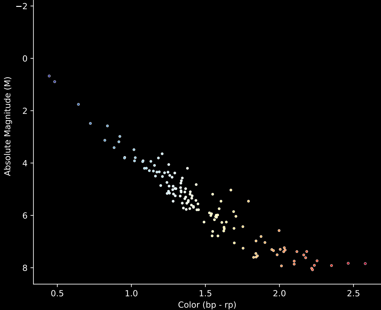
Gaia Cluster: [Stock_5] Stars (n= 136) Hertzsprung-Russel Diagram
