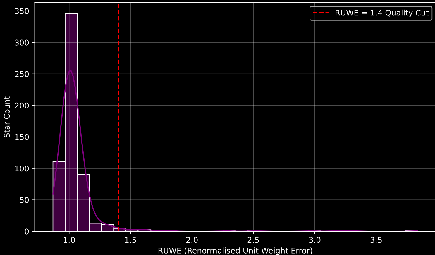
Gaia Cluster: [Stock_8] RUWE Distribution (n= 589)
