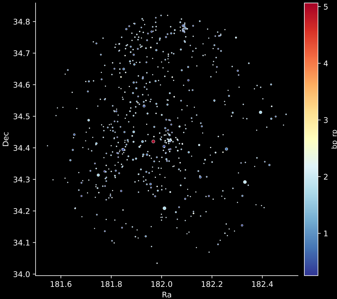
Gaia Cluster: [Stock_8] Stars: 590
