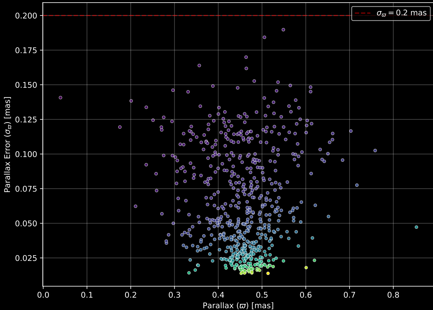
Gaia Cluster: [Stock_8] Parallax Quality (n= 590)
