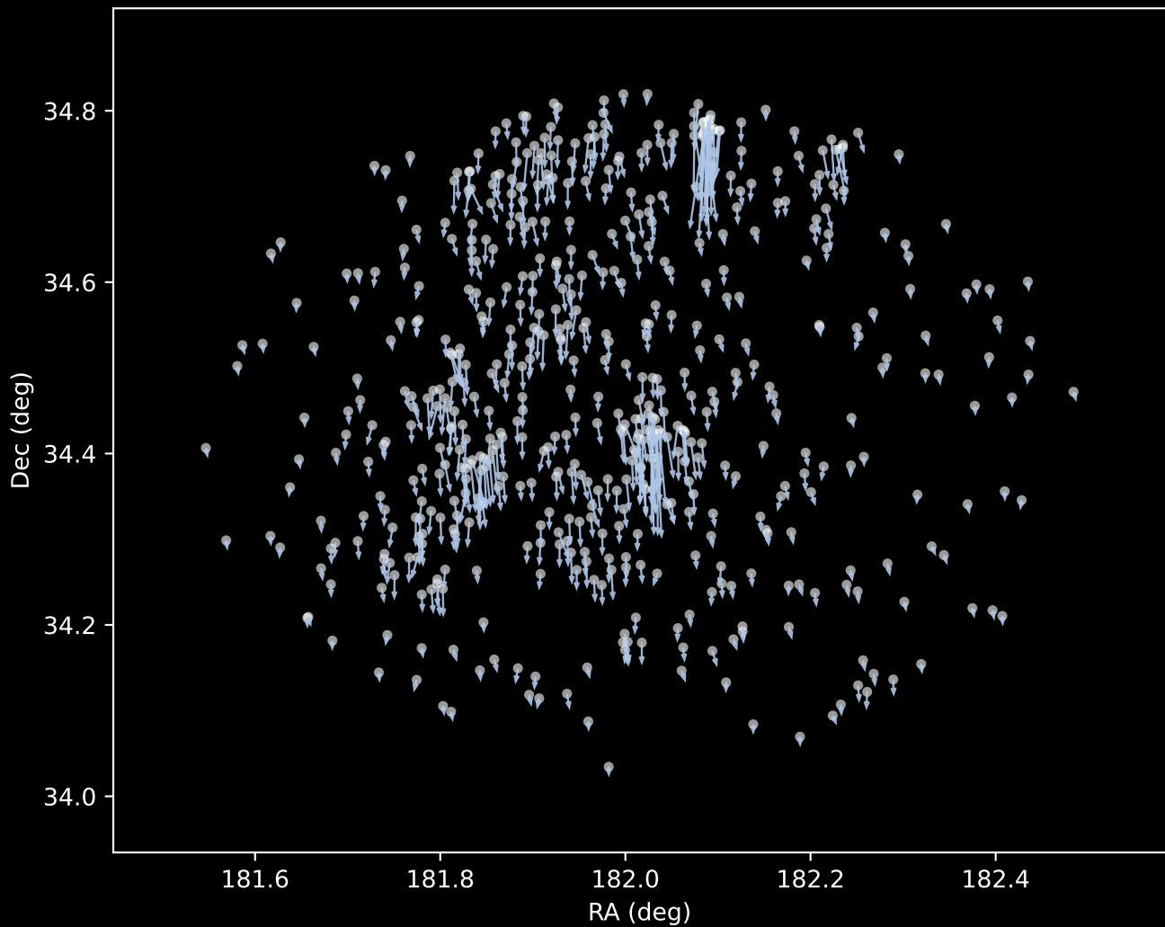
Gaia DR3 Cluster 1 Proper Motion Vectors (n=564)
