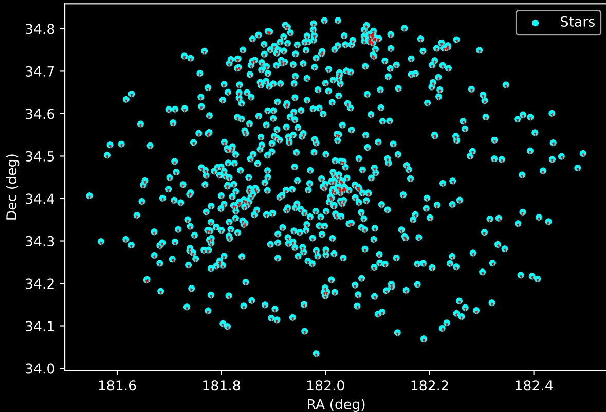
Gaia Cluster: [Stock_8] Proper Motion Vectors for Gaia Star Field (n= 590)
