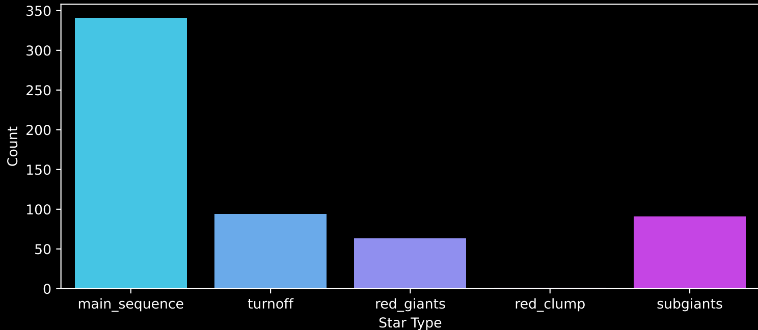
Gaia Cluster: [Stock_8] Count plot of Star Type
