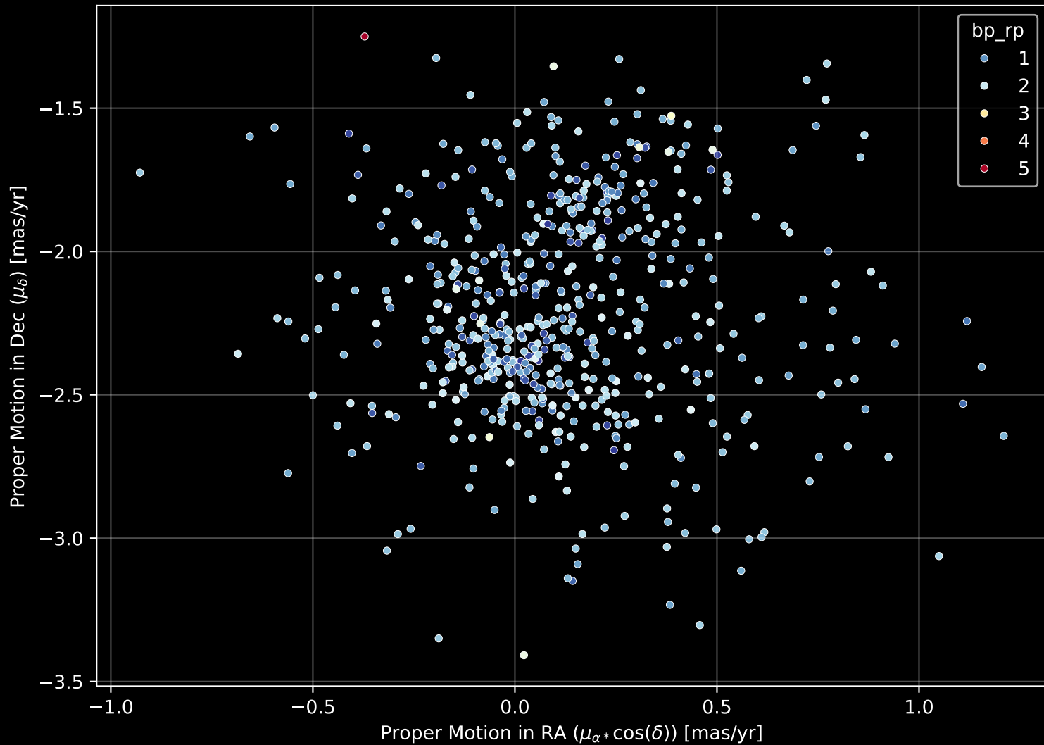
Gaia Cluster: [Stock_8] Proper Motion Diagram (n= 590)
