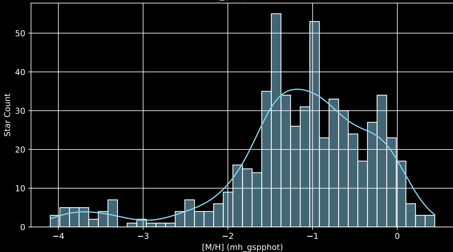
Gaia Cluster: [Stock_8 [M/H] (mh_gspphot) (n= 590)
