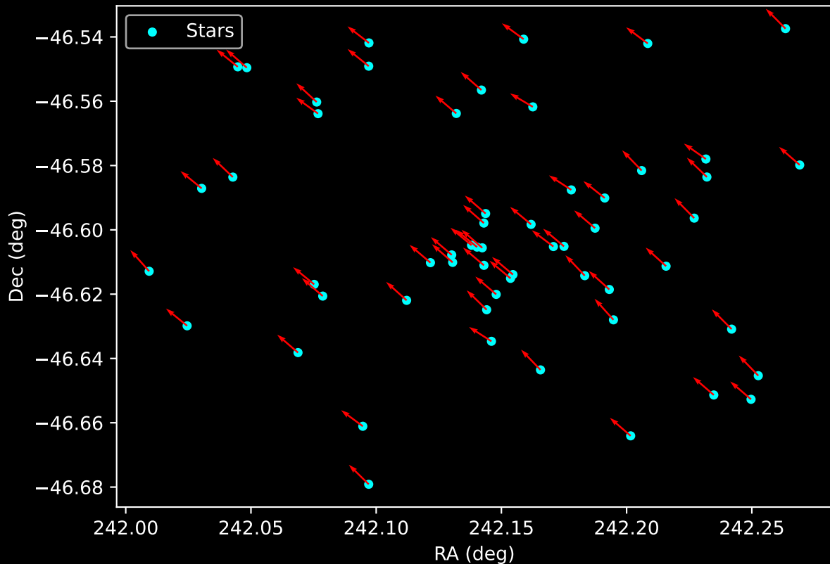
Gaia Cluster: [Teutsch_103] Proper Motion Vectors for Gaia Star Field (n= 57)
