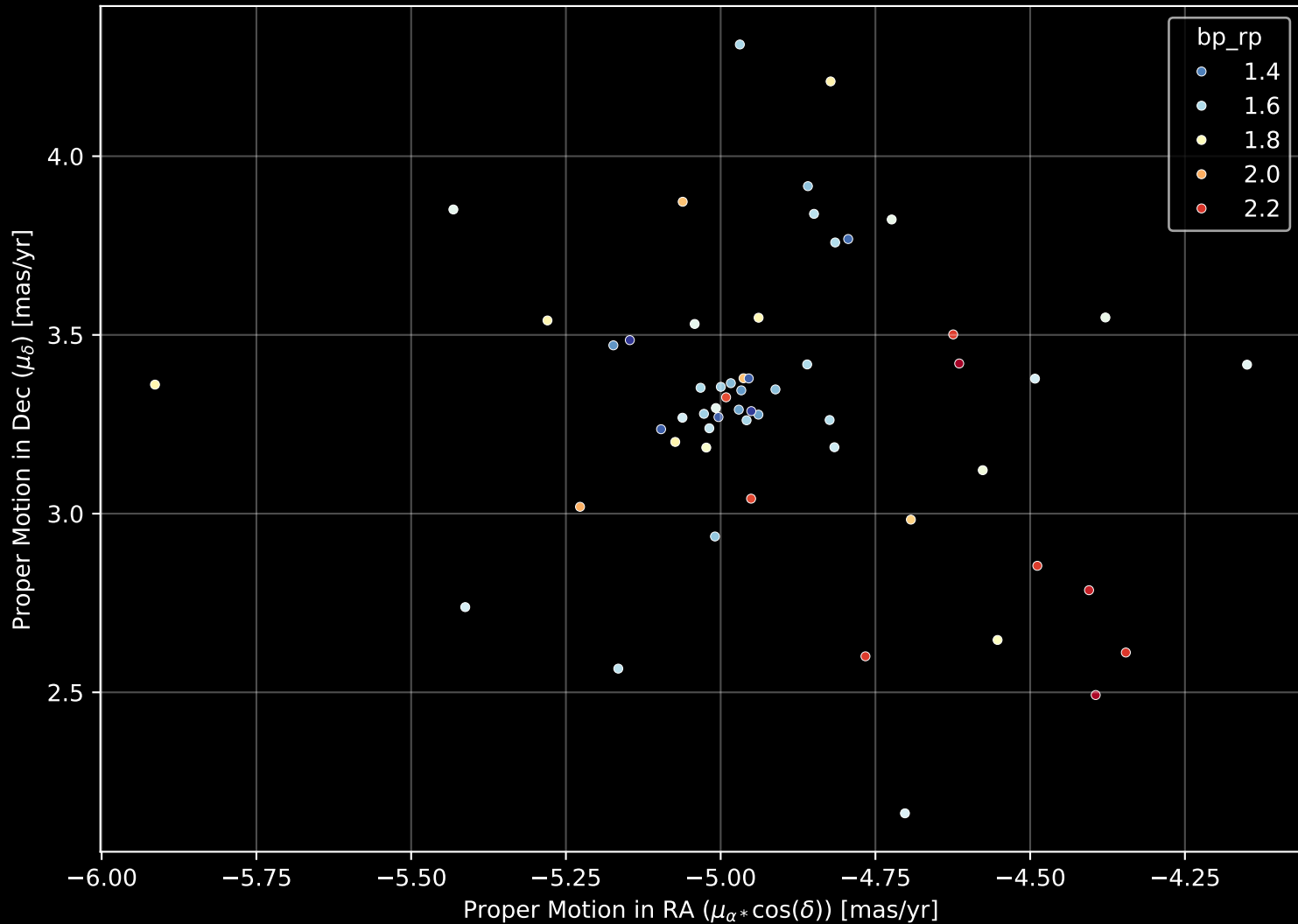
Gaia Cluster: [Deutsch_103] Proper Motion Diagram (n= 57)
