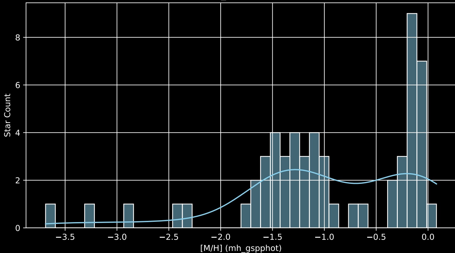
Gaia Cluster: [Deutsch_103 [M/H] (mh_gspphot) (n= 57)
