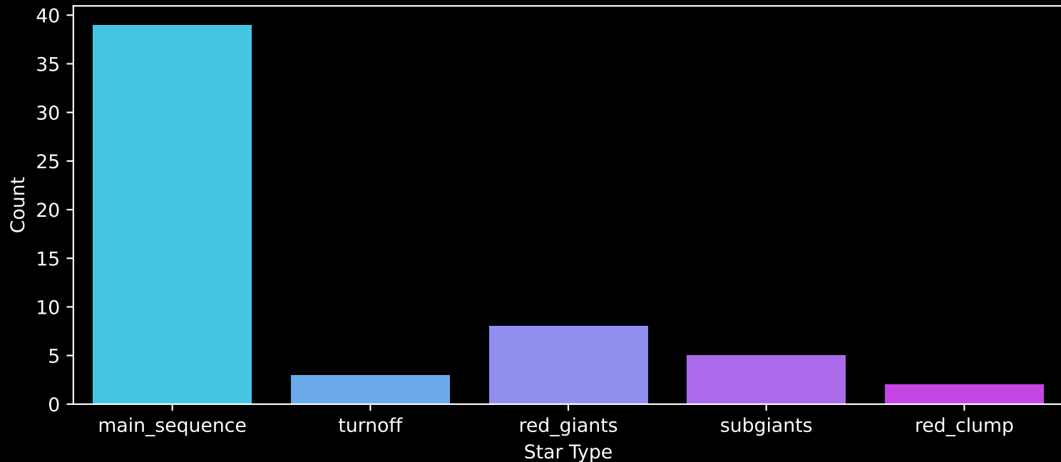
Gaia Cluster: [Teutsch_103] Count plot of Star Type
