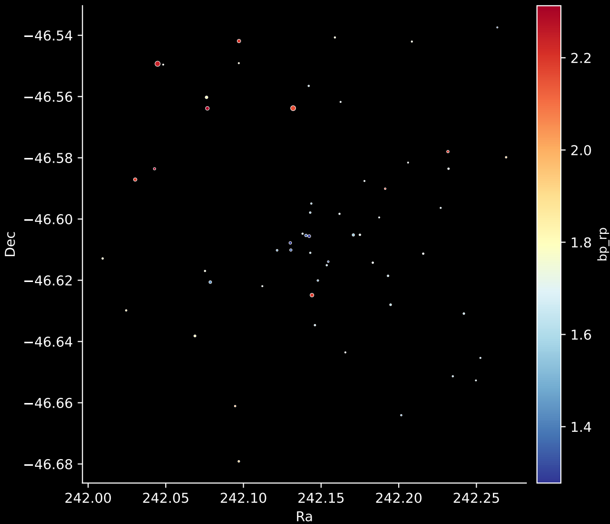
Gaia Cluster: [Teutsch_103] Stars: 57
