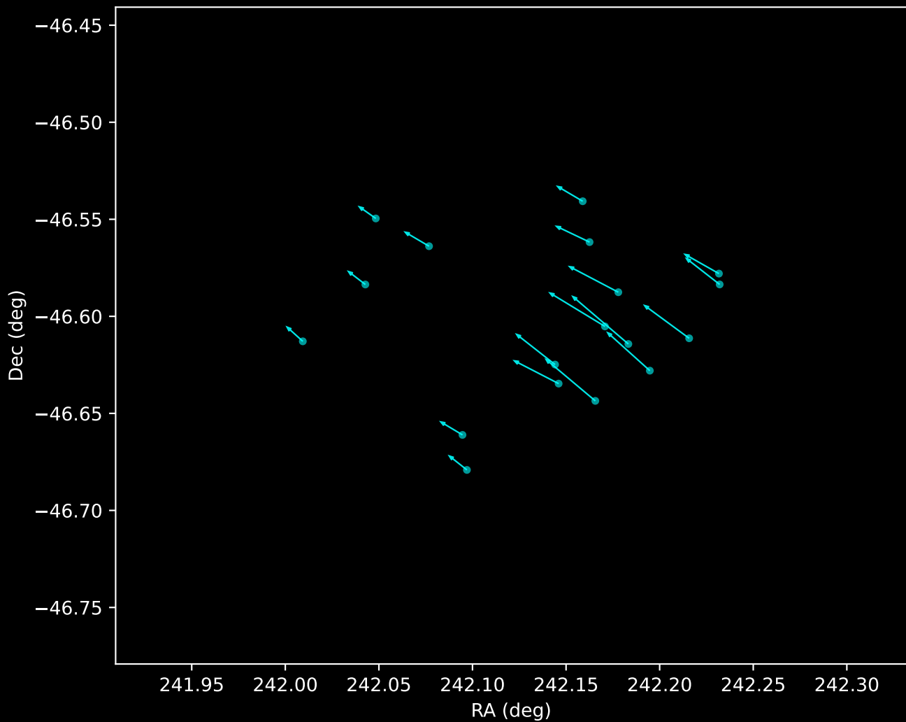
Gaia DR3 Noise Stream Proper Motion Vectors (n=18)
