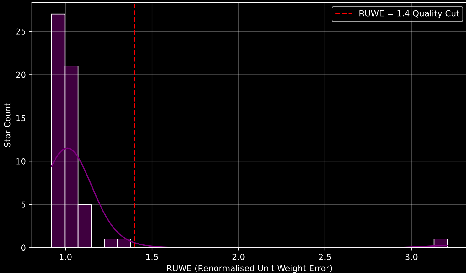
Gaia Cluster: [Teutsch_103] RUWE Distribution (n= 56)
