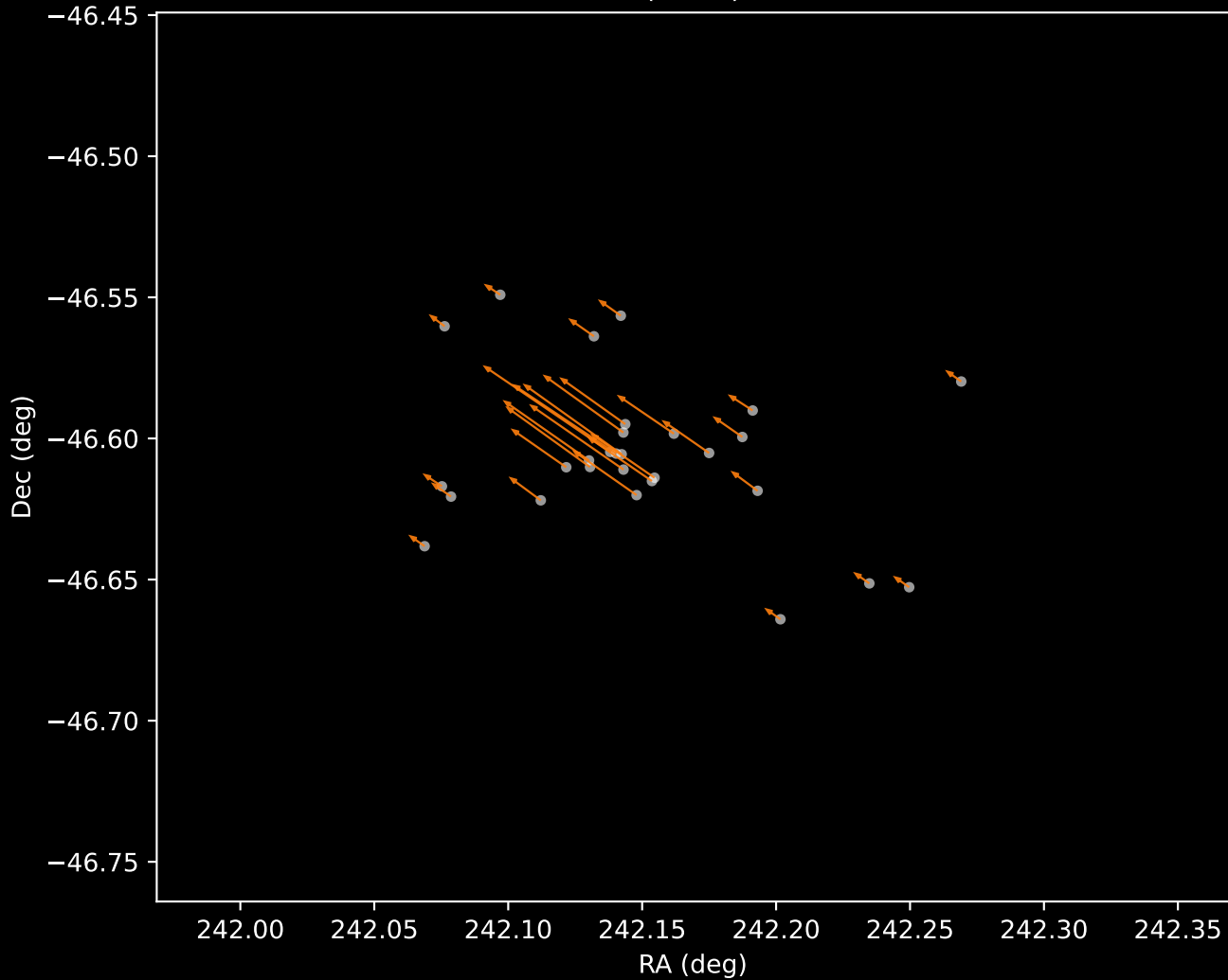
Gaia DR3 Cluster 2 Proper Motion Vectors (n=29)
