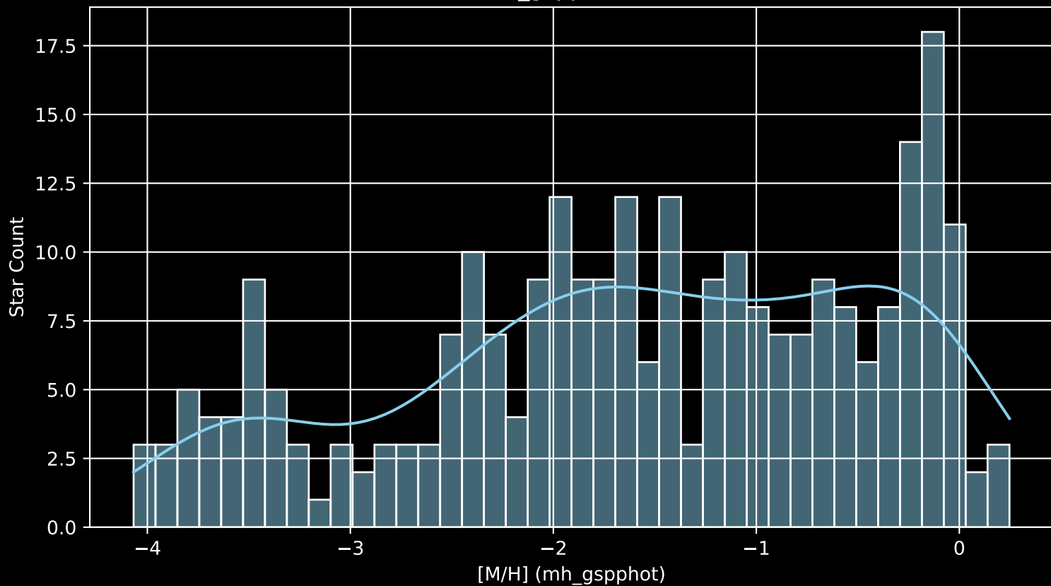
Gaia Cluster: [Deutsch_12 [M/H] (mh_gspphot) (n= 271)
