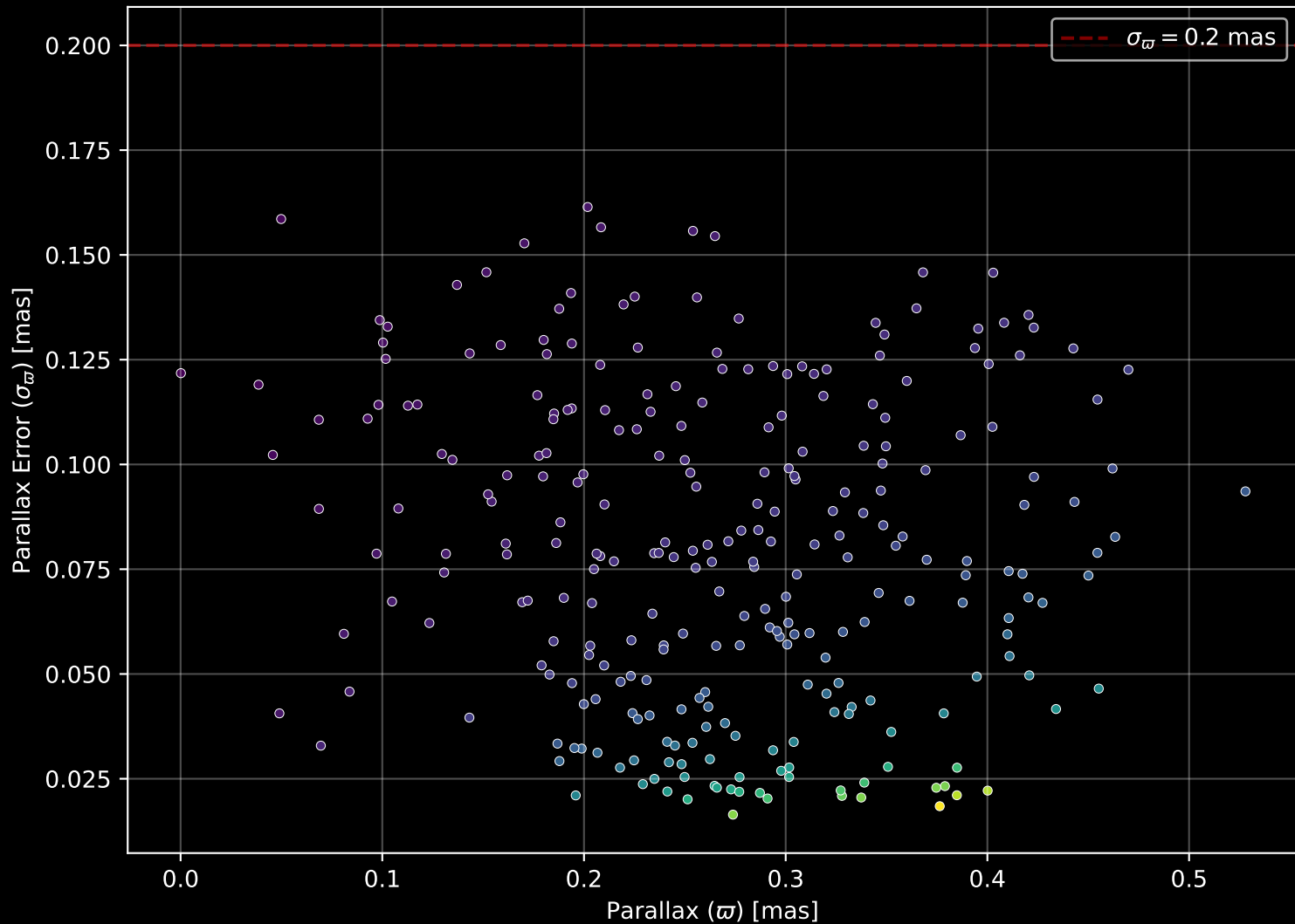
Gaia Cluster: [Deutsch_12] Parallax Quality (n= 273)
