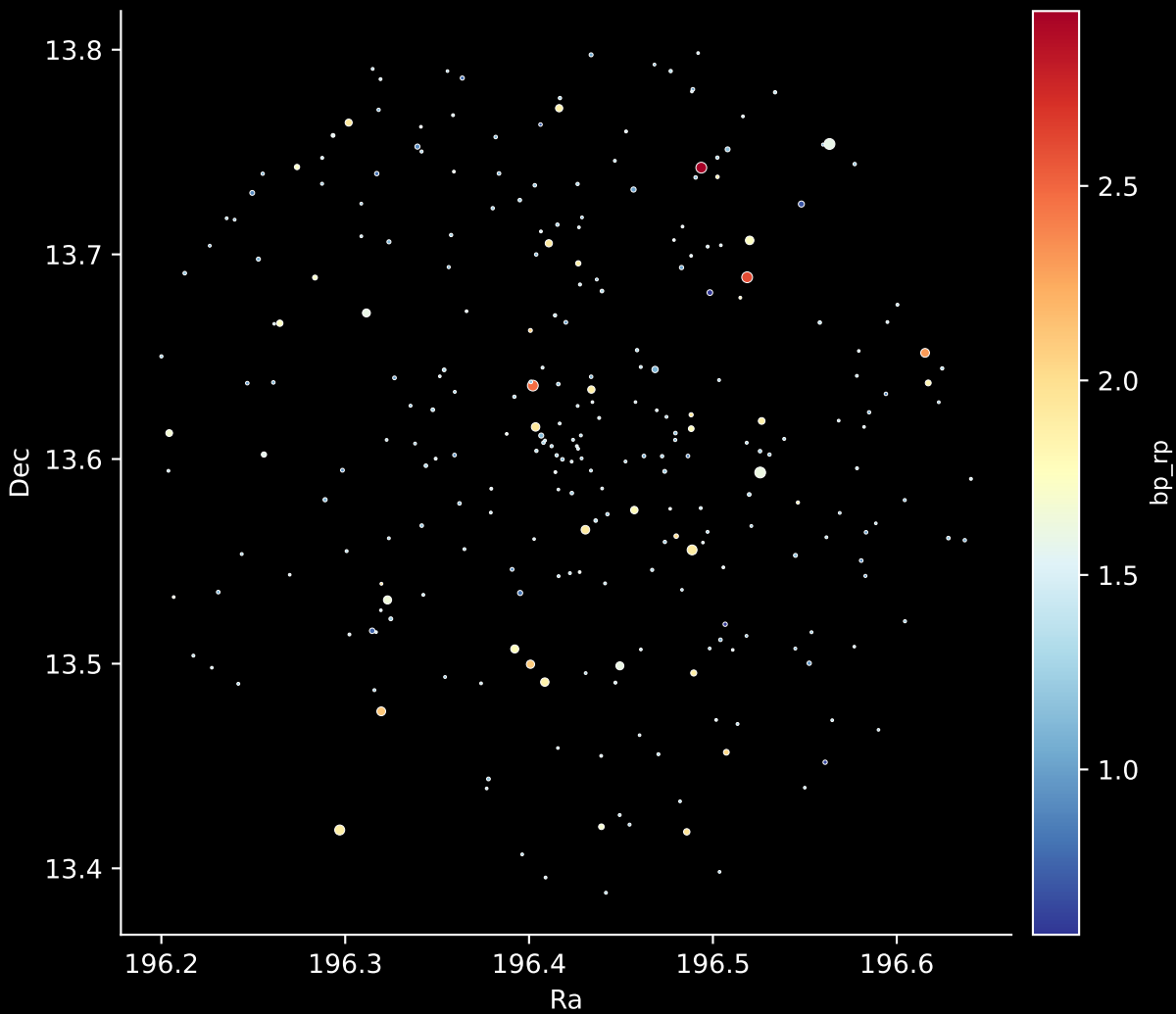
Gaia Cluster: [Teutsch_12] Stars: 273
