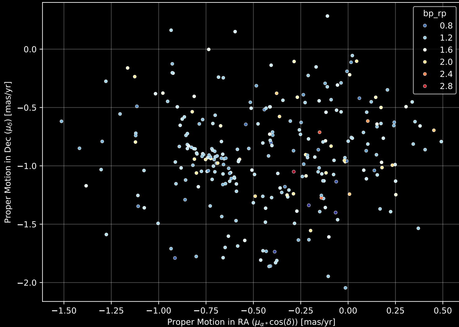
Gaia Cluster: [Deutsch_12] Proper Motion Diagram (n= 273)
