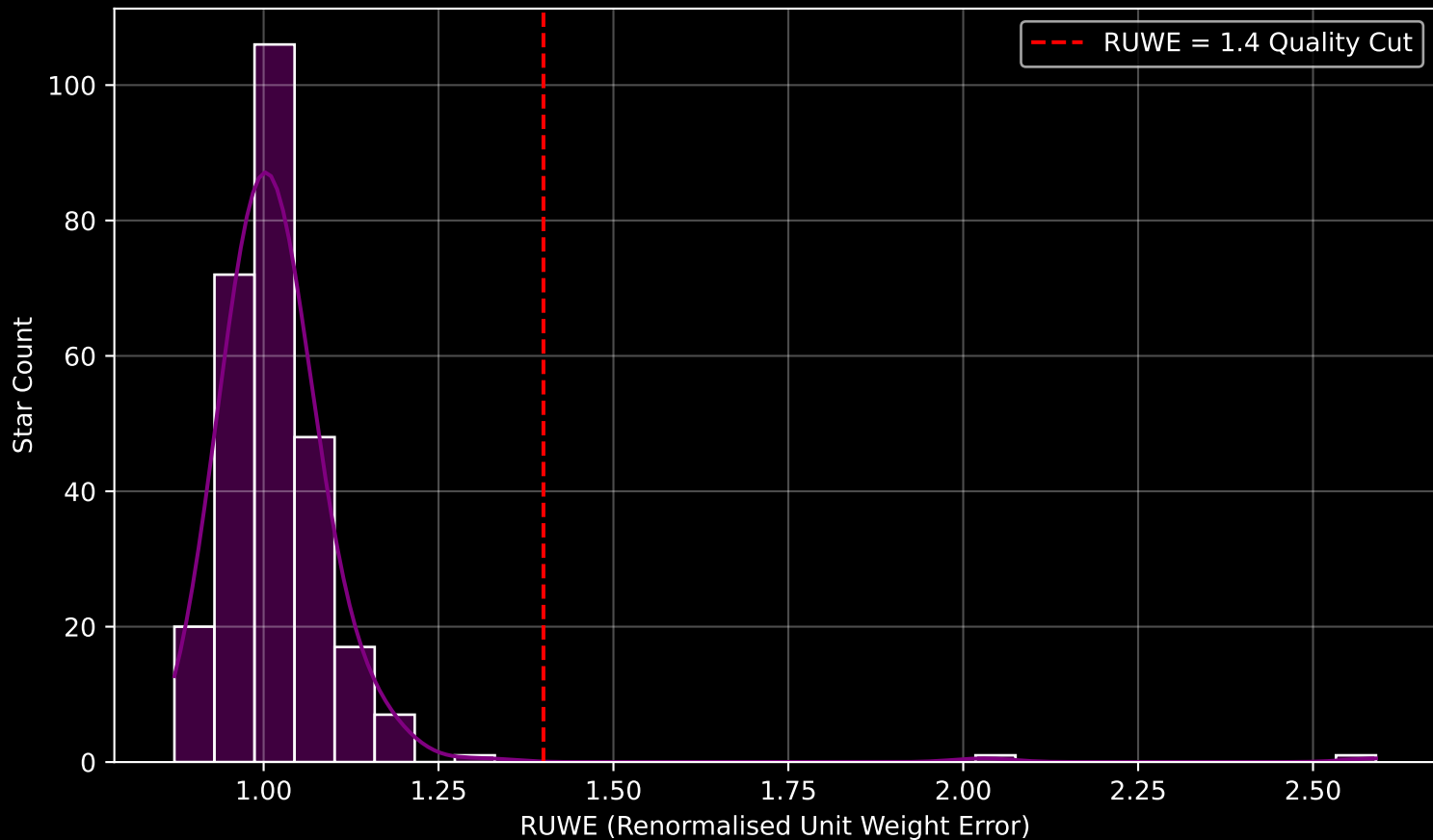
Gaia Cluster: [Teutsch_12] RUWE Distribution (n= 273)
