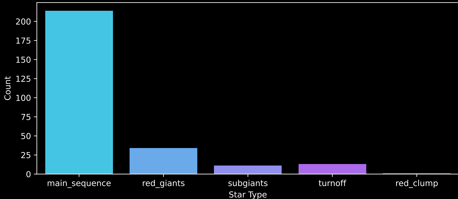
Gaia Cluster: [Teutsch_12] Count plot of Star Type
