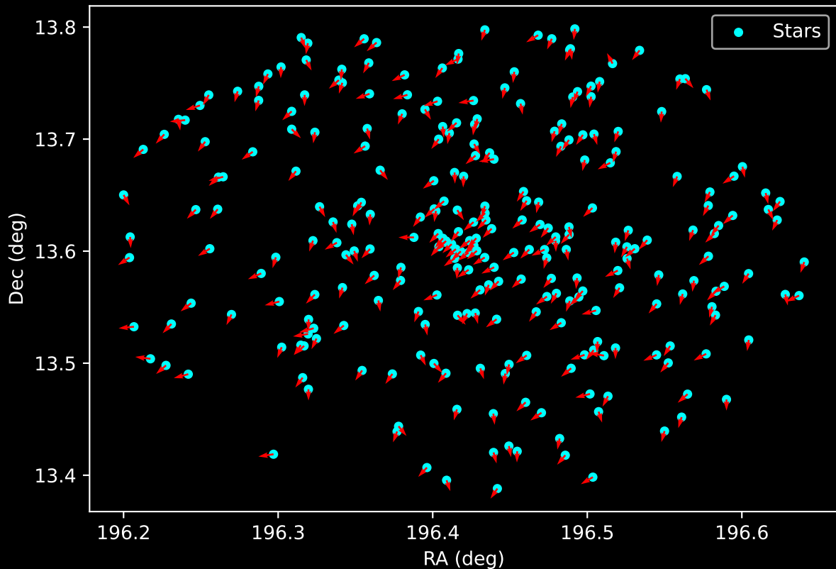
Gaia Cluster: [Deutsch_12] Proper Motion Vectors for Gaia Star Field (n= 273)
