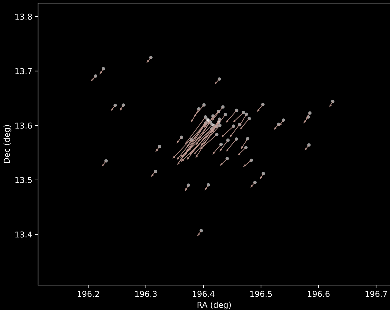
Gaia DR3 Cluster 11 Proper Motion Vectors (n=57)
