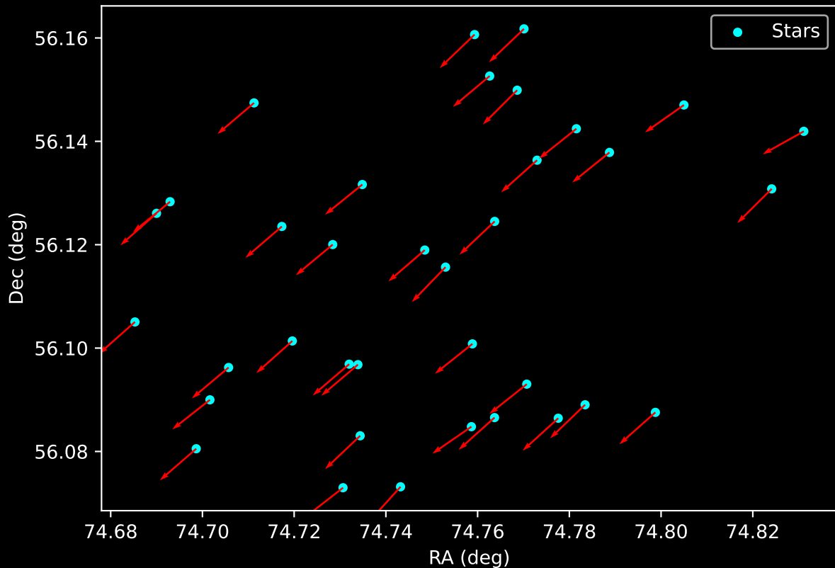
Gaia Cluster: [Teutsch_127] Proper Motion Vectors for Gaia Star Field (n= 36)
