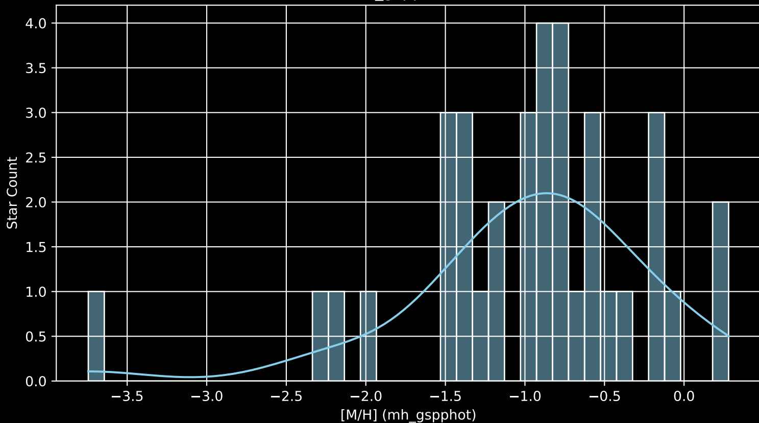
Gaia Cluster: [Teutsch_127 [M/H] (mh_gspphot) (n= 36)
