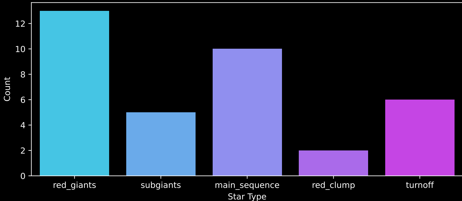
Gaia Cluster: [Teutsch_127] Count plot of Star Type
