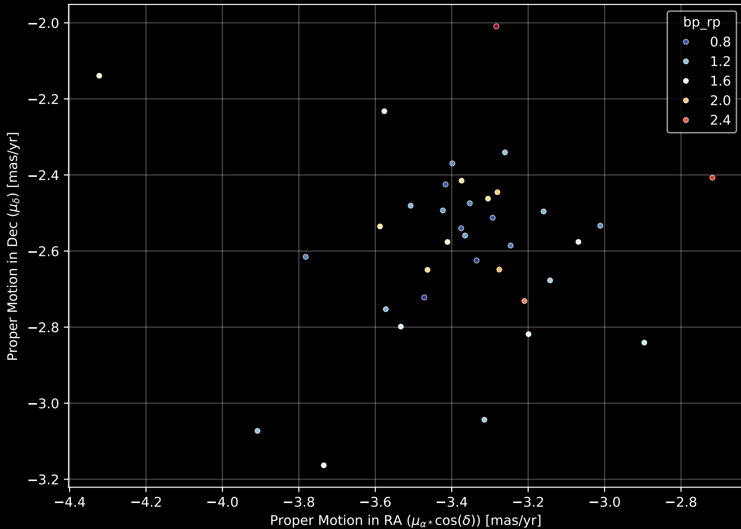
Gaia Cluster: [Deutsch_127] Proper Motion Diagram (n= 36)
