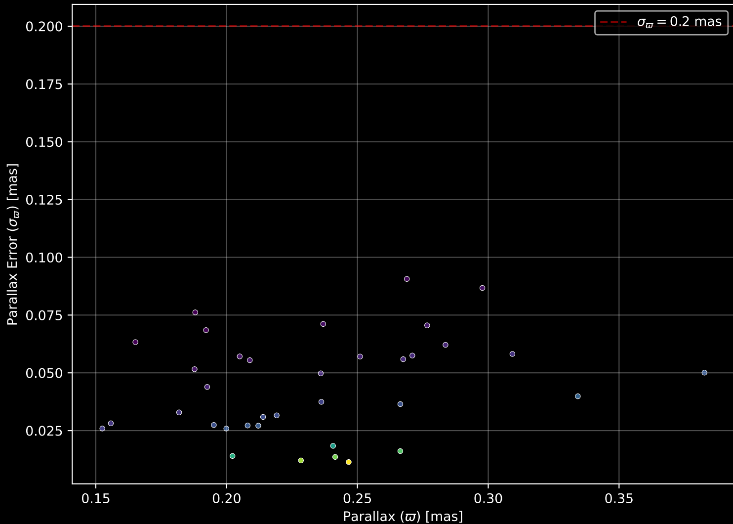
Gaia Cluster: [Teutsch_127] Parallax Quality (n= 36)
