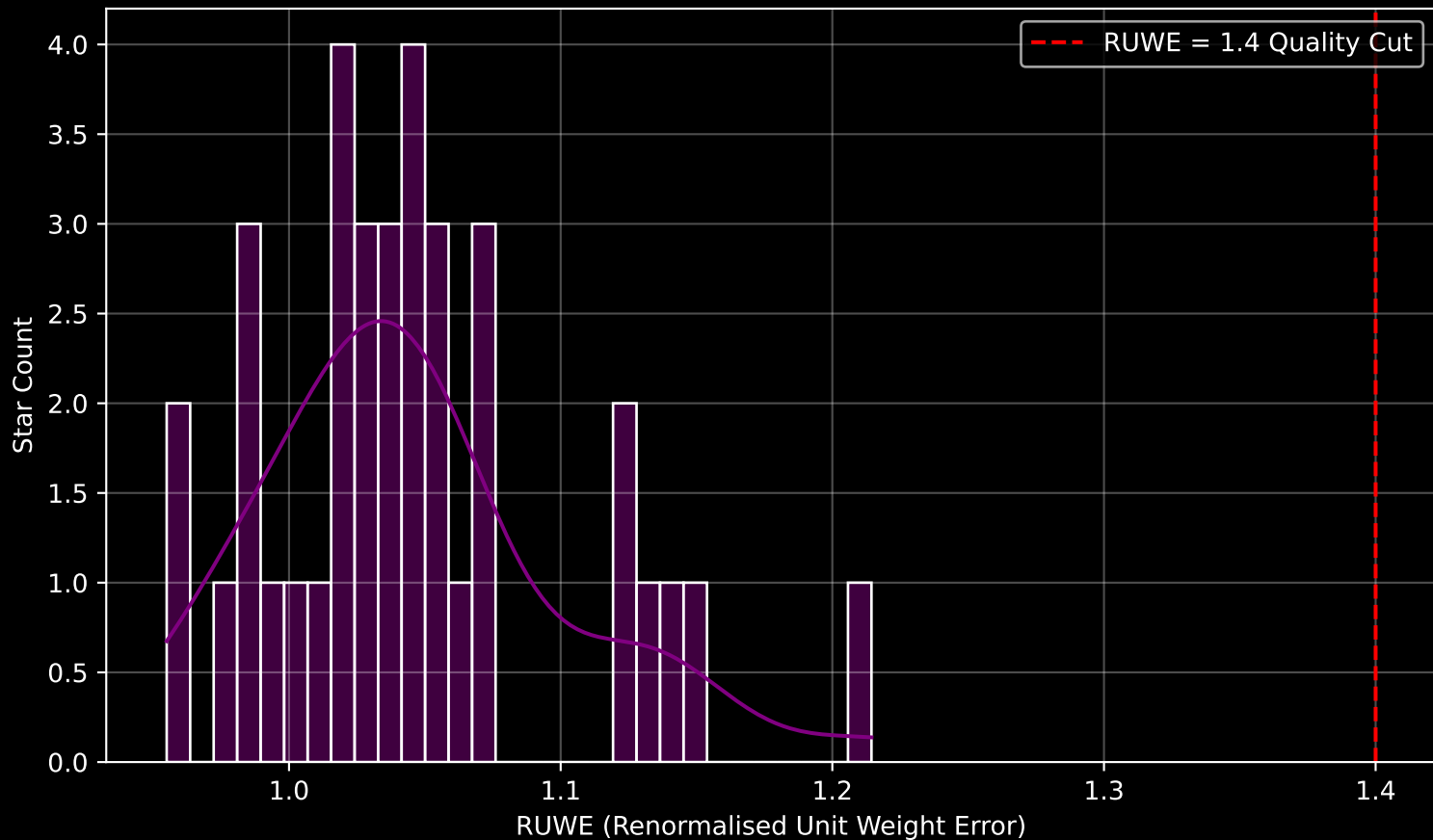
Gaia Cluster: [Teutsch_127] RUWE Distribution (n= 36)
