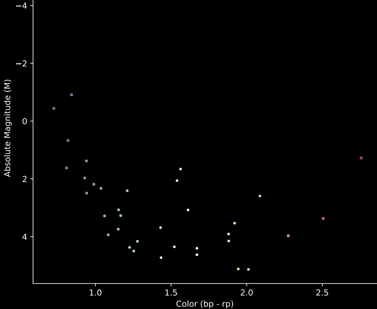
Gaia Cluster: [Teutsch_127] Stars (n= 36) Hertzsprung-Russel Diagram
