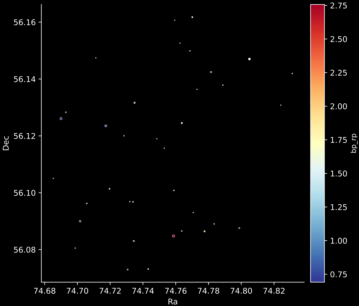
Gaia Cluster: [Teutsch_127] Stars: 36
