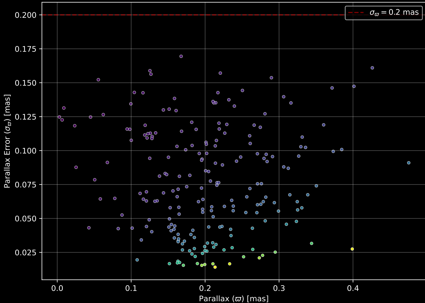
Gaia Cluster: [Teutsch_13] Parallax Quality (n= 213)
