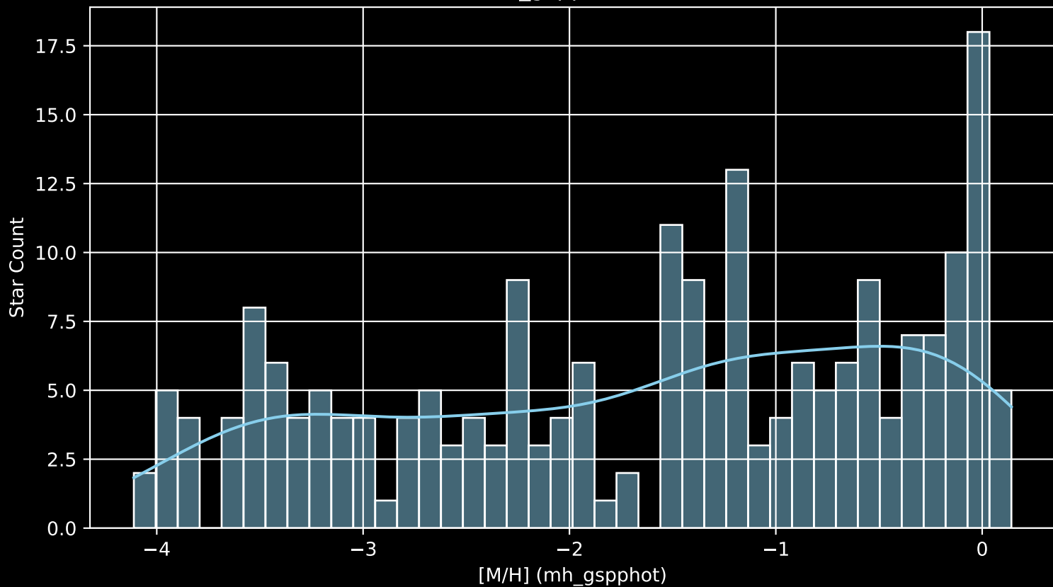
Gaia Cluster: [Teutsch_13 [M/H] (mh_gspphot) (n= 213)
