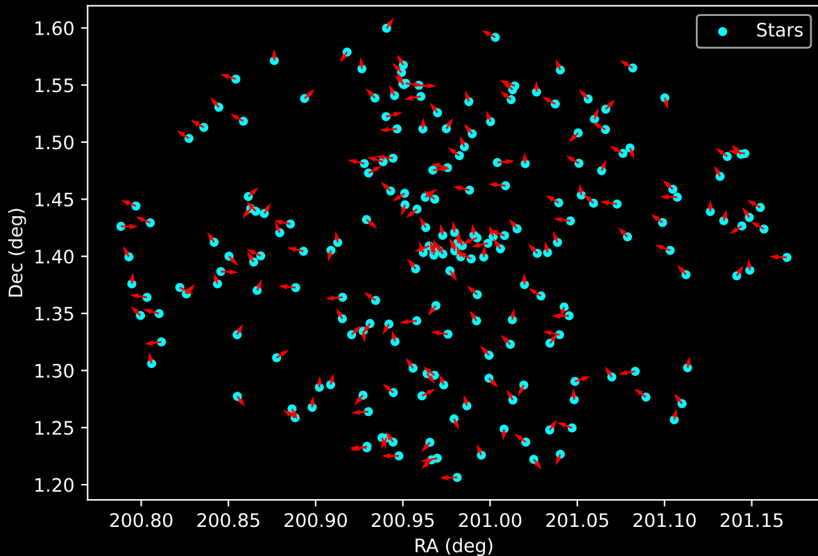
Gaia Cluster: [Teutsch_13] Proper Motion Vectors for Gaia Star Field (n= 213)
