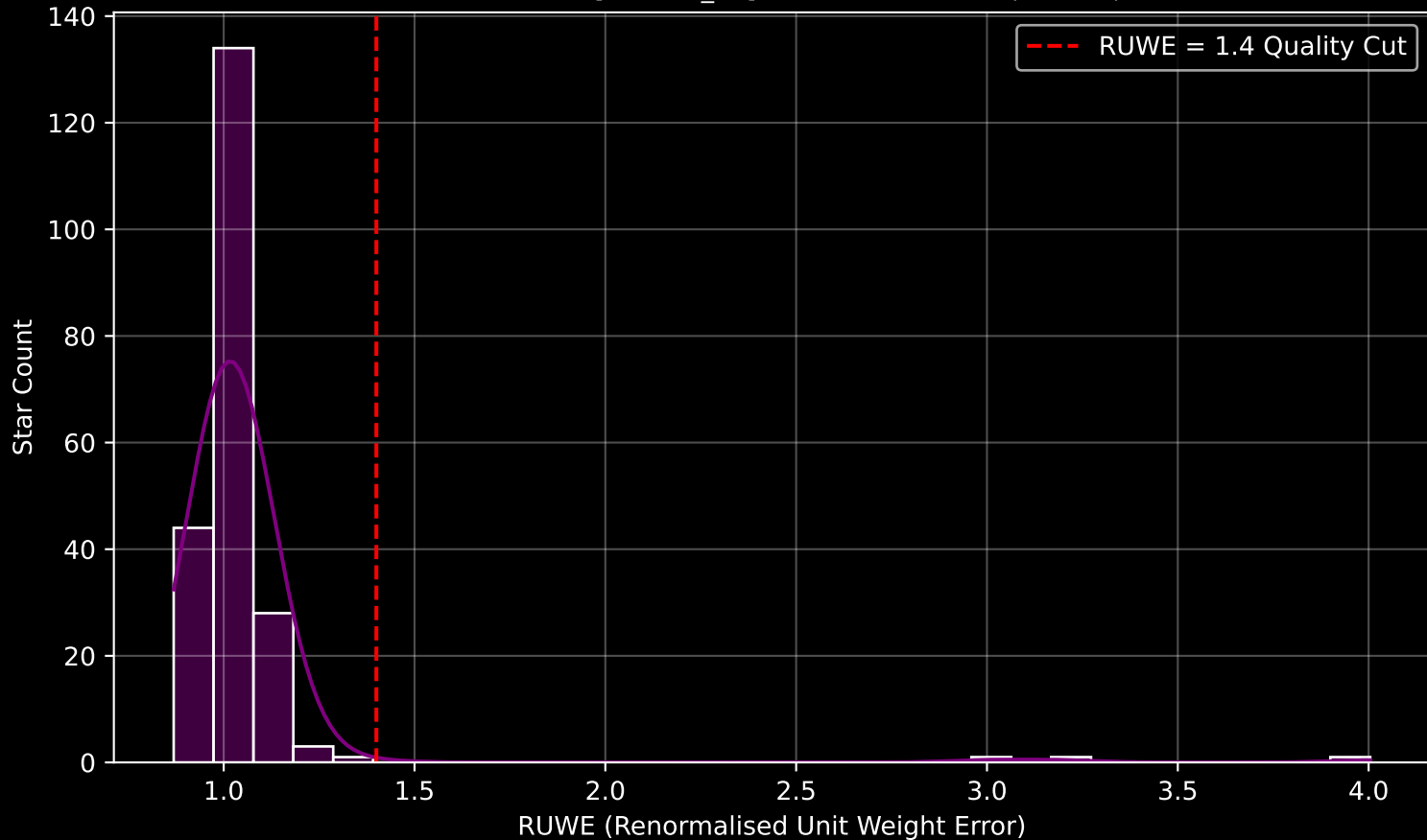
Gaia Cluster: [Teutsch_13] RUWE Distribution (n= 213)
