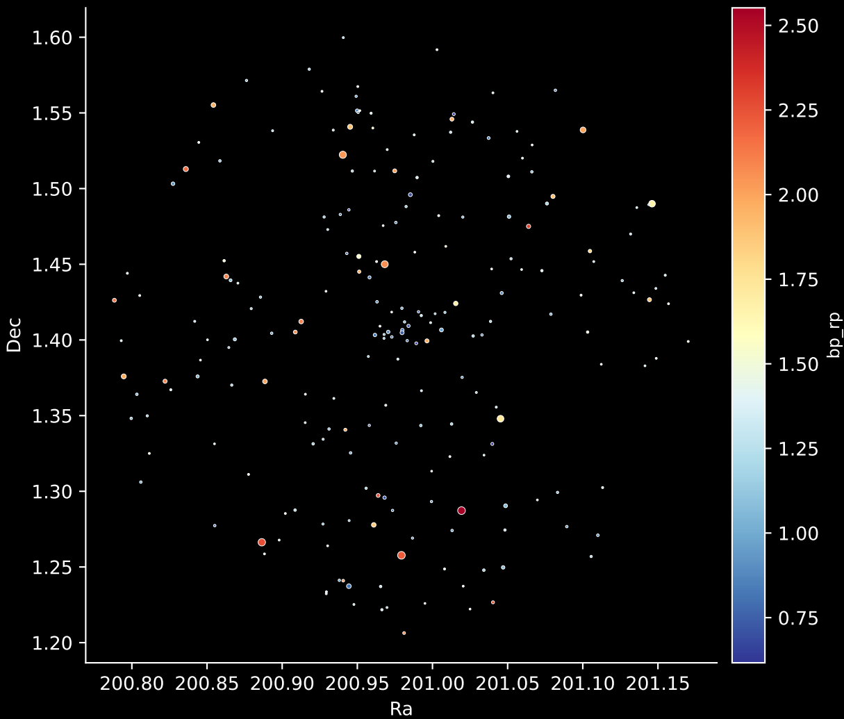
Gaia Cluster: [Teutsch_13] Stars: 213
