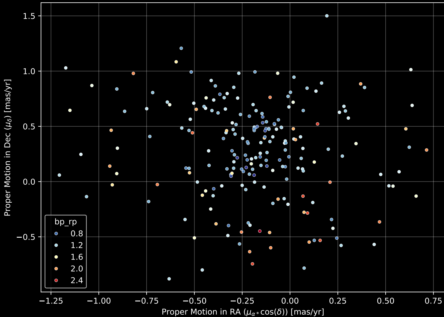
Gaia Cluster: [Deutsch_13] Proper Motion Diagram (n= 213)
