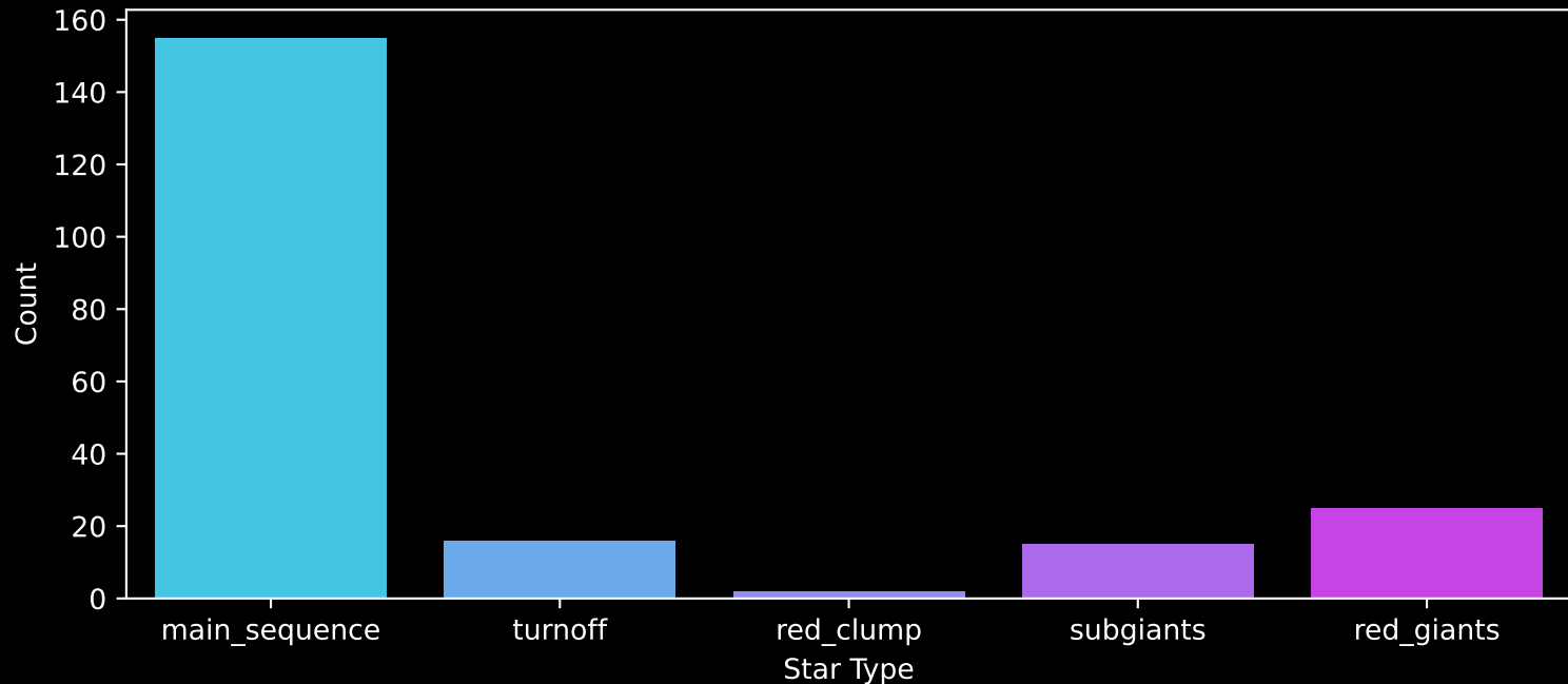
Gaia Cluster: [Teutsch_13] Count plot of Star Type
