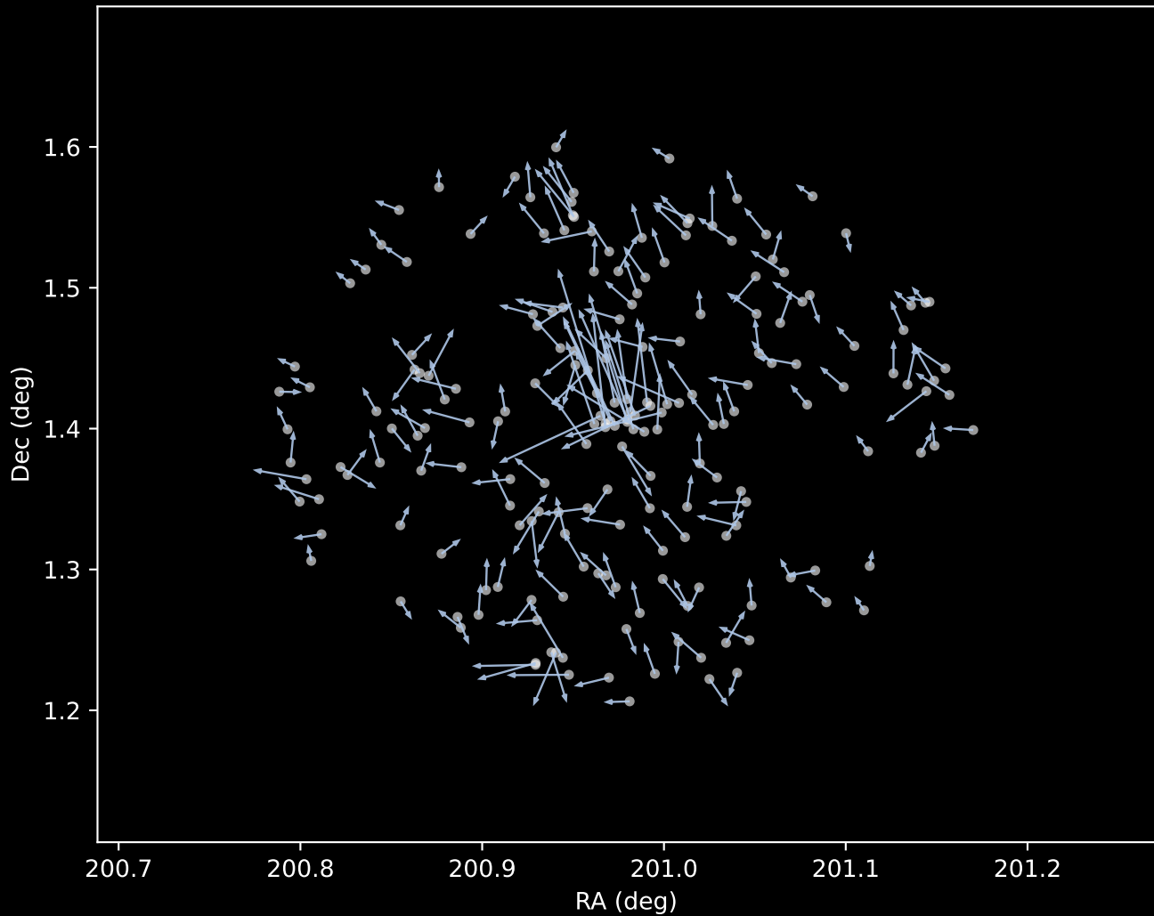
Gaia DR3 Cluster 1 Proper Motion Vectors (n=195)
