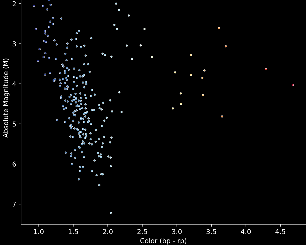
Gaia Cluster: [Teutsch_144] Stars (n= 243) Hertzsprung-Russel Diagram
