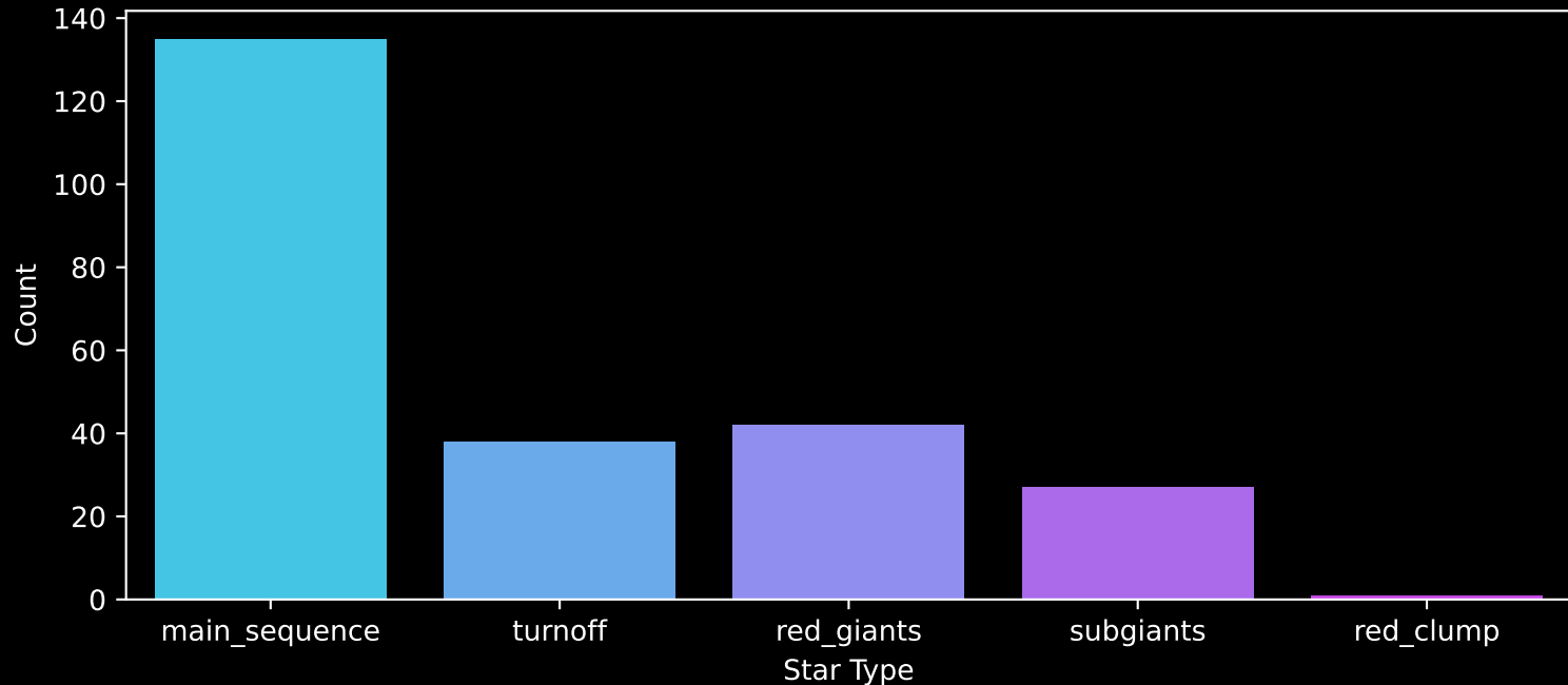
Gaia Cluster: [Teutsch_144] Count plot of Star Type
