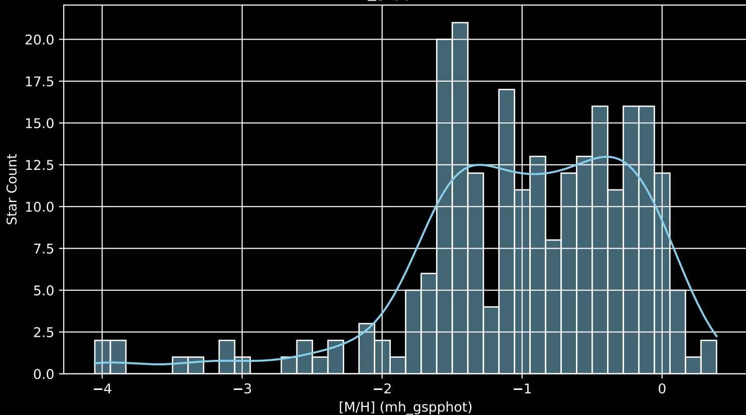
Gaia Cluster: [Teutsch_144 [M/H] (mh_gspphot) (n= 242)
