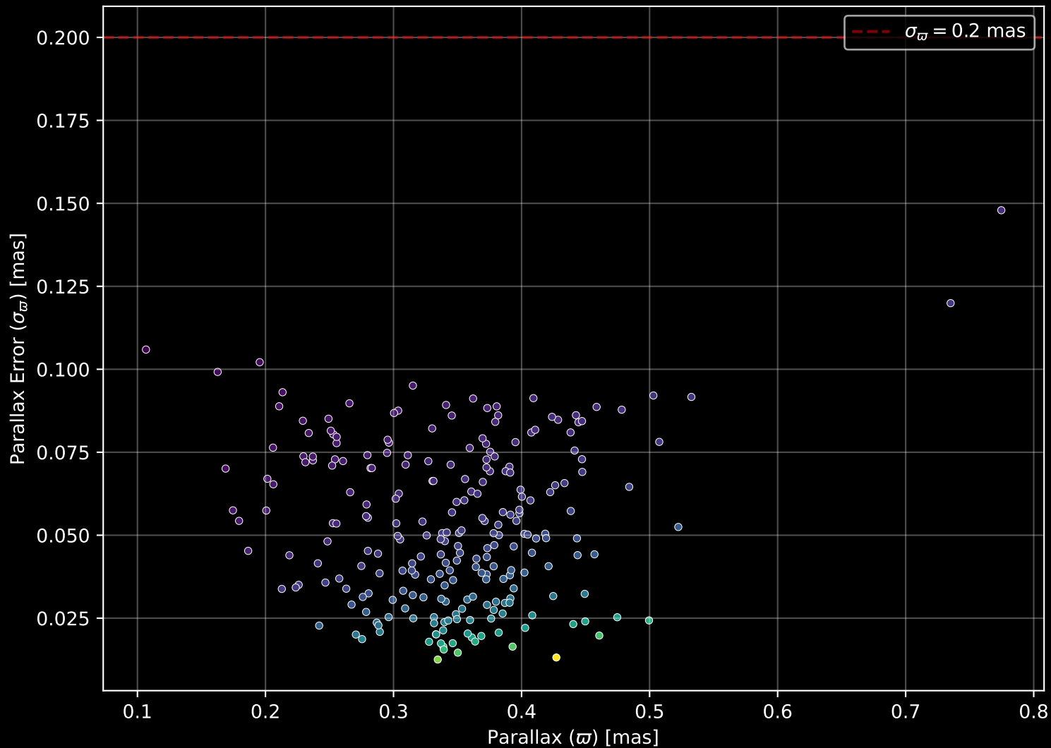
Gaia Cluster: [Teutsch_144] Parallax Quality (n= 243)
