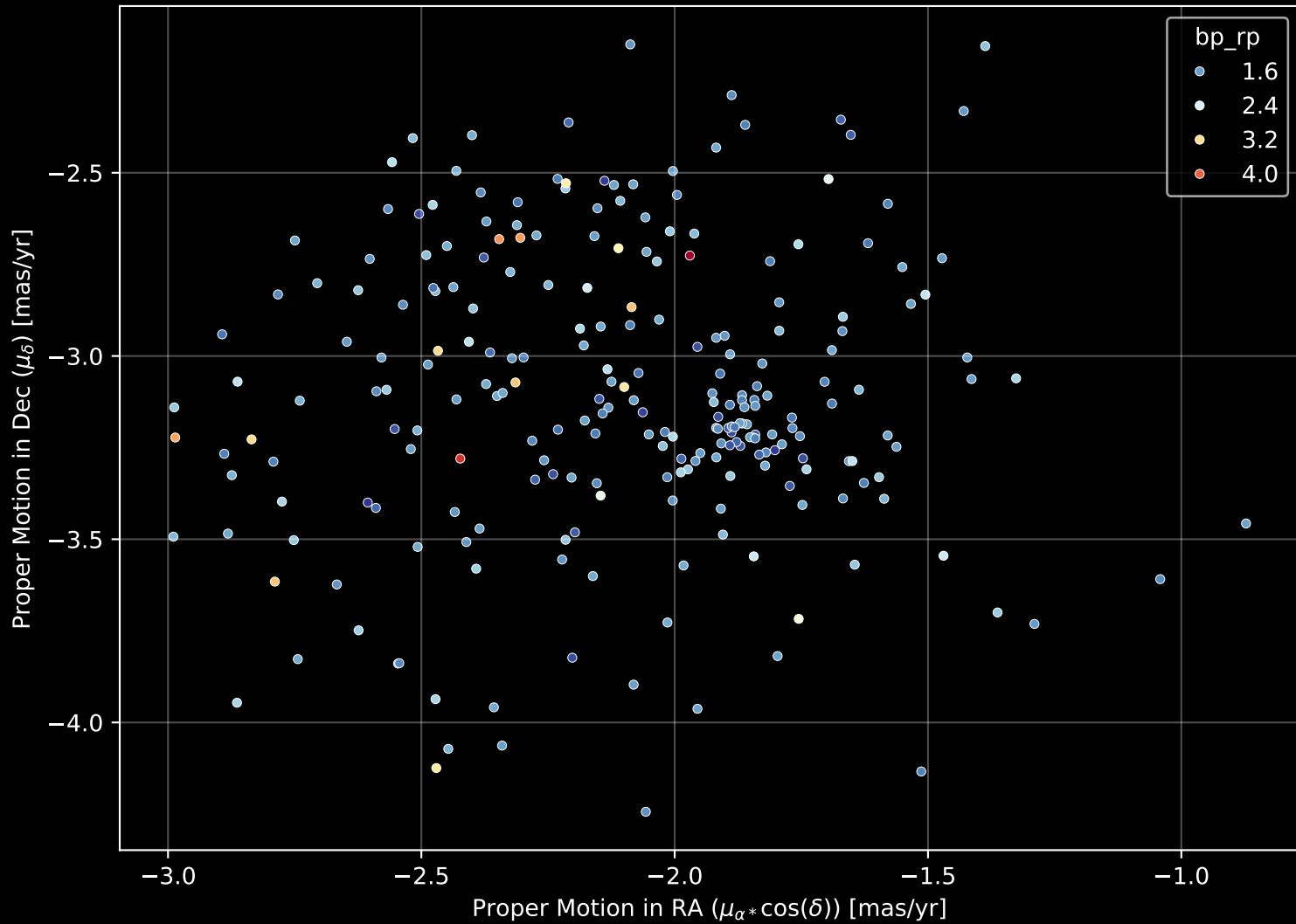
Gaia Cluster: [Teutsch_144] Proper Motion Diagram (n= 243)
