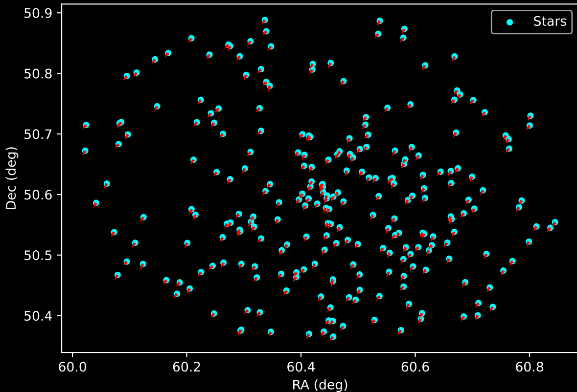
Gaia Cluster: [Teutsch_144] Proper Motion Vectors for Gaia Star Field (n= 243)
