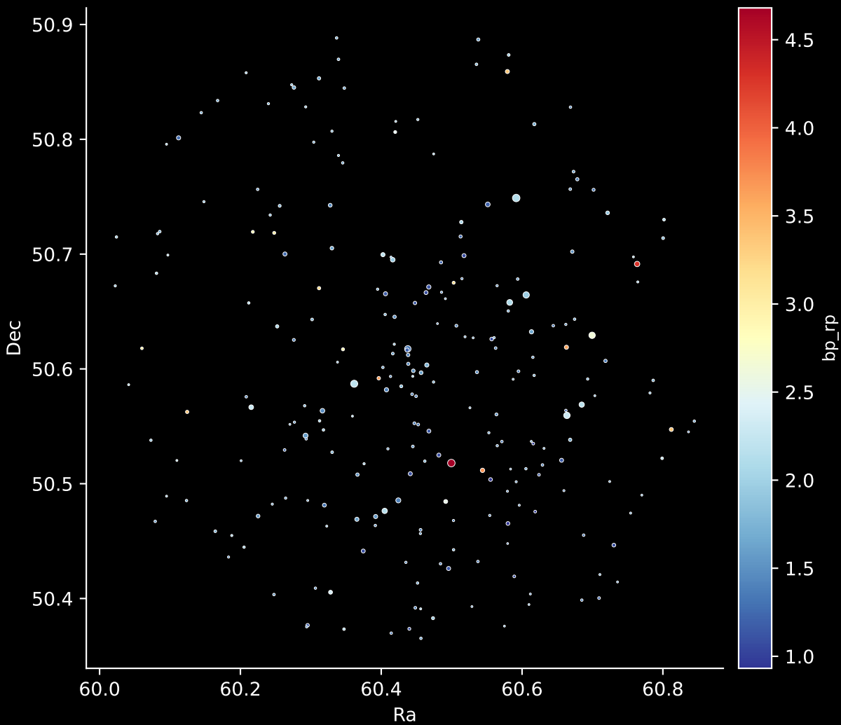
Gaia Cluster: [Teutsch_144] Stars: 243
