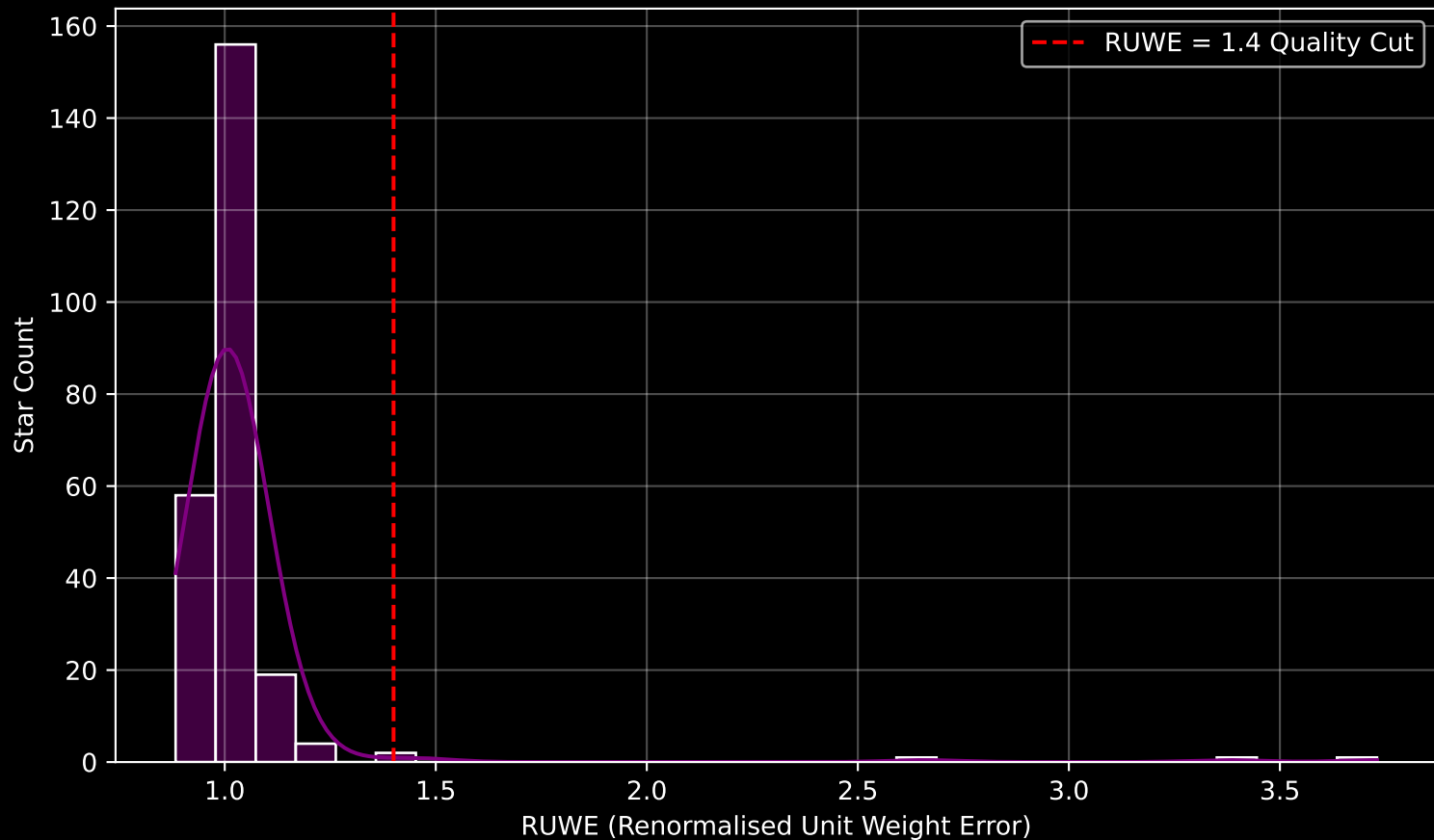
Gaia Cluster: [Teutsch_144] RUWE Distribution (n= 242)
