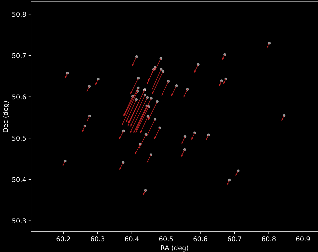
Gaia DR3 Cluster 6 Proper Motion Vectors (n=49)
