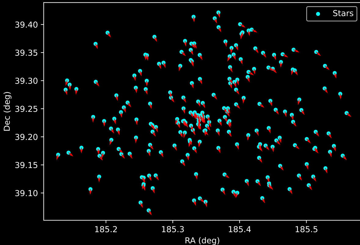
Gaia Cluster: [Teutsch_2] Proper Motion Vectors for Gaia Star Field (n= 212)
