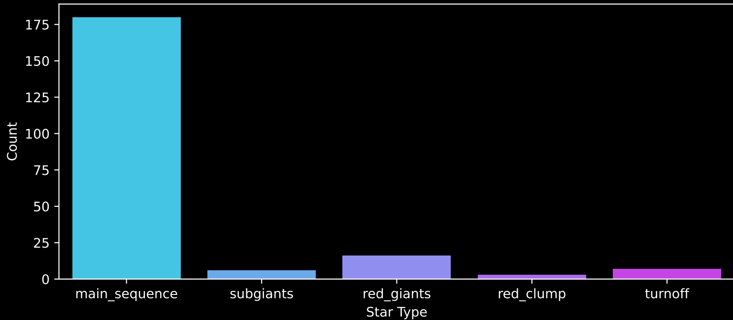
Gaia Cluster: [Teutsch_2] Count plot of Star Type
