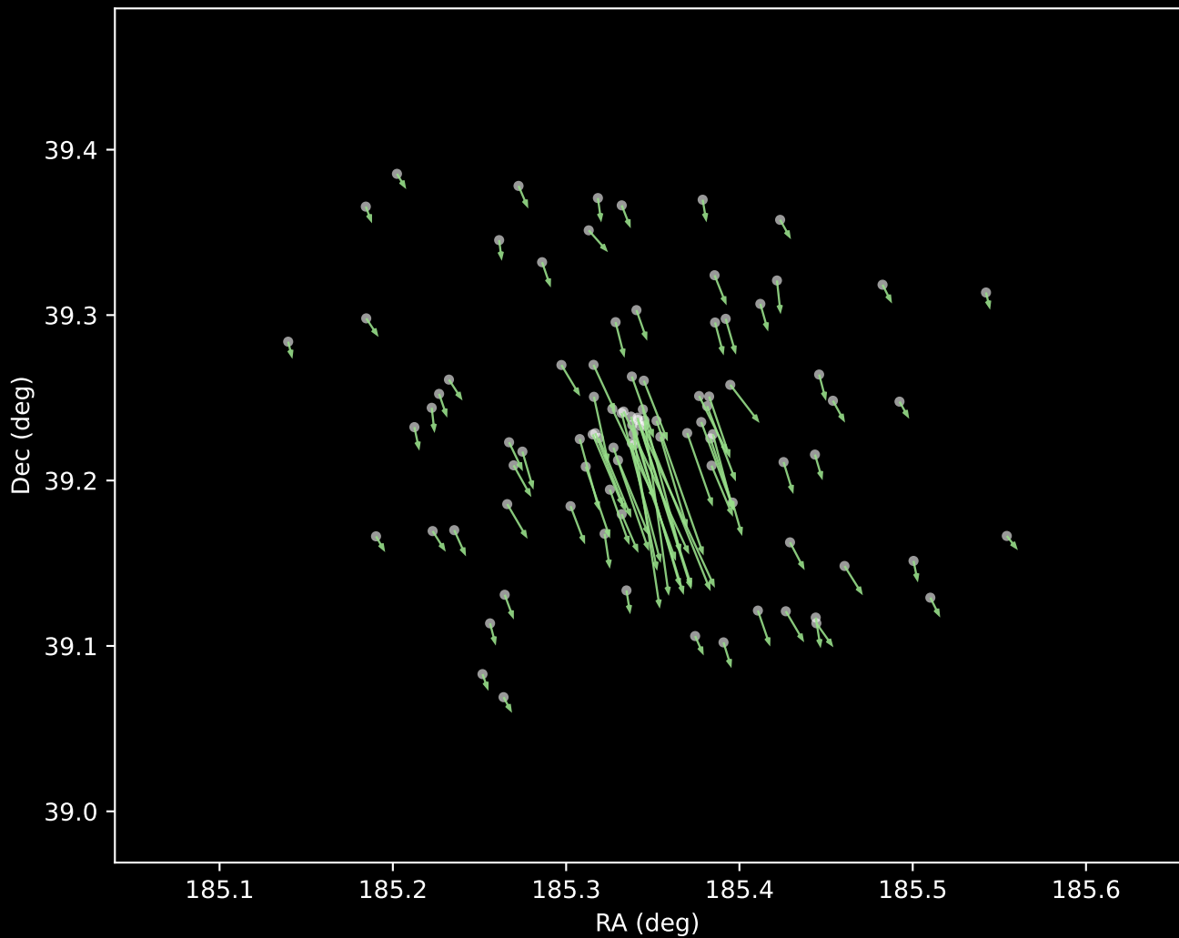
Gaia DR3 Cluster 5 Proper Motion Vectors (n=95)
