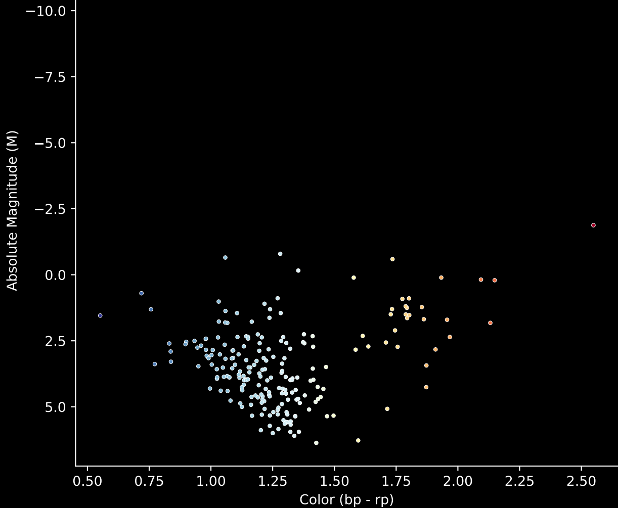
Gaia Cluster: [Teutsch_2] Stars (n= 212) Hertzsprung-Russel Diagram
