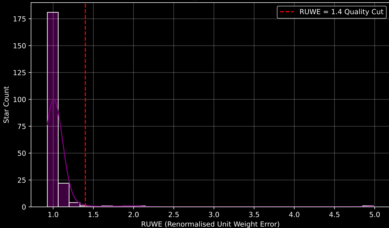
Gaia Cluster: [Teutsch_2] RUWE Distribution (n= 212)
