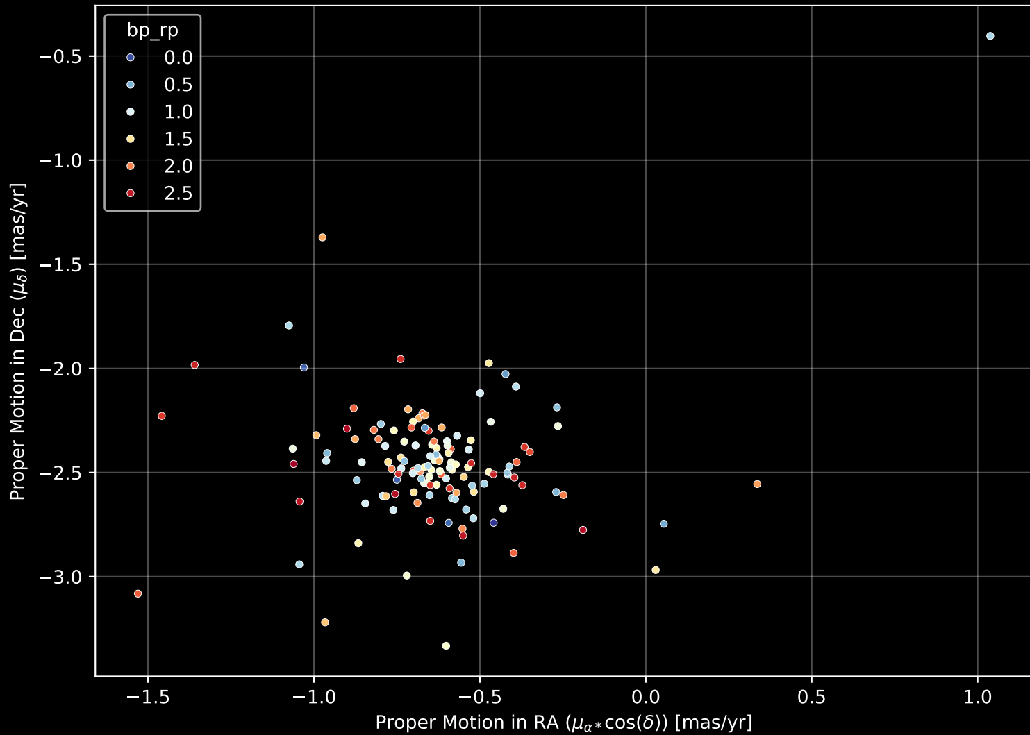
Gaia Cluster: [Teutsch_35] Proper Motion Diagram (n= 135)
