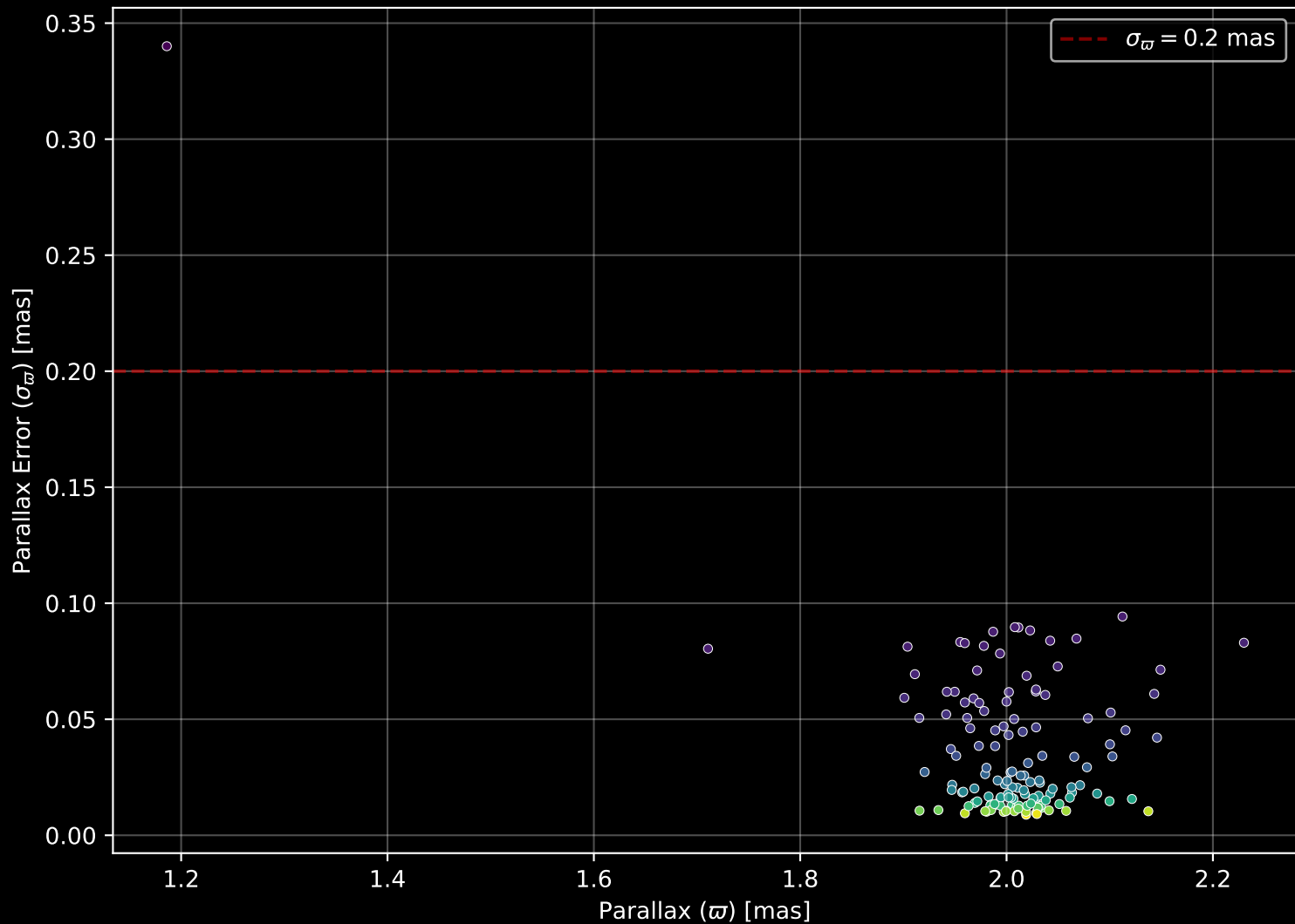
Gaia Cluster: [Teutsch_35] Parallax Quality (n= 135)
