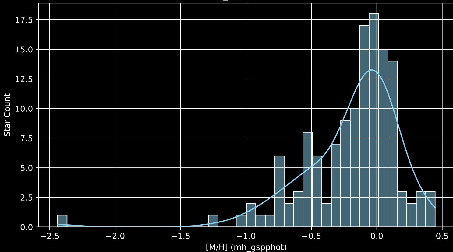
Gaia Cluster: [Teutsch_35 [M/H] (mh_gspphot) (n= 135)
