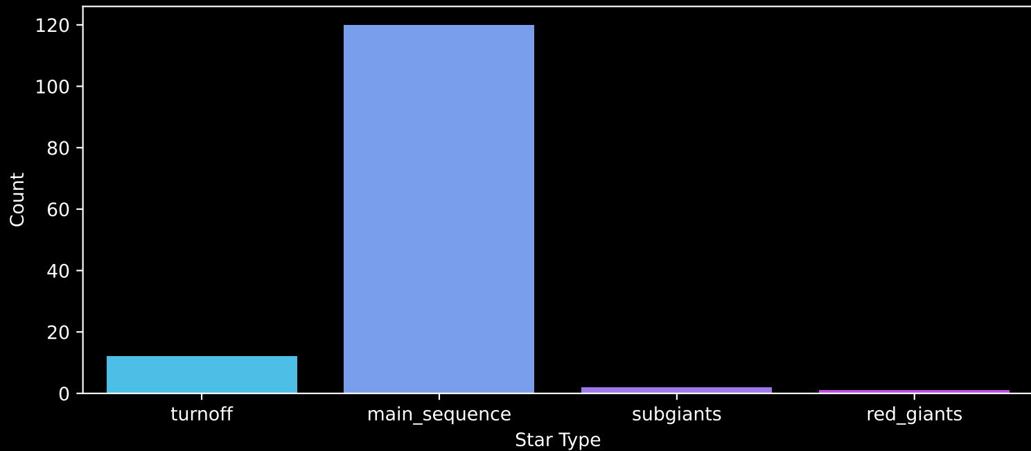
Gaia Cluster: [Teutsch_35] Count plot of Star Type
