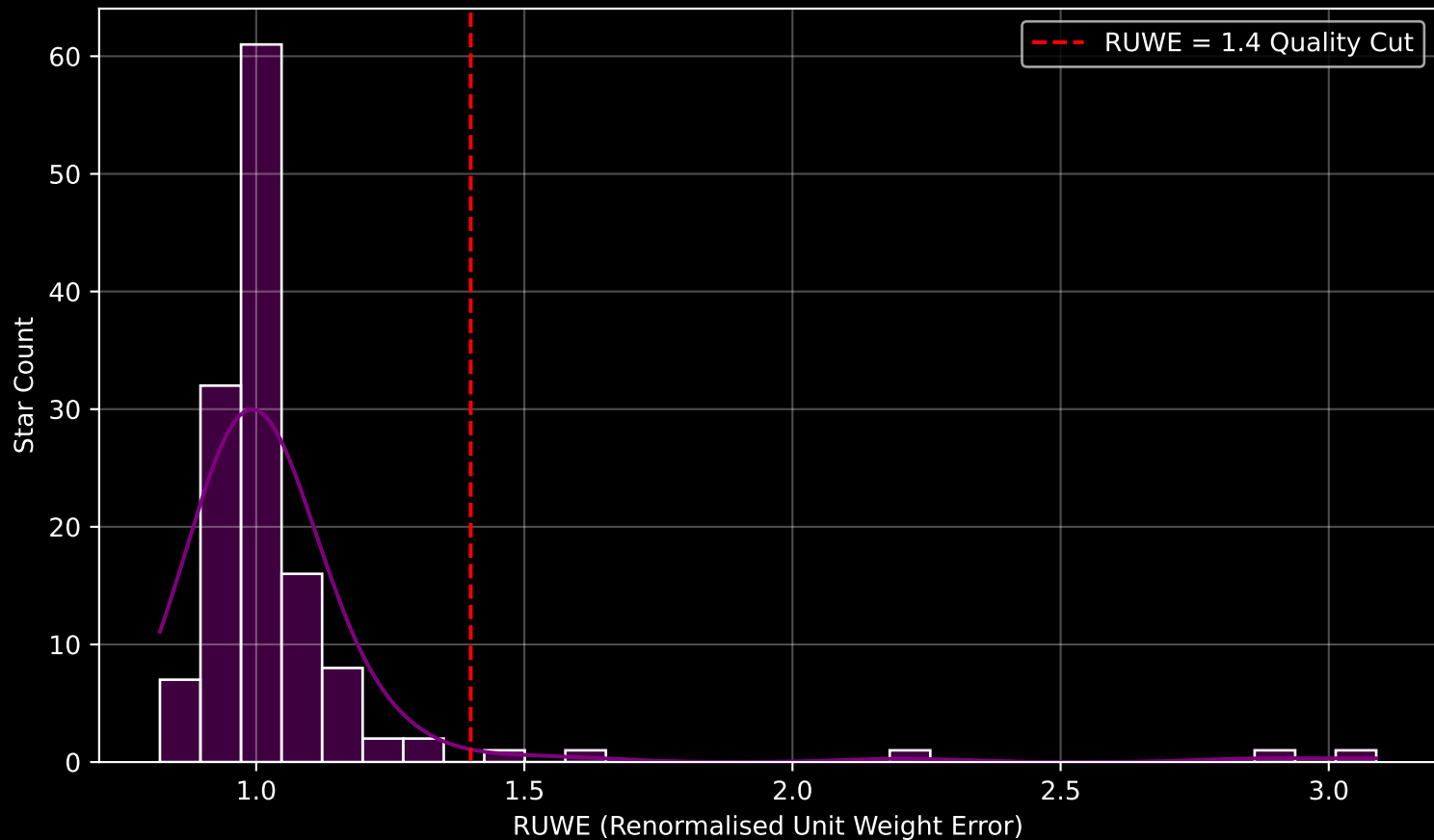
Gaia Cluster: [Teutsch_35] RUWE Distribution (n= 133)
