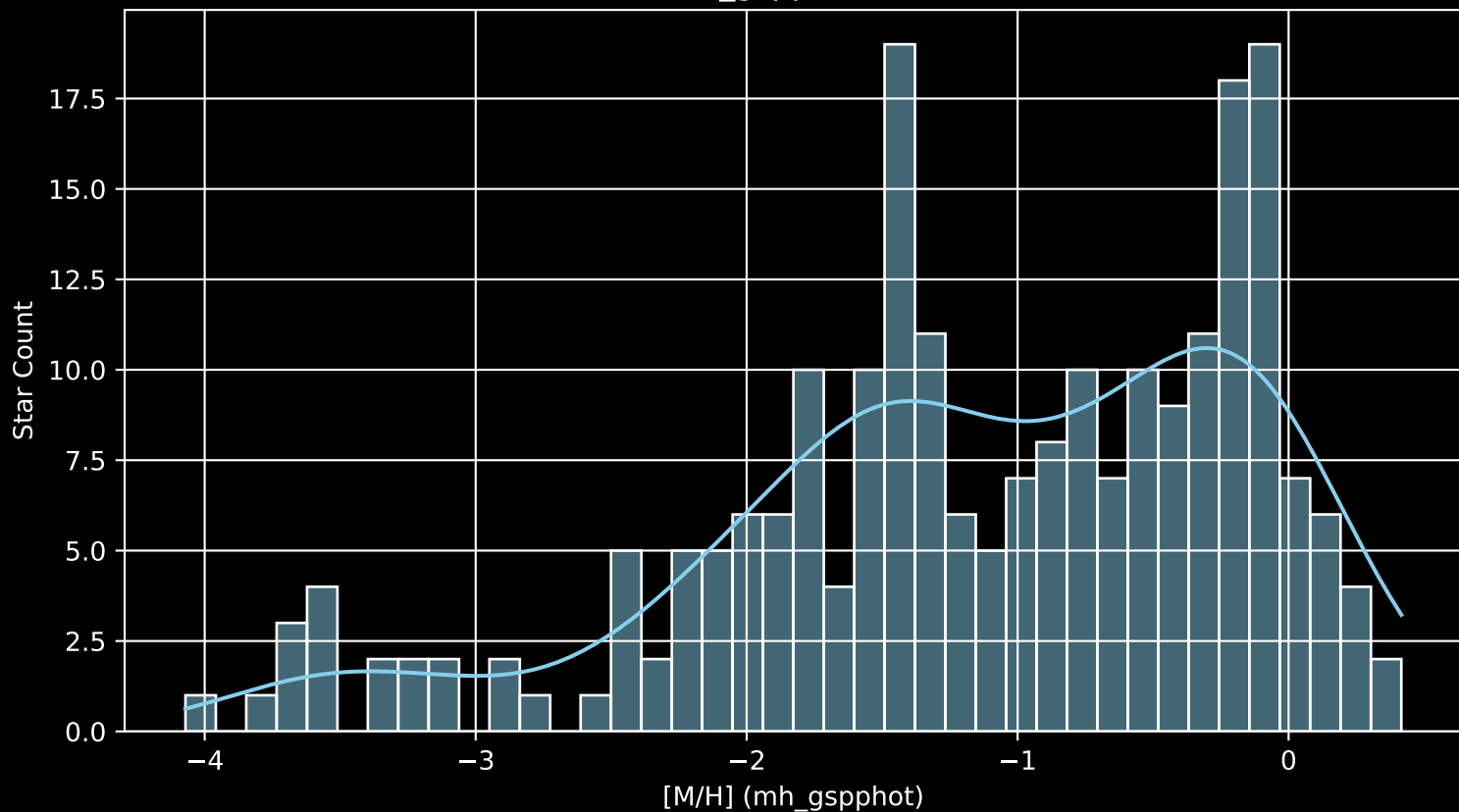
Gaia Cluster: [Teutsch_44 [M/H] (mh_gspphot) (n= 231)
