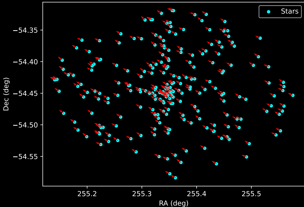
Gaia Cluster: [Teutsch_44] Proper Motion Vectors for Gaia Star Field (n= 233)
