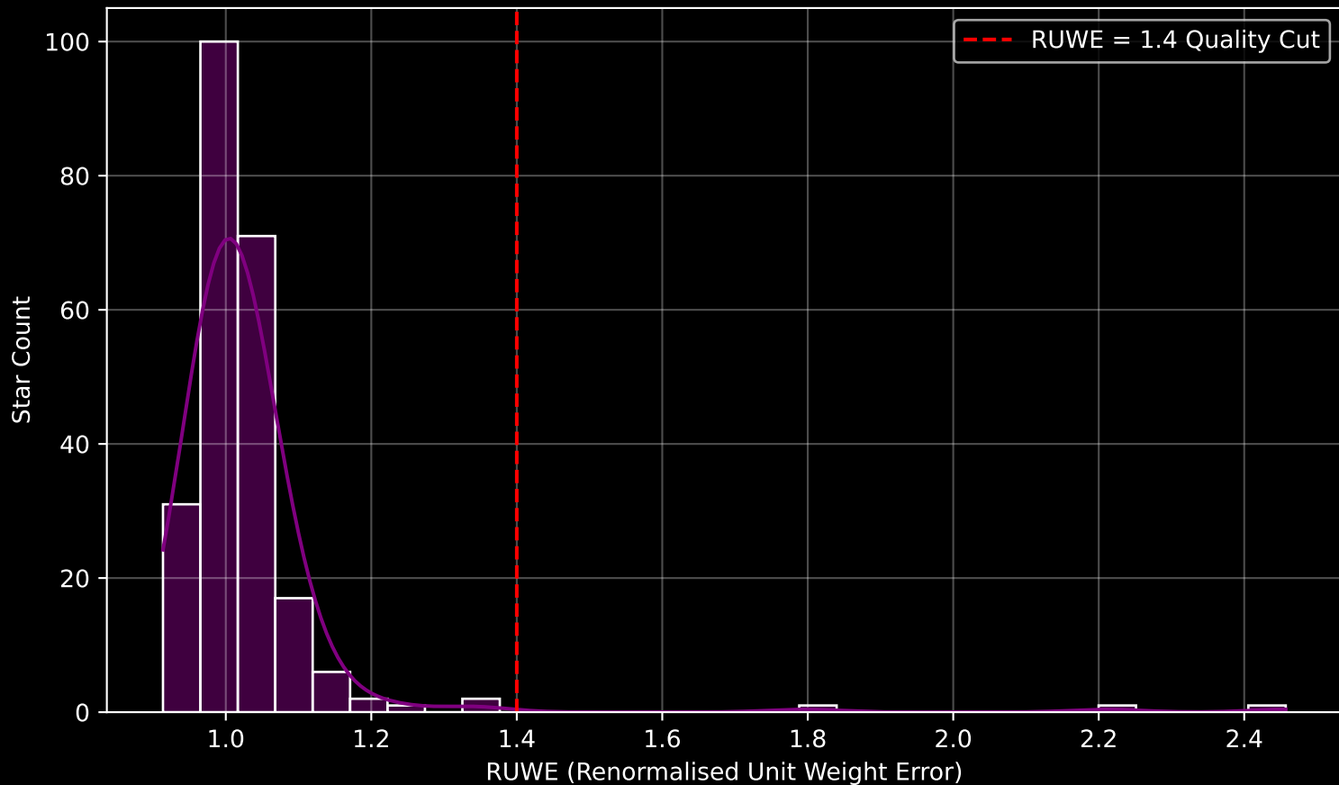
Gaia Cluster: [Teutsch_44] RUWE Distribution (n= 233)
