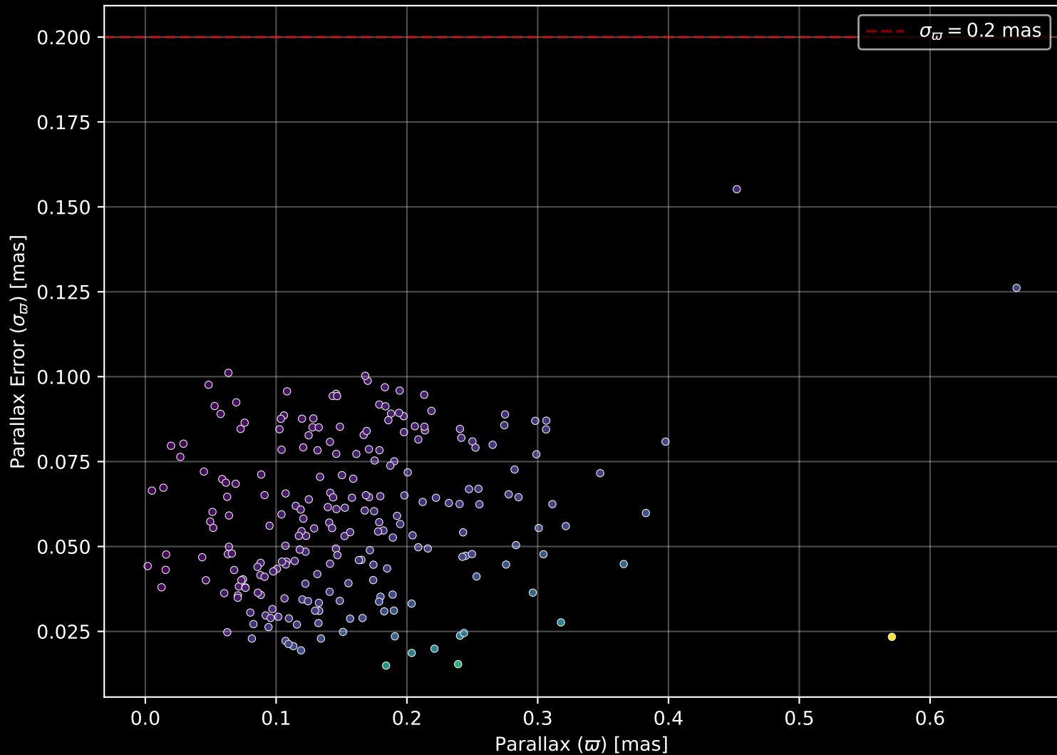
Gaia Cluster: [Teutsch_44] Parallax Quality (n= 233)
