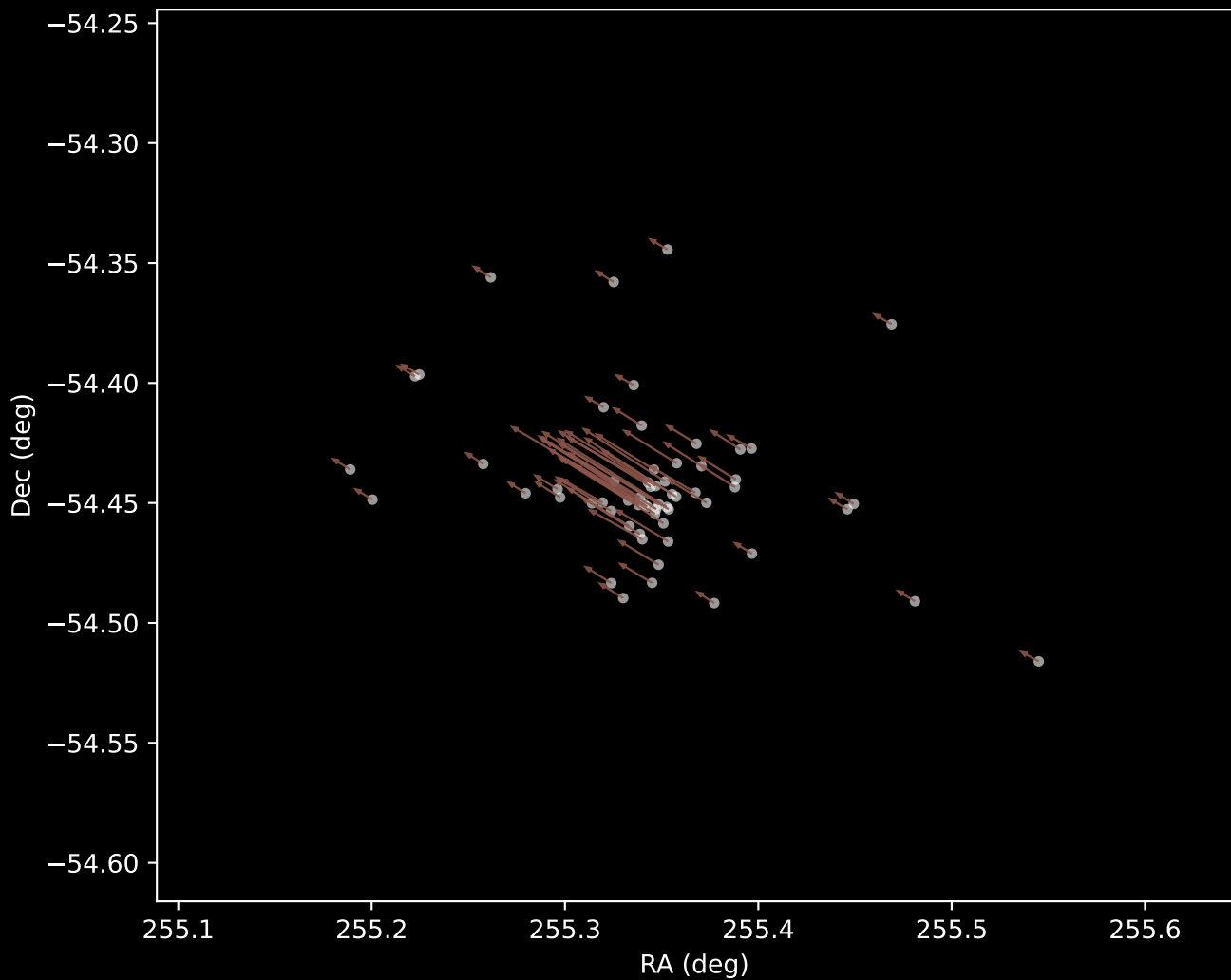
Gaia DR3 Cluster 10 Proper Motion Vectors (n=60)
