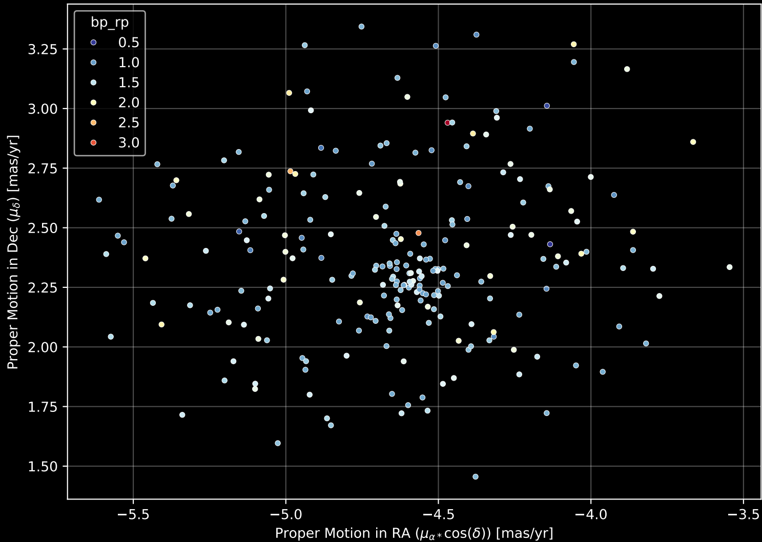
Gaia Cluster: [Teutsch_44] Proper Motion Diagram (n= 233)
