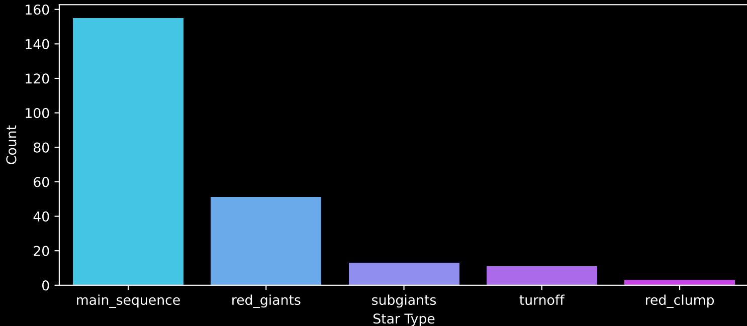
Gaia Cluster: [Teutsch_44] Count plot of Star Type
