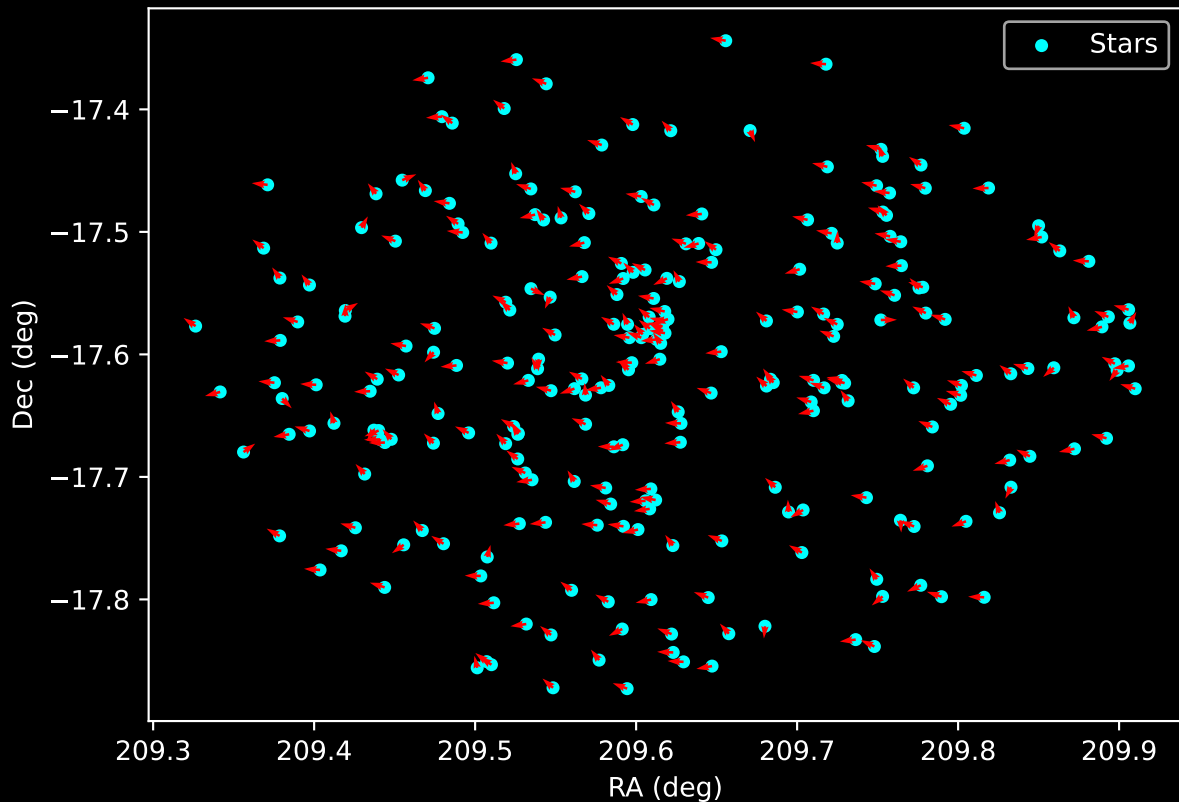
Gaia Cluster: [Teutsch_49] Proper Motion Vectors for Gaia Star Field (n= 255)
