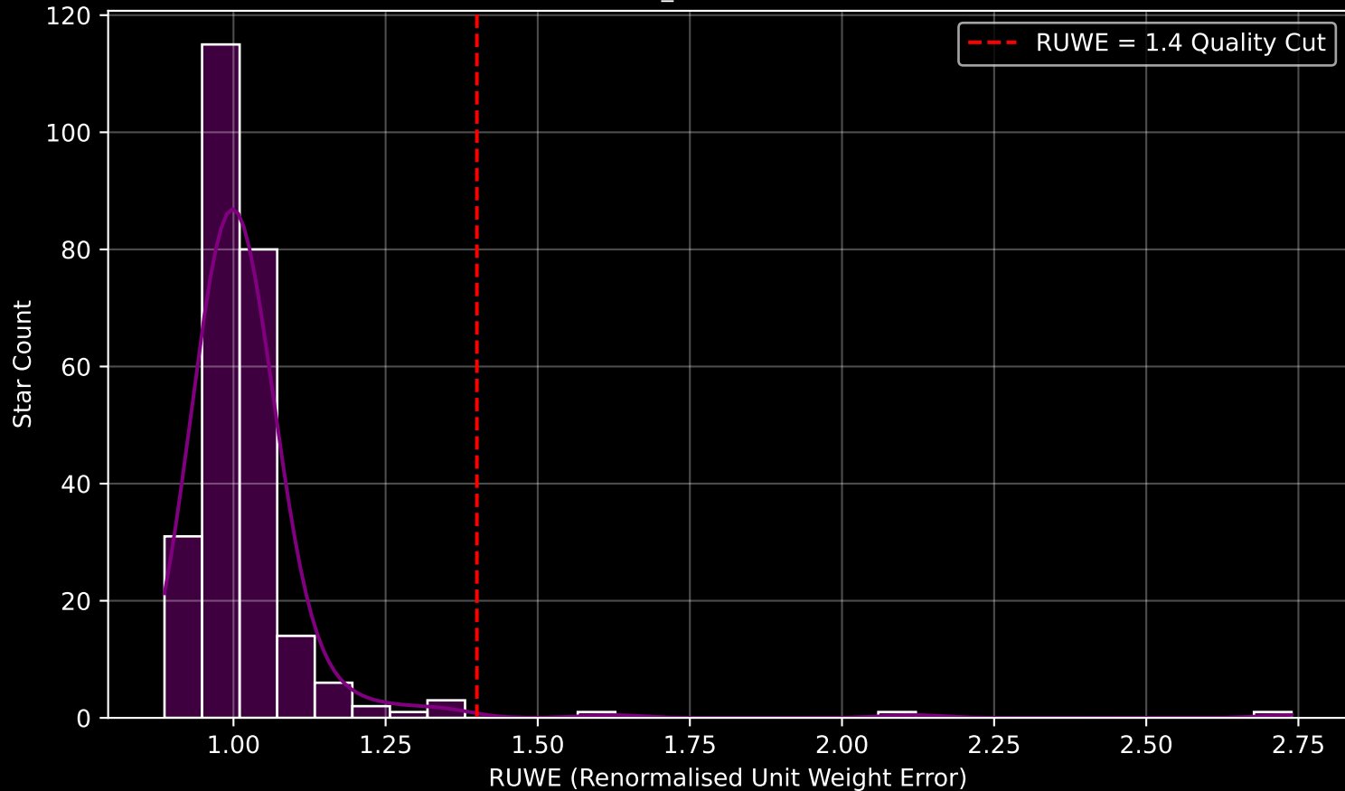
Gaia Cluster: [Teutsch_49] RUWE Distribution (n= 255)
