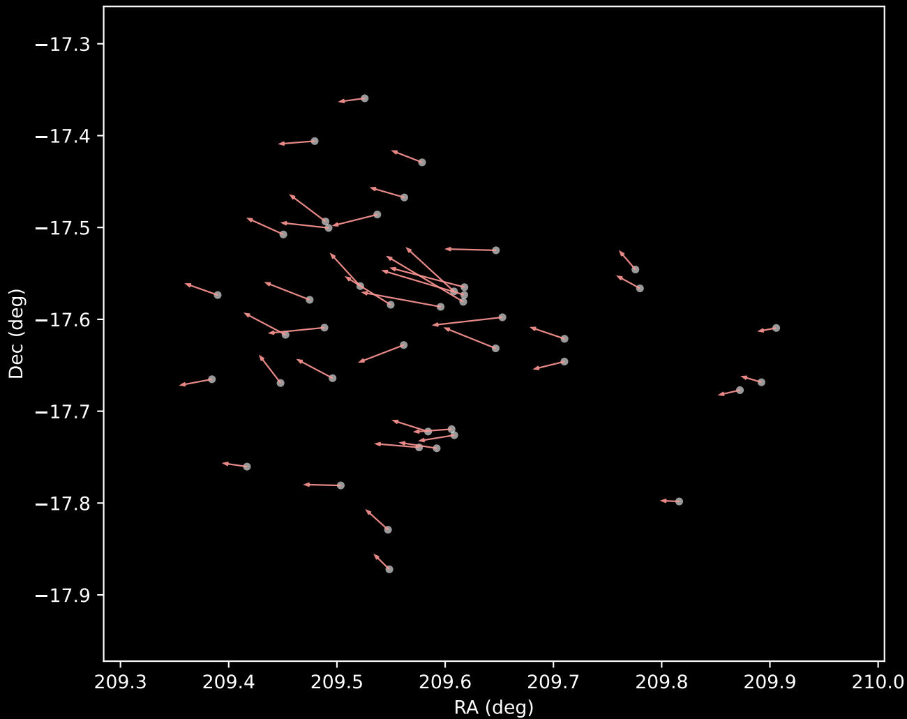
Gaia DR3 Cluster 7 Proper Motion Vectors (n=43)
