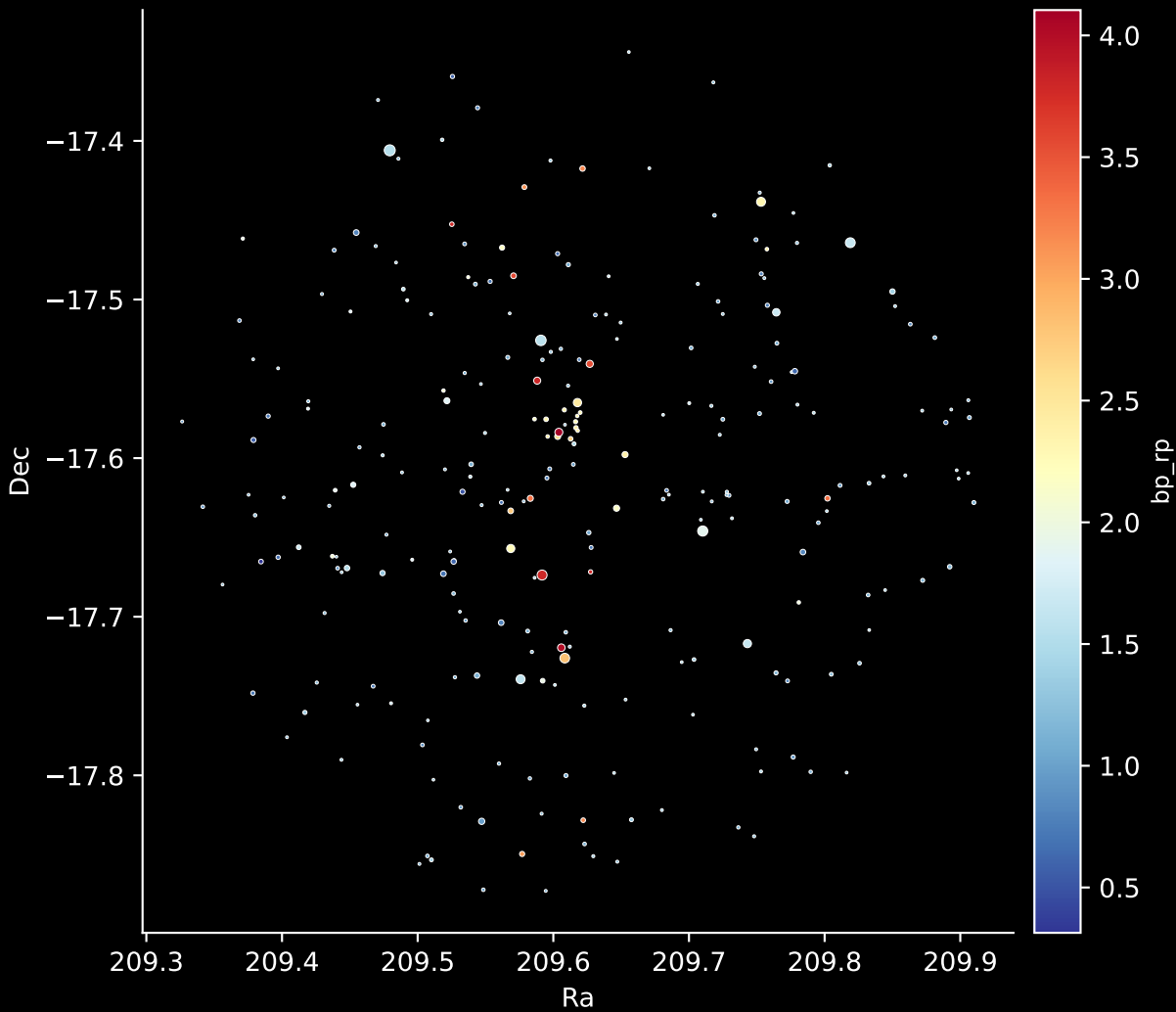
Gaia Cluster: [Teutsch_49] Stars: 255
