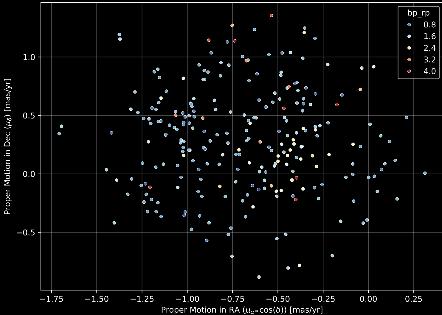
Gaia Cluster: [Deutsch_49] Proper Motion Diagram (n= 255)
