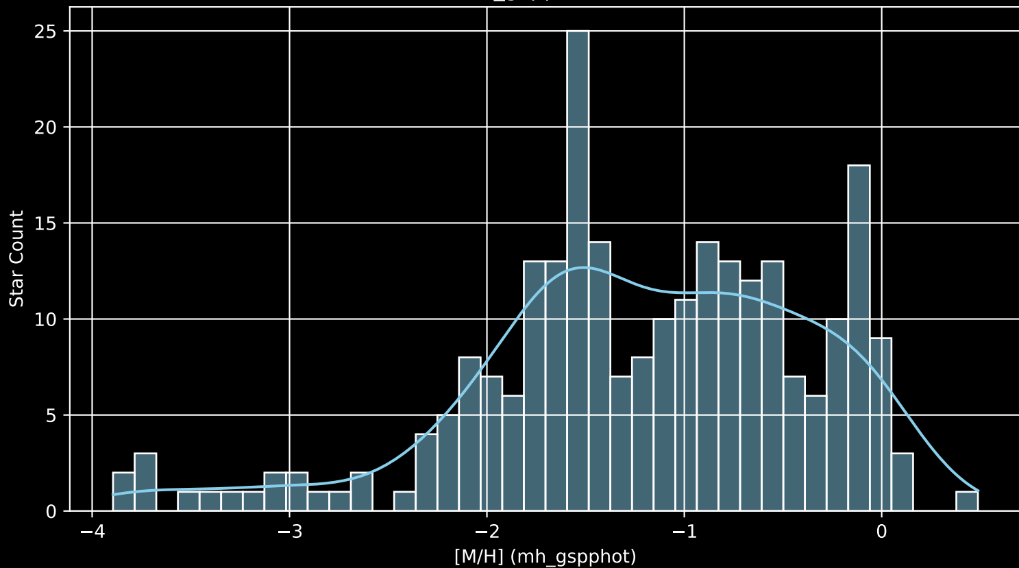
Gaia Cluster: [Teutsch_49 [M/H] (mh_gspphot) (n= 255)
