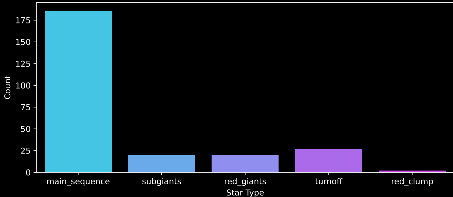
Gaia Cluster: [Teutsch_49] Count plot of Star Type
