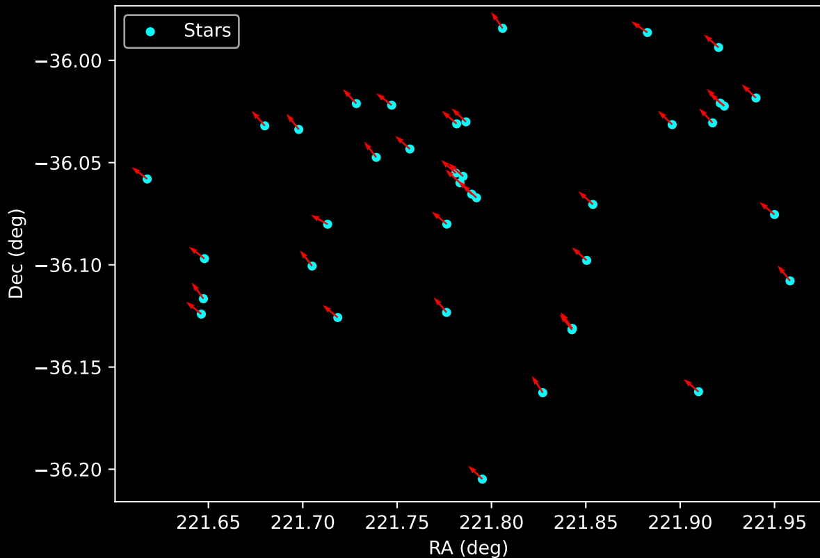
Gaia Cluster: [Teutsch_50] Proper Motion Vectors for Gaia Star Field (n= 39)
