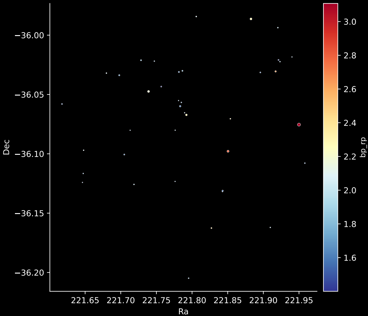
Gaia Cluster: [Teutsch_50] Stars: 39
