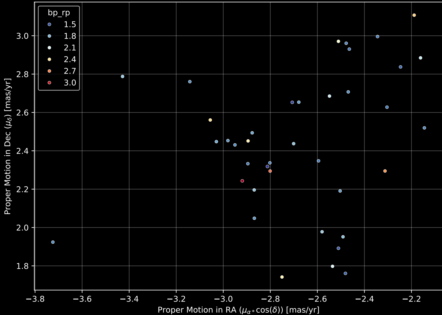
Gaia Cluster: [Teutsch_50] Proper Motion Diagram (n= 39)
