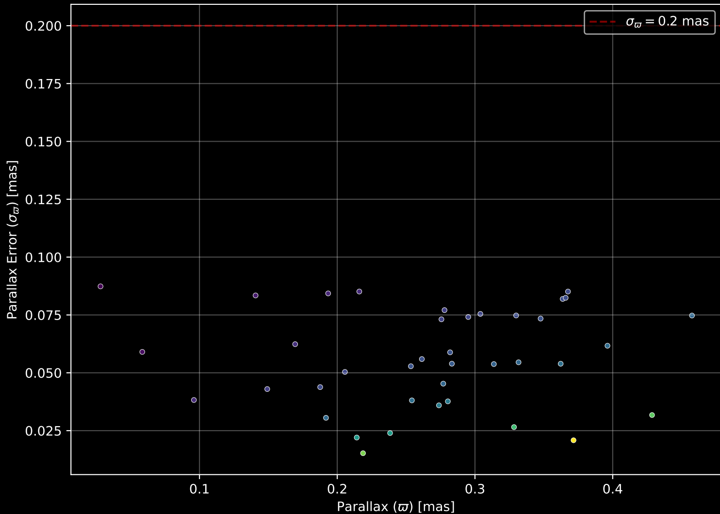
Gaia Cluster: [Teutsch_50] Parallax Quality (n= 39)
