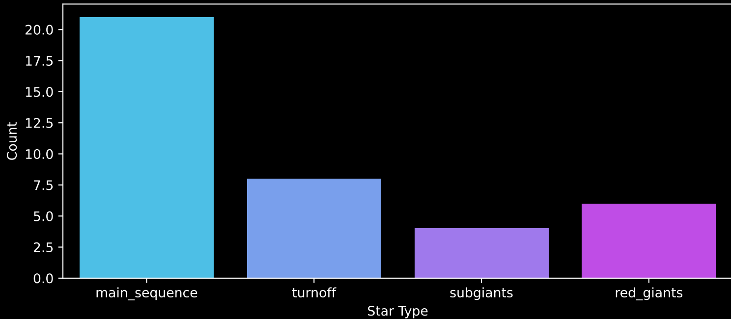
Gaia Cluster: [Teutsch_50] Count plot of Star Type
