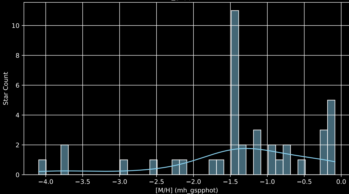
Gaia Cluster: [Teutsch_50 [M/H] (mh_gspphot) (n= 39)
