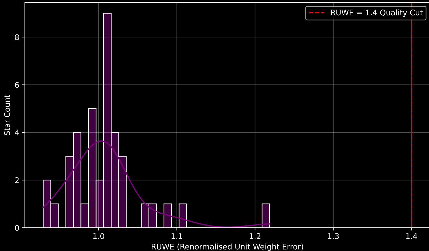
Gaia Cluster: [Teutsch_50] RUWE Distribution (n= 39)
