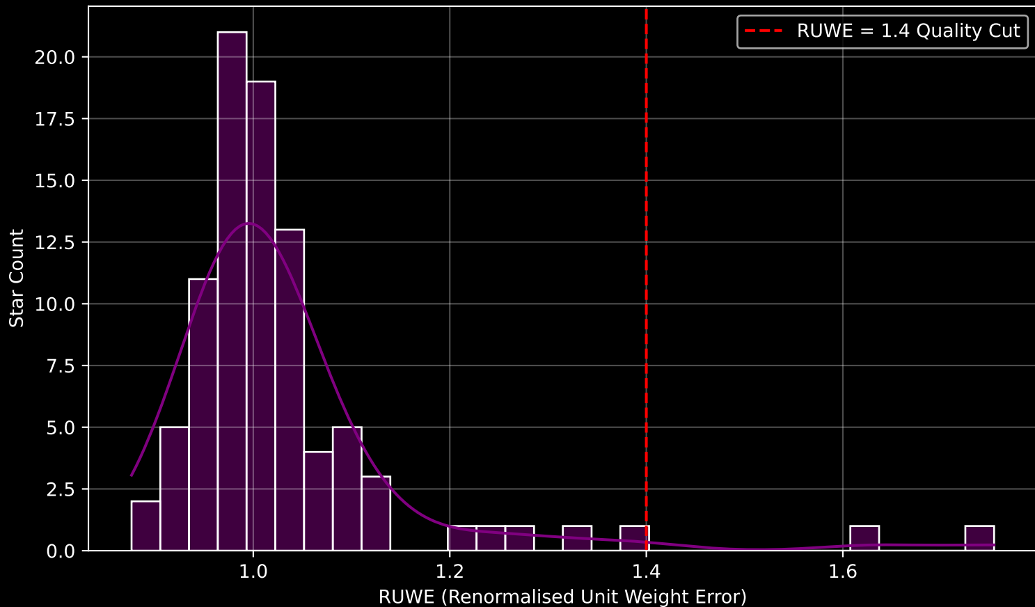
Gaia Cluster: [Teutsch_52] RUWE Distribution (n= 90)
