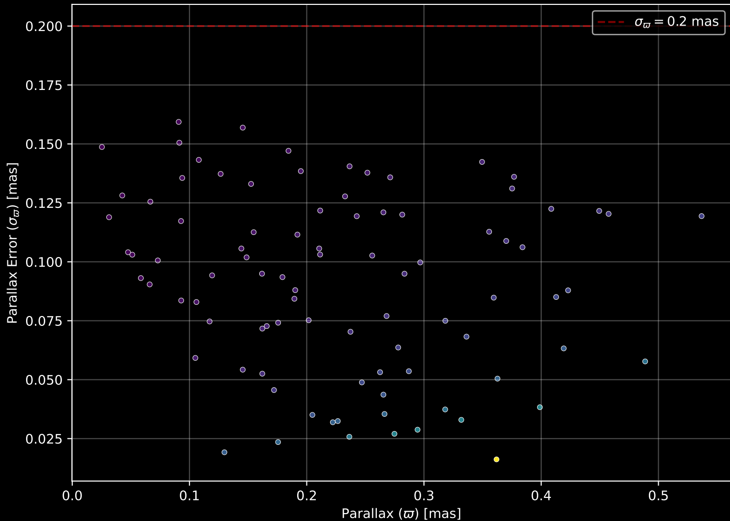
Gaia Cluster: [Deutsch_52] Parallax Quality (n= 90)
