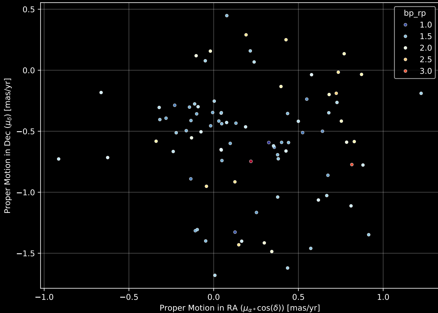
Gaia Cluster: [Teutsch_52] Proper Motion Diagram (n= 90)
