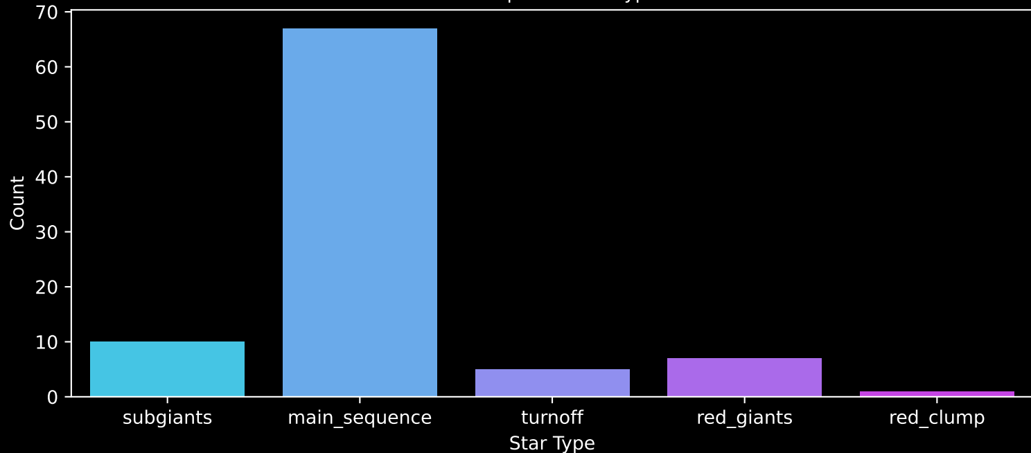
Gaia Cluster: [Teutsch_52] Count plot of Star Type
