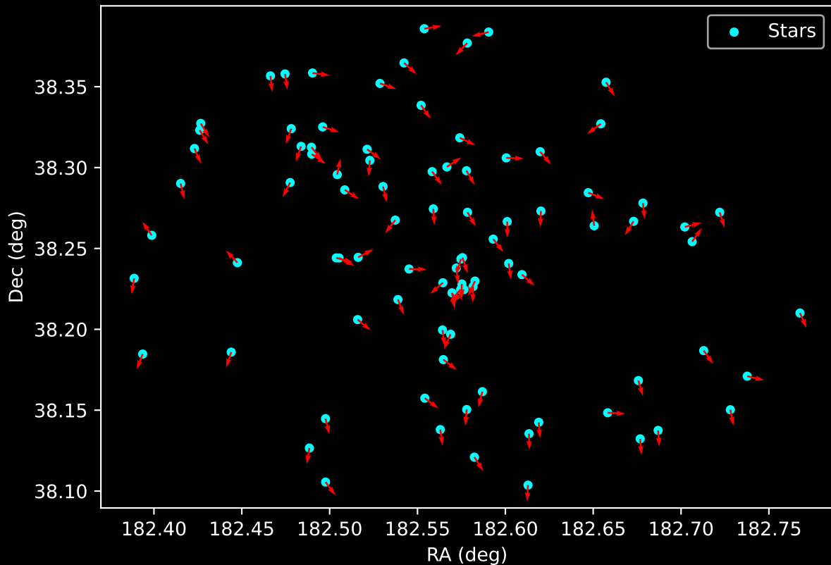
Gaia Cluster: [Teutsch_52] Proper Motion Vectors for Gaia Star Field (n= 90)
