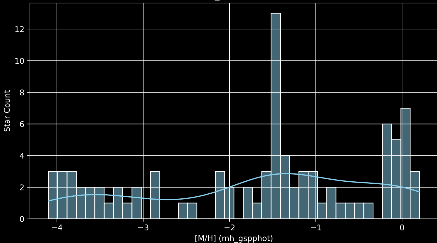
Gaia Cluster: [Teutsch_52 [M/H] (mh_gspphot) (n= 90)
