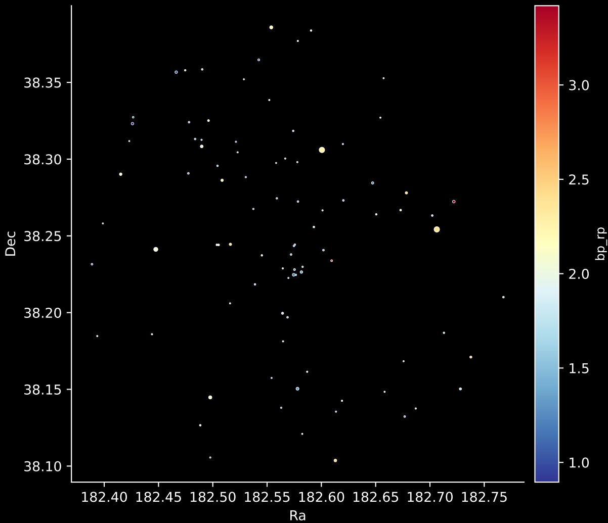
Gaia Cluster: [Teutsch_52] Stars: 90
