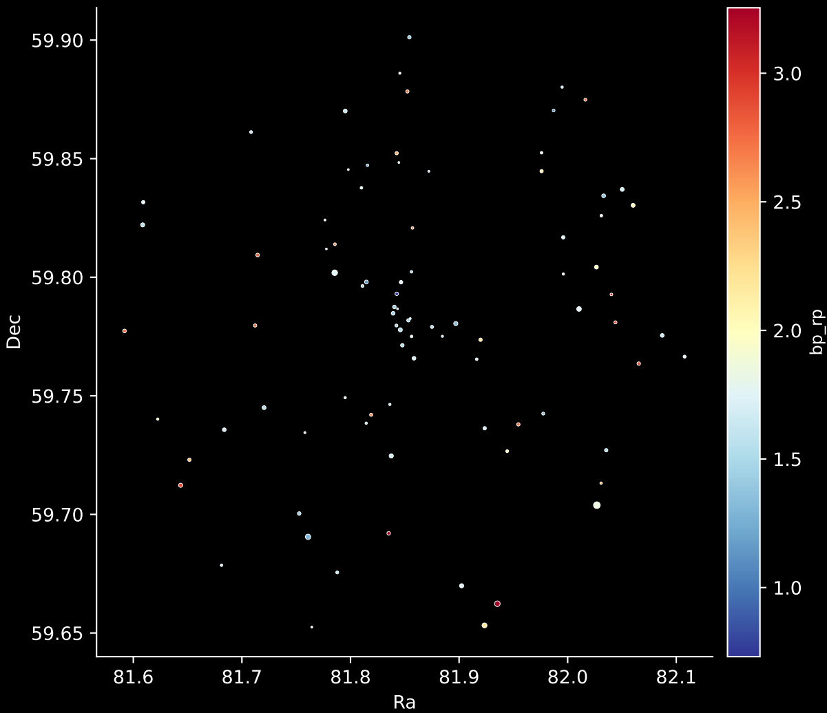
Gaia Cluster: [Teutsch_54] Stars: 86
