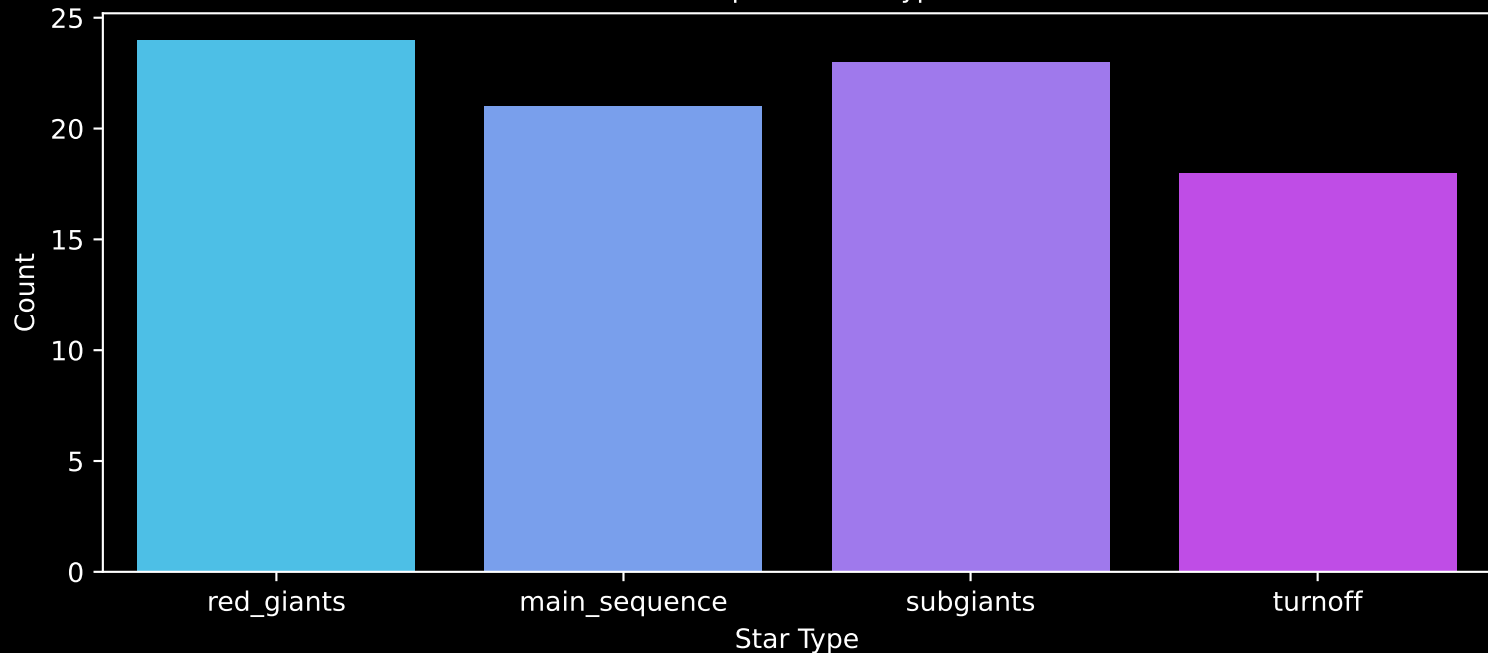
Gaia Cluster: [Teutsch_54] Count plot of Star Type
