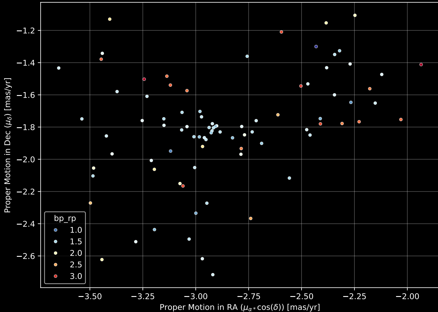
Gaia Cluster: [Teutsch_54] Proper Motion Diagram (n= 86)
