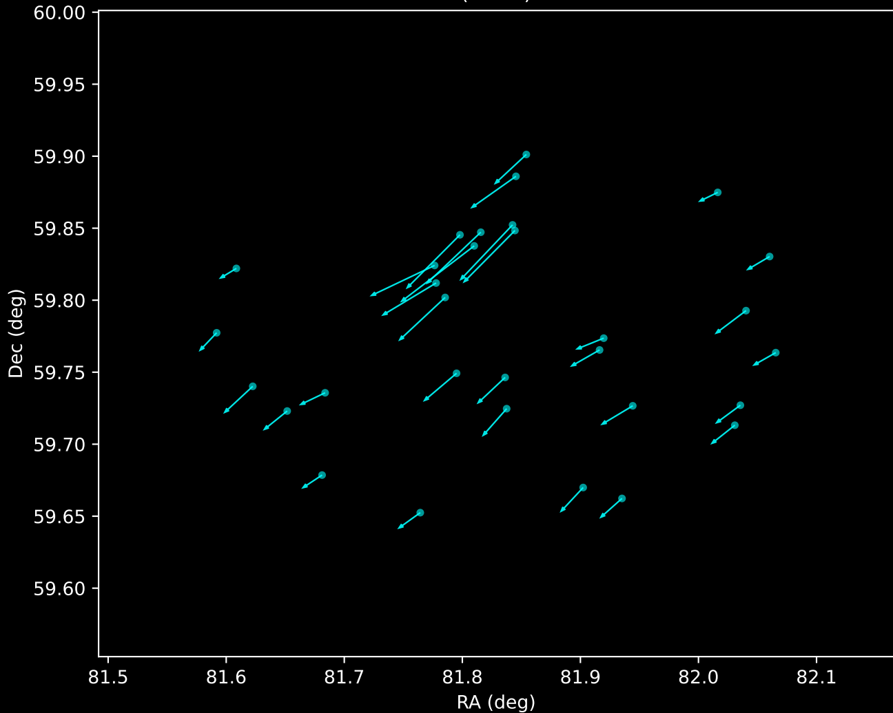
Gaia DR3 Noise Stream Proper Motion Vectors (n=31)
