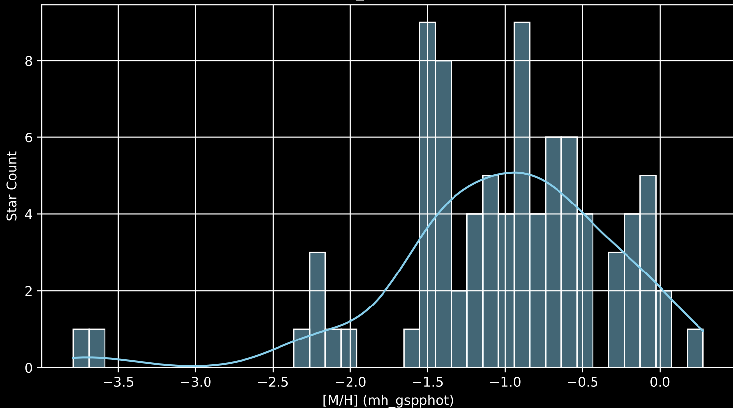
Gaia Cluster: [Teutsch_54 [M/H] (mh_gspphot) (n= 85)
