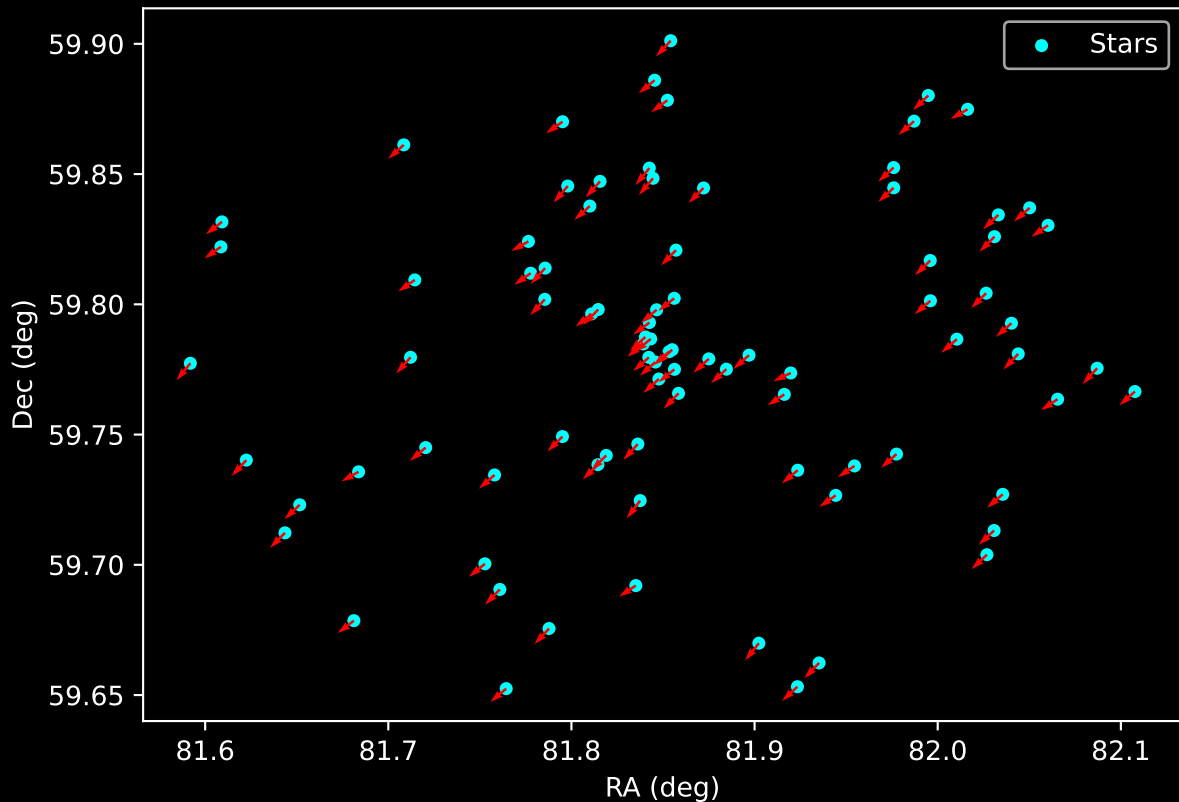
Gaia Cluster: [Teutsch_54] Proper Motion Vectors for Gaia Star Field (n= 86)
