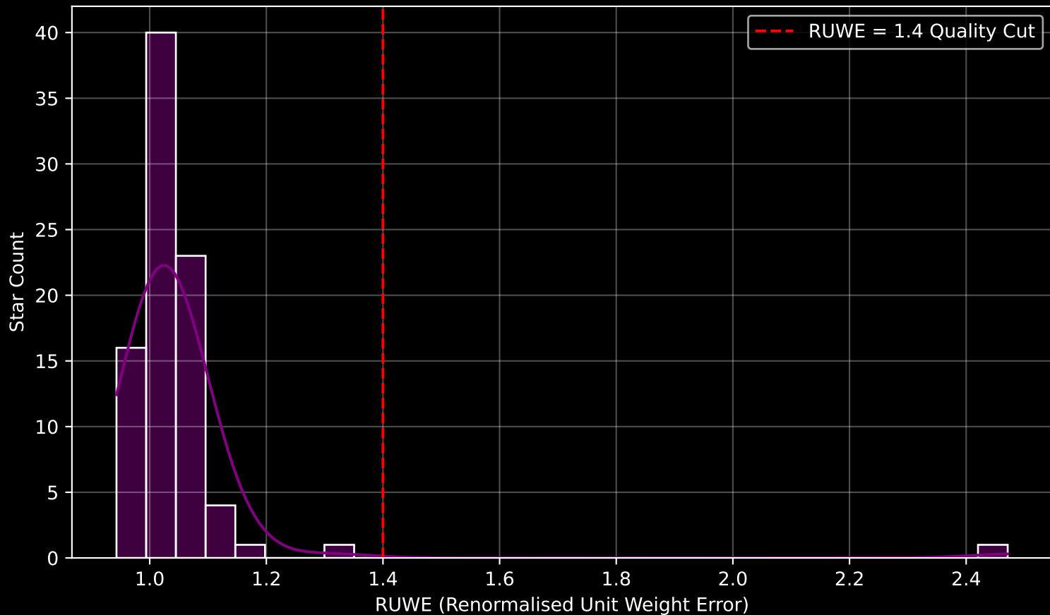
Gaia Cluster: [Teutsch_54] RUWE Distribution (n= 86)
