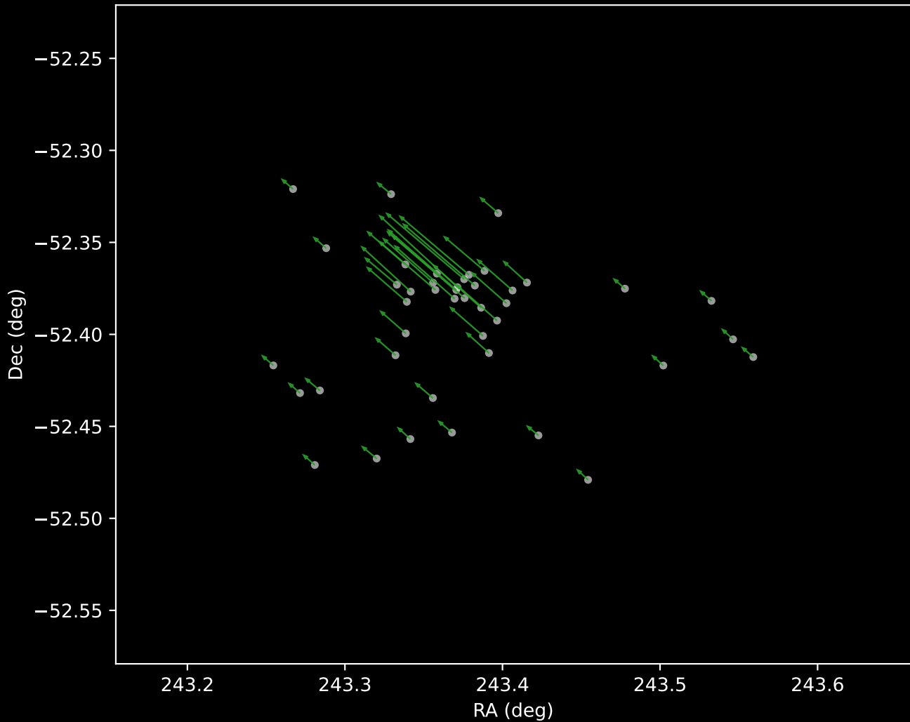
Gaia DR3 Cluster 4 Proper Motion Vectors (n=43)
