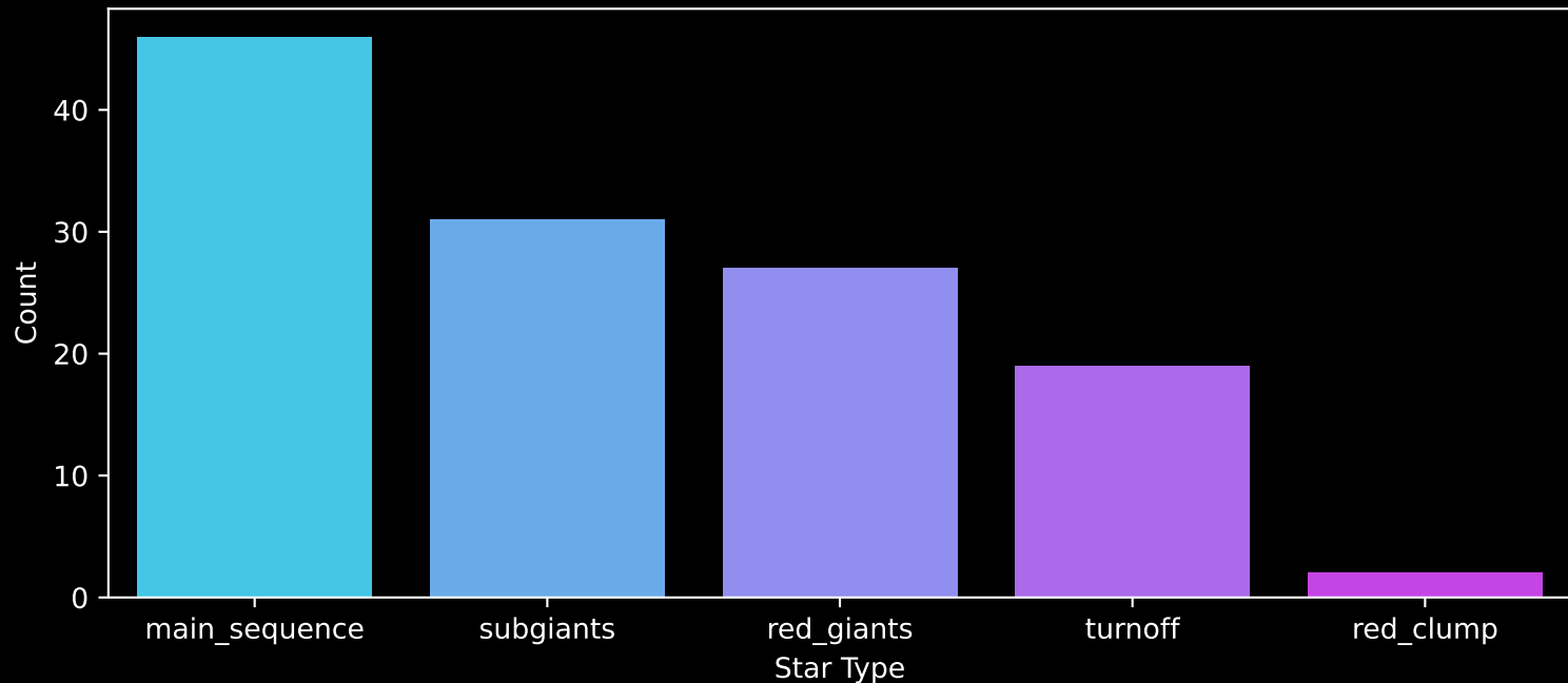
Gaia Cluster: [Teutsch_66] Count plot of Star Type
