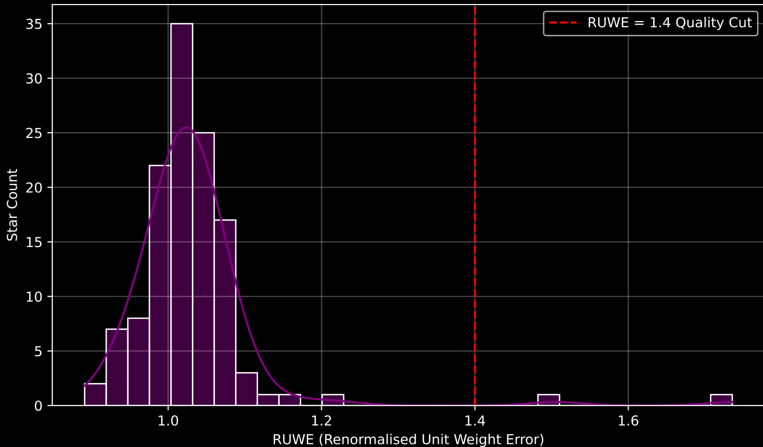
Gaia Cluster: [Teutsch_66] RUWE Distribution (n= 124)
