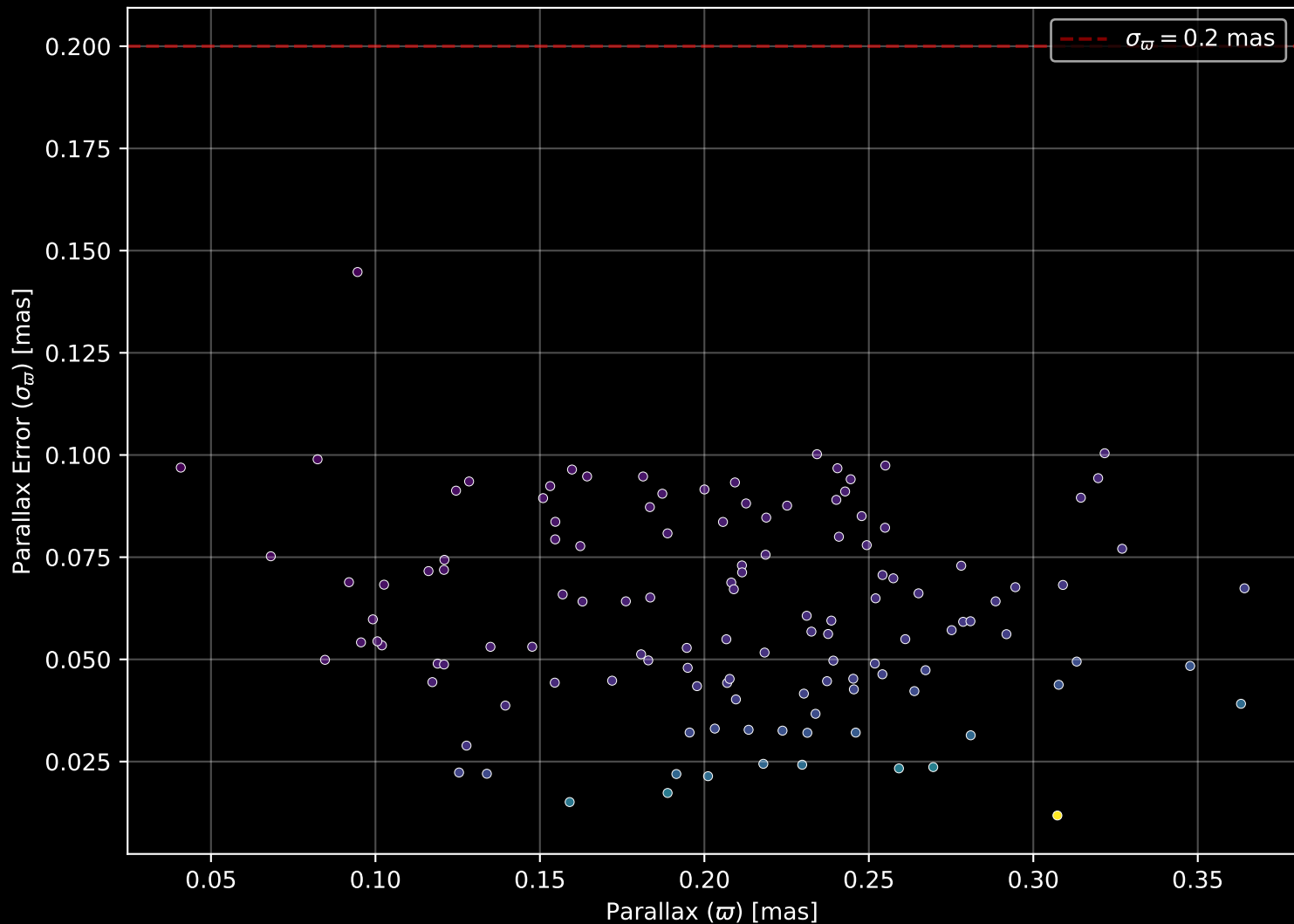
Gaia Cluster: [Teutsch_66] Parallax Quality (n= 125)
