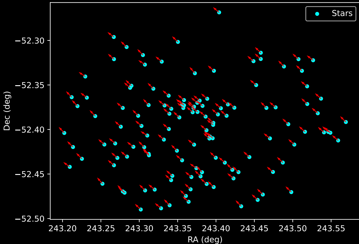
Gaia Cluster: [Teutsch_66] Proper Motion Vectors for Gaia Star Field (n= 125)
