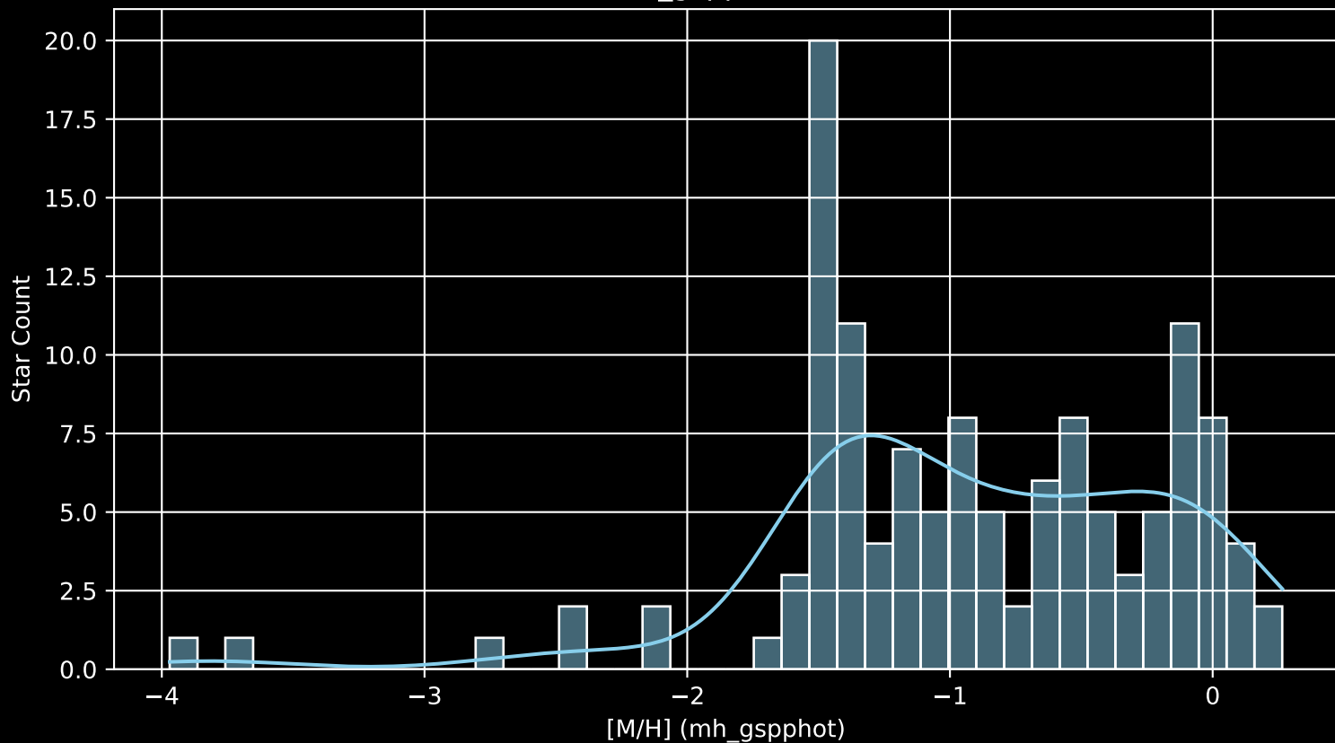
Gaia Cluster: [Deutsch_66 [M/H] (mh_gspphot) (n= 125)
