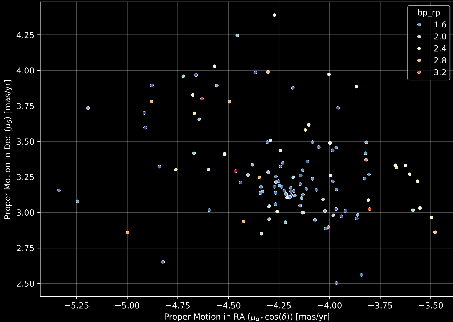
Gaia Cluster: [Teutsch_66] Proper Motion Diagram (n= 125)
