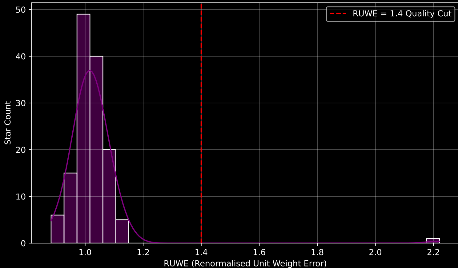
Gaia Cluster: [Teutsch_84] RUWE Distribution (n= 136)
