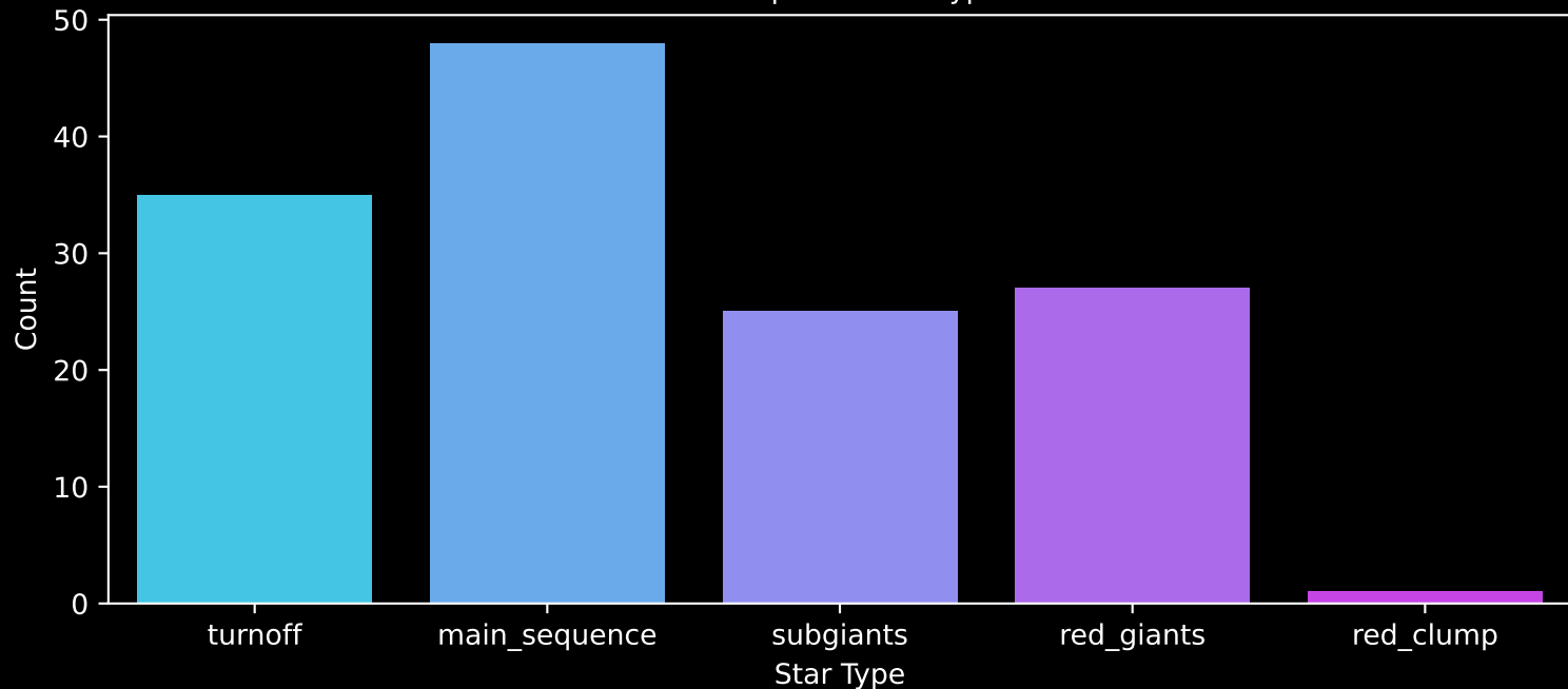
Gaia Cluster: [Teutsch_84] Count plot of Star Type
