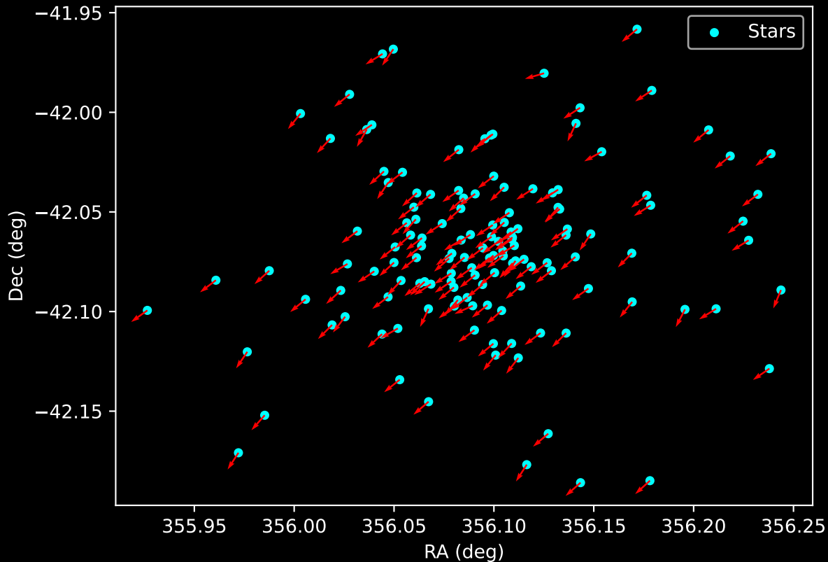
Gaia Cluster: [Teutsch_84] Proper Motion Vectors for Gaia Star Field (n= 136)
