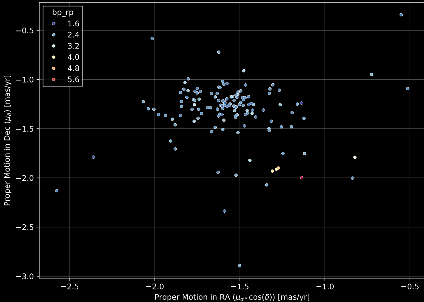
Gaia Cluster: [Teutsch_84] Proper Motion Diagram (n= 136)
