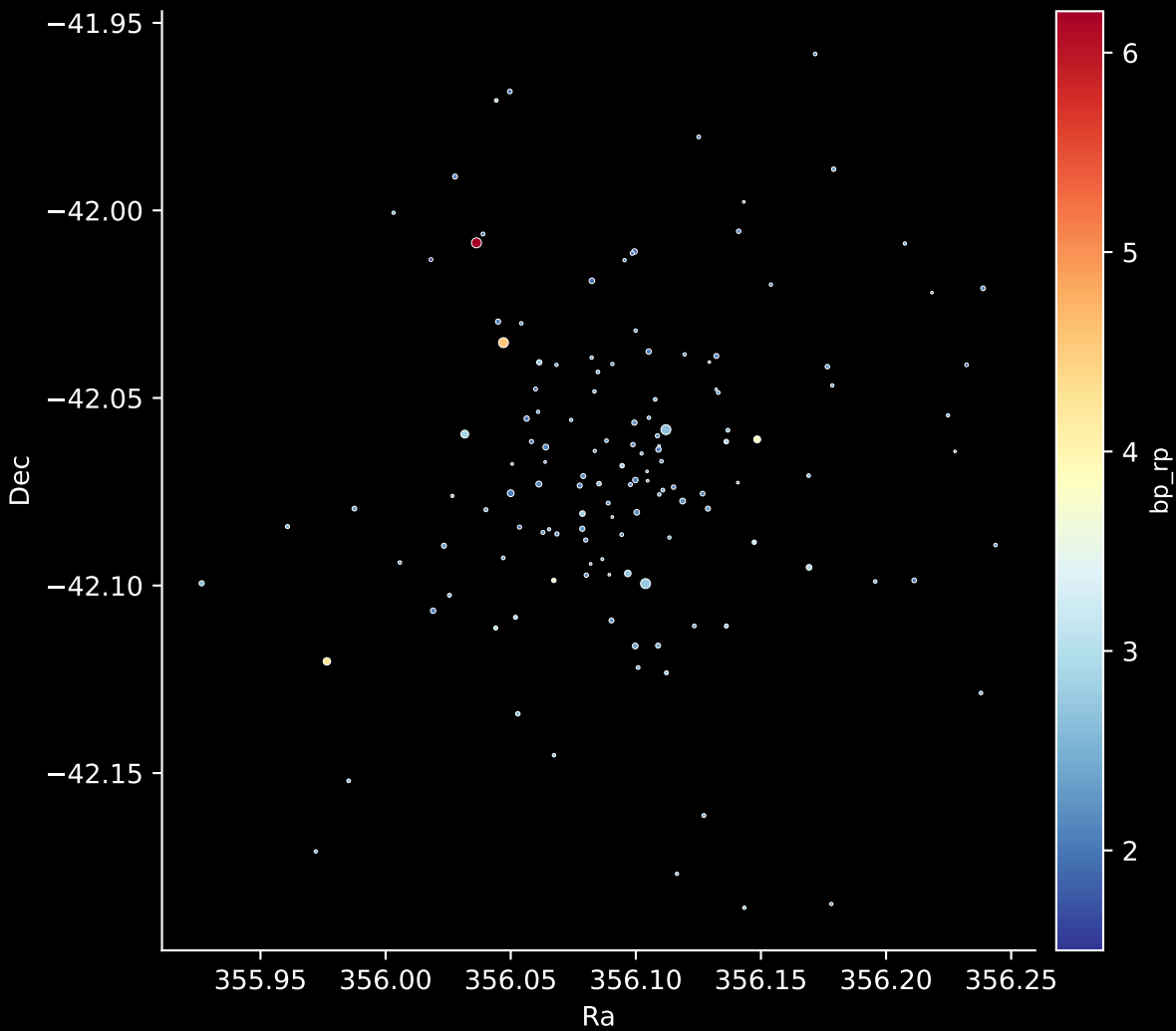
Gaia Cluster: [Teutsch_84] Stars: 136
