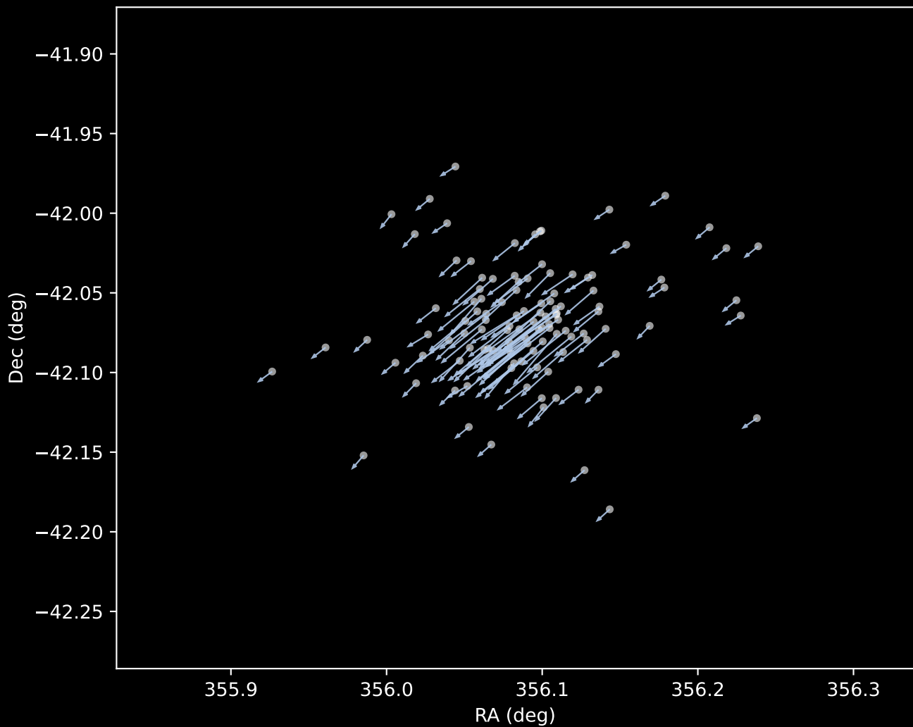
Gaia DR3 Cluster 1 Proper Motion Vectors (n=114)
