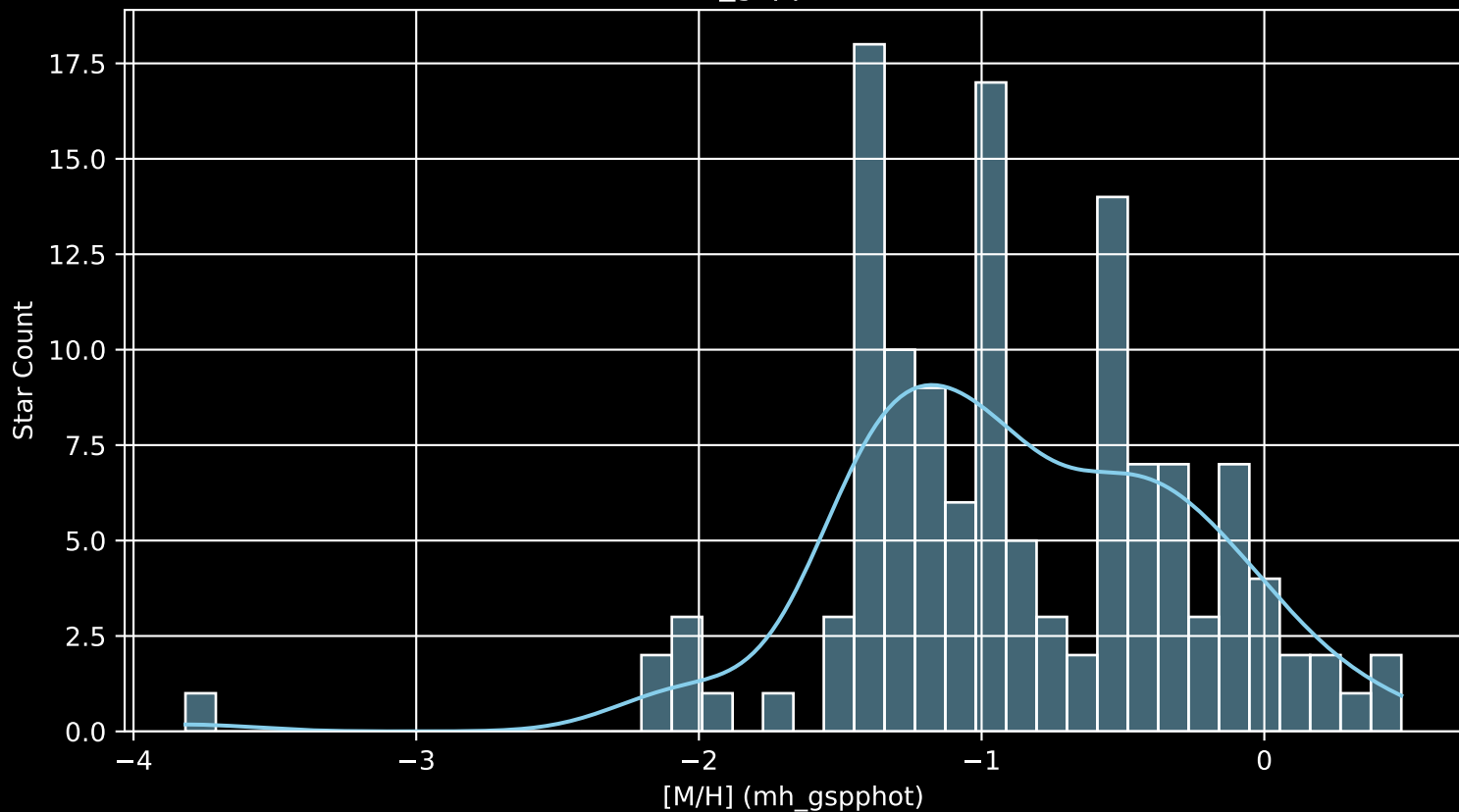
Gaia Cluster: [Teutsch_84 [M/H] (mh_gspphot) (n= 130)
