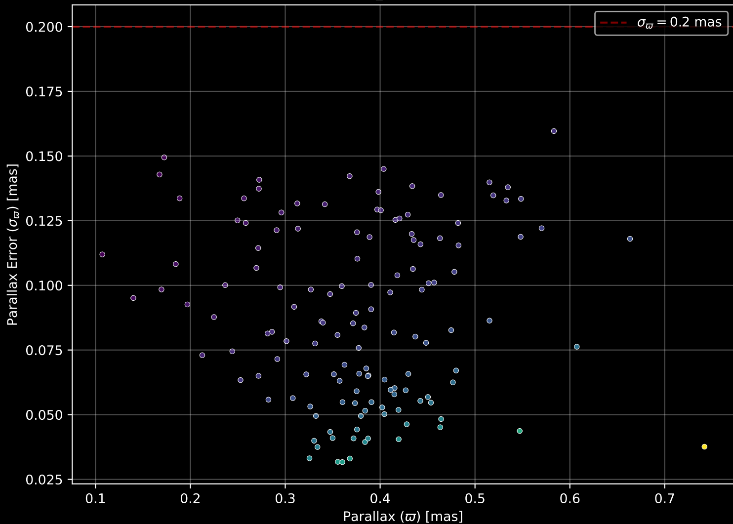
Gaia Cluster: [Teutsch_84] Parallax Quality (n= 136)
