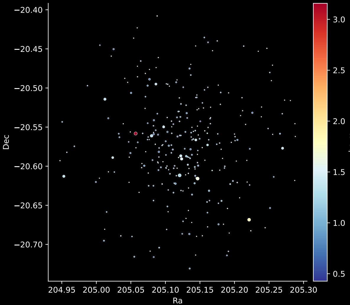
Gaia Cluster: [Tombaugh_1] Stars: 286
