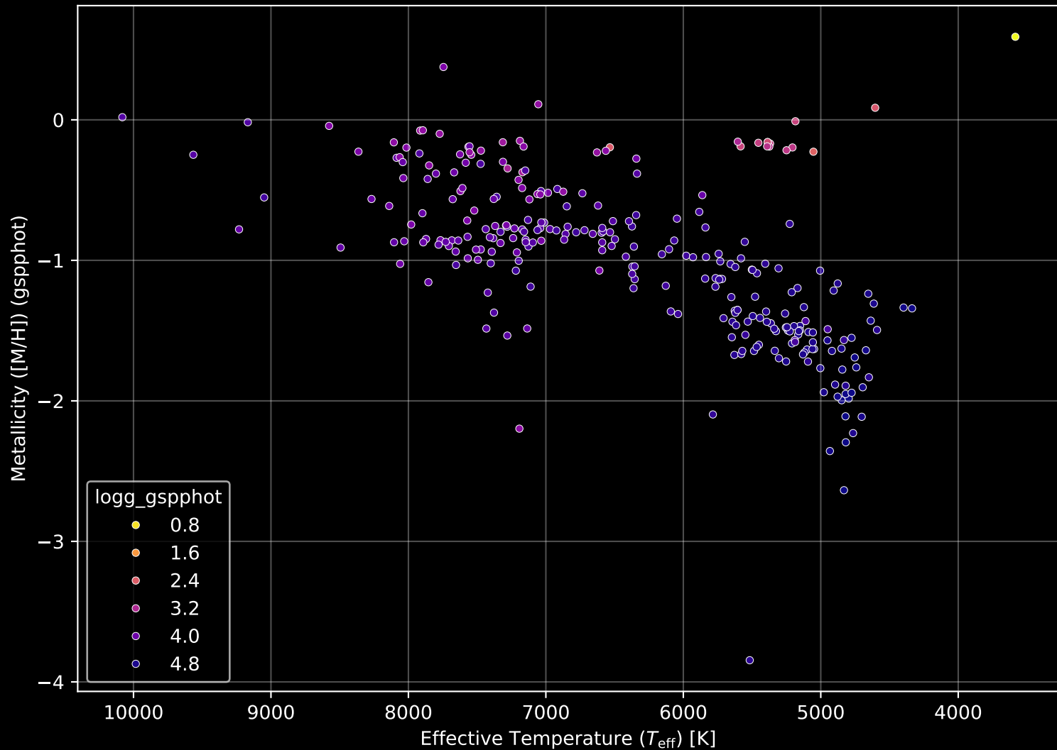
Gaia Cluster: [Tombaugh_1] Stellar Population Parameters (n= 286)
