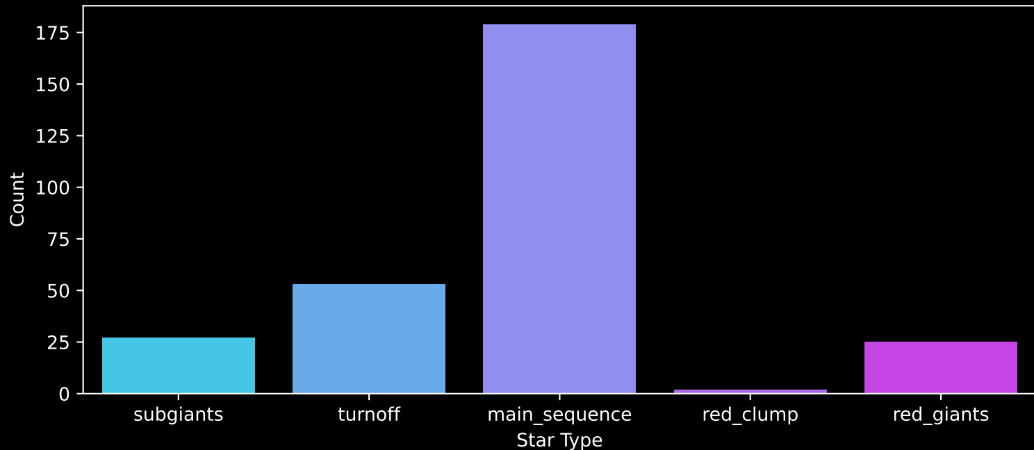
Gaia Cluster: [Tombaugh_1] Count plot of Star Type
