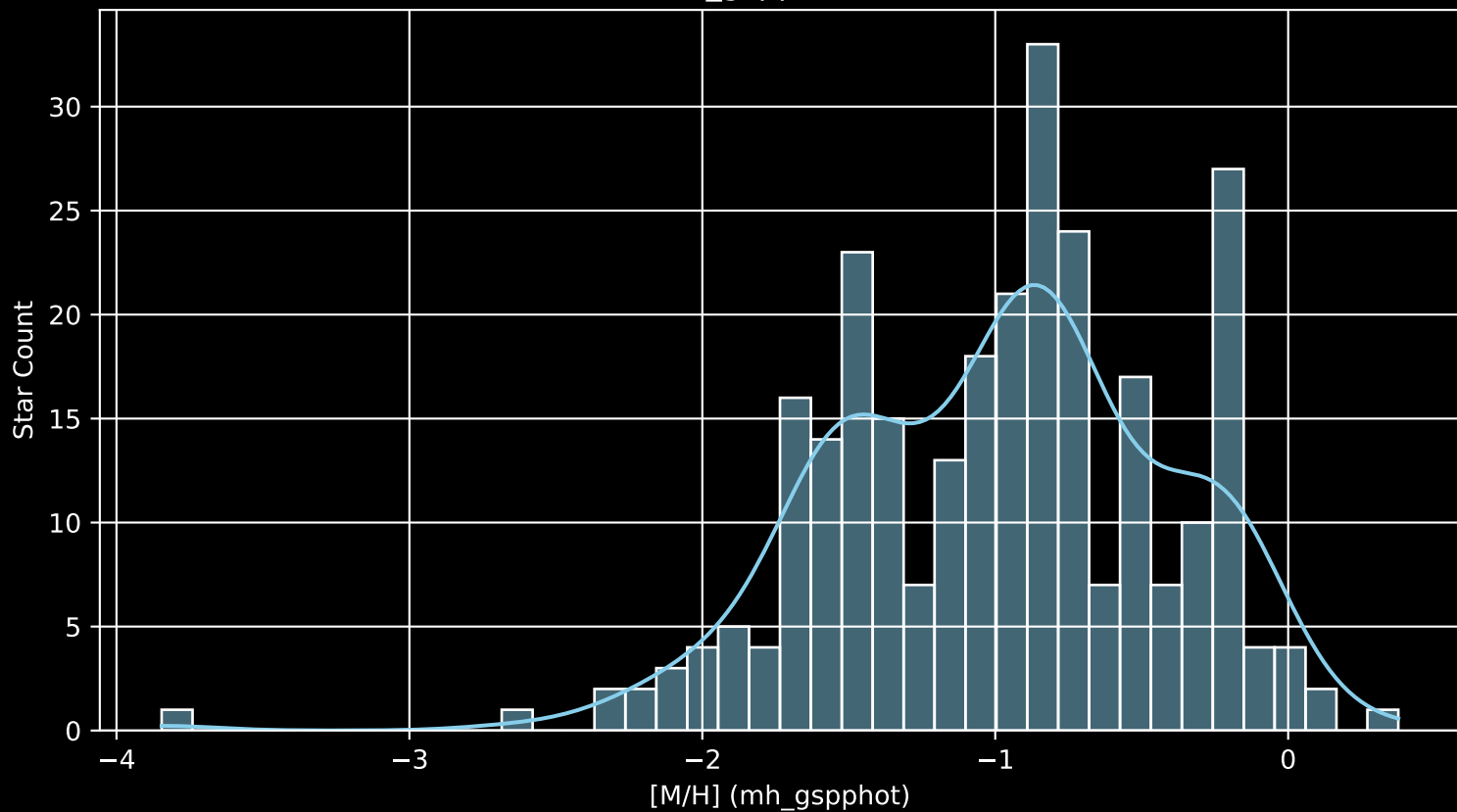
Gaia Cluster: [Tombaugh_1 [M/H] (mh_gspphot) (n= 285)
