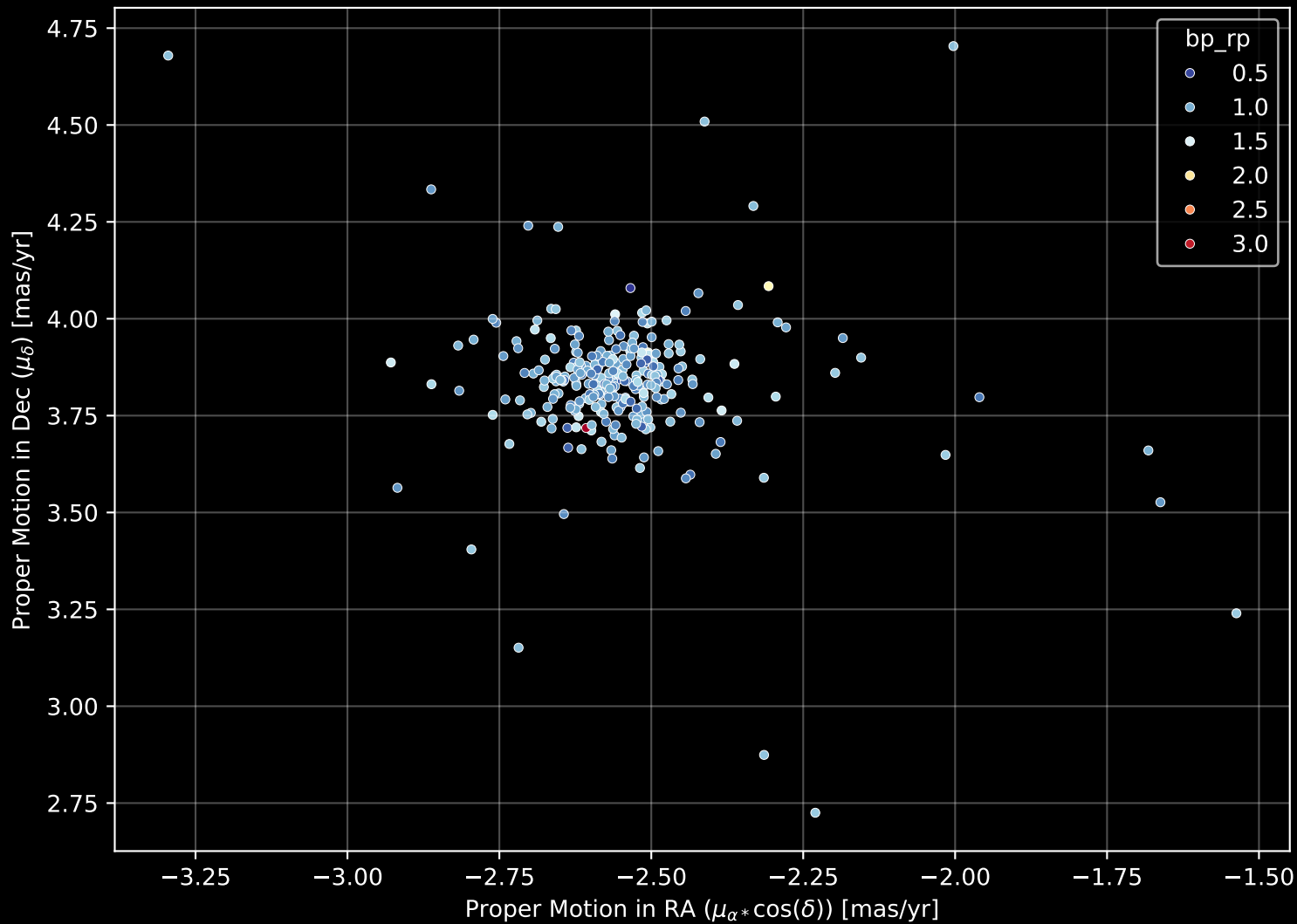
Gaia Cluster: [Tombaugh_1] Proper Motion Diagram (n= 286)
