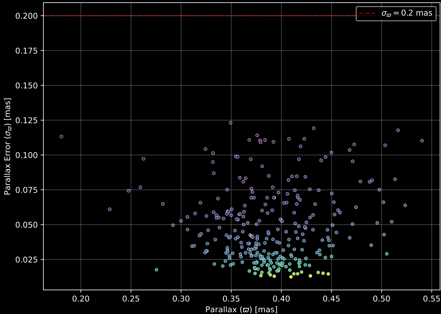
Gaia Cluster: [Tombaugh_1] Parallax Quality (n= 286)
