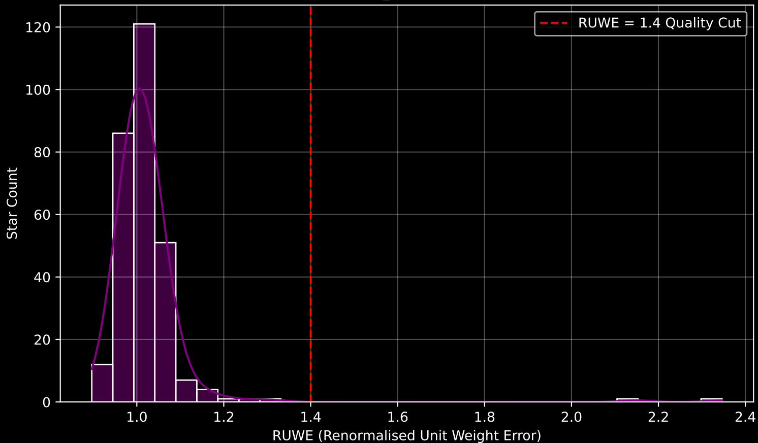
Gaia Cluster: [Tombaugh_1] RUWE Distribution (n= 286)
