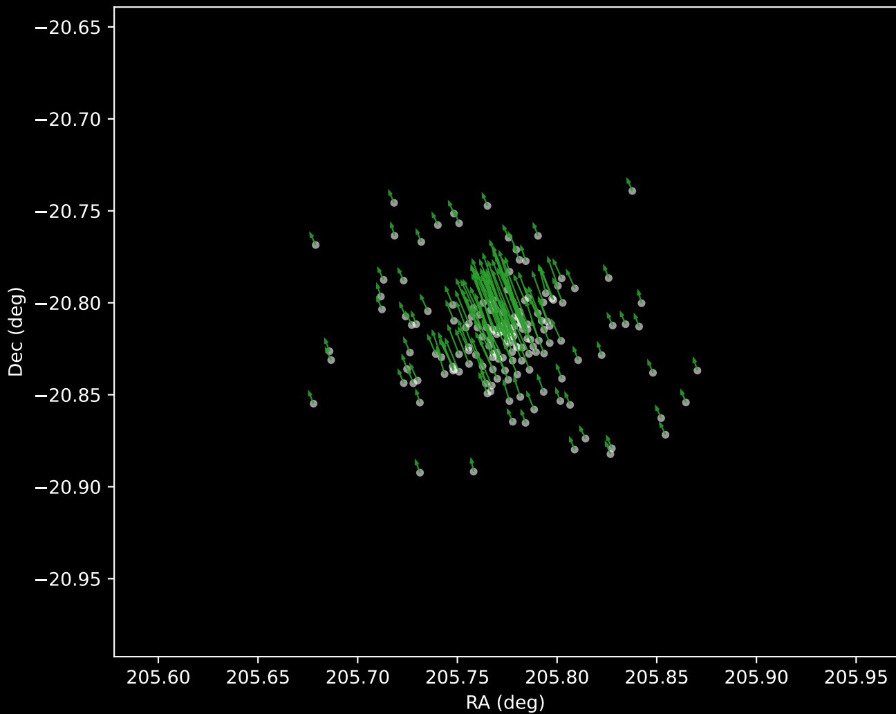
Gaia DR3 Cluster 4 Proper Motion Vectors (n=162)
