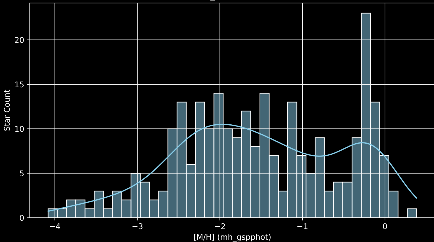
Gaia Cluster: [Tombaugh_2 [M/H] (mh_gspphot) (n= 260)
