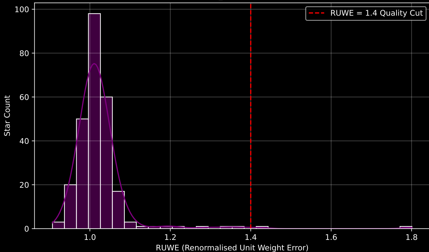
Gaia Cluster: [Tombaugh_2] RUWE Distribution (n= 260)
