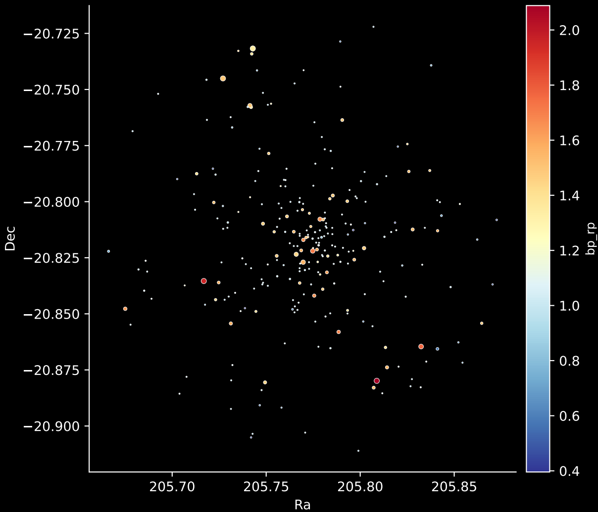
Gaia Cluster: [Tombaugh_2] Stars: 260
