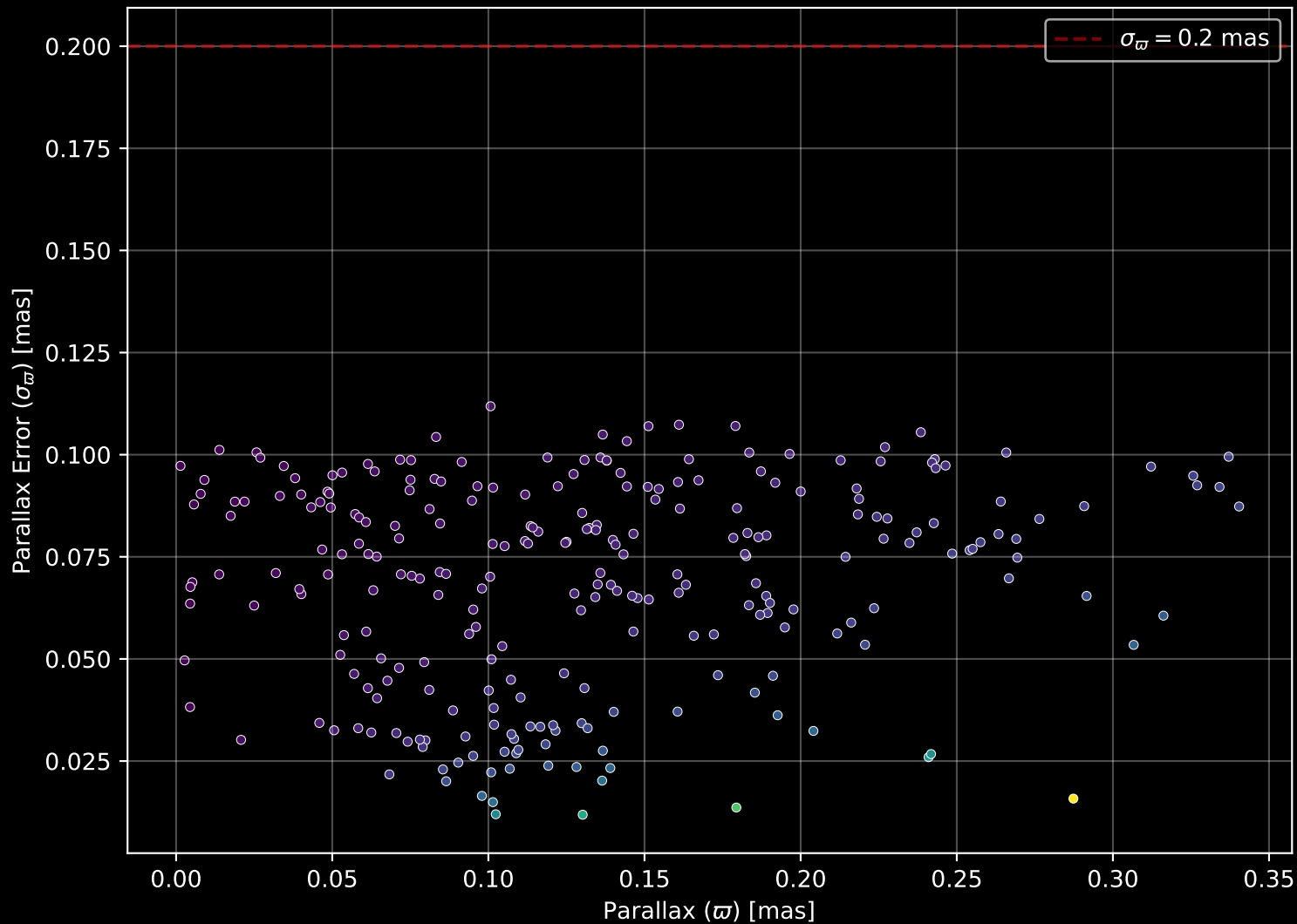
Gaia Cluster: [Tombaugh_2] Parallax Quality (n= 260)
