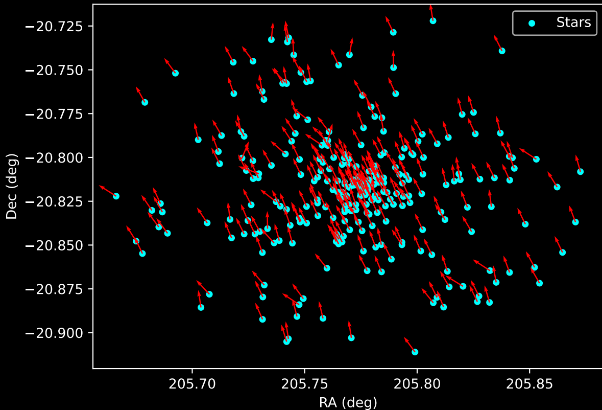
Gaia Cluster: [Tombaugh_2] Proper Motion Vectors for Gaia Star Field (n= 260)
