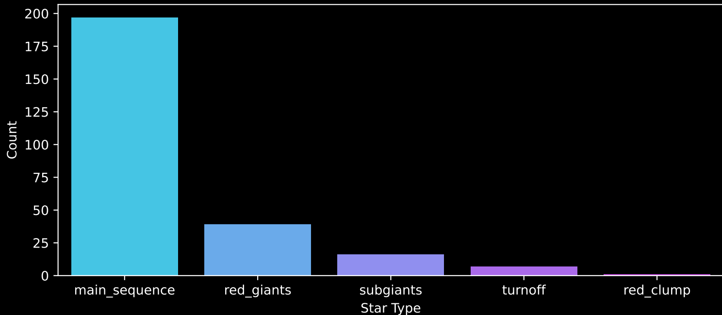
Gaia Cluster: [Tombaugh_2] Count plot of Star Type
