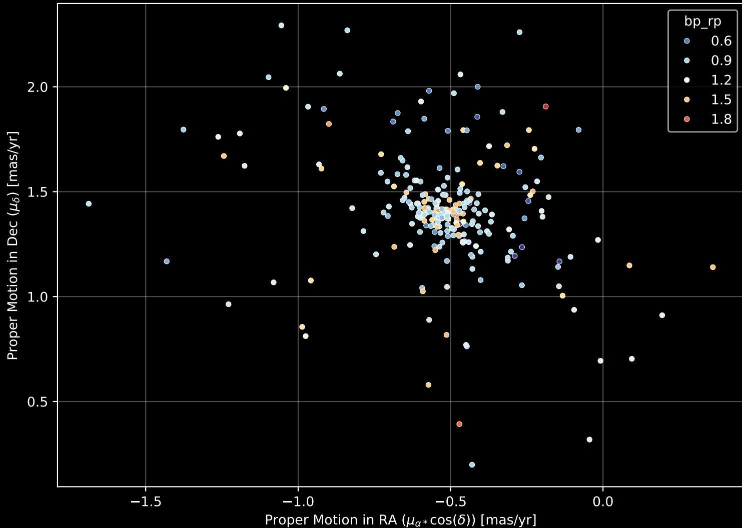
Gaia Cluster: [Tombaugh_2] Proper Motion Diagram (n= 260)
