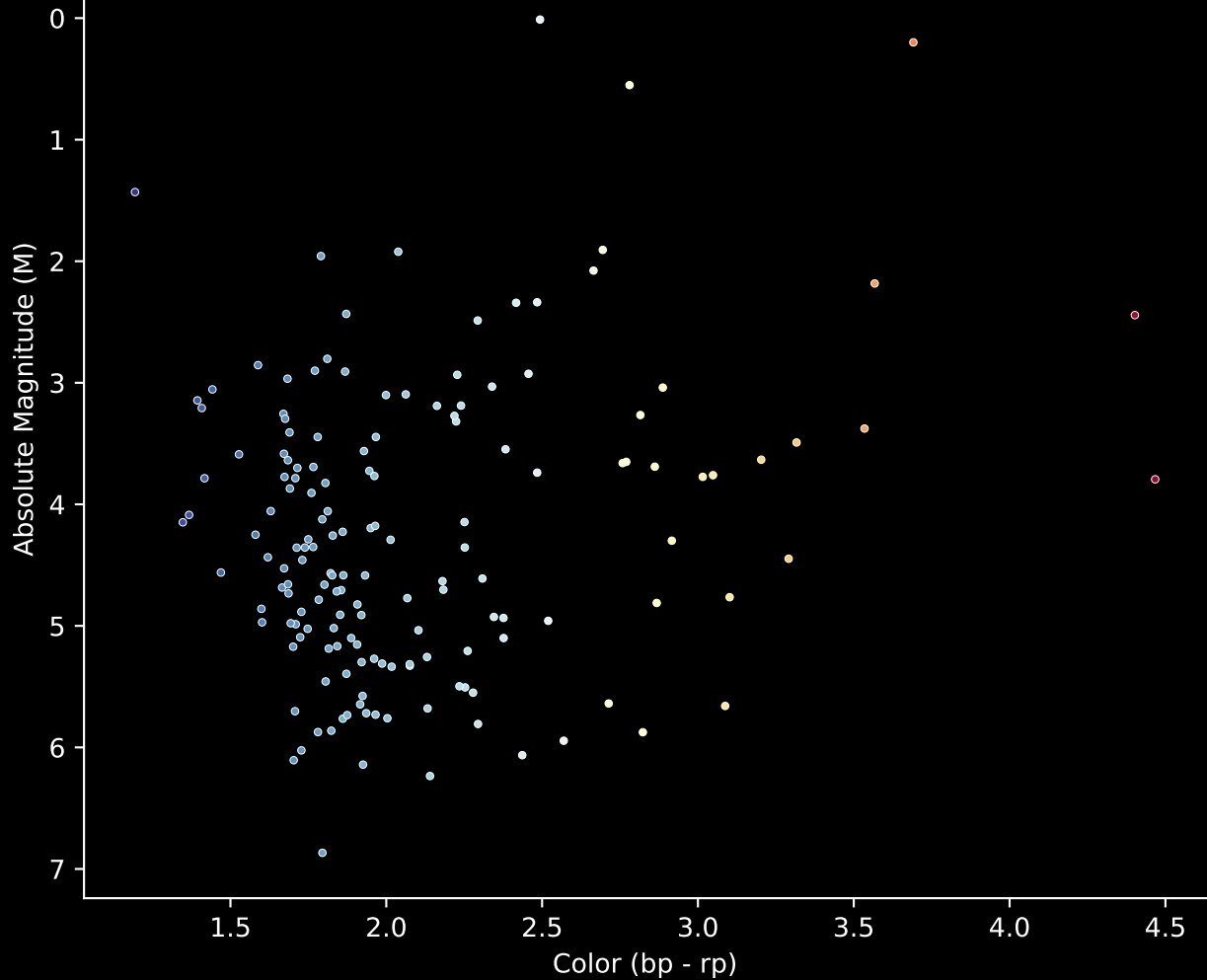
Gaia Cluster: [Tombaugh_4] Stars (n= 160) Hertzsprung-Russel Diagram
