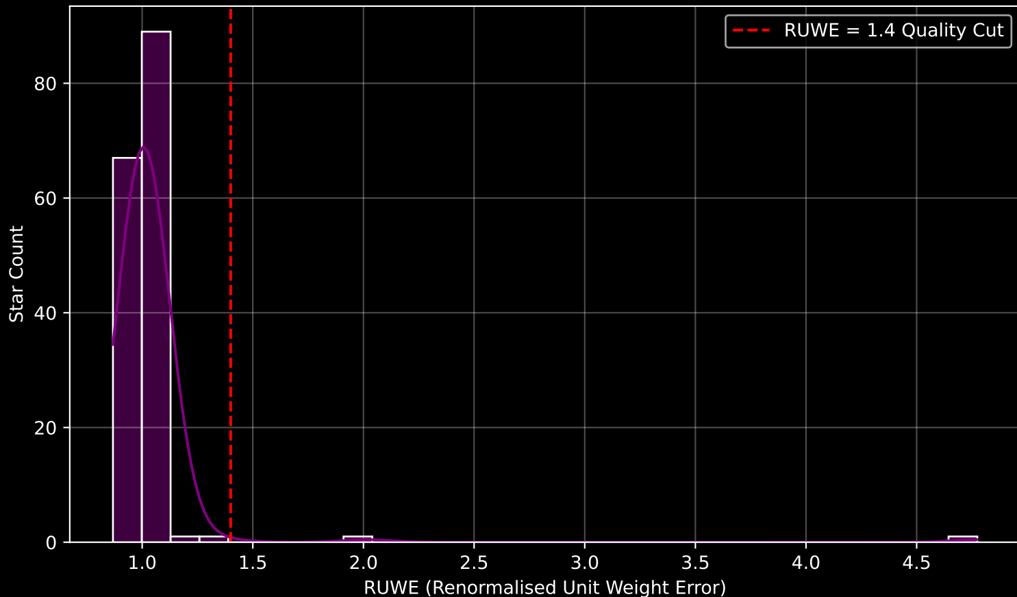
Gaia Cluster: [Tombaugh_4] RUWE Distribution (n= 160)
