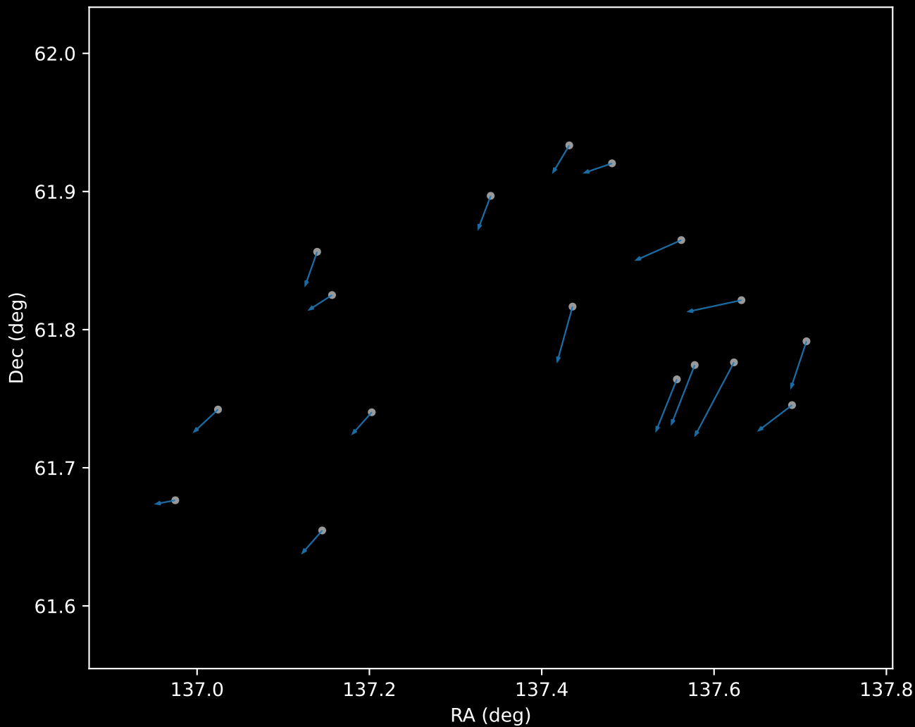
Gaia DR3 Cluster 0 Proper Motion Vectors (n=17)
