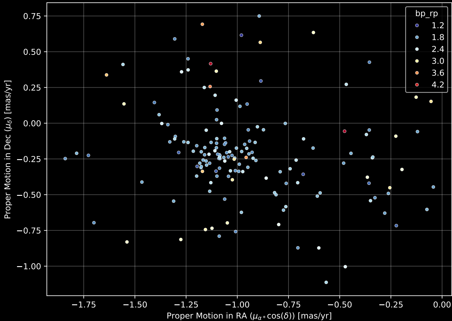
Gaia Cluster: [Tombaugh_4] Proper Motion Diagram (n= 160)
