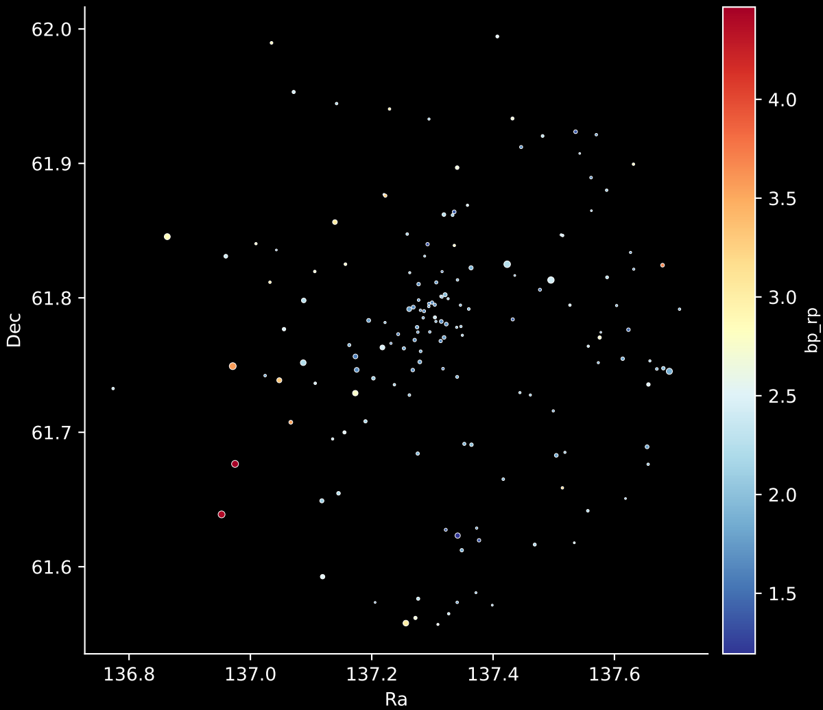
Gaia Cluster: [Tombaugh_4] Stars: 160
