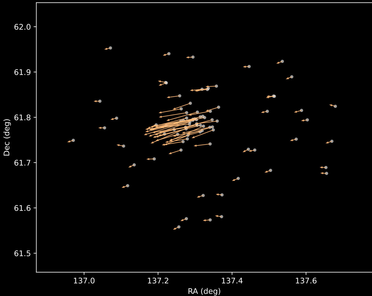
Gaia DR3 Cluster 3 Proper Motion Vectors (n=82)
