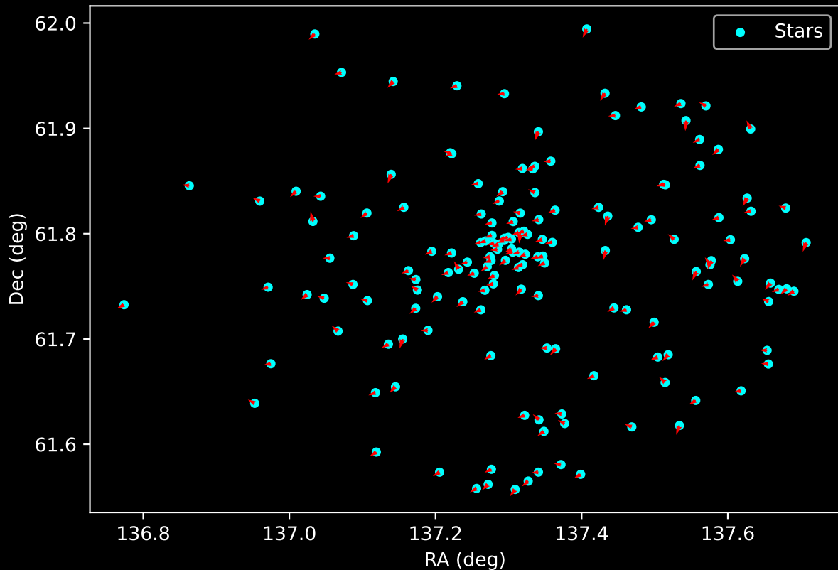
Gaia Cluster: [Tombaugh_4] Proper Motion Vectors for Gaia Star Field (n= 160)
