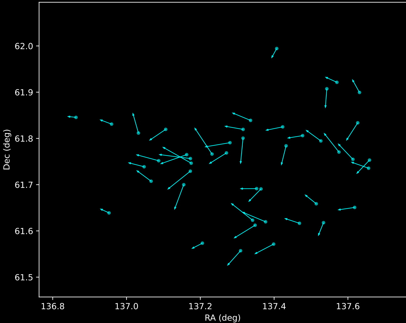
Gaia DR3 Noise Stream Proper Motion Vectors (n=44)
