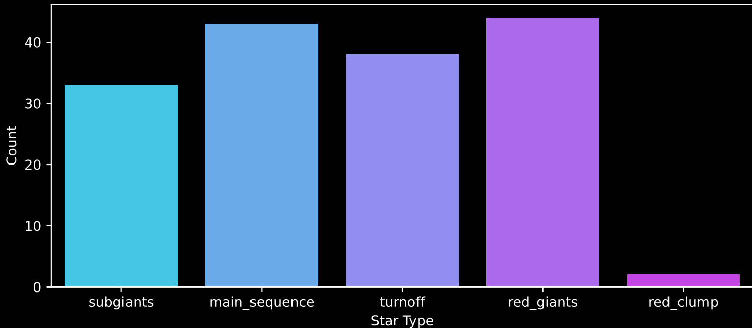
Gaia Cluster: [Tombaugh_4] Count plot of Star Type
