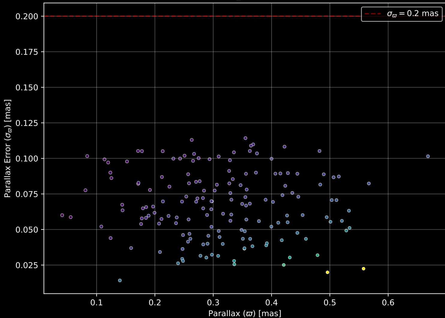
Gaia Cluster: [Tombaugh_4] Parallax Quality (n= 160)
