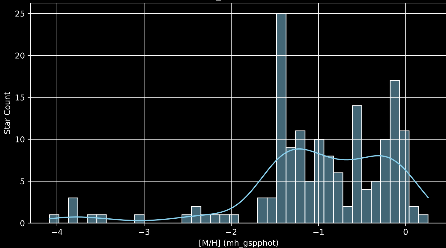
Gaia Cluster: [Tombaugh_4 [M/H] (mh_gspphot) (n= 160)
