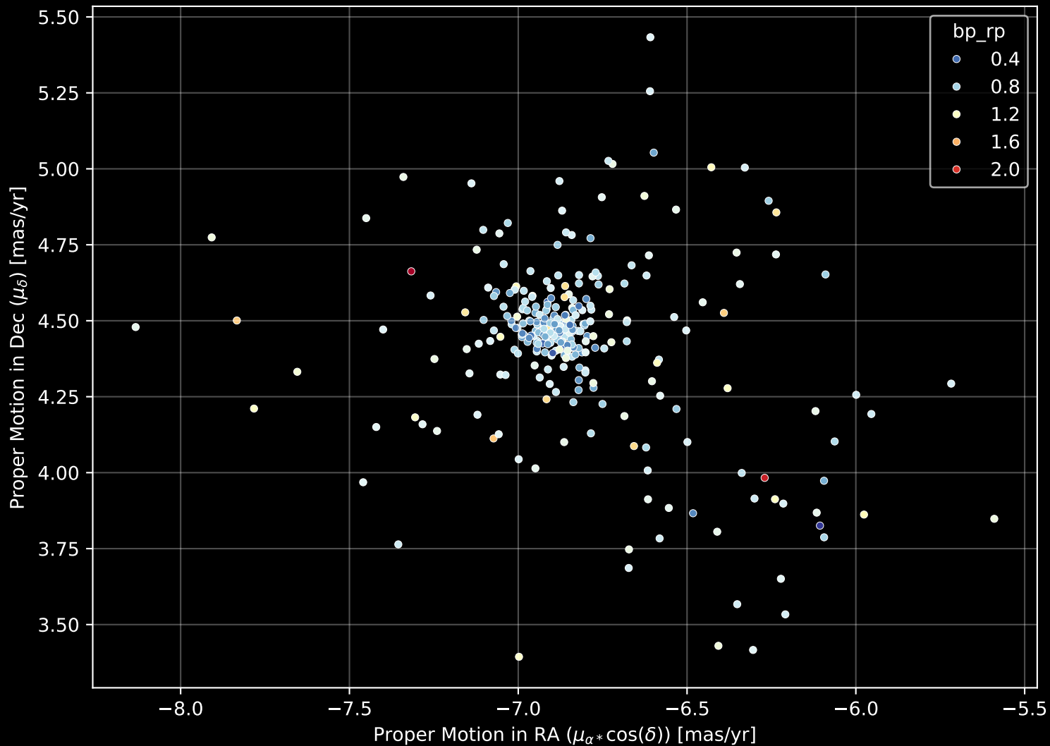
Gaia Cluster: [Trumpler_12] Proper Motion Diagram (n= 307)
