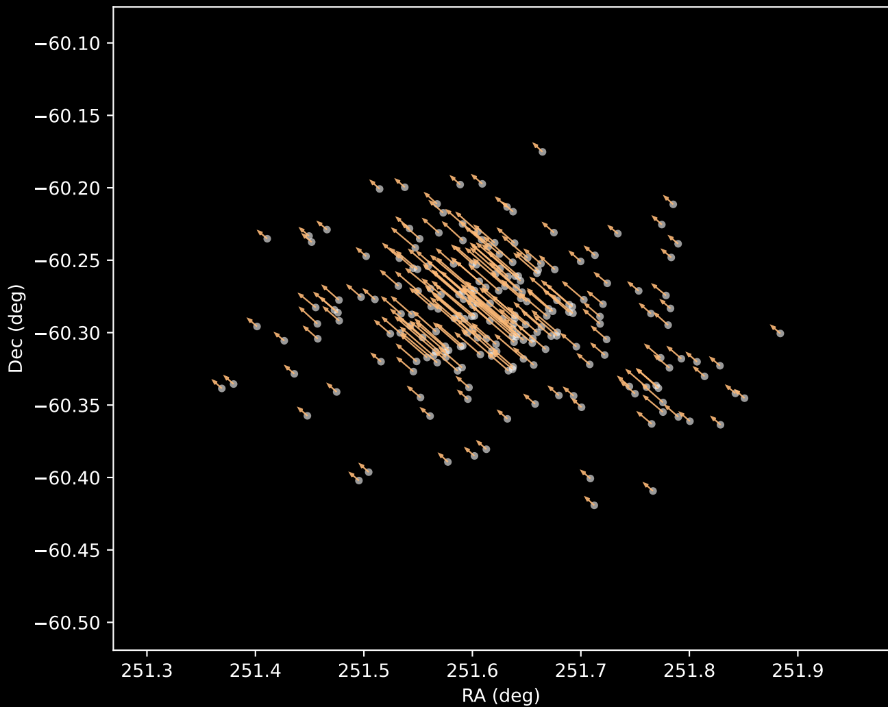
Gaia DR3 Cluster 3 Proper Motion Vectors (n=212)
