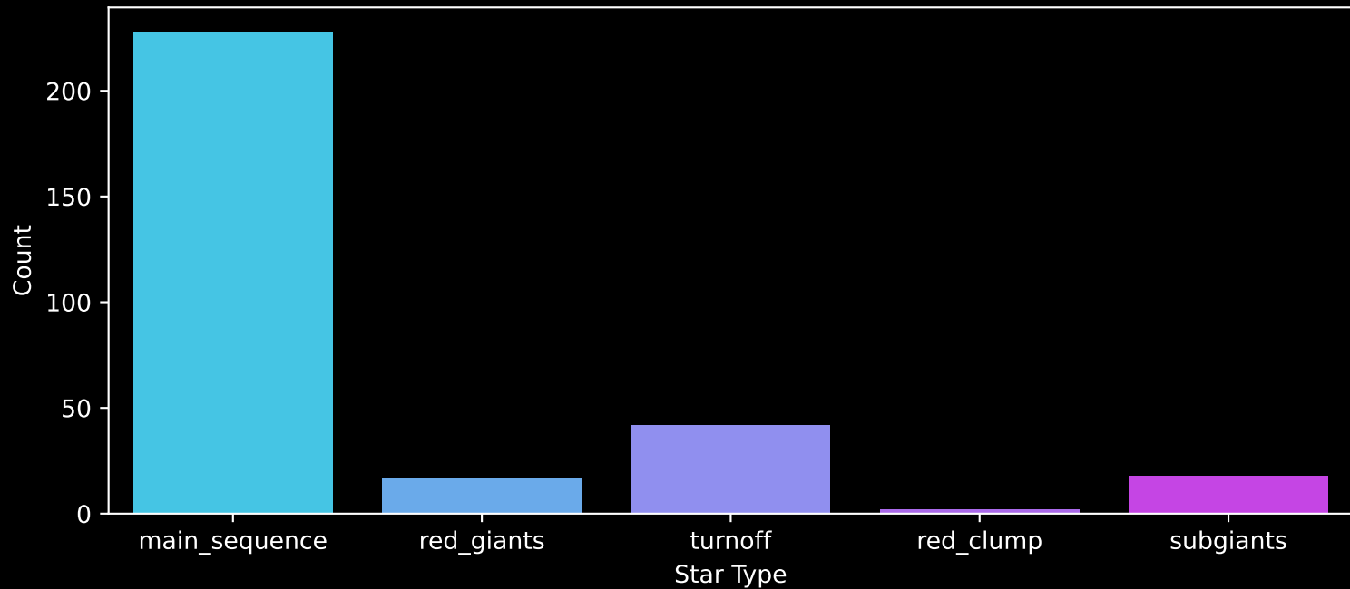
Gaia Cluster: [Trumpler_12] Count plot of Star Type
