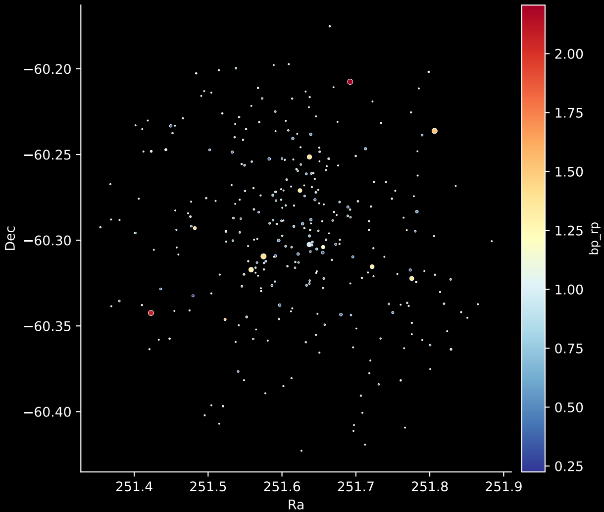
Gaia Cluster: [Trumpler_12] Stars: 307
