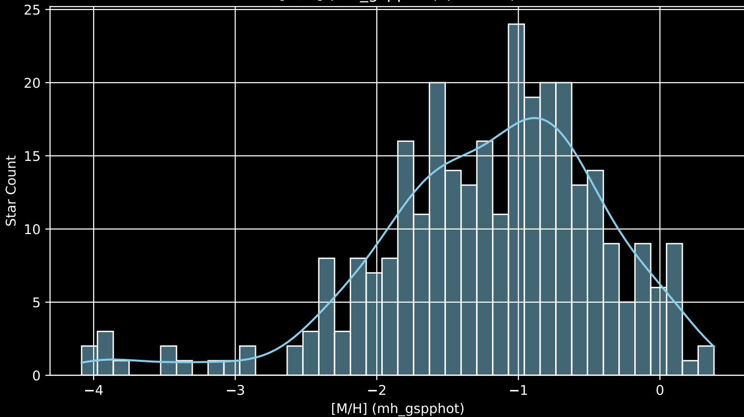
Gaia Cluster: [Trumpler_12 [M/H] (mh_gspphot) (n= 304)
