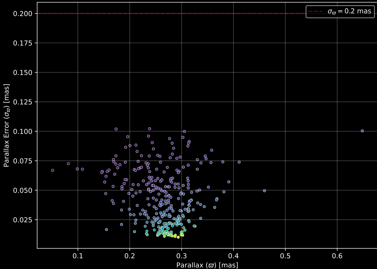
Gaia Cluster: [Trumpler_12] Parallax Quality (n= 307)
