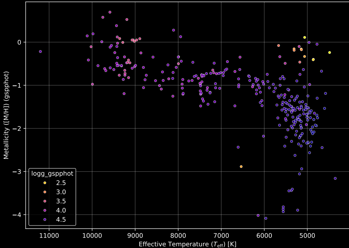
Gaia Cluster: [Trumpler_12] Stellar Population Parameters (n= 307)
