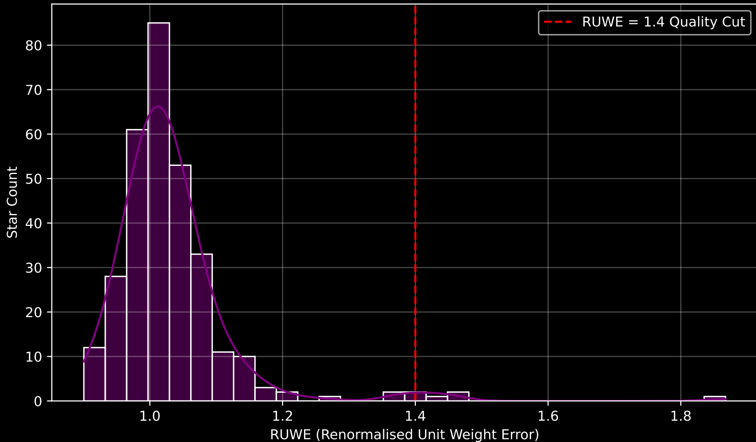
Gaia Cluster: [Trumpler_12] RUWE Distribution (n= 307)
