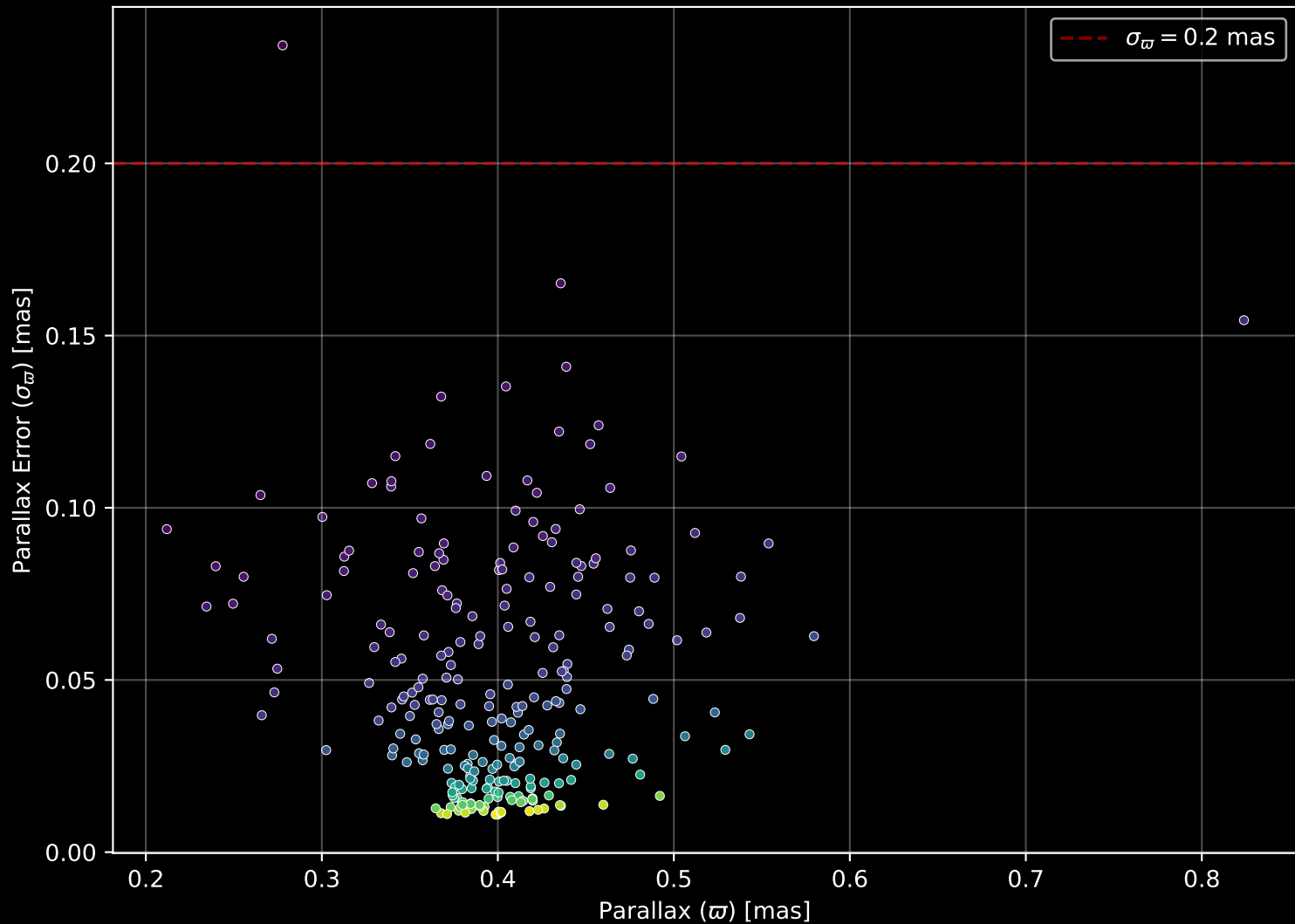
Gaia Cluster: [Trumpler_14] Parallax Quality (n= 253)
