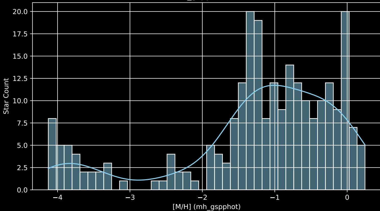
Gaia Cluster: [Trumpler_14 [M/H] (mh_gspphot) (n= 250)
