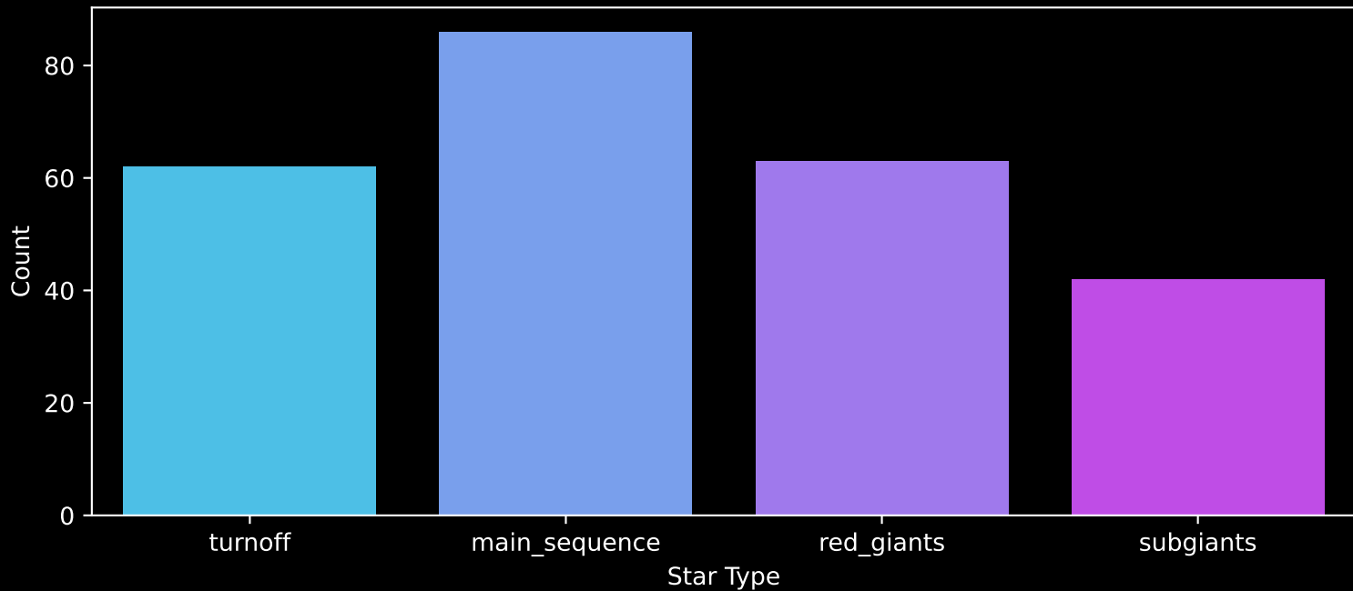
Gaia Cluster: [Trumpler_14] Count plot of Star Type
