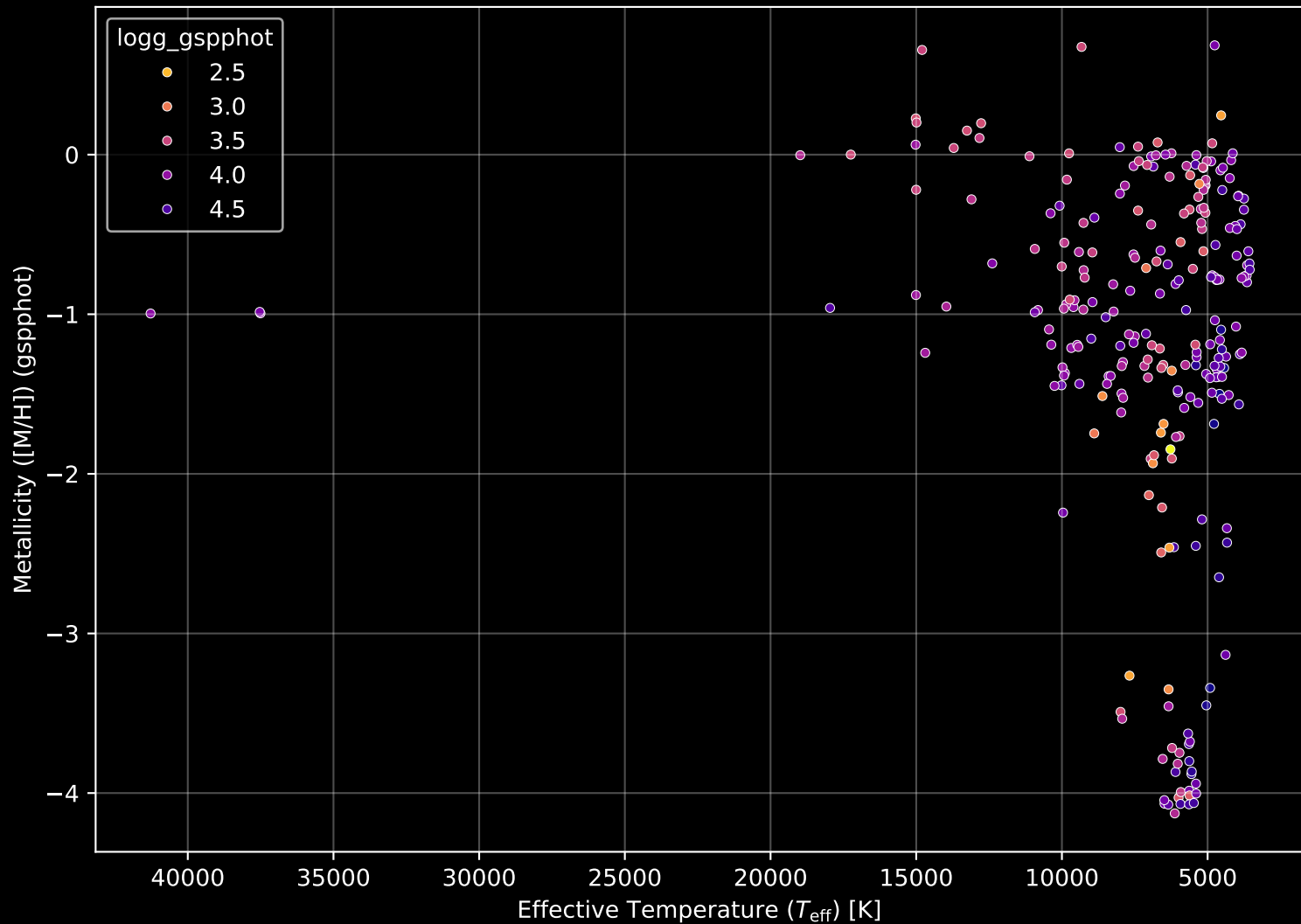
Gaia Cluster: [Trumpler_14] Stellar Population Parameters (n= 253)
