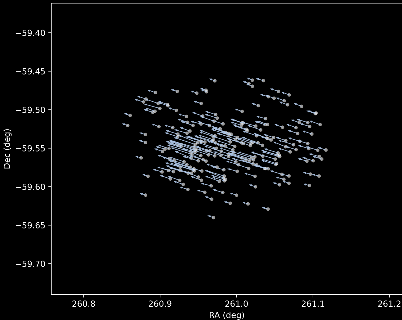
Gaia DR3 Cluster 1 Proper Motion Vectors (n=218)
