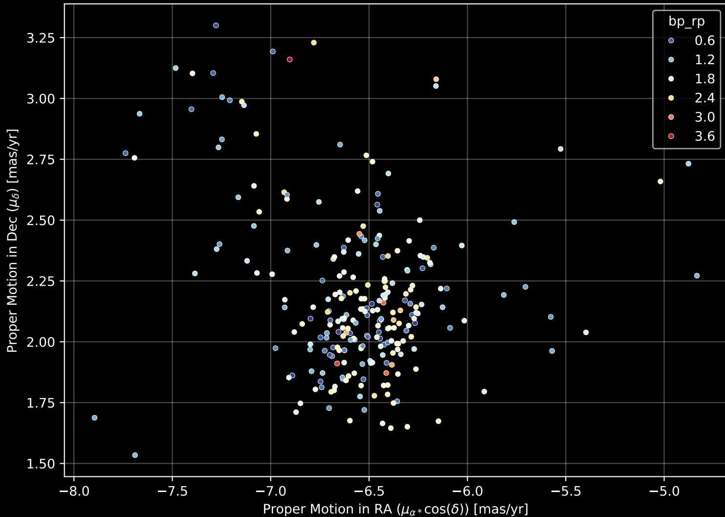
Gaia Cluster: [Trumpler_14] Proper Motion Diagram (n= 253)
