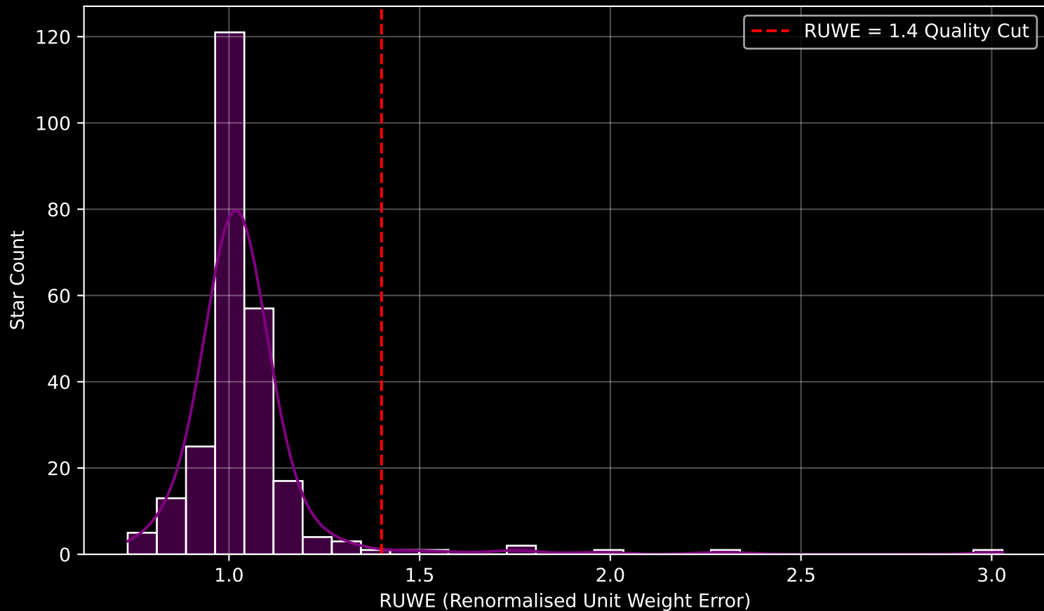
Gaia Cluster: [Trumpler_14] RUWE Distribution (n= 253)
