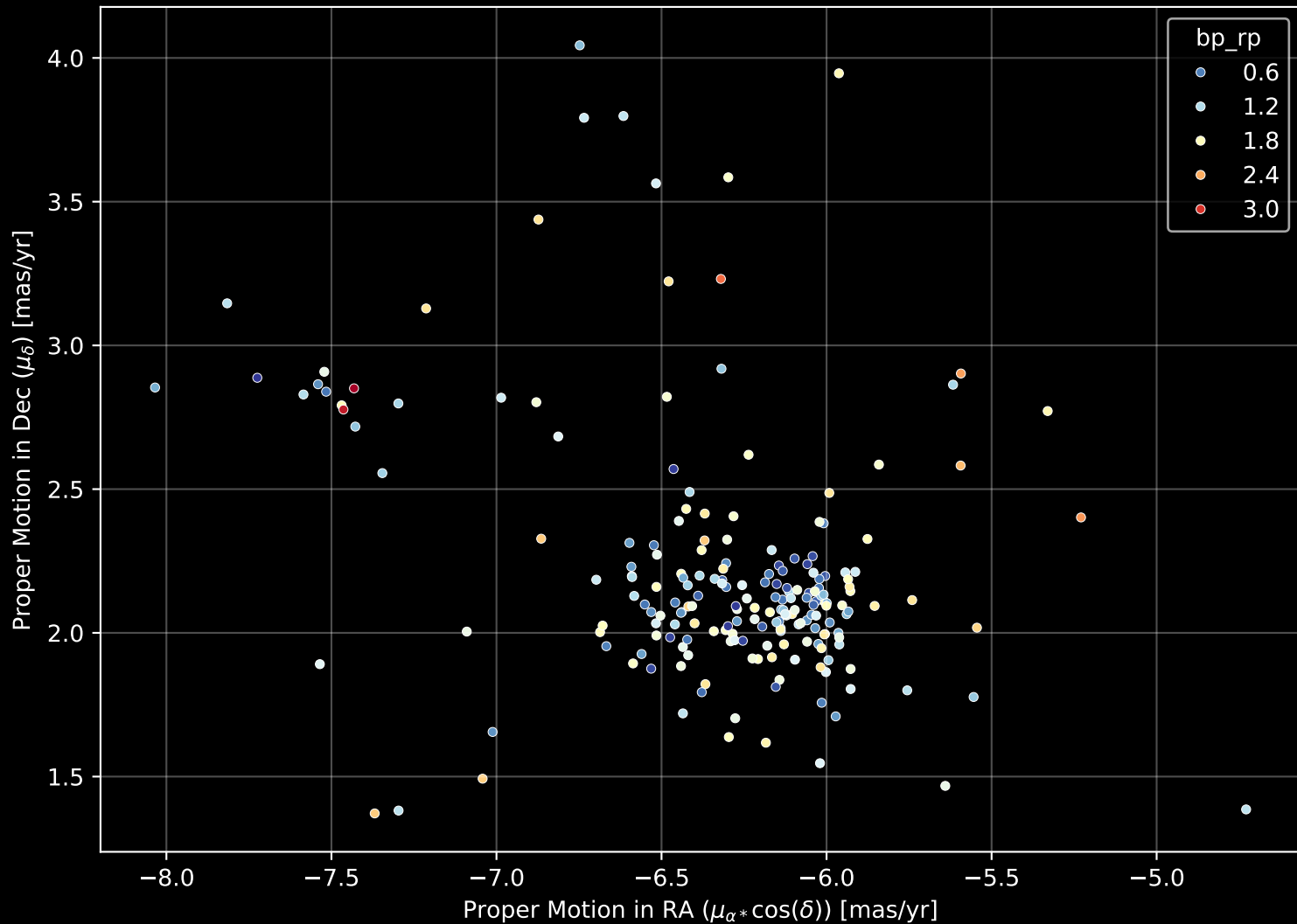
Gaia Cluster: [Trumpler_15] Proper Motion Diagram (n= 206)
