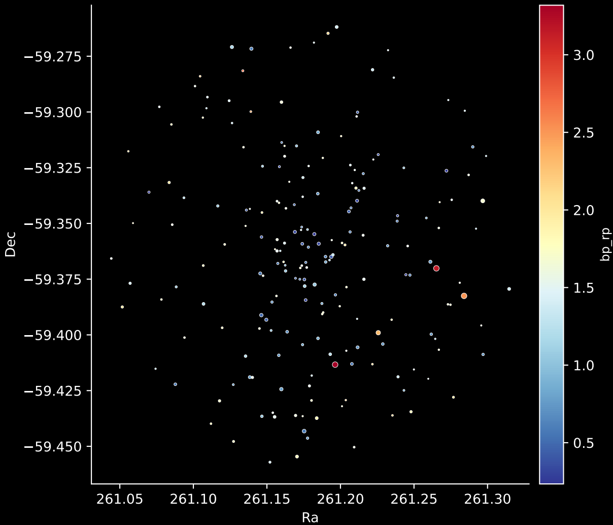
Gaia Cluster: [Trumpler_15] Stars: 206
