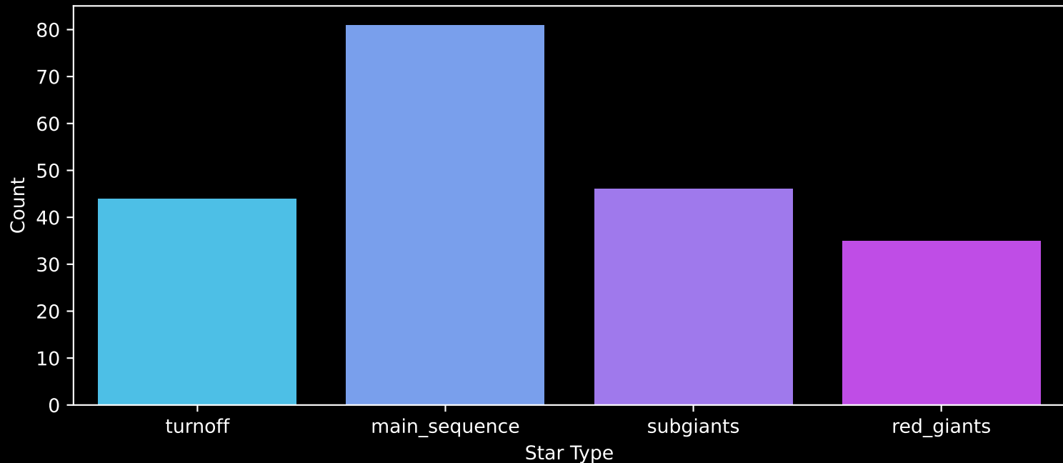
Gaia Cluster: [Trumpler_15] Count plot of Star Type
