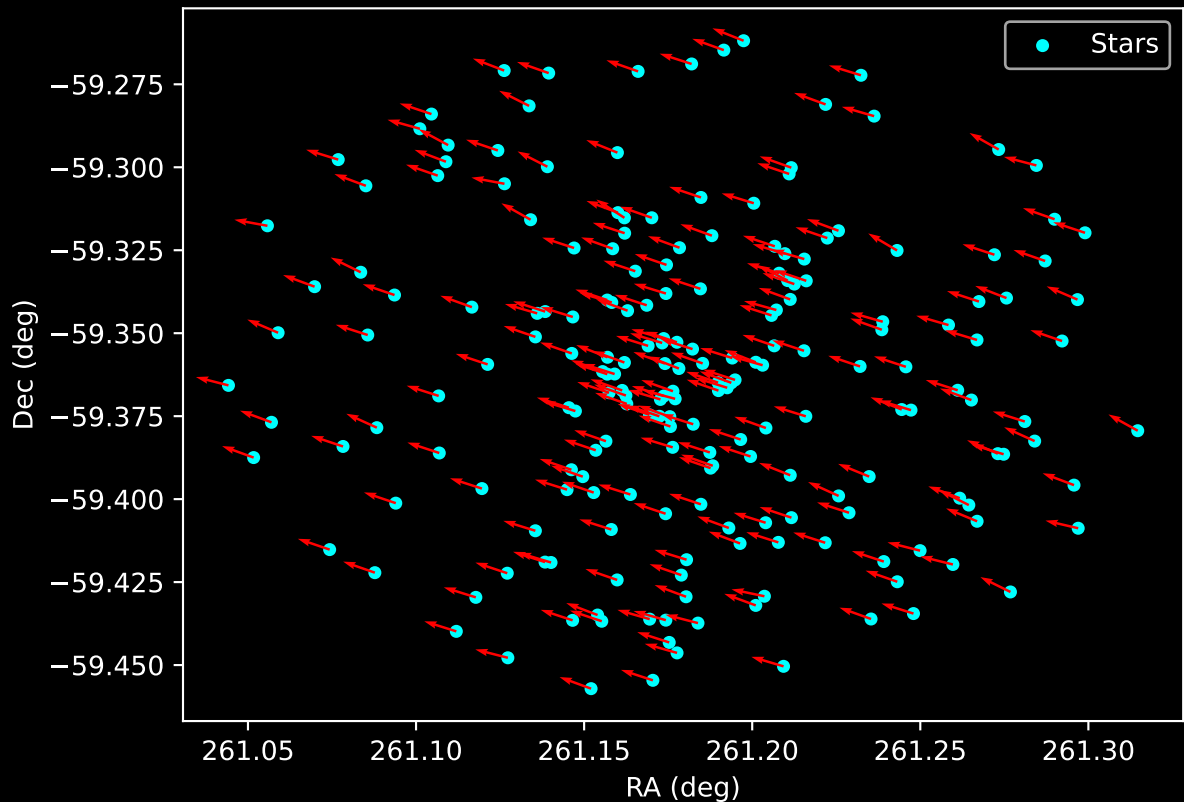
Gaia Cluster: [Trumpler_15] Proper Motion Vectors for Gaia Star Field (n= 206)
