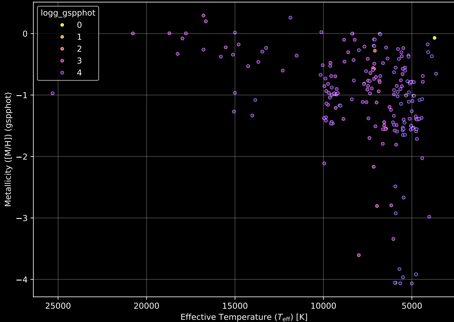
Gaia Cluster: [Trumpler_15] Stellar Population Parameters (n= 206)
