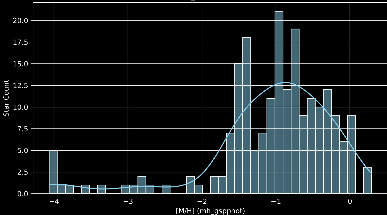
Gaia Cluster: [Trumpler_15 [M/H] (mh_gspphot) (n= 206)
