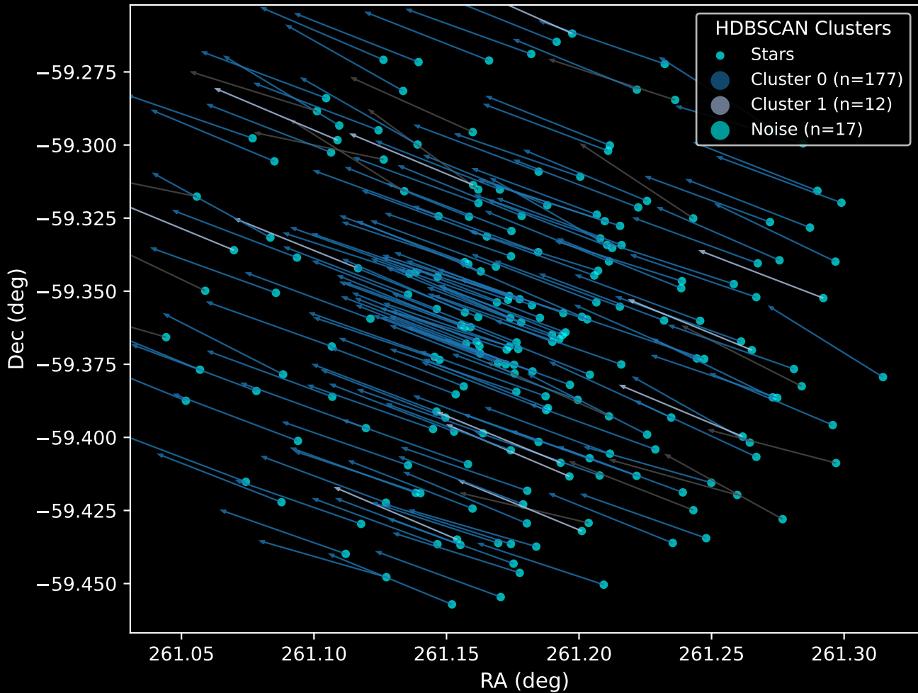
Gaia Cluster: [Trumpler_15] Proper Motion Vectors with HDBSCAN (n=206)
