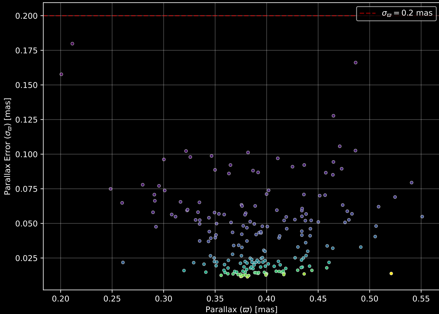
Gaia Cluster: [Trumpler_15] Parallax Quality (n= 206)
