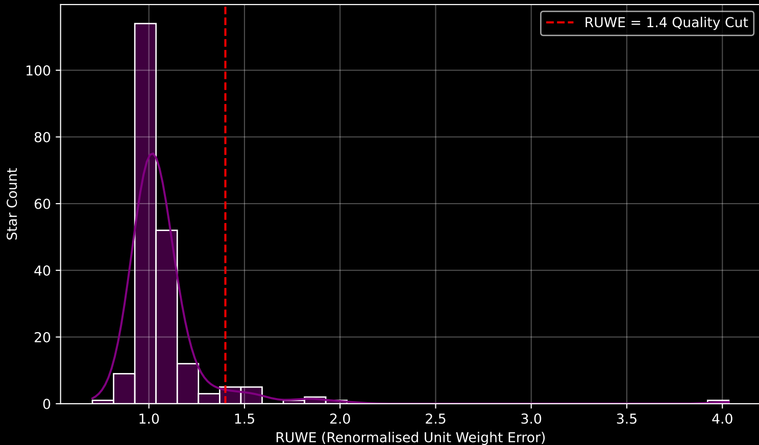
Gaia Cluster: [Trumpler_15] RUWE Distribution (n= 206)
