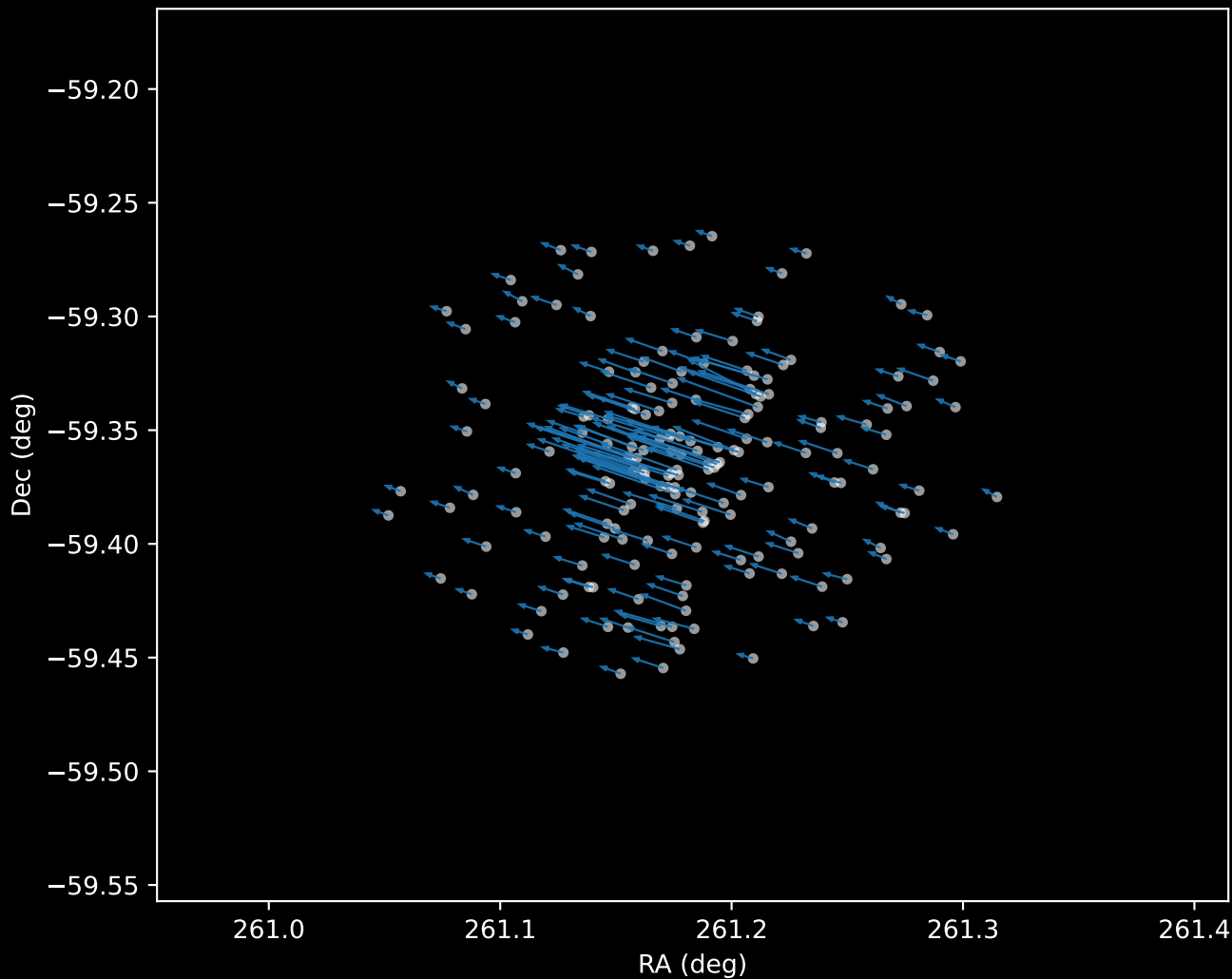
Gaia DR3 Cluster 0 Proper Motion Vectors (n=177)
