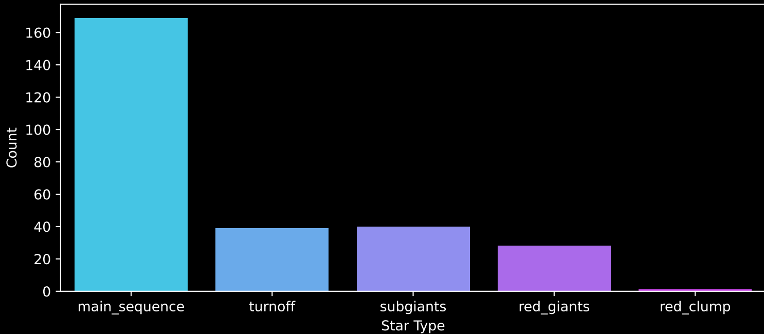
Gaia Cluster: [Trumpler_17] Count plot of Star Type
