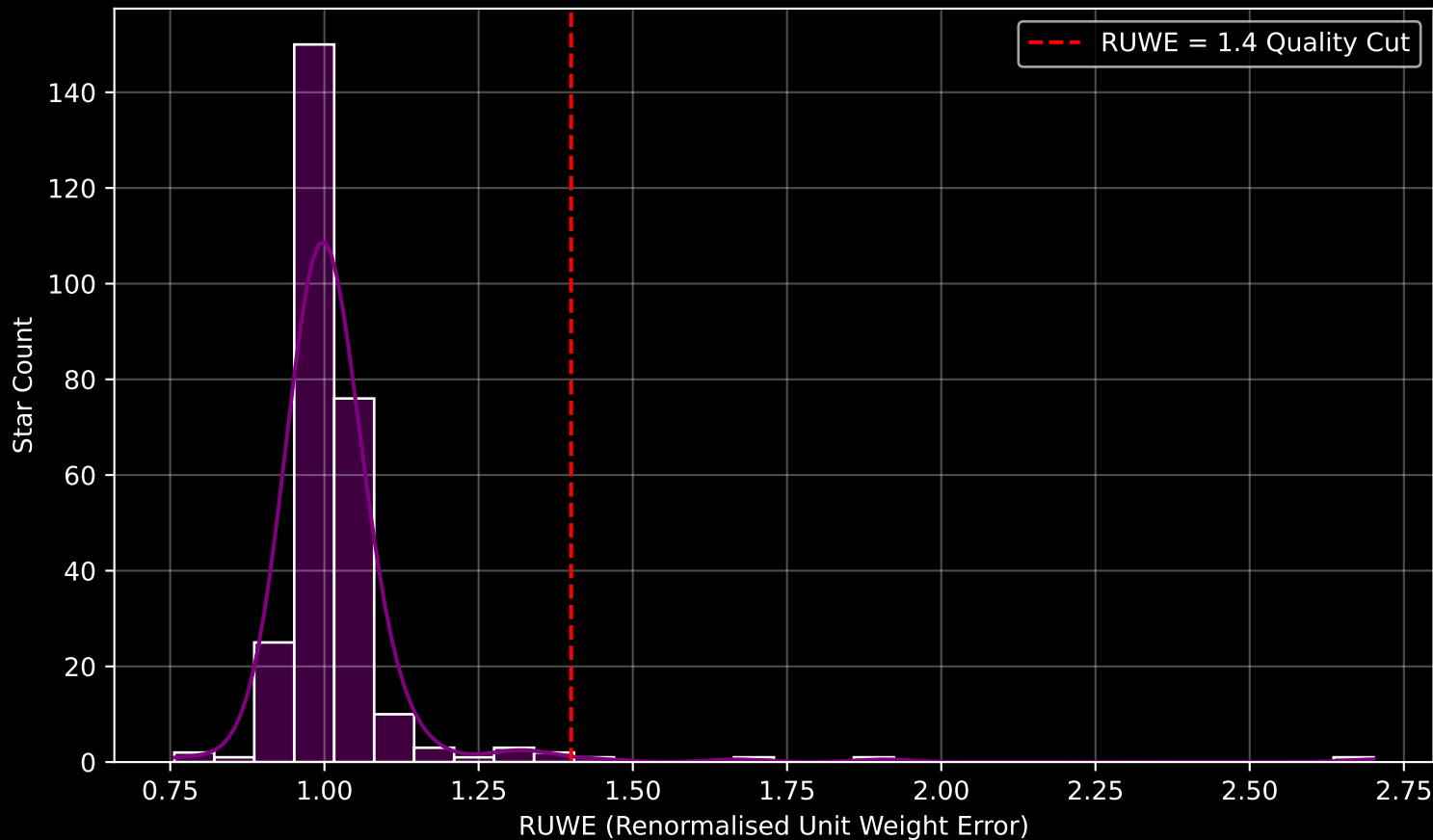
Gaia Cluster: [Trumpler_17] RUWE Distribution (n= 277)
