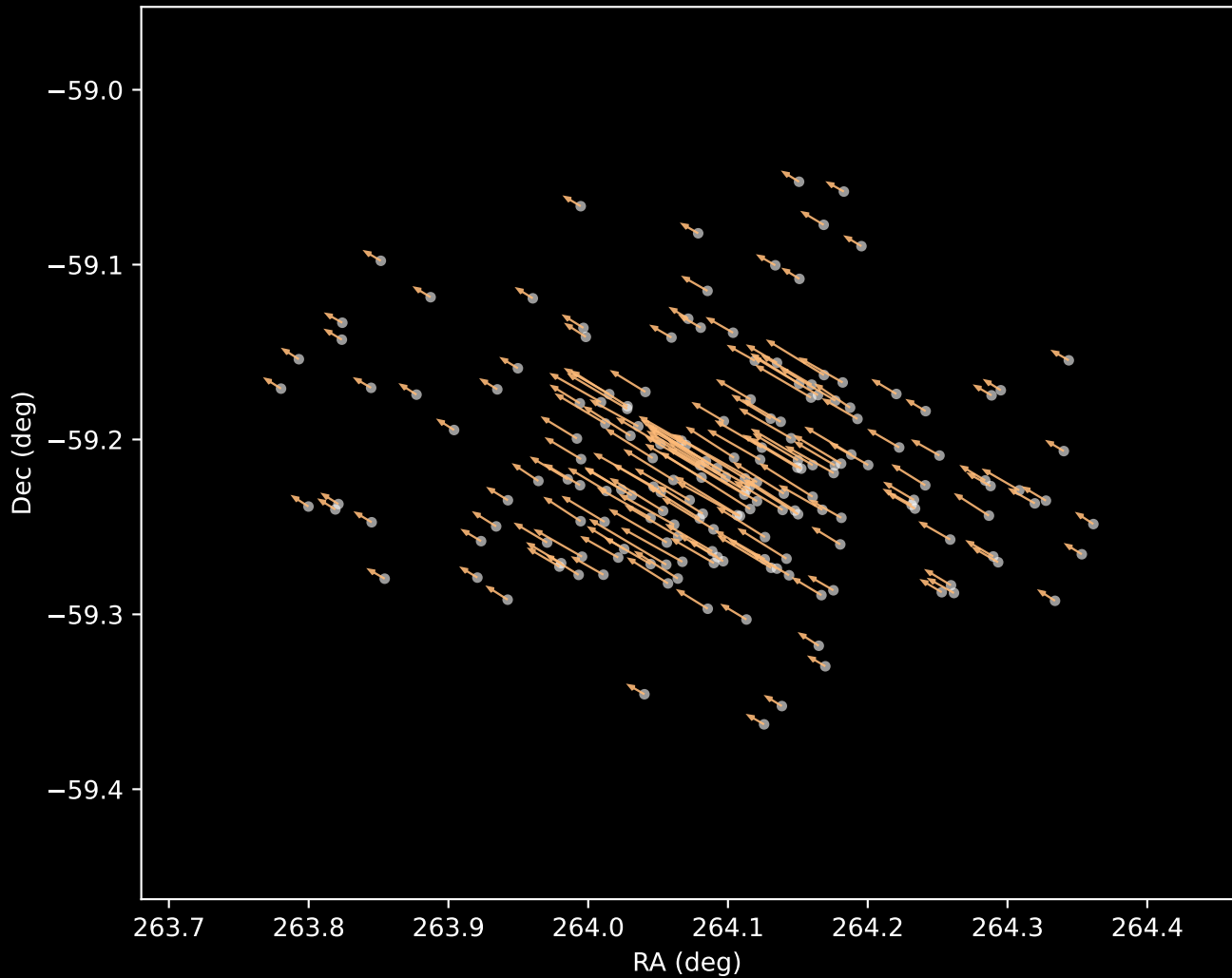
Gaia DR3 Cluster 3 Proper Motion Vectors (n=181)
