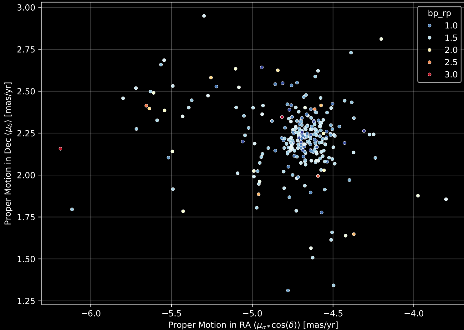
Gaia Cluster: [Trumpler_17] Proper Motion Diagram (n= 277)
