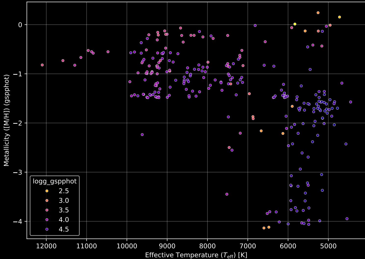
Gaia Cluster: [Trumpler_17] Stellar Population Parameters (n= 277)
