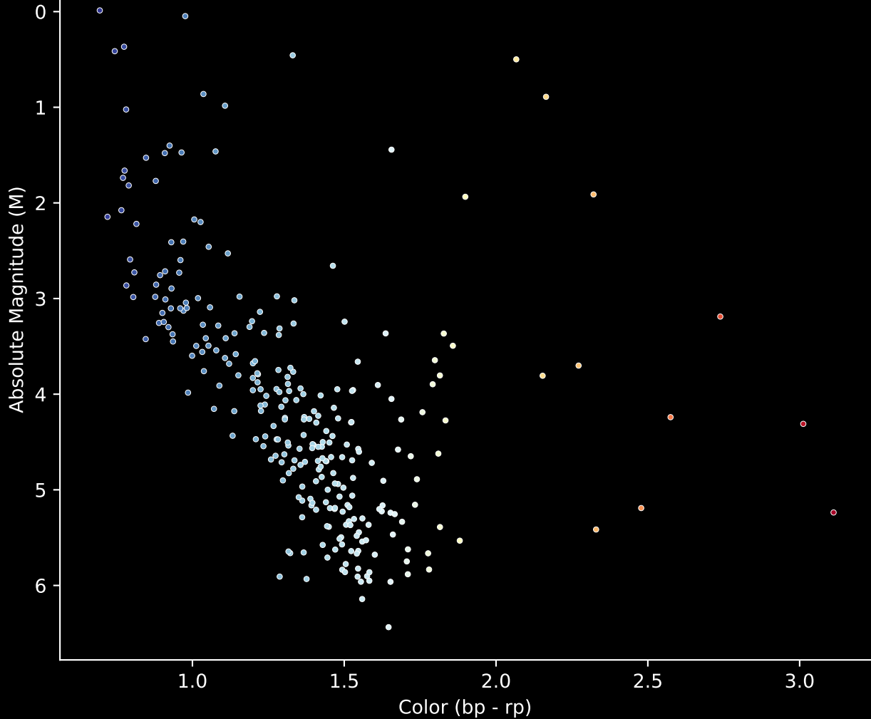
Gaia Cluster: [Trumpler_17] Stars (n= 277) Hertzsprung-Russel Diagram
