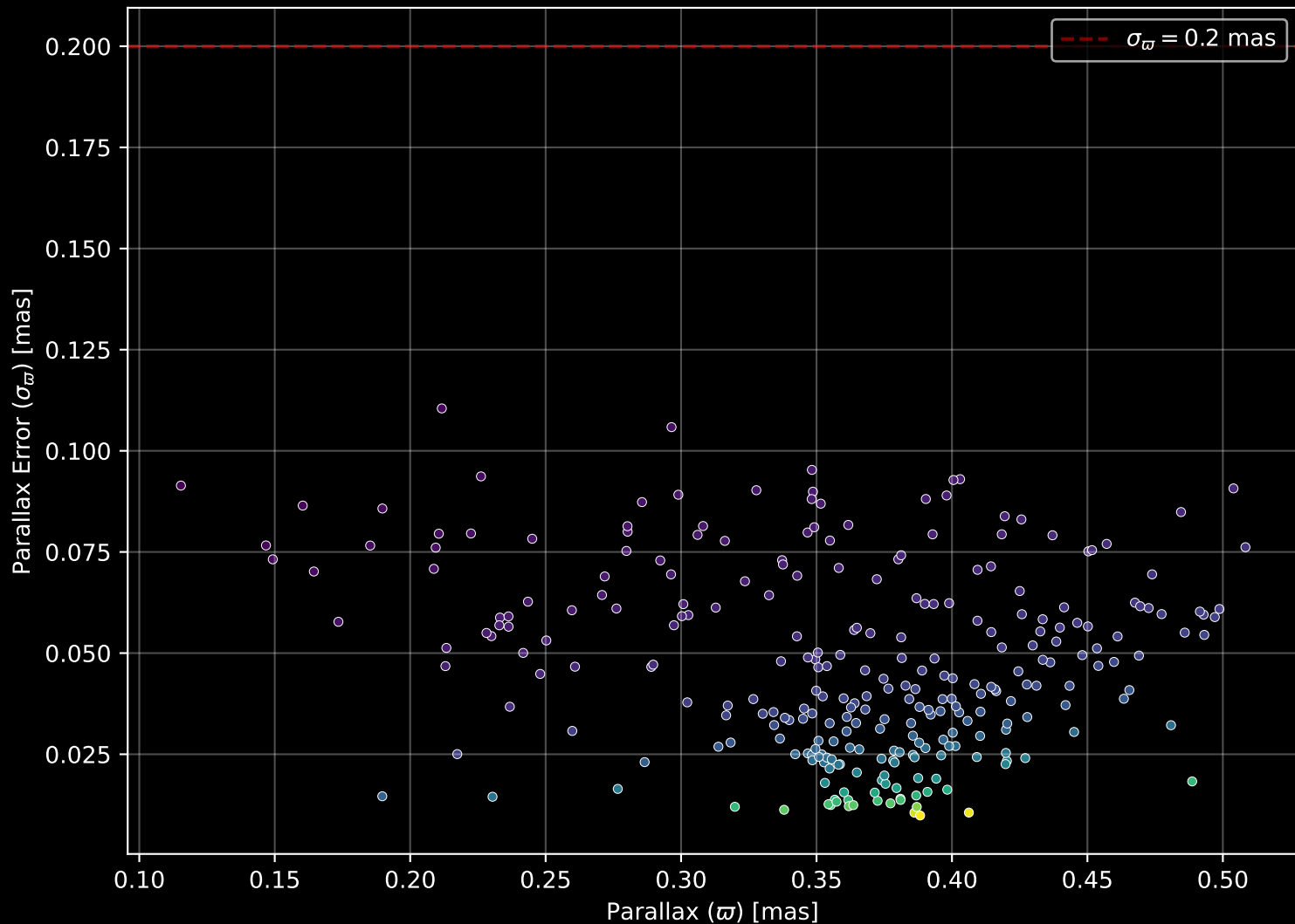
Gaia Cluster: [Trumpler_17] Parallax Quality (n= 277)
