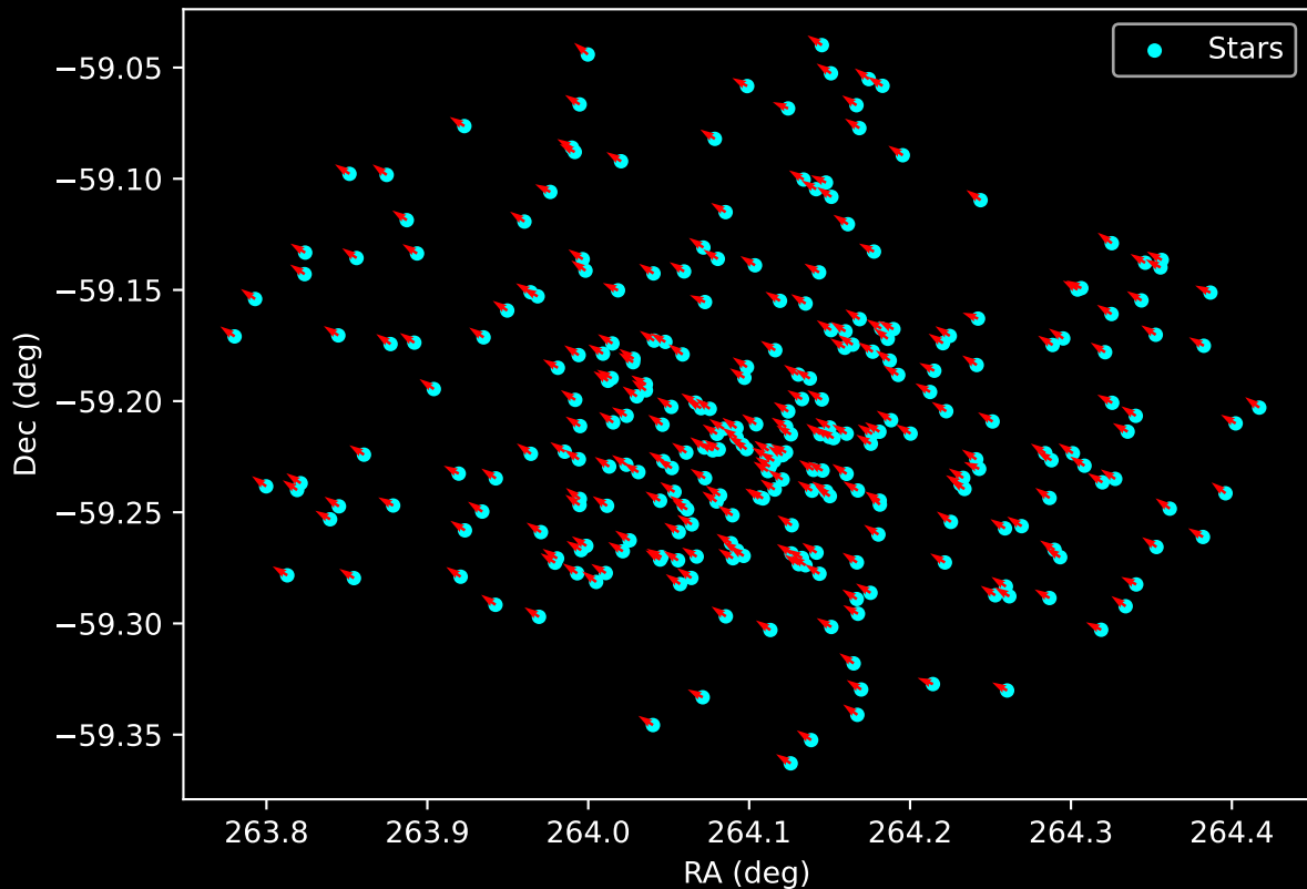
Gaia Cluster: [Trumpler_17] Proper Motion Vectors for Gaia Star Field (n= 277)
