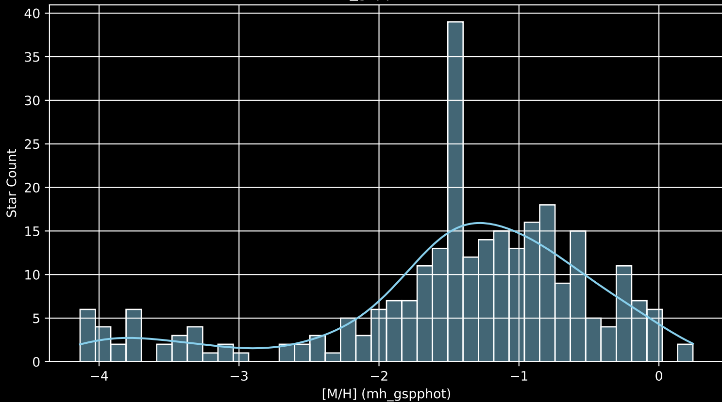
Gaia Cluster: [Trumpler_17 [M/H] (mh_gspphot) (n= 277)
