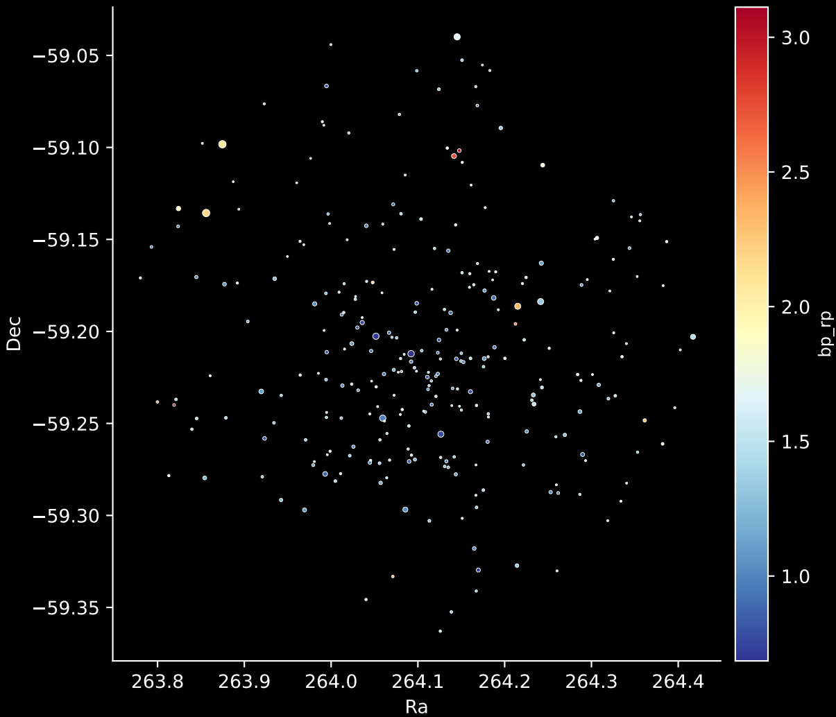
Gaia Cluster: [Trumpler_17] Stars: 277
