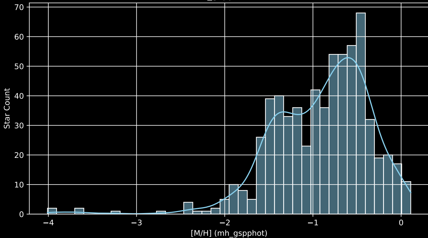
Gaia Cluster: [Trumpler_19 [M/H] (mh_gspphot) (n= 649)
