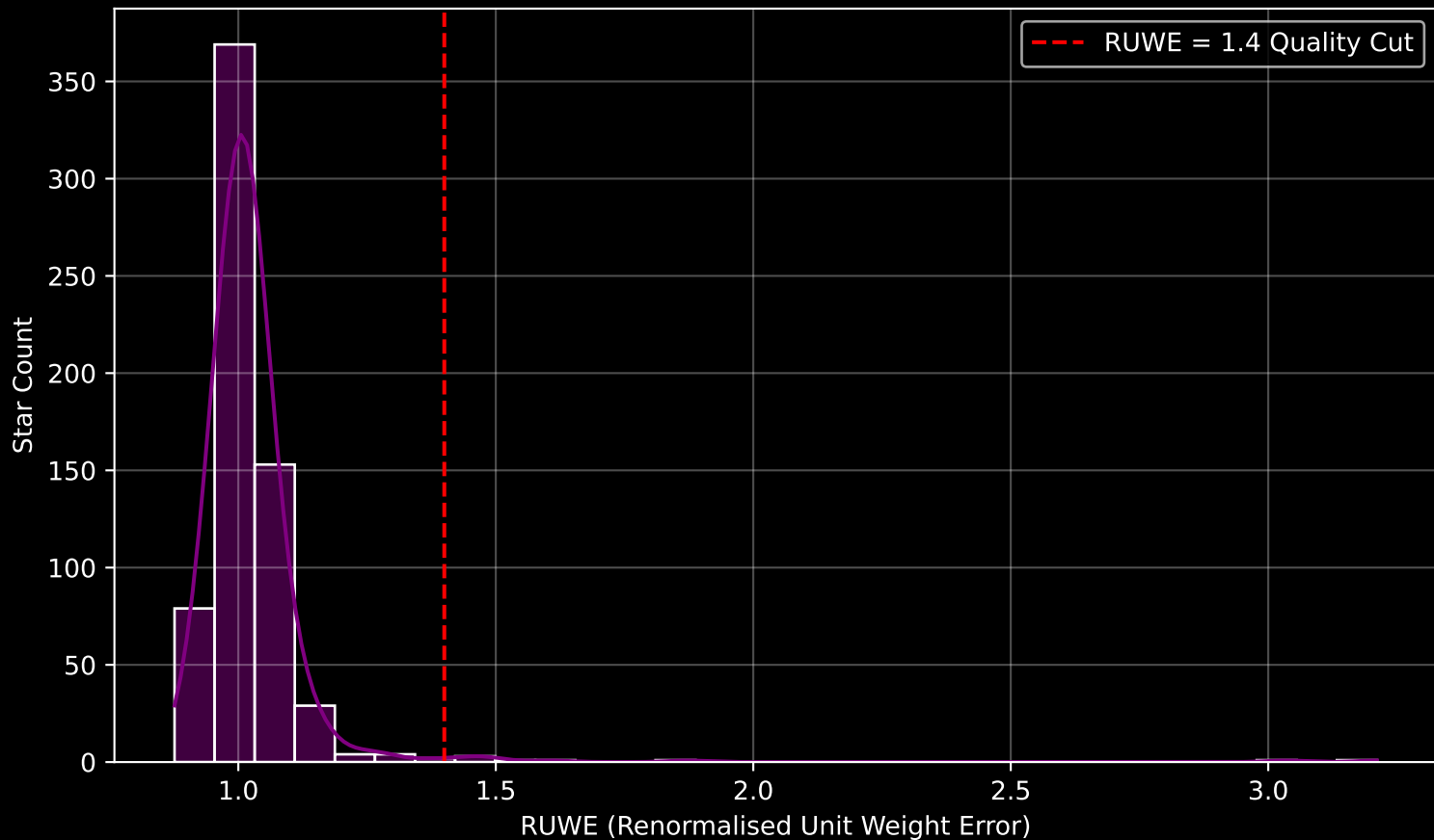
Gaia Cluster: [Trumpler_19] RUWE Distribution (n= 648)
