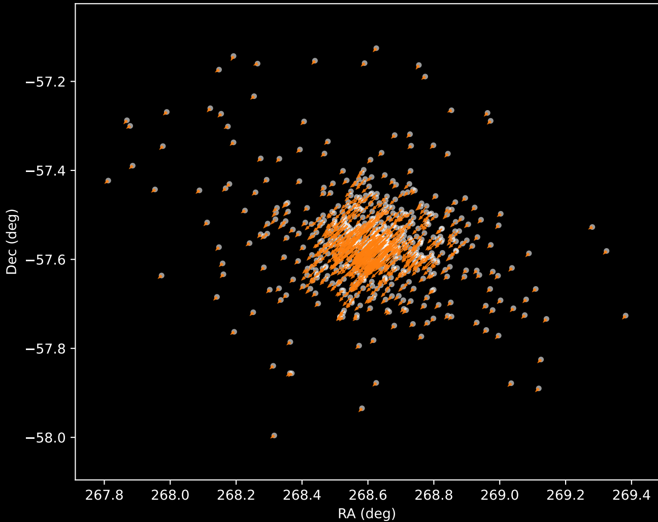
Gaia DR3 Cluster 2 Proper Motion Vectors (n=607)
