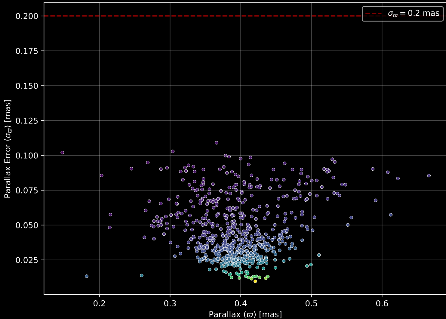
Gaia Cluster: [Trumpler_19] Parallax Quality (n= 649)
