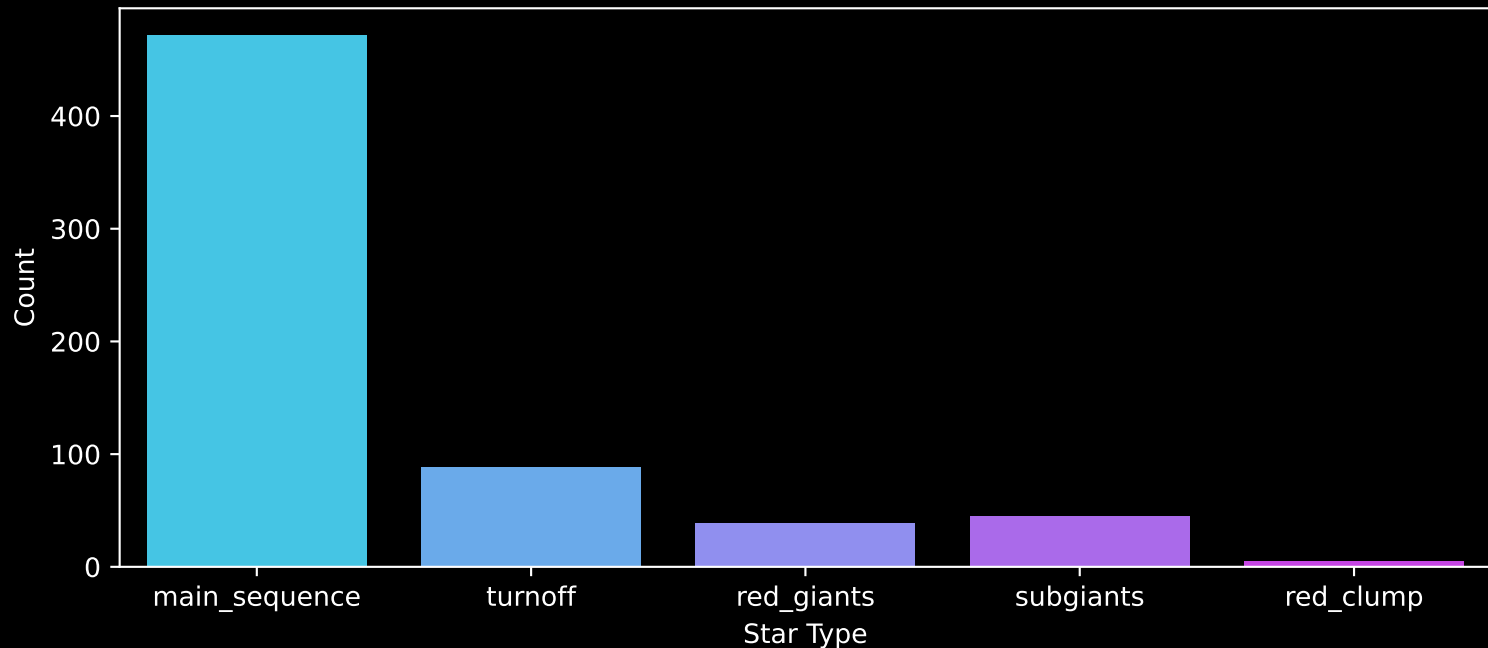
Gaia Cluster: [Trumpler_19] Count plot of Star Type
