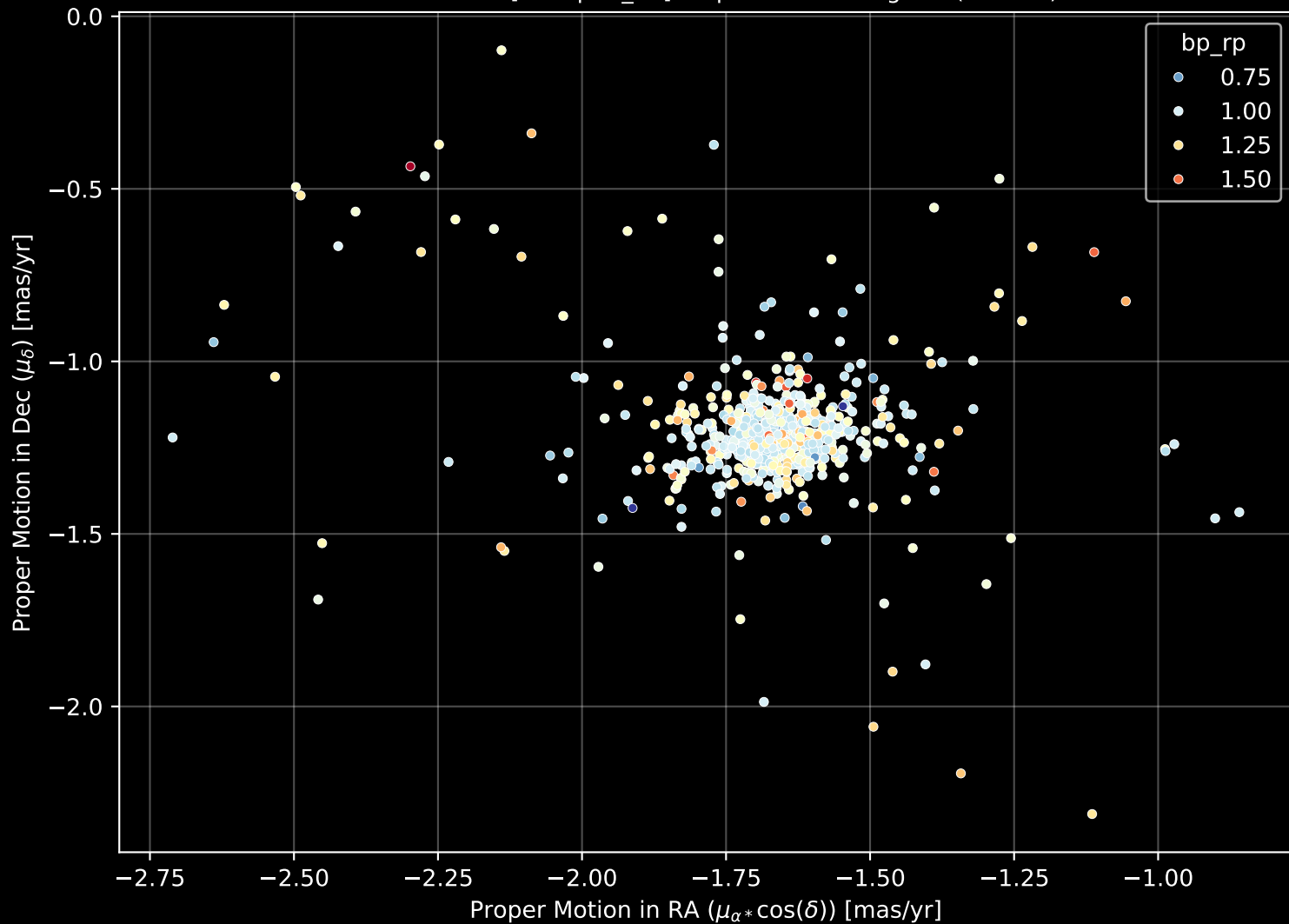
Gaia Cluster: [Trumpler_19] Proper Motion Diagram (n= 649)
