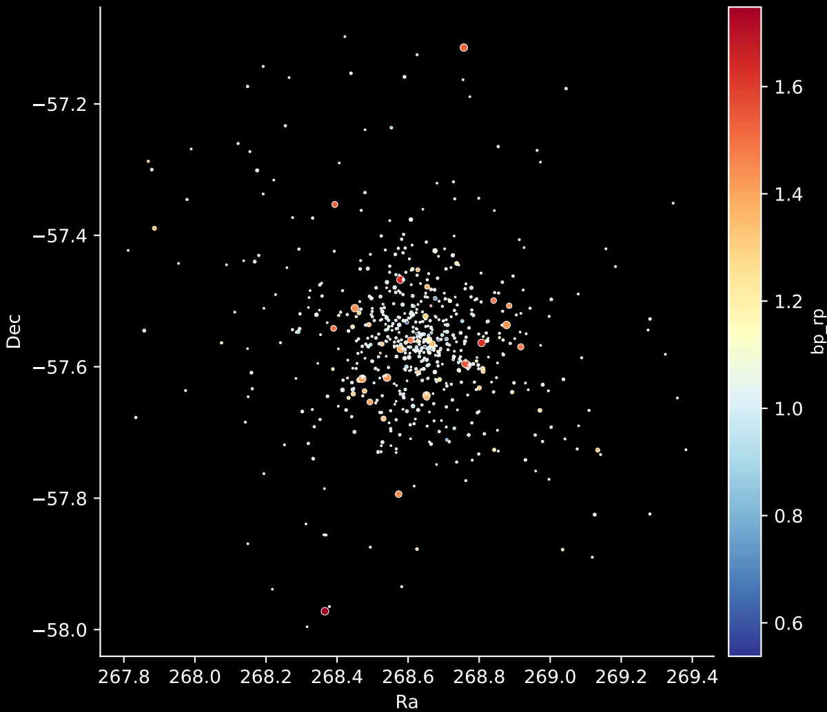
Gaia Cluster: [Trumpler_19] Stars: 649
