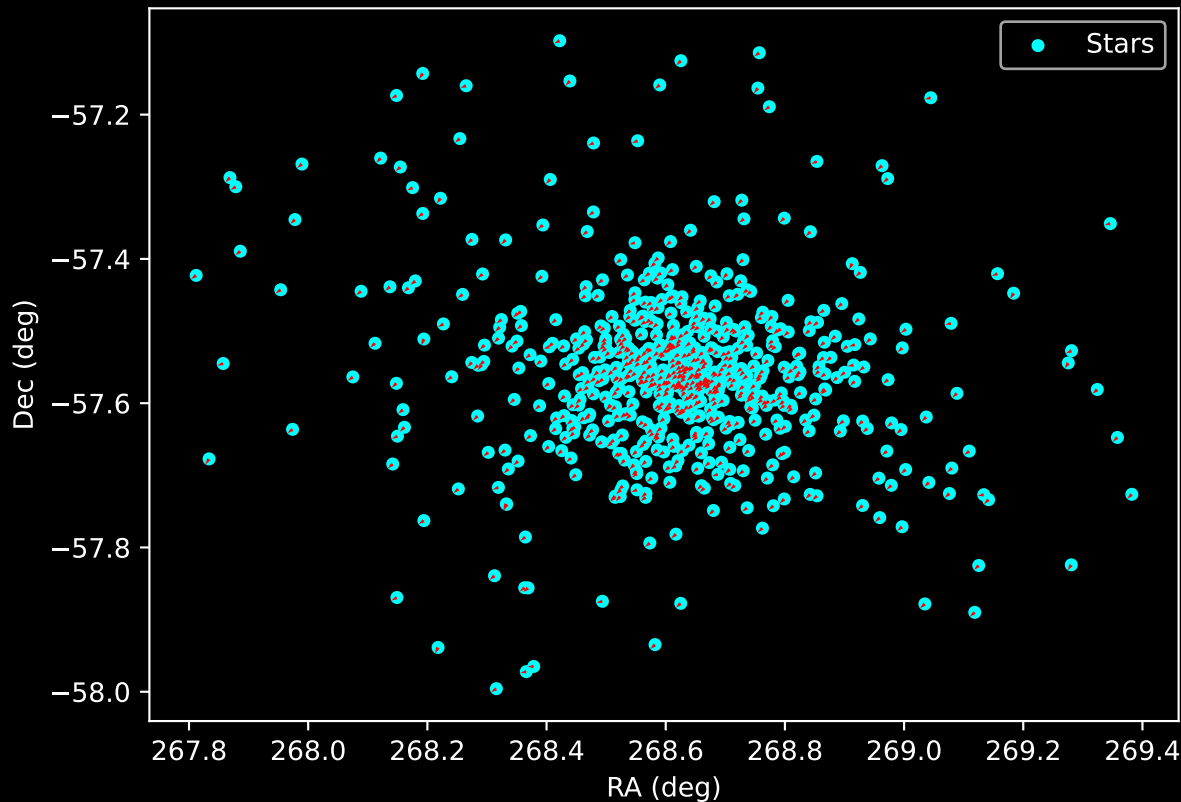
Gaia Cluster: [Trumpler_19] Proper Motion Vectors for Gaia Star Field (n= 649)
