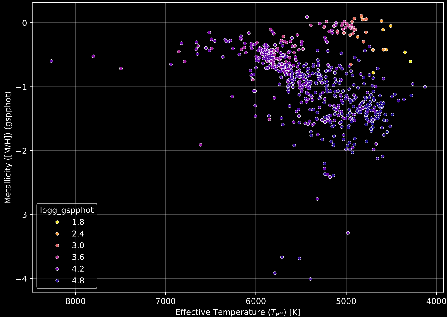
Gaia Cluster: [Trumpler_19] Stellar Population Parameters (n= 649)
