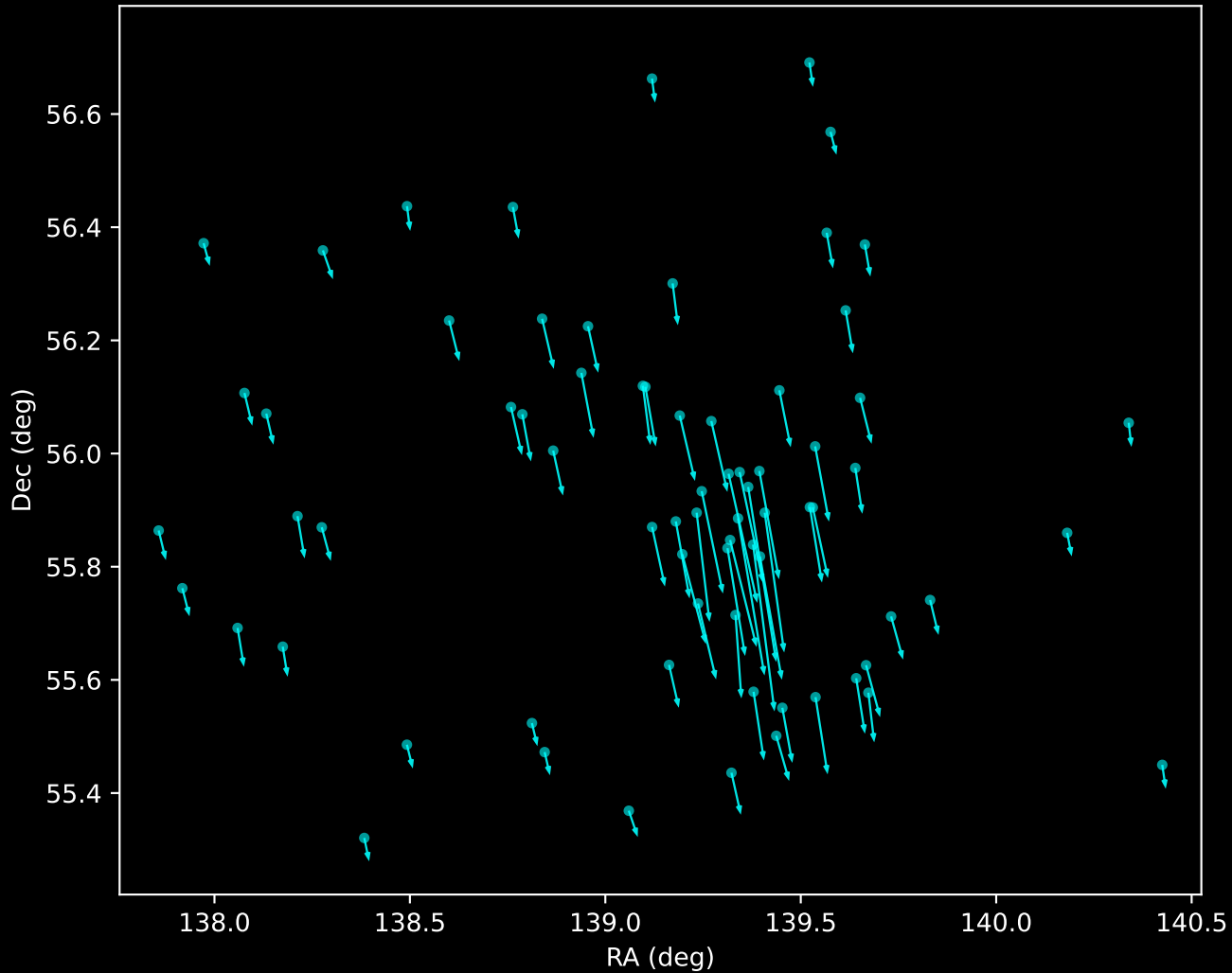
Gaia DR3 Noise Stream Proper Motion Vectors (n=72)
