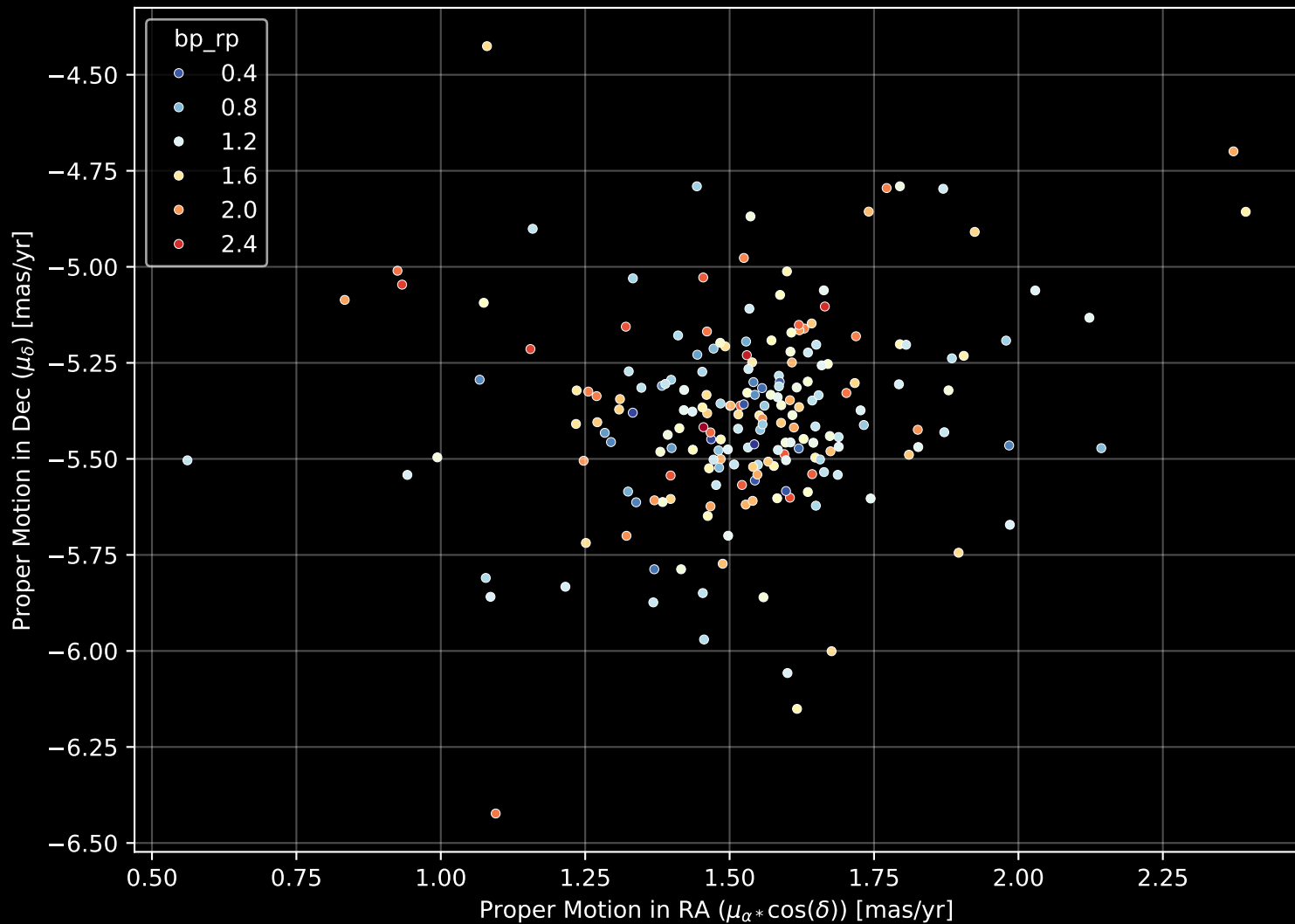
Gaia Cluster: [Trumpler_2] Proper Motion Diagram (n= 204)
