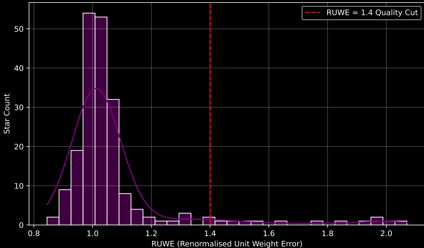
Gaia Cluster: [Trumpler_2] RUWE Distribution (n= 202)
