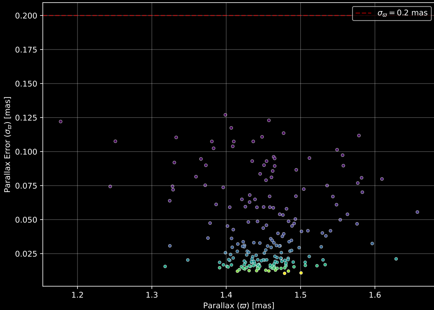
Gaia Cluster: [Trumpler_2] Parallax Quality (n= 204)
