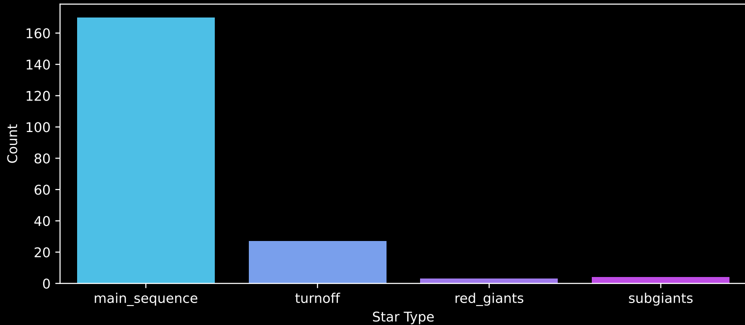
Gaia Cluster: [Trumpler_2] Count plot of Star Type
