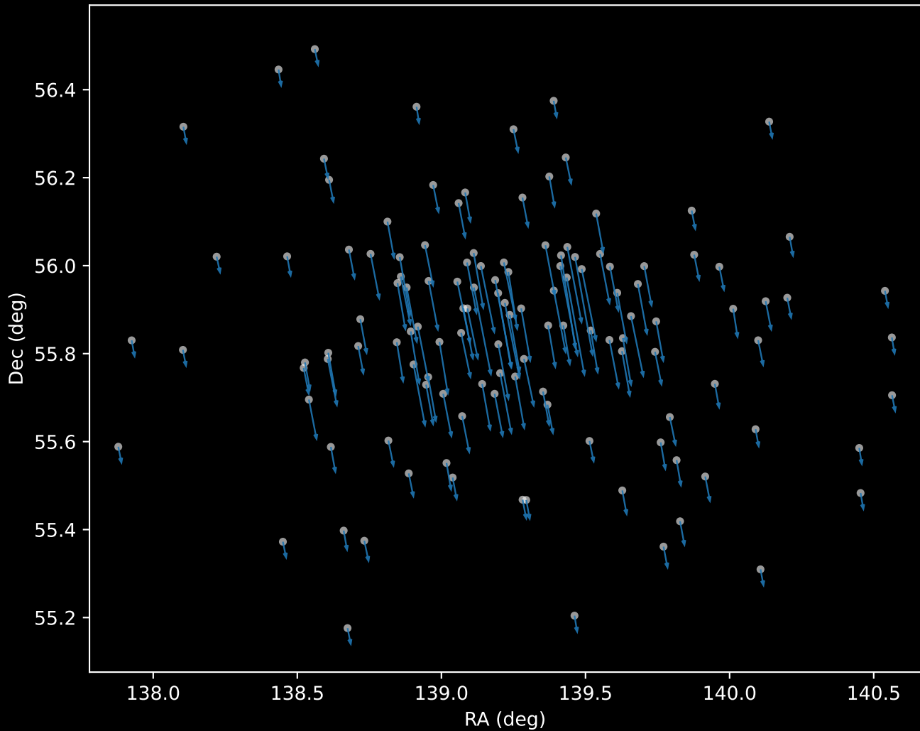
Gaia DR3 Cluster 0 Proper Motion Vectors (n=127)
