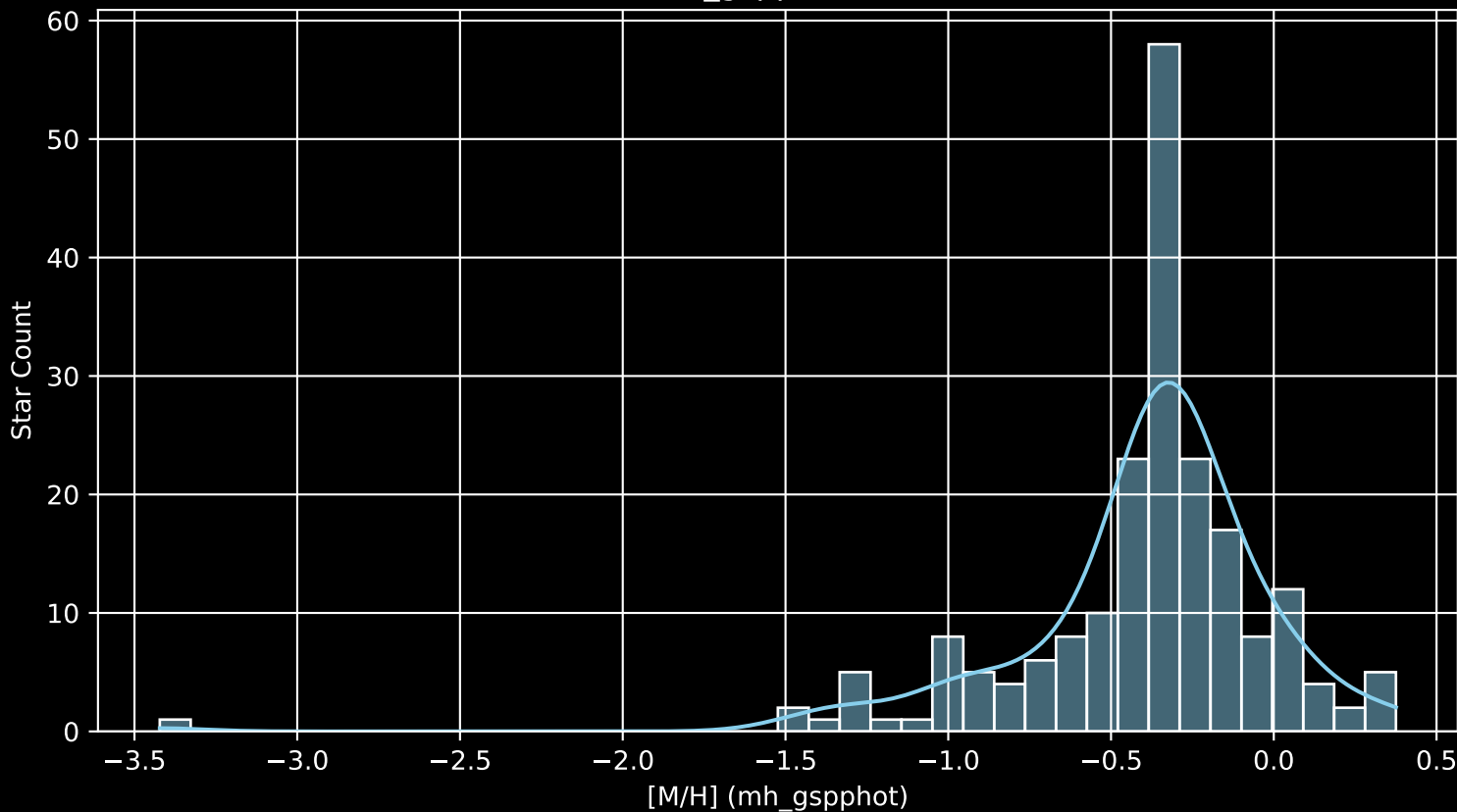
Gaia Cluster: [Trumpler_2 [M/H] (mh_gspphot) (n= 204)
