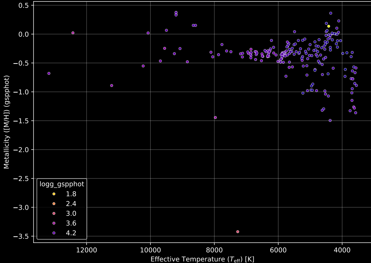
Gaia Cluster: [Trumpler_2] Stellar Population Parameters (n= 204)
