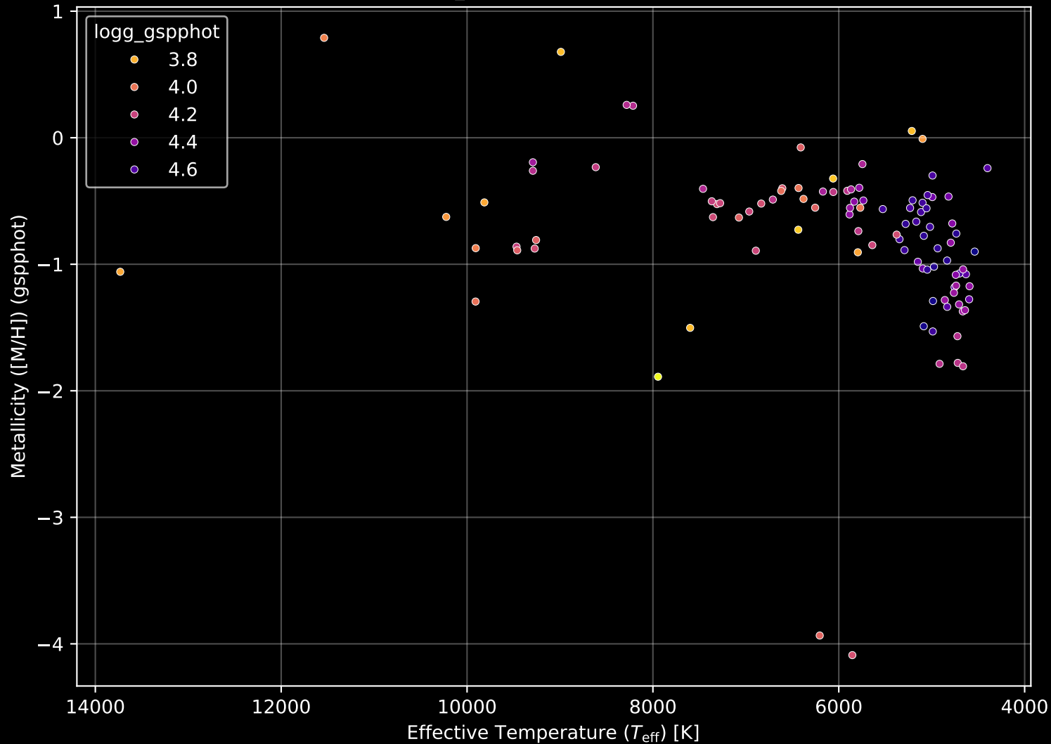
Gaia Cluster: [Trumpler_21] Stellar Population Parameters (n= 103)
