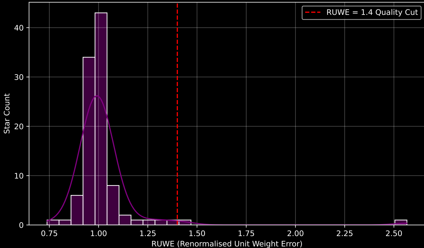
Gaia Cluster: [Trumpler_21] RUWE Distribution (n= 101)
