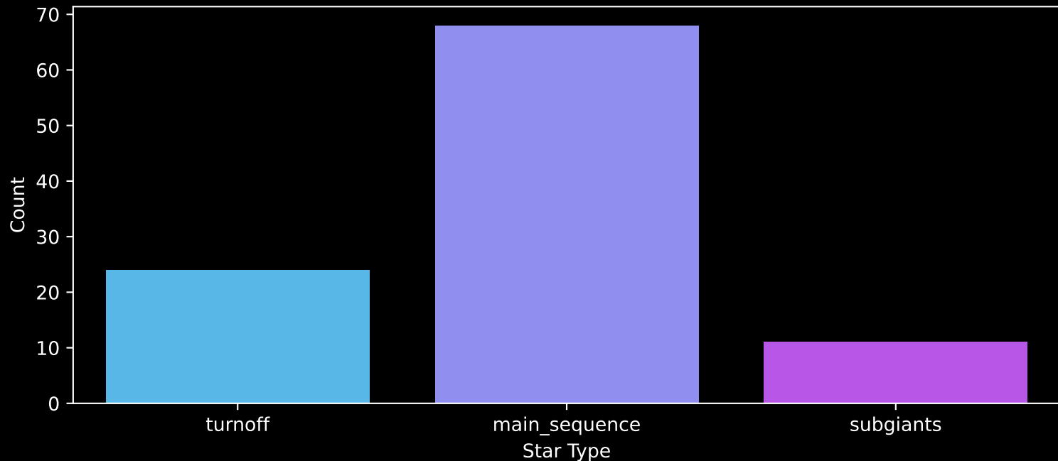
Gaia Cluster: [Trumpler_21] Count plot of Star Type
