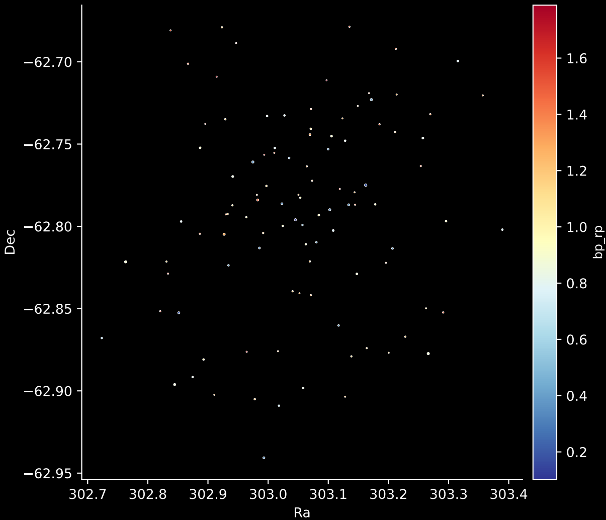
Gaia Cluster: [Trumpler_21] Stars: 103
