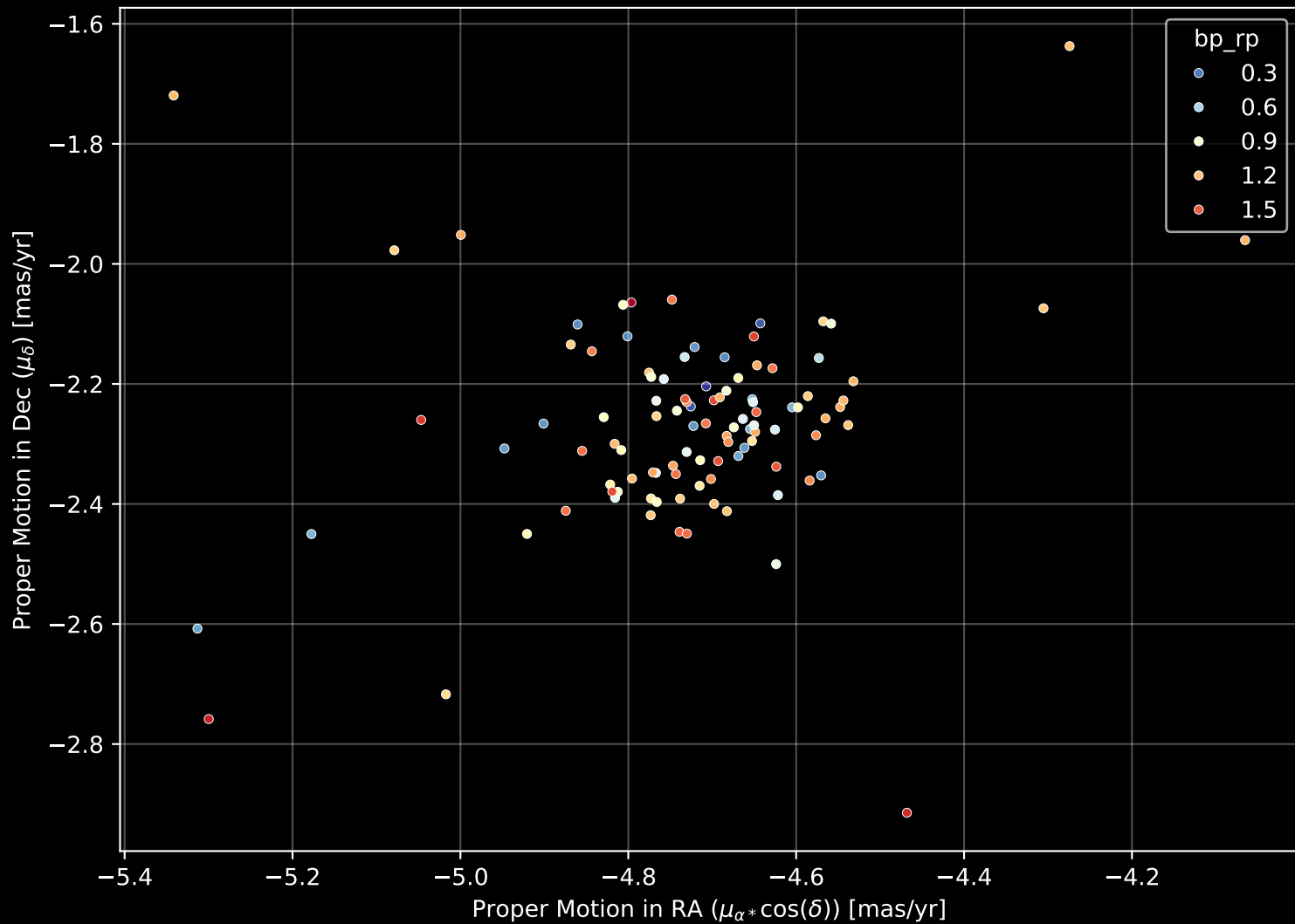
Gaia Cluster: [Trumpler_21] Proper Motion Diagram (n= 103)
