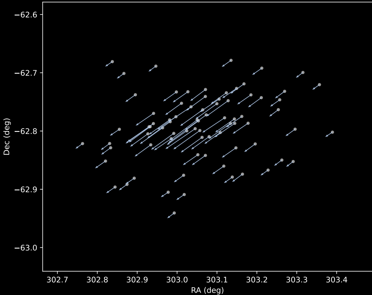
Gaia DR3 Cluster 1 Proper Motion Vectors (n=77)
