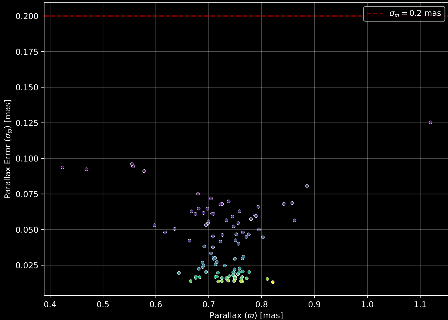
Gaia Cluster: [Trumpler_21] Parallax Quality (n= 103)
