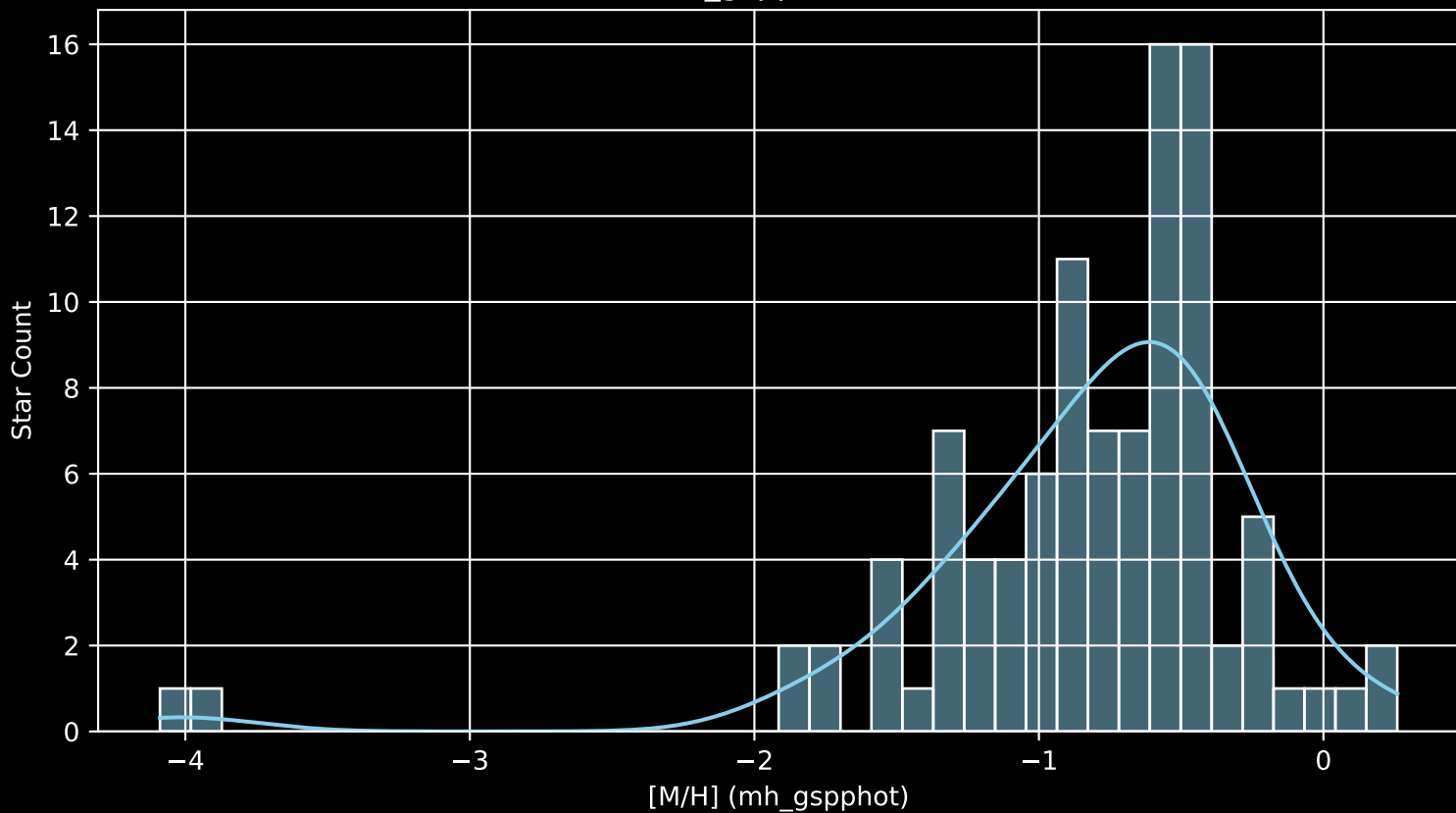
Gaia Cluster: [Trumpler_21 [M/H] (mh_gspphot) (n= 101)
