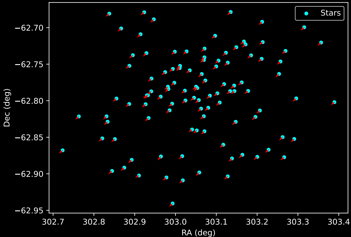
Gaia Cluster: [Trumpler_21] Proper Motion Vectors for Gaia Star Field (n= 103)
