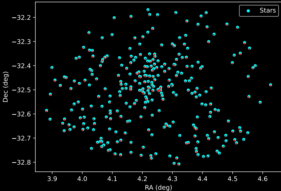
Gaia Cluster: [Trumpler_28] Proper Motion Vectors for Gaia Star Field (n= 294)
