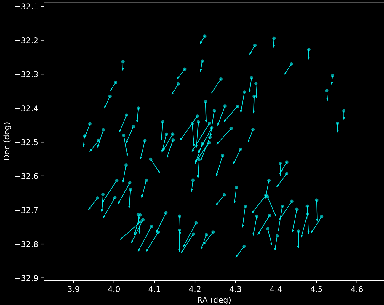
Gaia DR3 Noise Stream Proper Motion Vectors (n=95)
