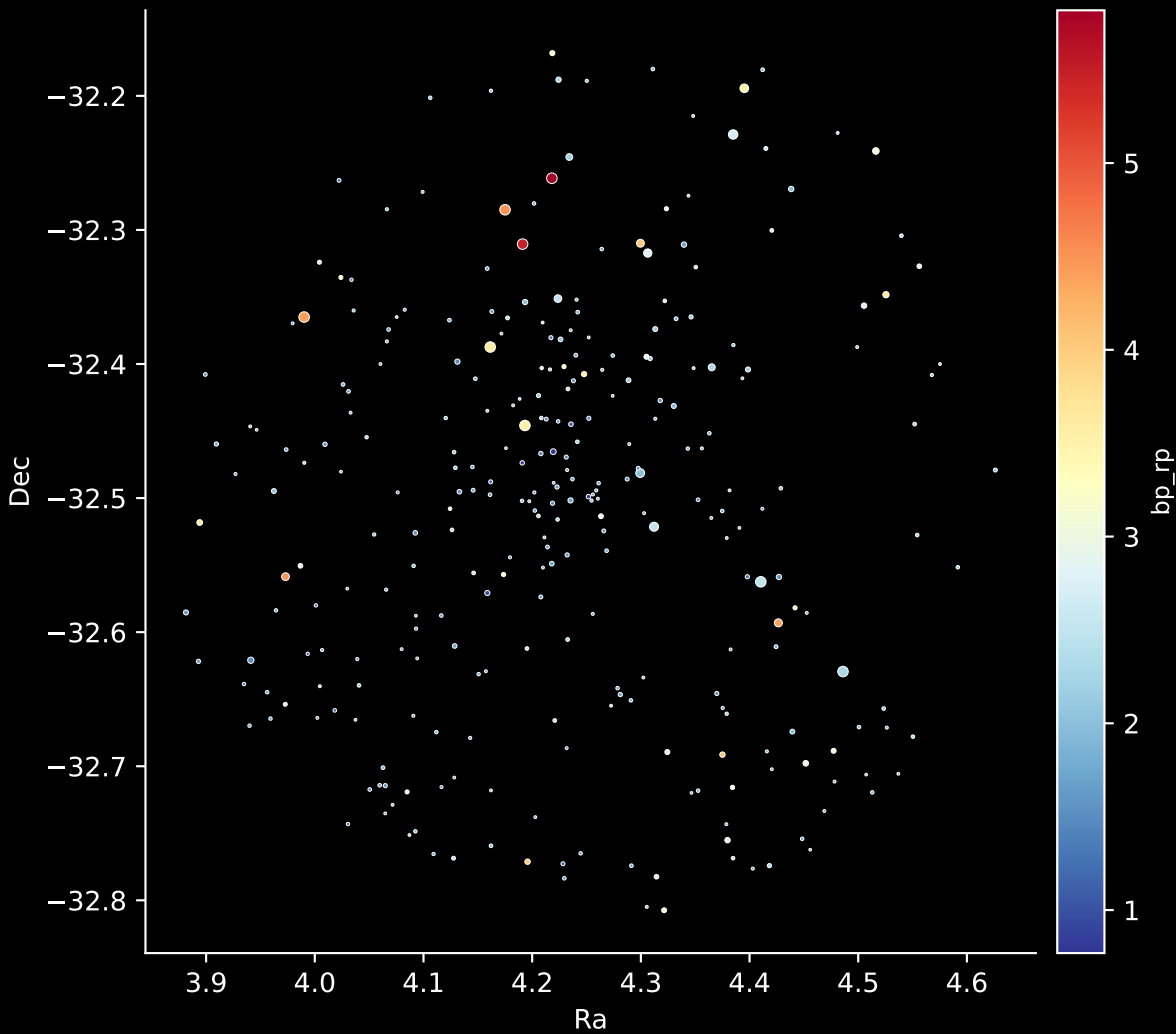
Gaia Cluster: [Trumpler_28] Stars: 294
