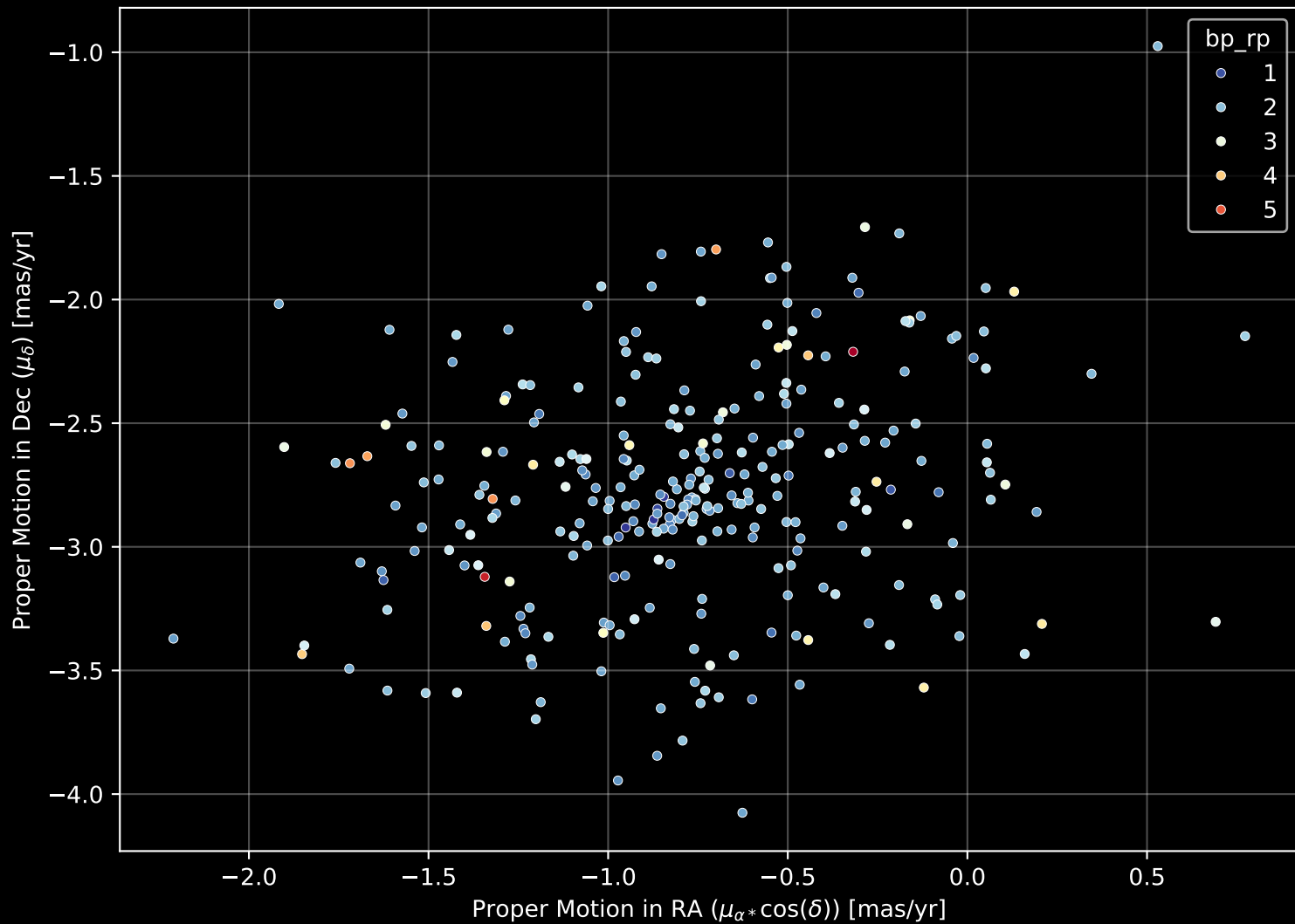
Gaia Cluster: [Trumpler_28] Proper Motion Diagram (n= 294)
