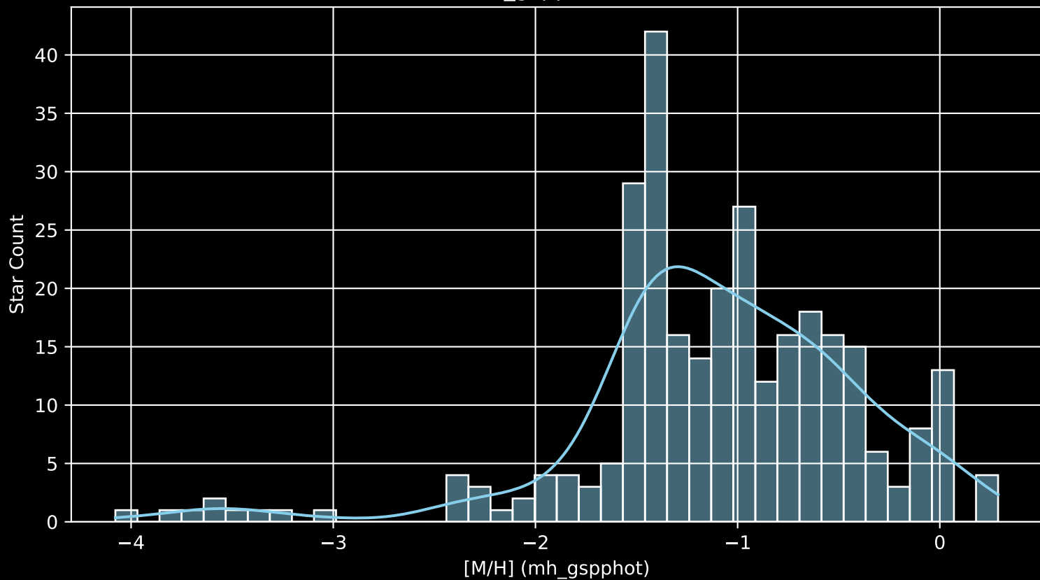
Gaia Cluster: [Trumpler_28 [M/H] (mh_gspphot) (n= 294)
