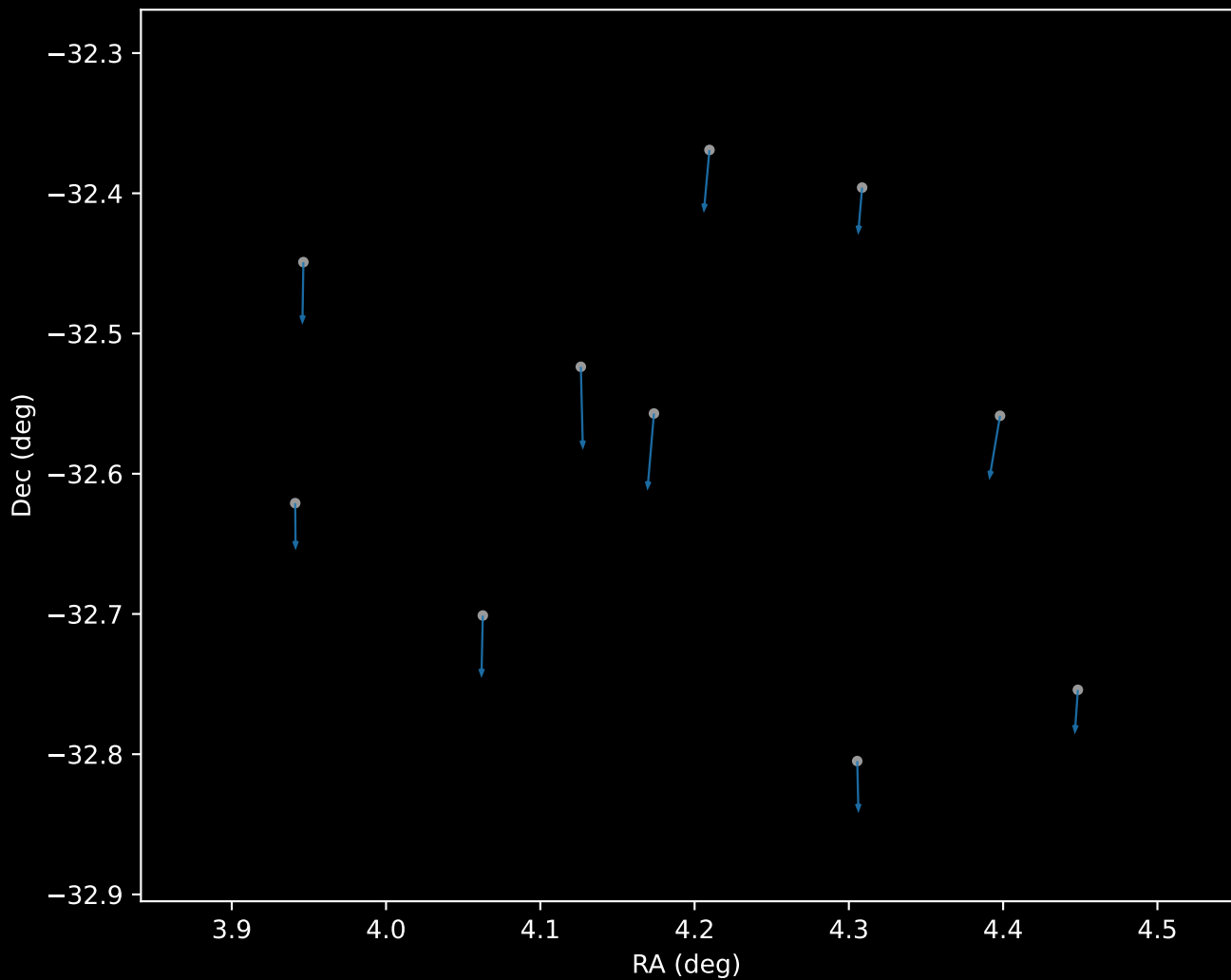
Gaia DR3 Cluster 0 Proper Motion Vectors (n=10)
