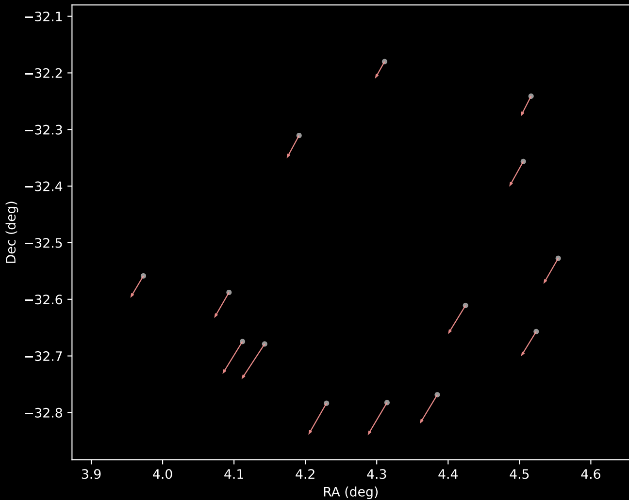
Gaia DR3 Cluster 7 Proper Motion Vectors (n=14)
