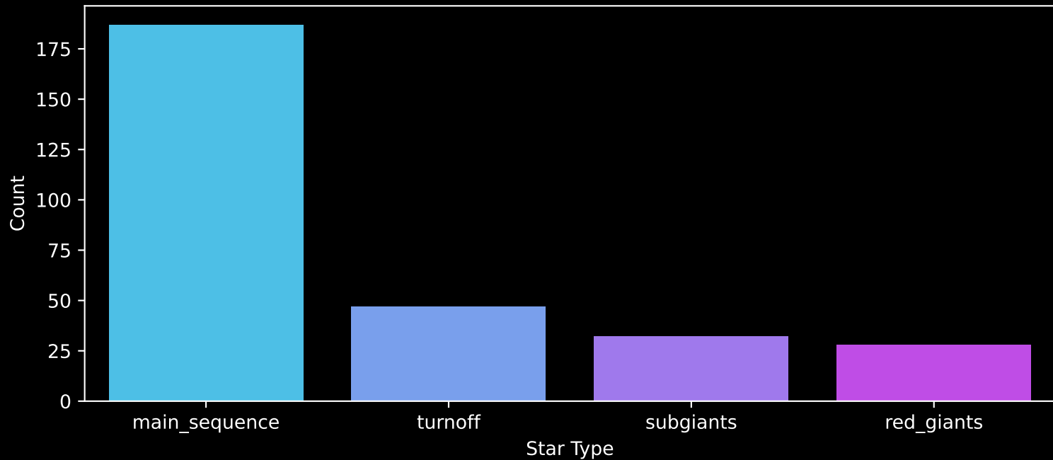
Gaia Cluster: [Trumpler_28] Count plot of Star Type
