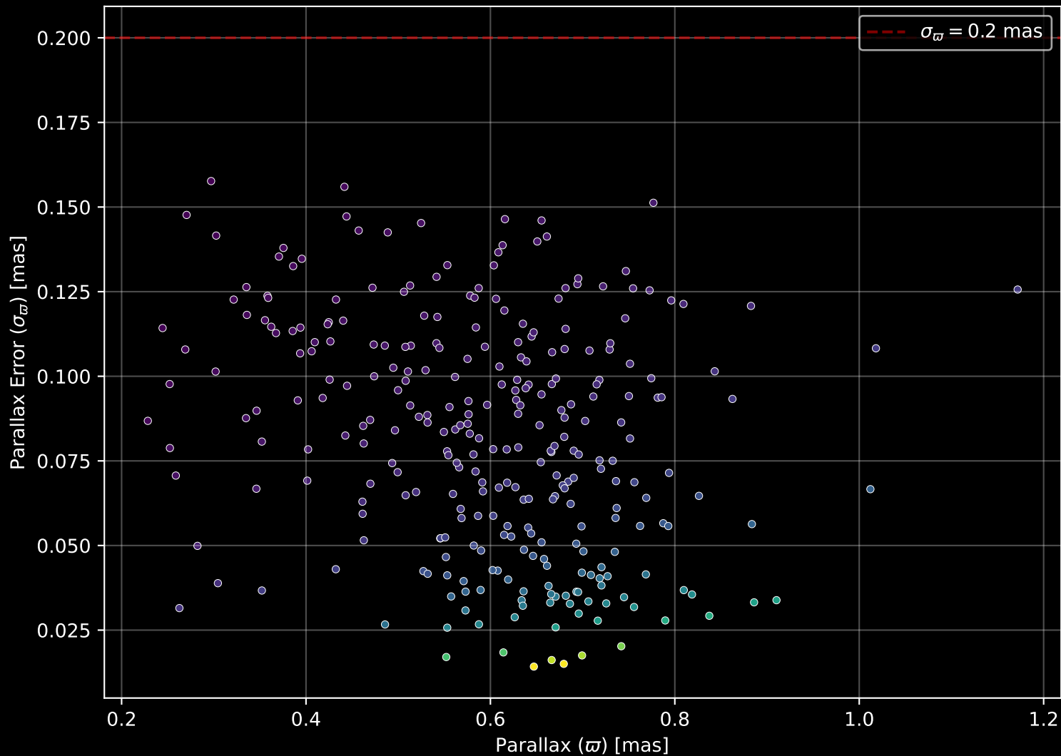
Gaia Cluster: [Trumpler_28] Parallax Quality (n= 294)
