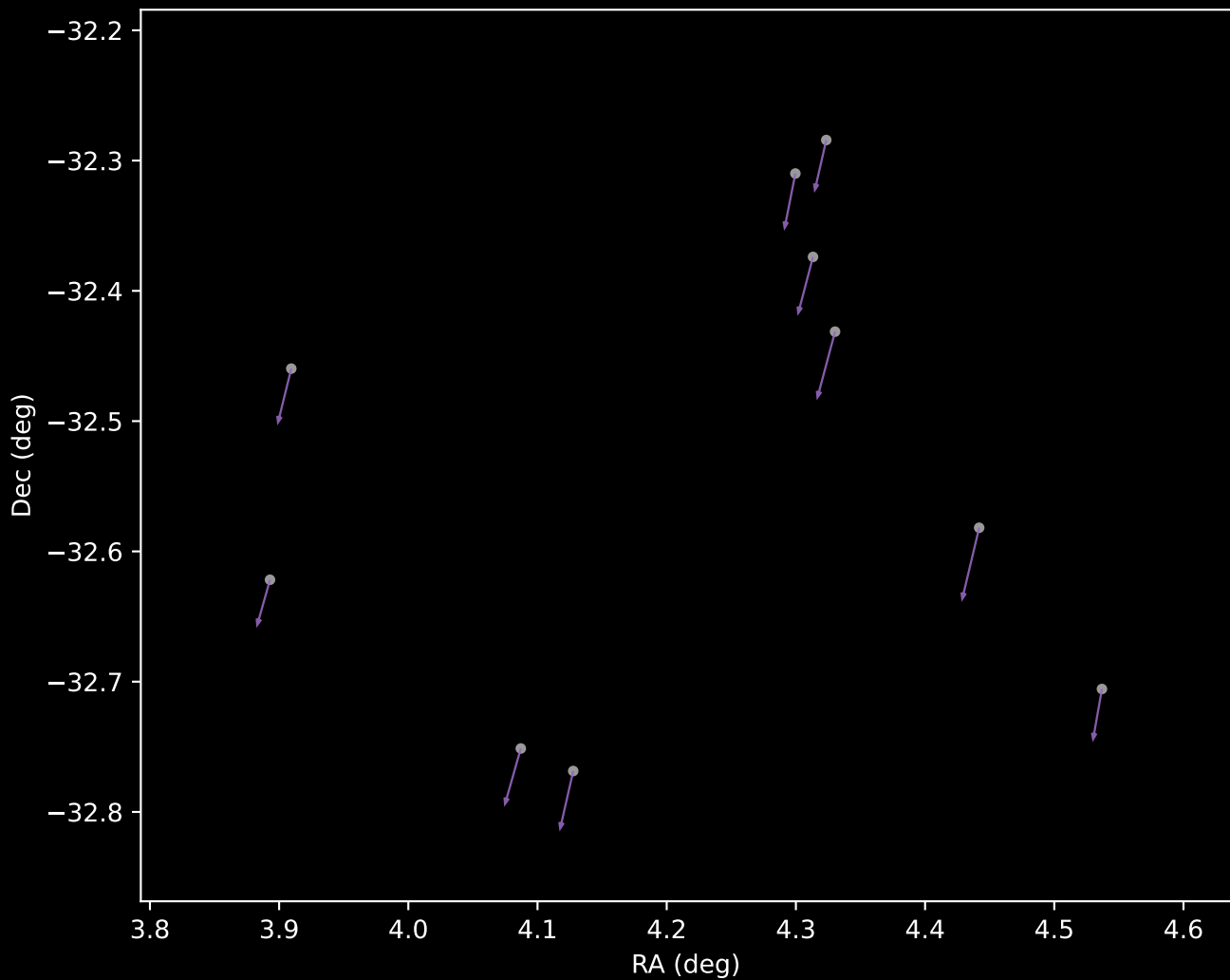
Gaia DR3 Cluster 8 Proper Motion Vectors (n=10)
