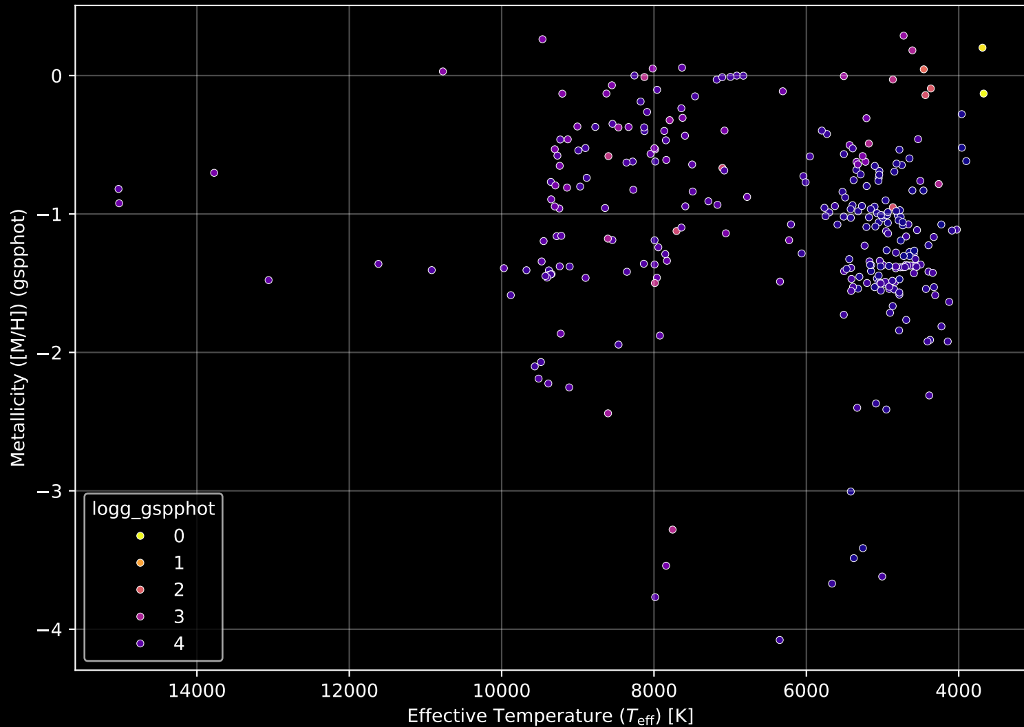
Gaia Cluster: [Trumpler_28] Stellar Population Parameters (n= 294)
