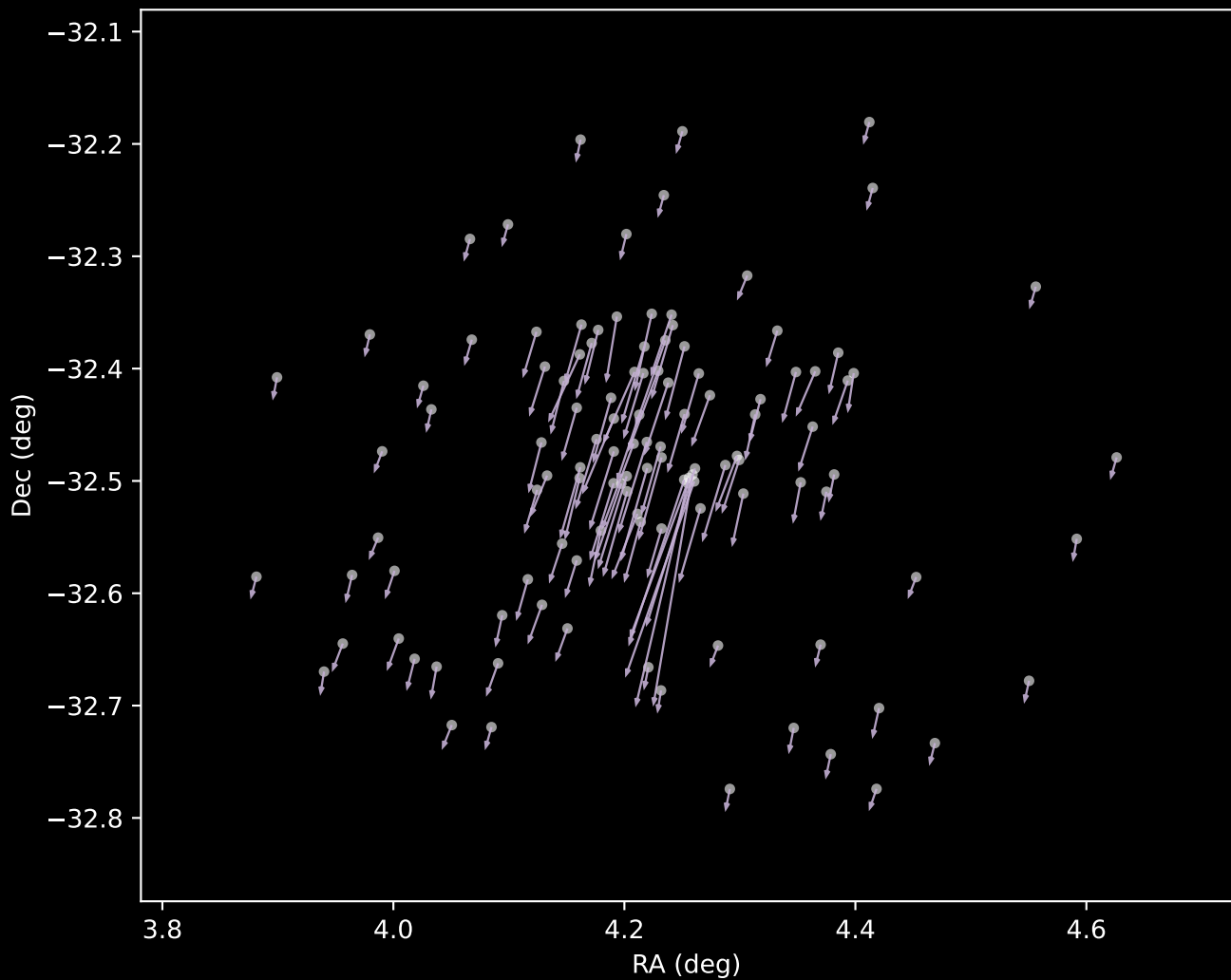
Gaia DR3 Cluster 9 Proper Motion Vectors (n=116)
