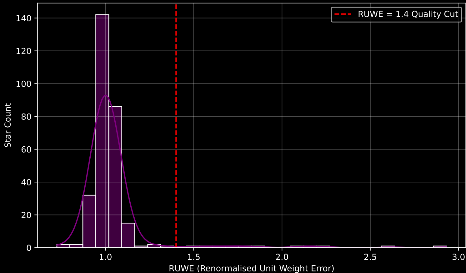
Gaia Cluster: [Trumpler_28] RUWE Distribution (n= 294)
