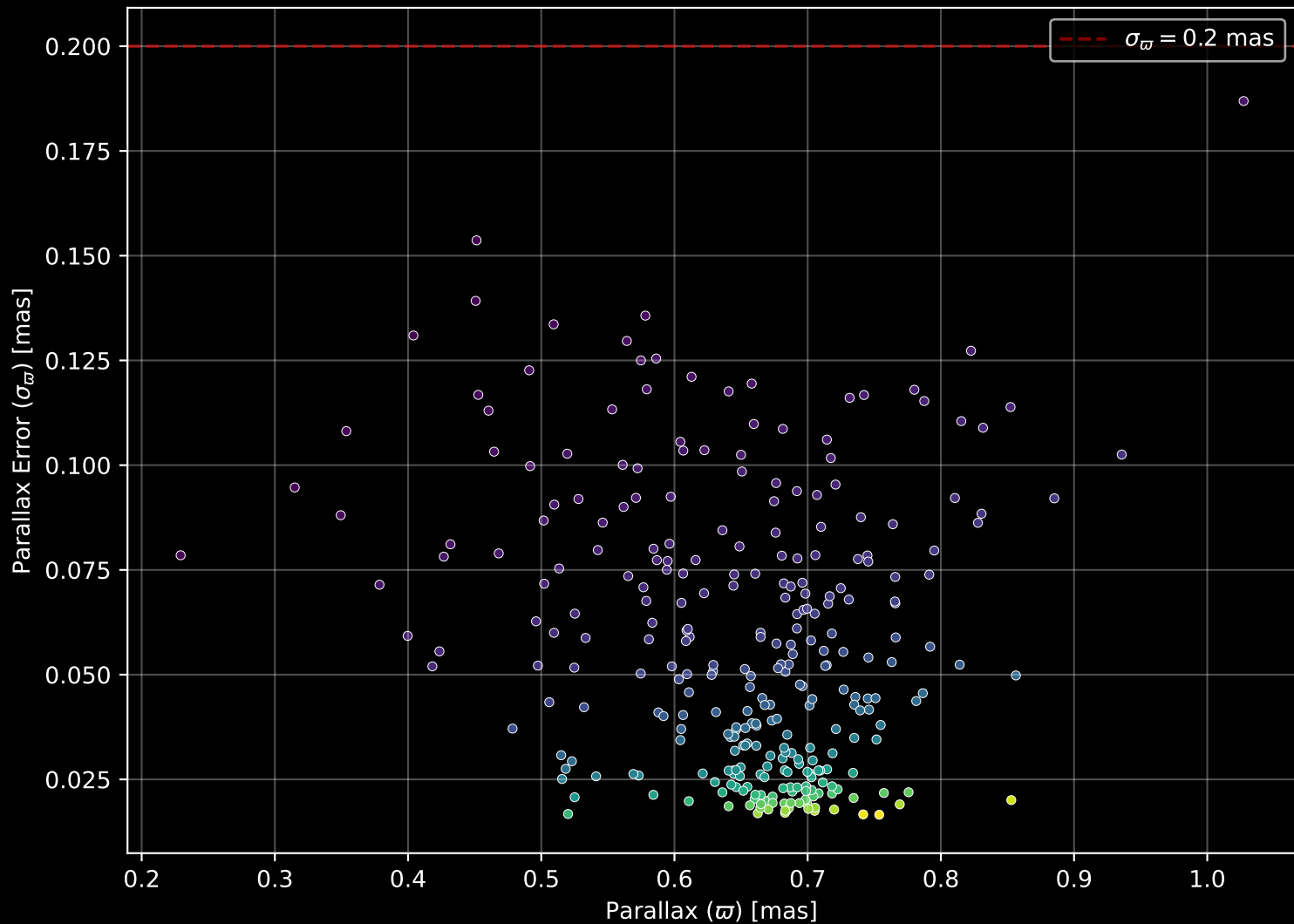
Gaia Cluster: [Trumpler_29] Parallax Quality (n= 298)
