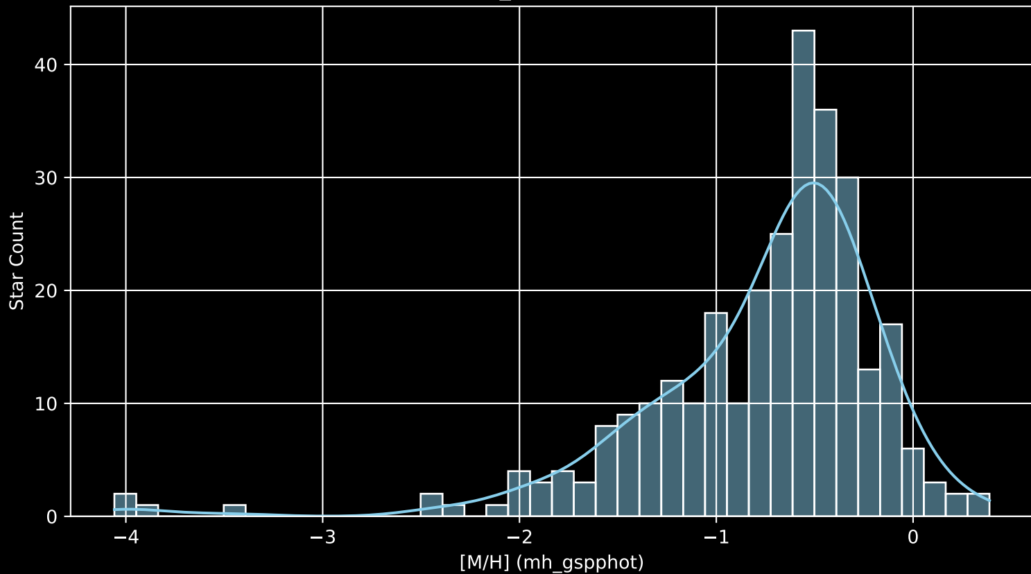
Gaia Cluster: [Trumpler_29 [M/H] (mh_gspphot) (n= 296)
