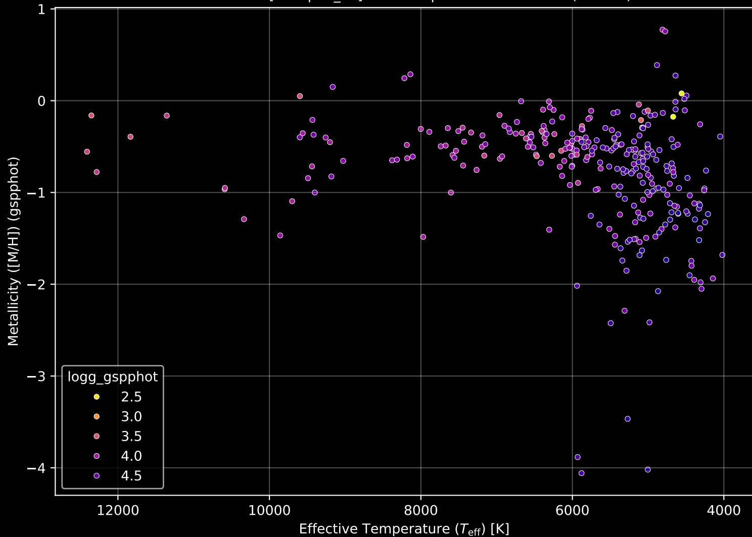
Gaia Cluster: [Trumpler_29] Stellar Population Parameters (n= 298)
