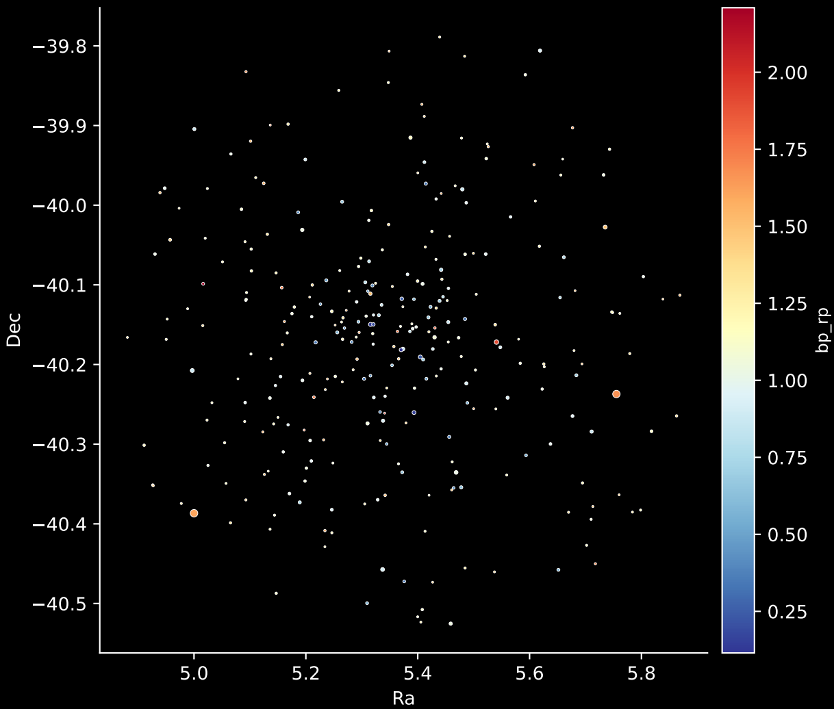
Gaia Cluster: [Trumpler_29] Stars: 298
