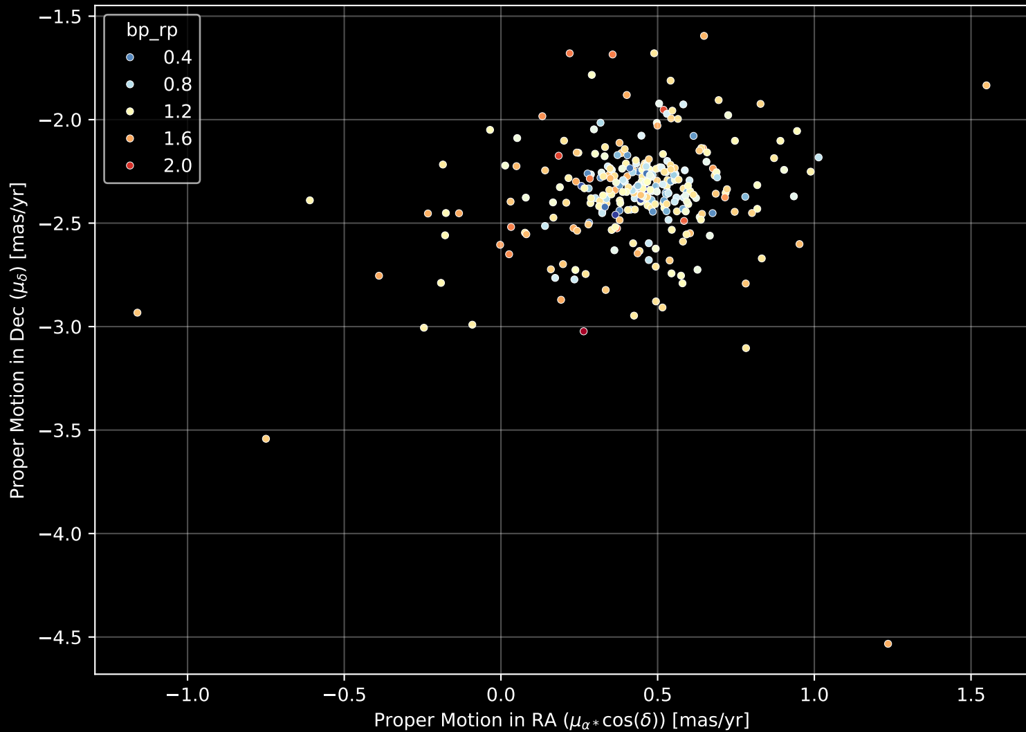
Gaia Cluster: [Trumpler_29] Proper Motion Diagram (n= 298)
