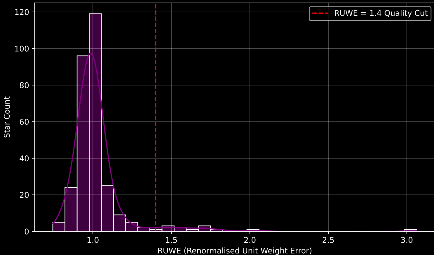
Gaia Cluster: [Trumpler_29] RUWE Distribution (n= 298)
