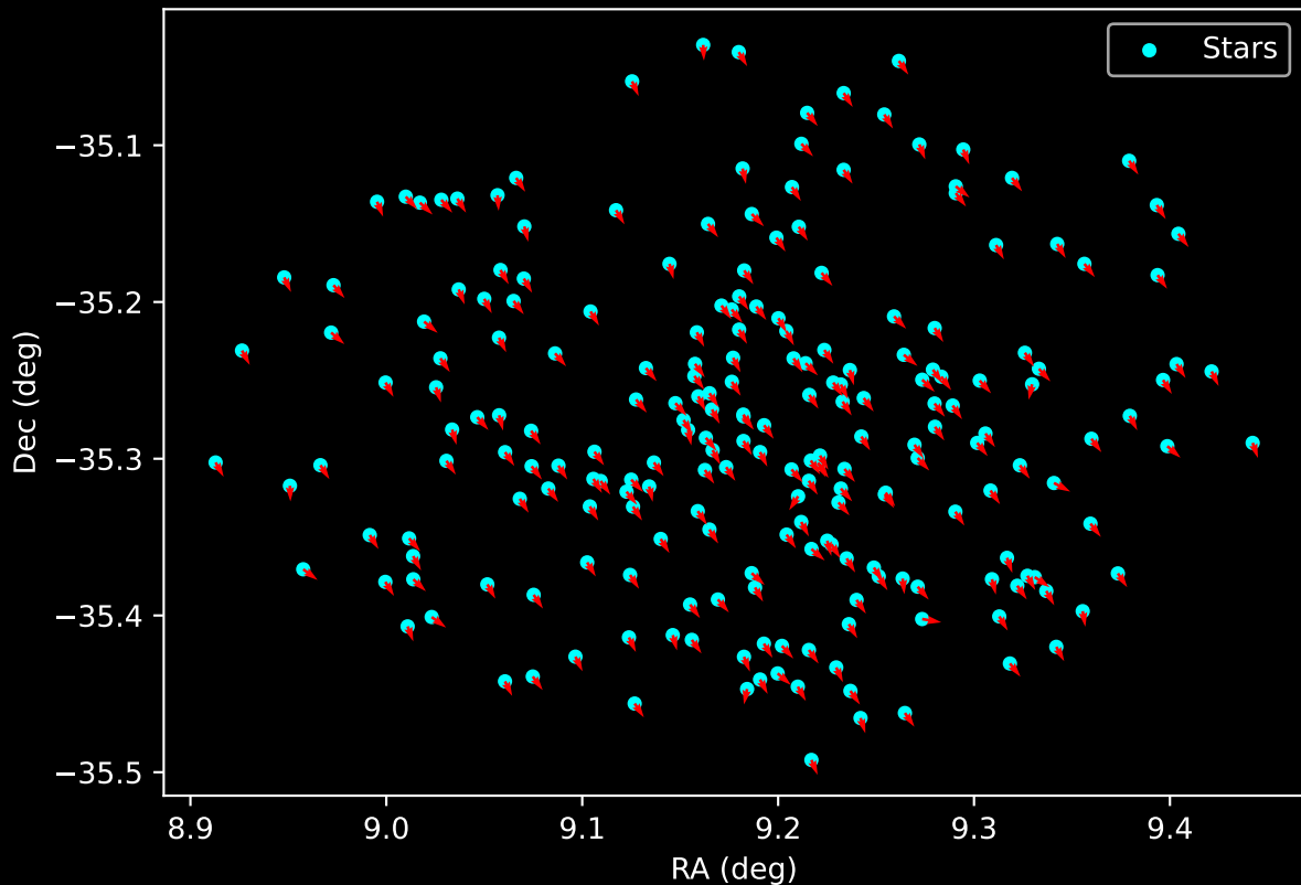
Gaia Cluster: [Trumpler_30] Proper Motion Vectors for Gaia Star Field (n= 220)
