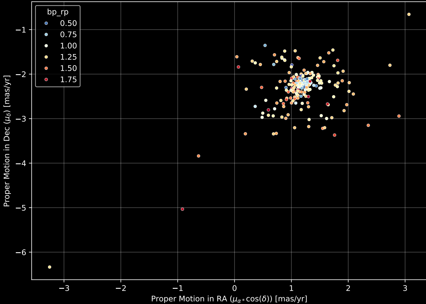
Gaia Cluster: [Trumpler_30] Proper Motion Diagram (n= 220)
