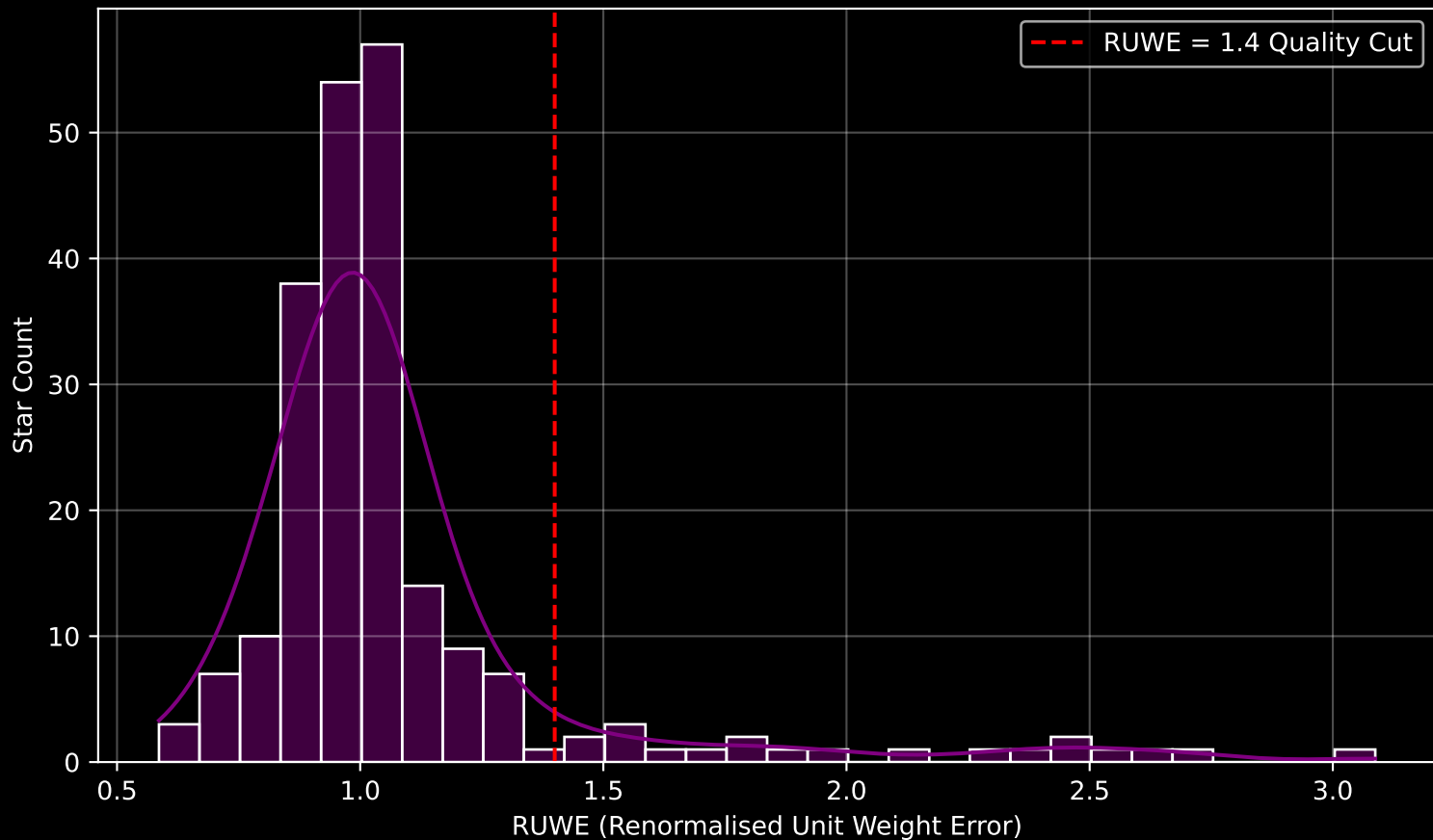
Gaia Cluster: [Trumpler_30] RUWE Distribution (n= 220)
