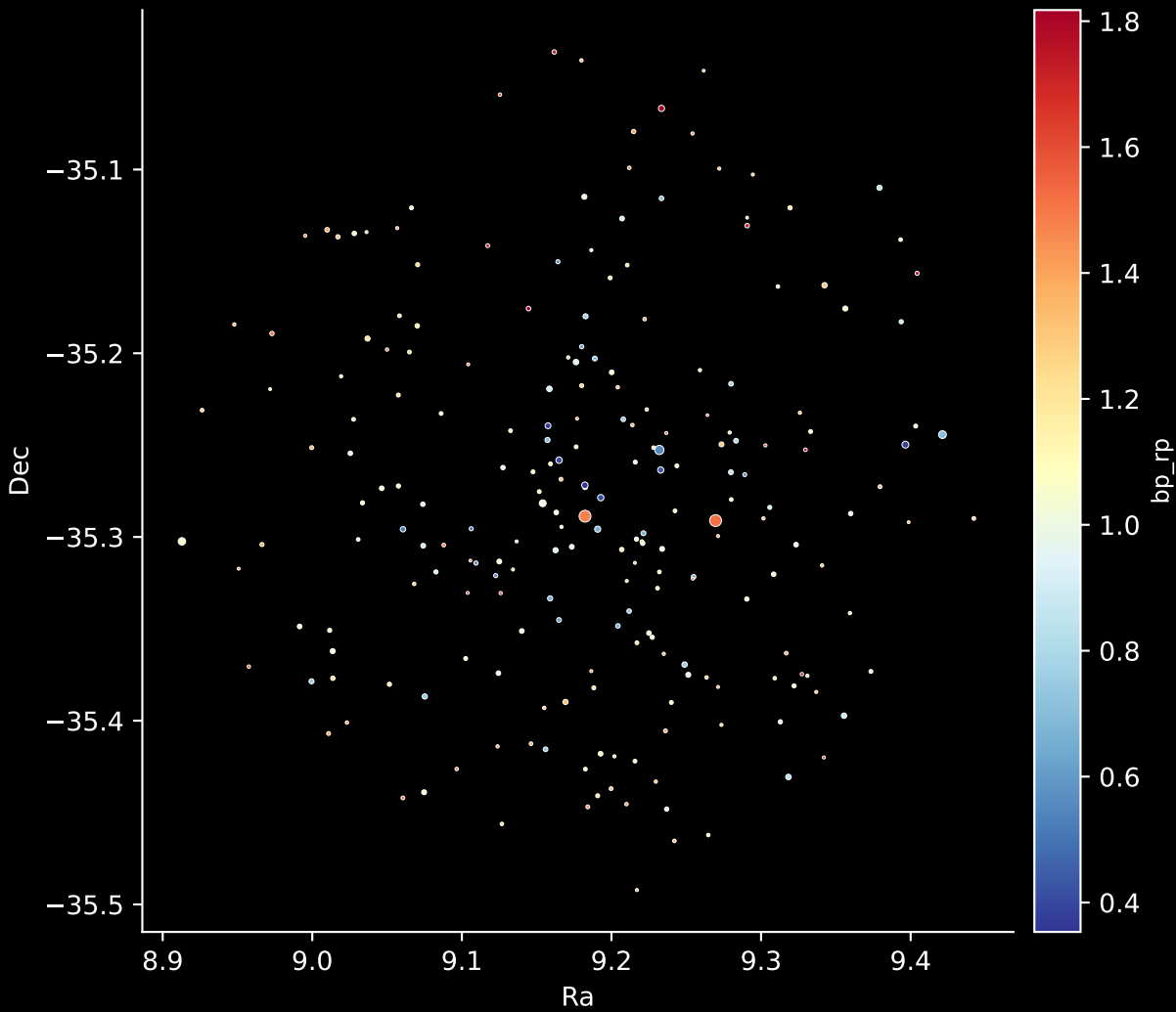
Gaia Cluster: [Trumpler_30] Stars: 220
