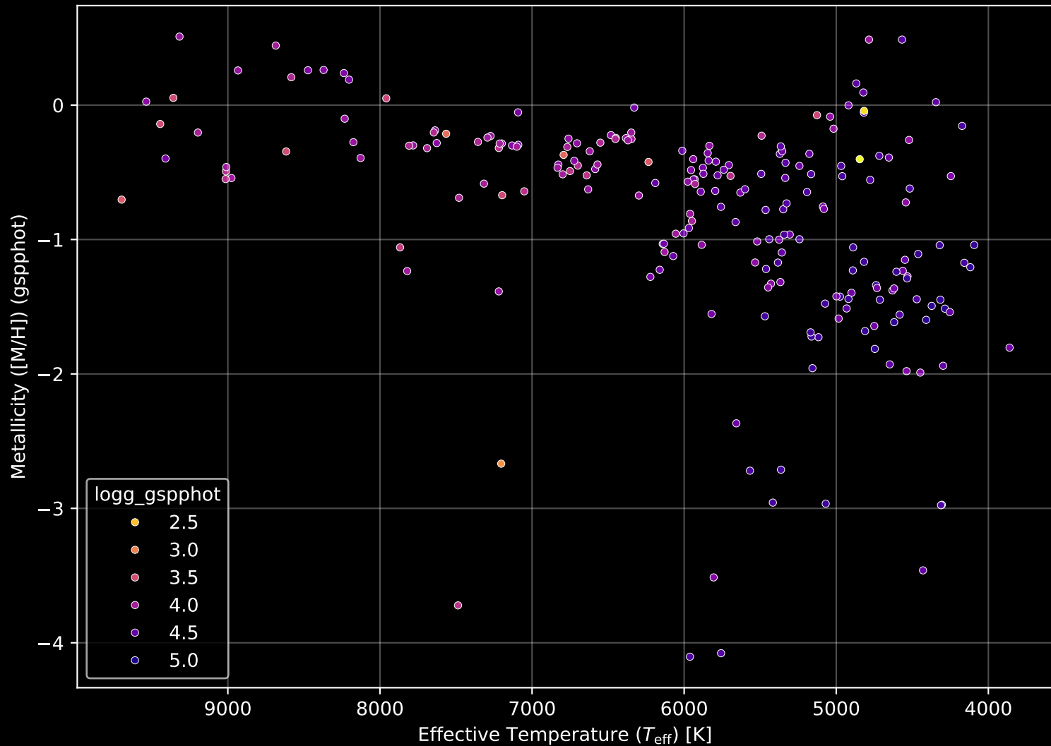
Gaia Cluster: [Trumpler_30] Stellar Population Parameters (n= 220)
