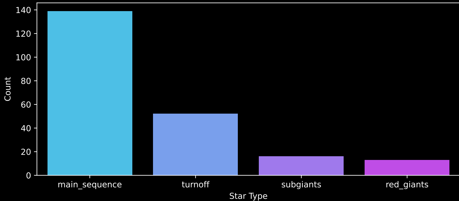
Gaia Cluster: [Trumpler_30] Count plot of Star Type
