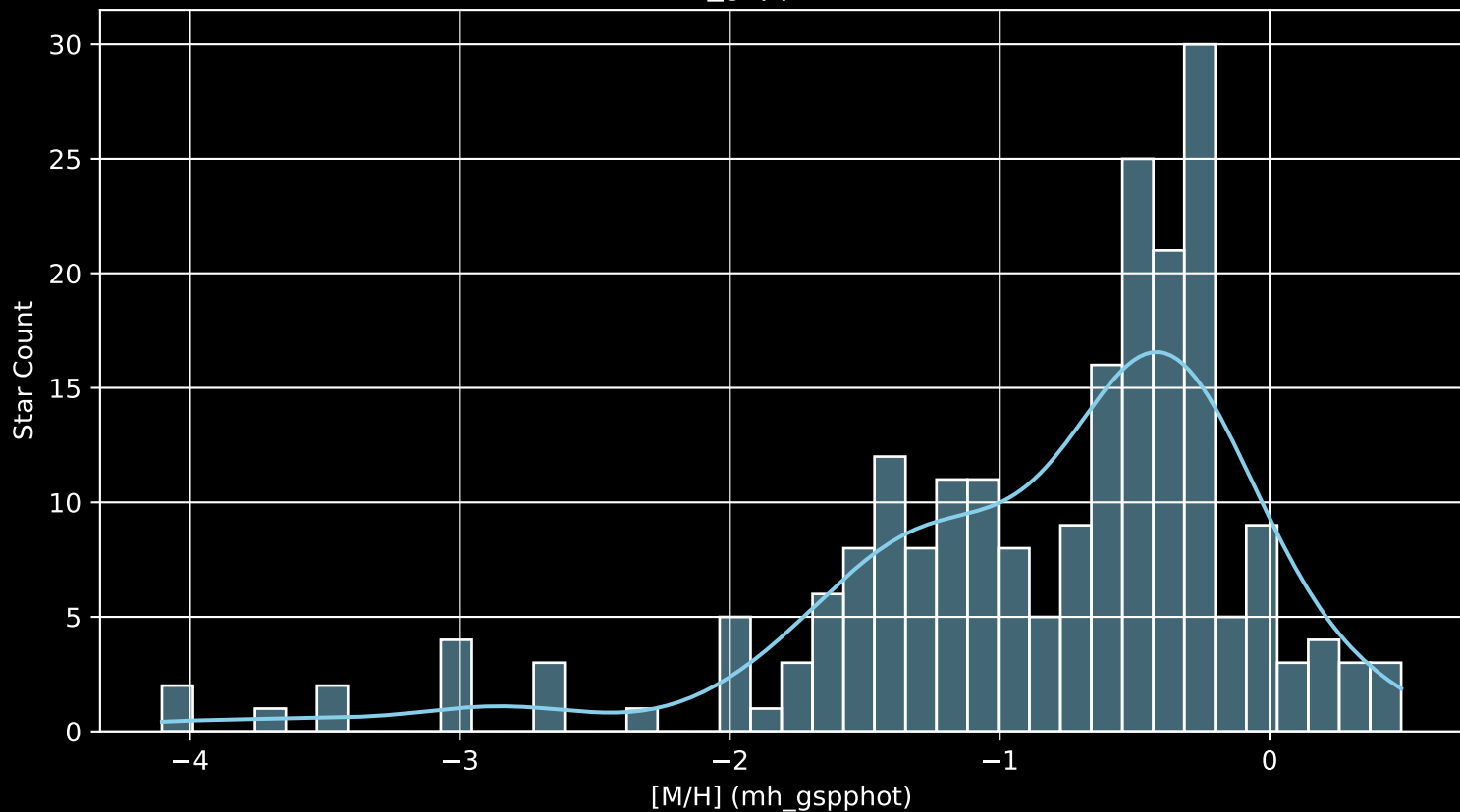
Gaia Cluster: [Trumpler_30 [M/H] (mh_gspphot) (n= 219)
