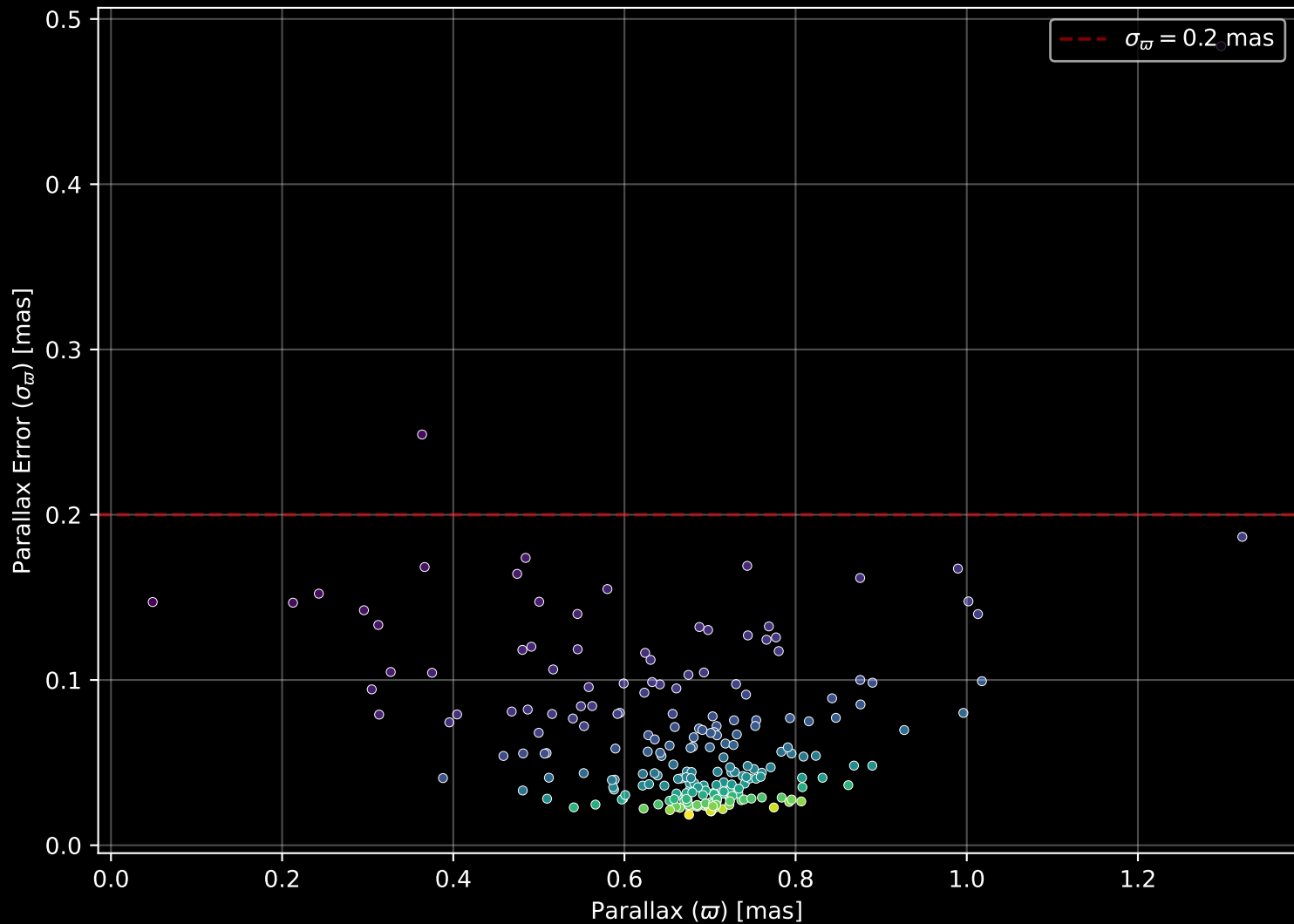
Gaia Cluster: [Trumpler_30] Parallax Quality (n= 220)
