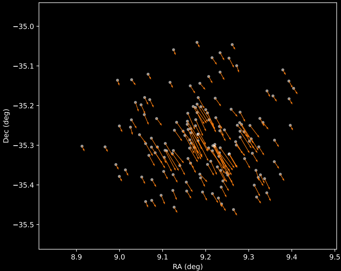
Gaia DR3 Cluster 2 Proper Motion Vectors (n=150)
