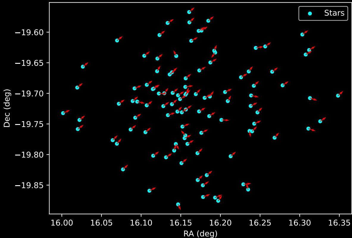
Gaia Cluster: [Trumpler_33] Proper Motion Vectors for Gaia Star Field (n= 104)
