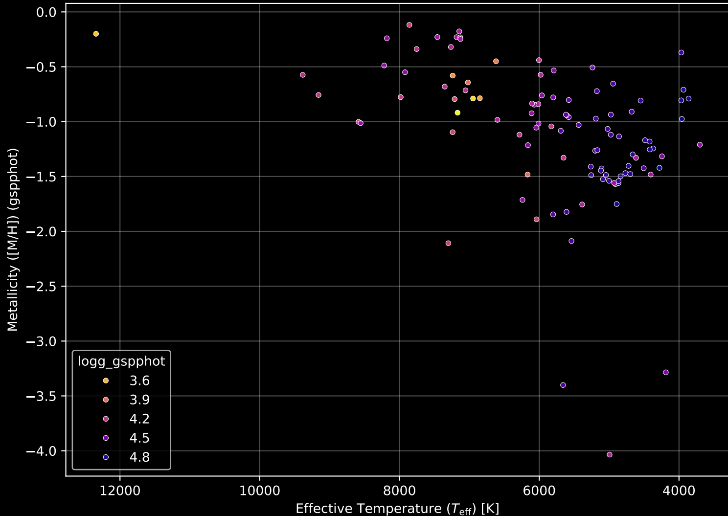
Gaia Cluster: [Trumpler_33] Stellar Population Parameters (n= 104)
