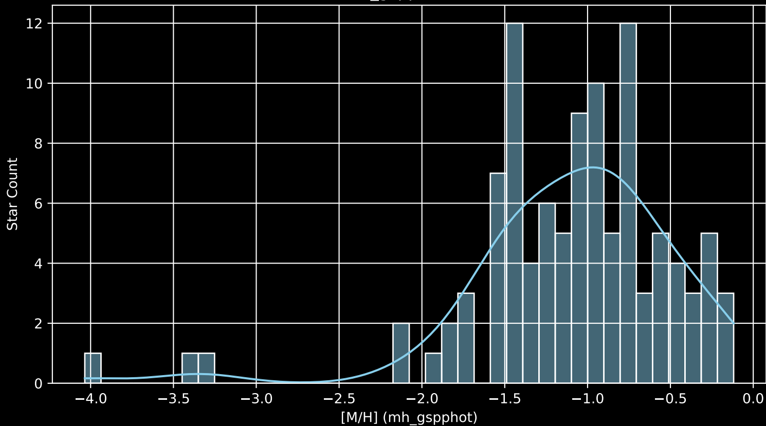
Gaia Cluster: [Trumpler_33 [M/H] (mh_gspphot) (n= 104)
