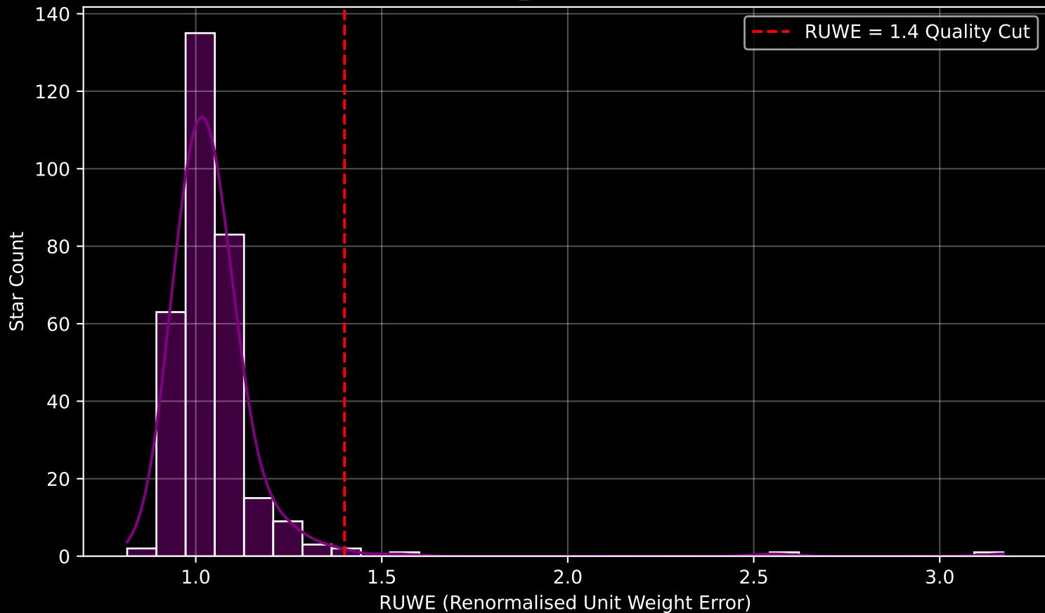
Gaia Cluster: [Trumpler_35] RUWE Distribution (n= 315)
