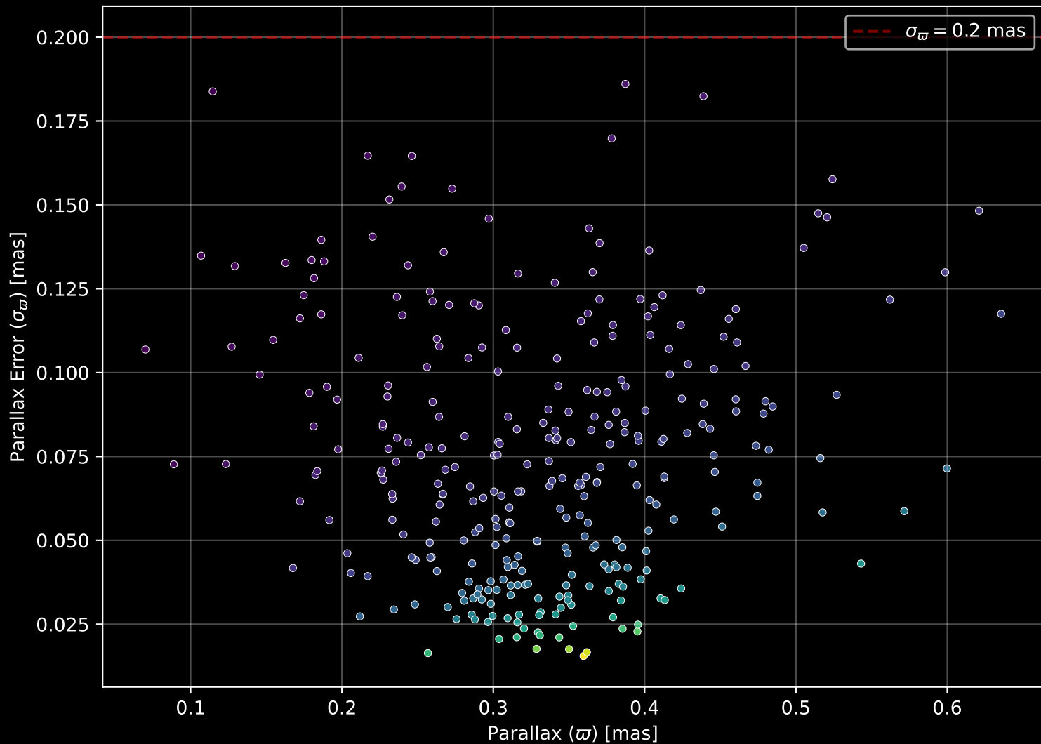
Gaia Cluster: [Trumpler_35] Parallax Quality (n= 315)
