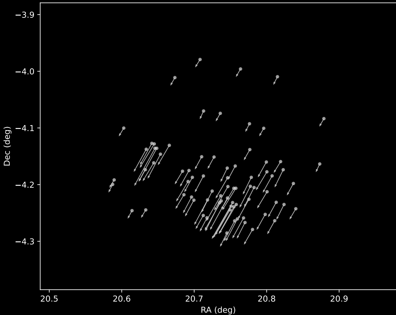
Gaia DR3 Cluster 15 Proper Motion Vectors (n=76)
