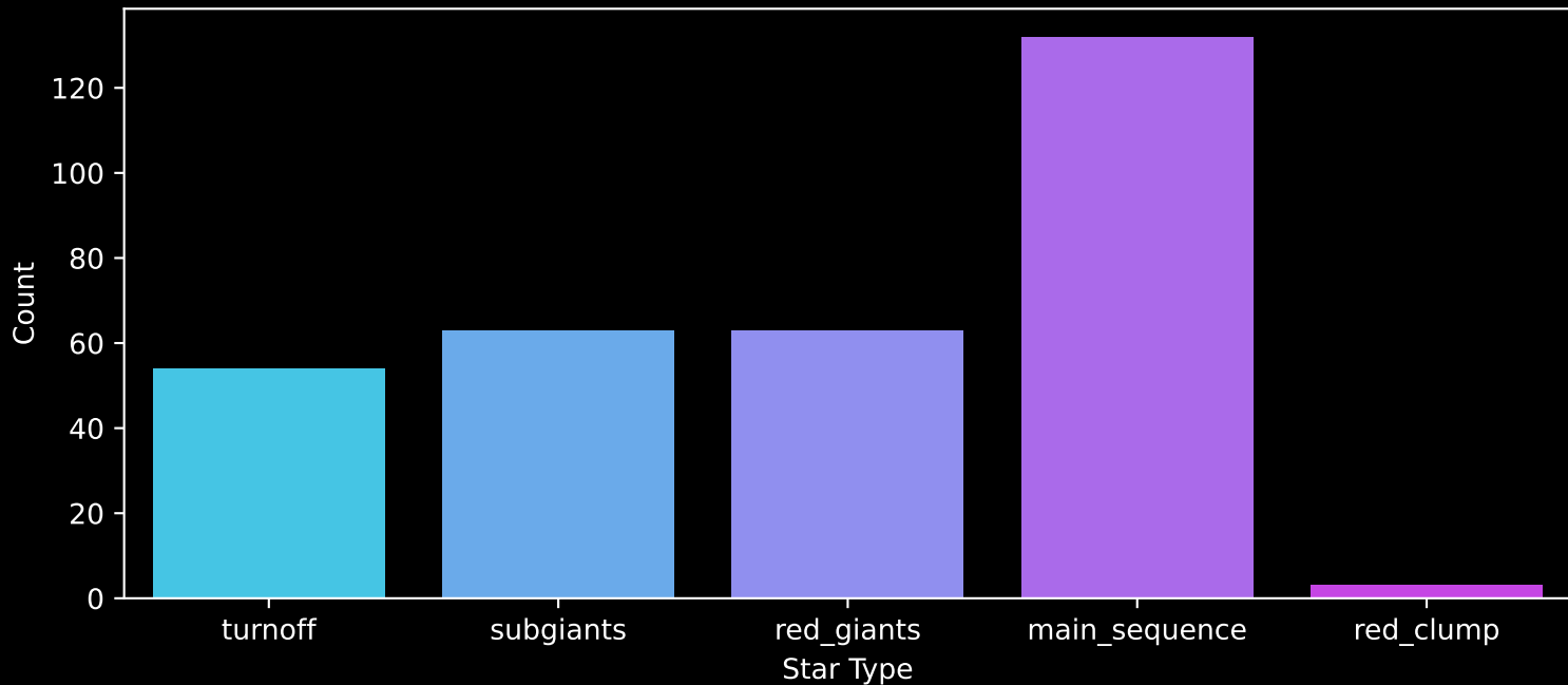
Gaia Cluster: [Trumpler_35] Count plot of Star Type
