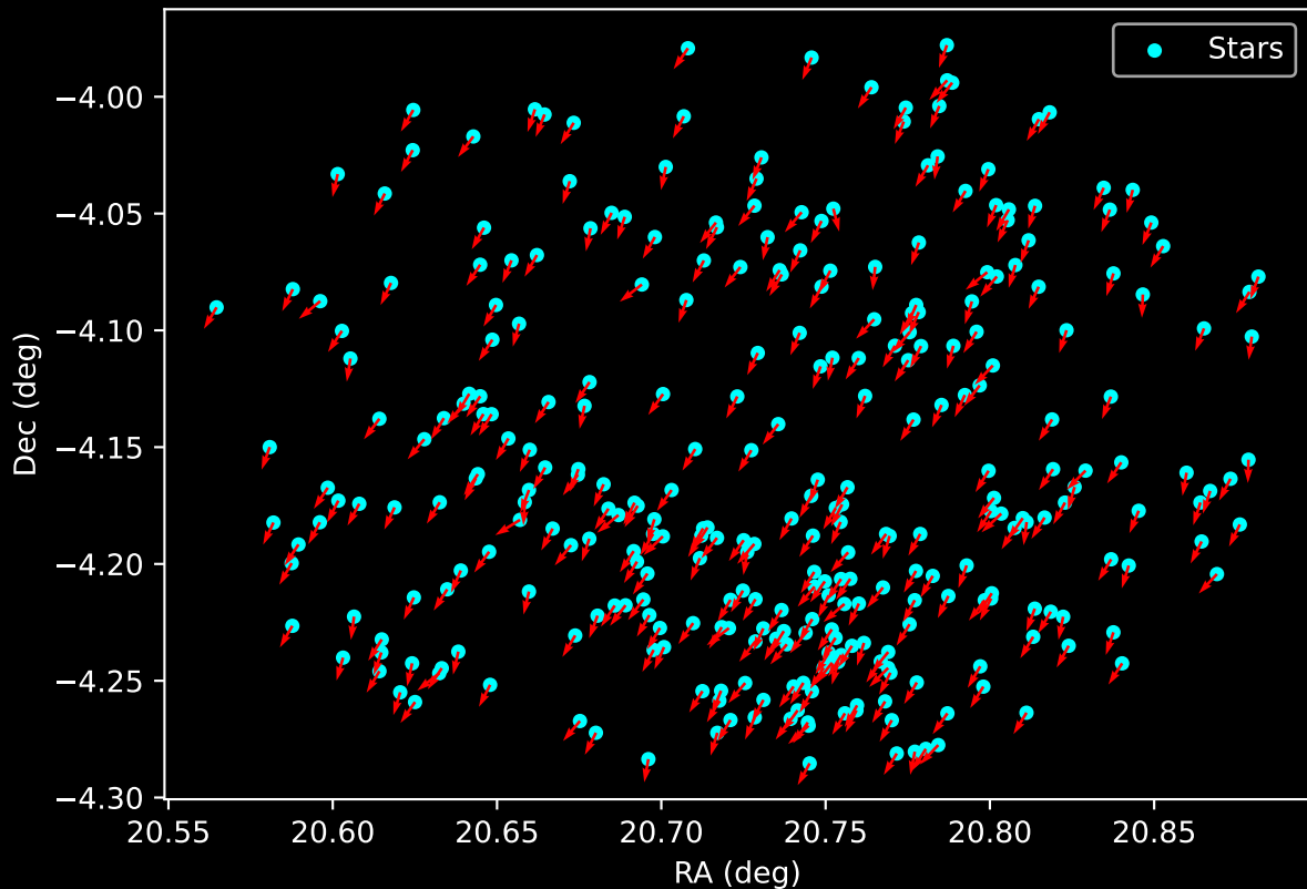
Gaia Cluster: [Trumpler_35] Proper Motion Vectors for Gaia Star Field (n= 315)
