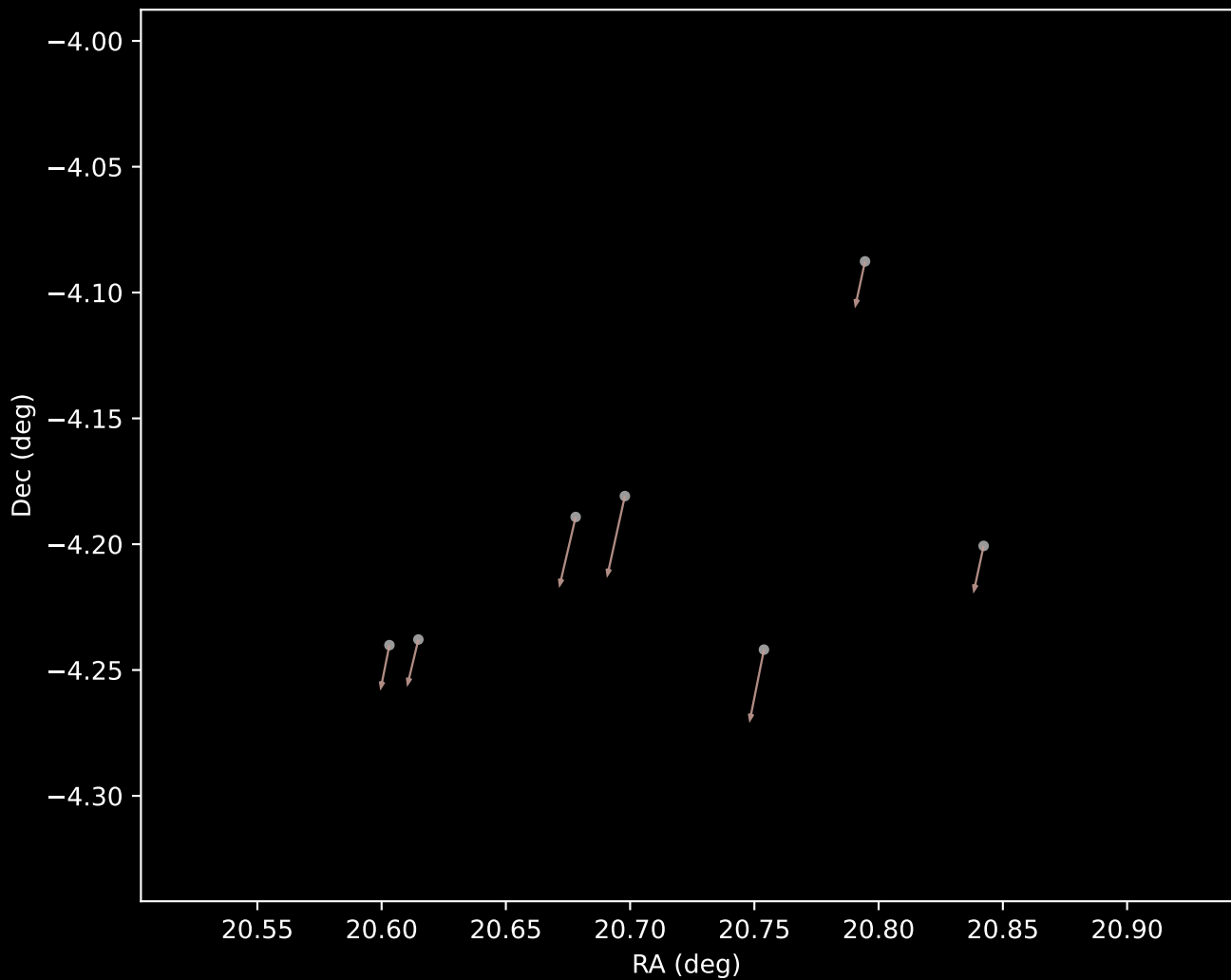
Gaia DR3 Cluster 11 Proper Motion Vectors (n=7)
