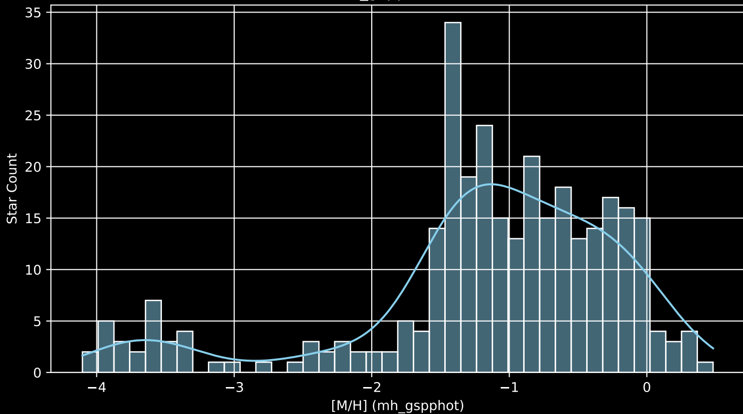
Gaia Cluster: [Trumpler_35 [M/H] (mh_gspphot) (n= 313)
