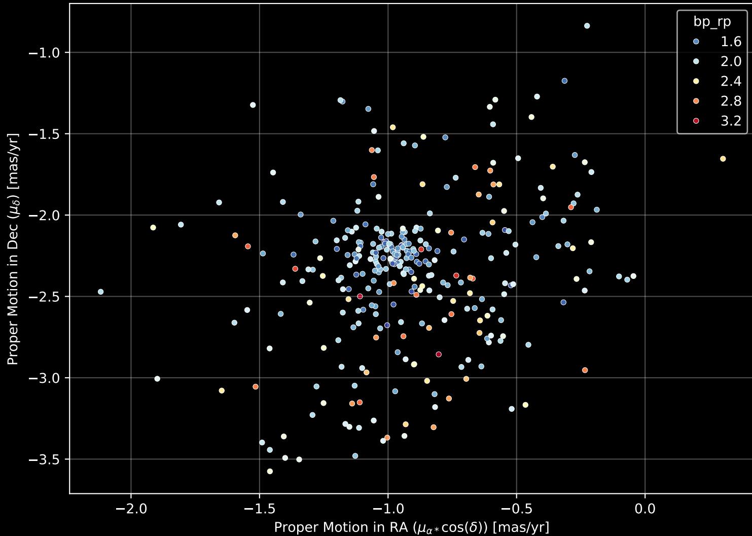
Gaia Cluster: [Trumpler_35] Proper Motion Diagram (n= 315)
