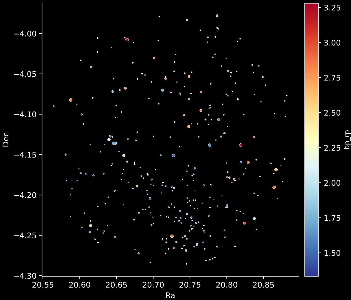
Gaia Cluster: [Trumpler_35] Stars: 315
