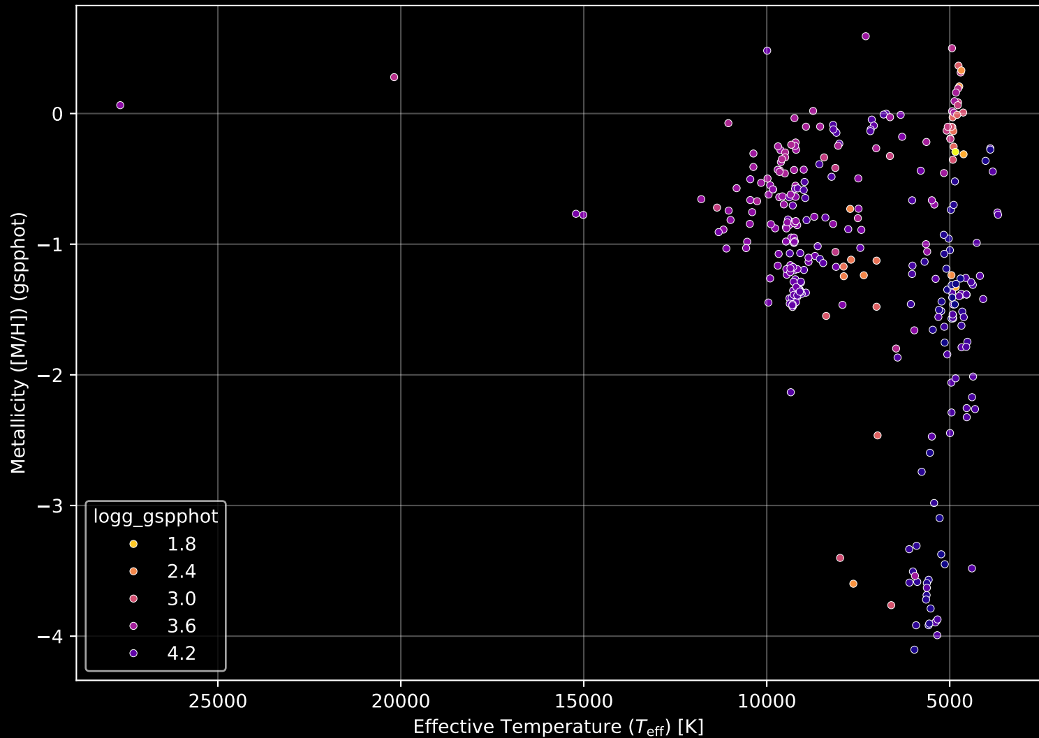
Gaia Cluster: [Trumpler_35] Stellar Population Parameters (n= 315)
