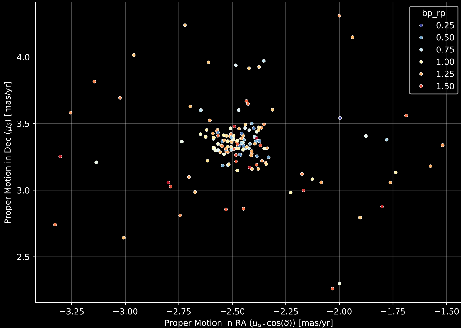
Gaia Cluster: [Trumpler_7] Proper Motion Diagram (n= 152)
