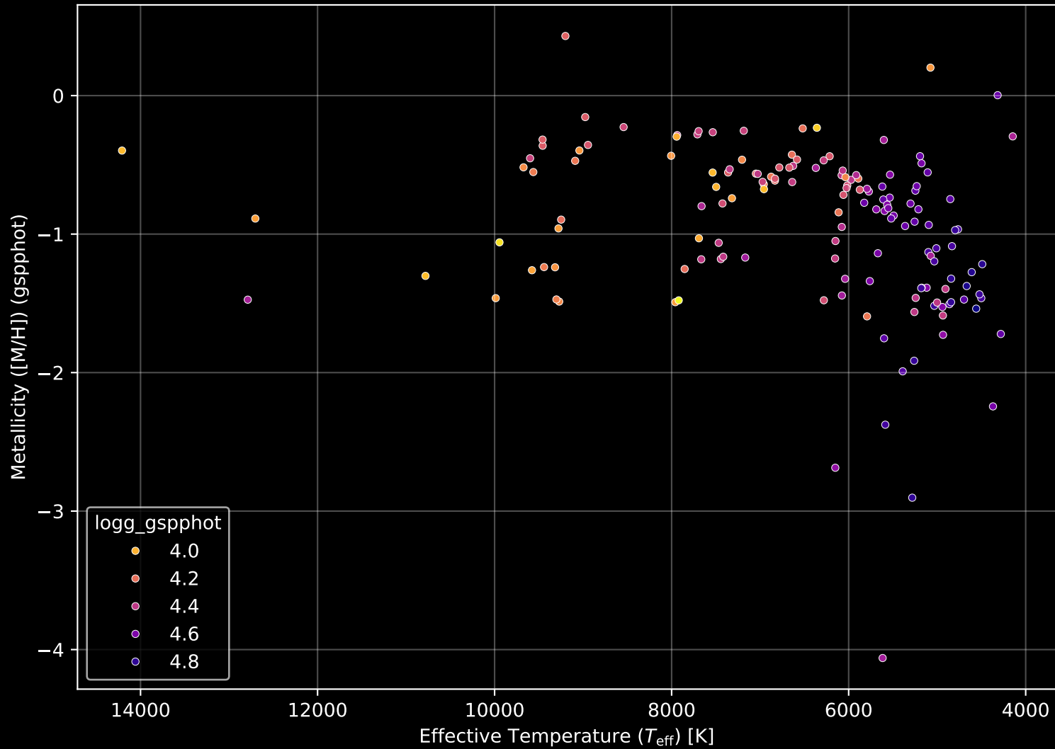
Gaia Cluster: [Trumpler_7] Stellar Population Parameters (n= 152)
