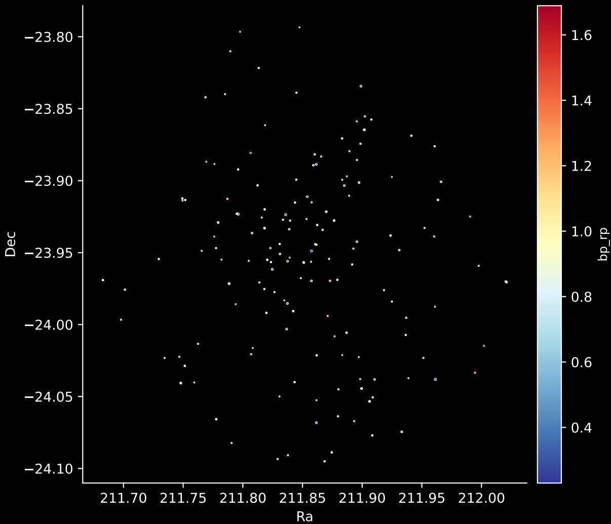
Gaia Cluster: [Trumpler_7] Stars: 152
