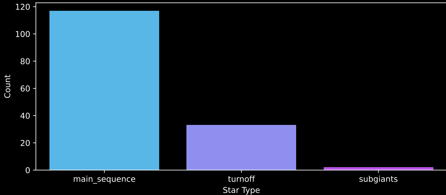
Gaia Cluster: [Trumpler_7] Count plot of Star Type
