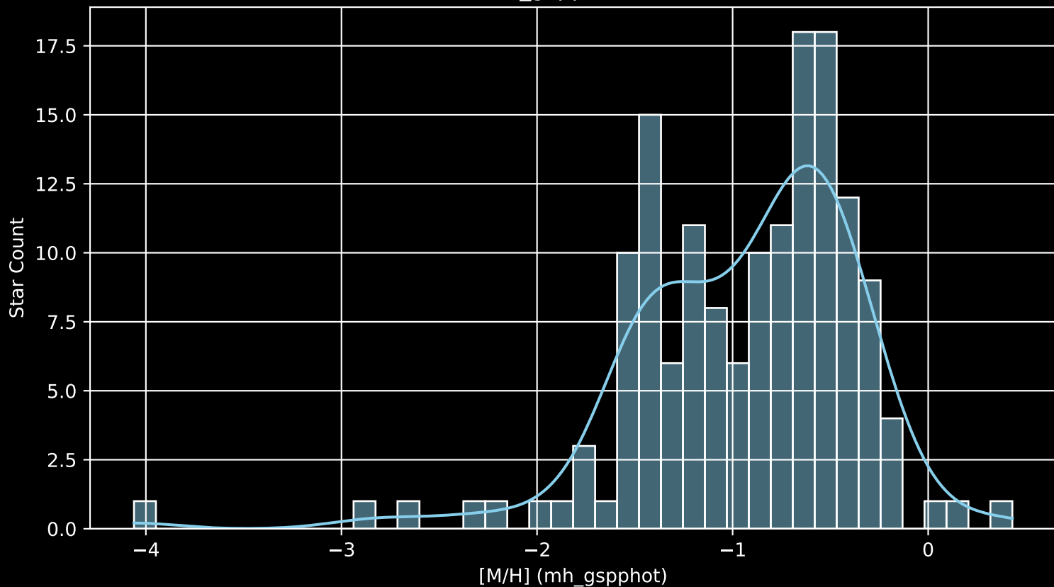
Gaia Cluster: [Trumpler 7 [M/H] (mh_gspphot) (n= 152)
