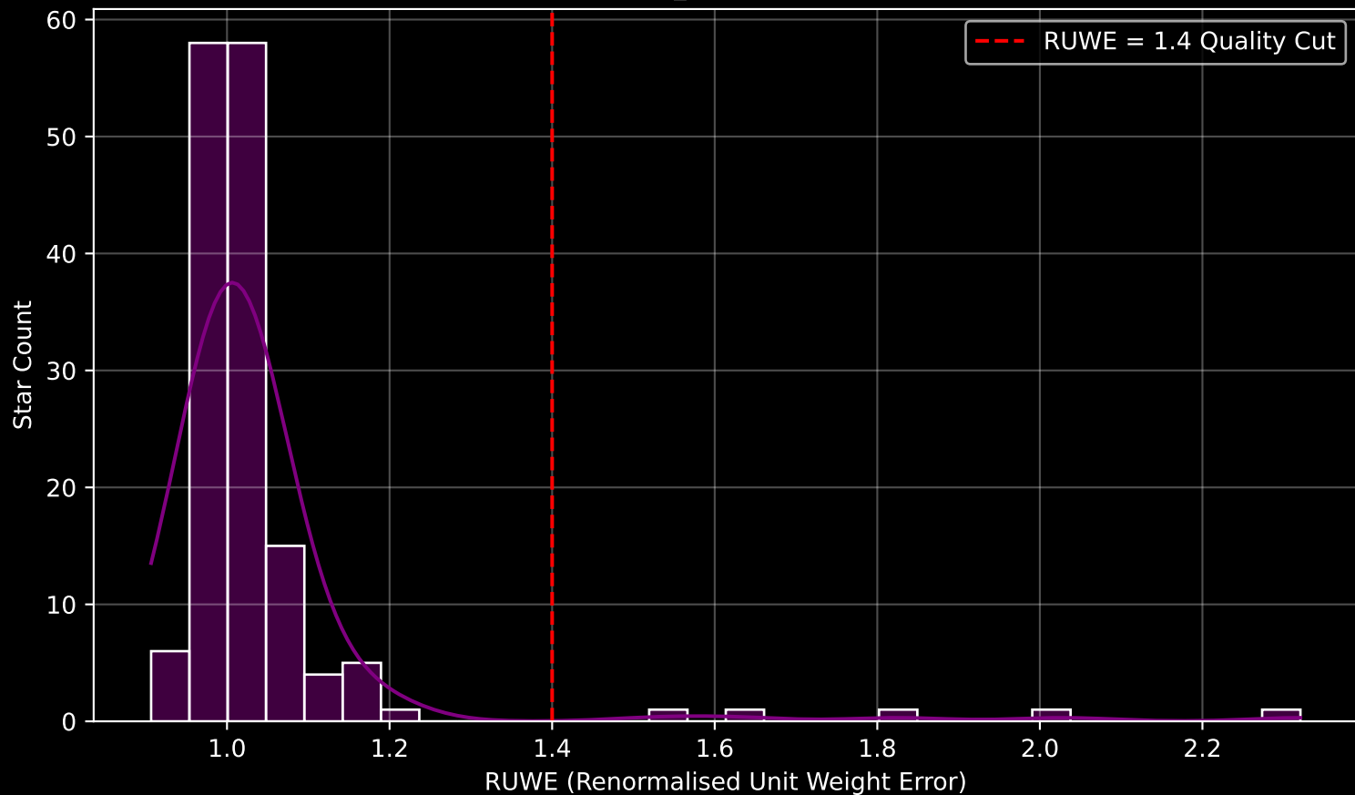
Gaia Cluster: [Trumpler_7] RUWE Distribution (n= 152)
