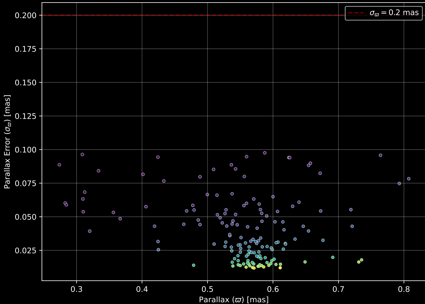
Gaia Cluster: [Trumpler_7] Parallax Quality (n= 152)
