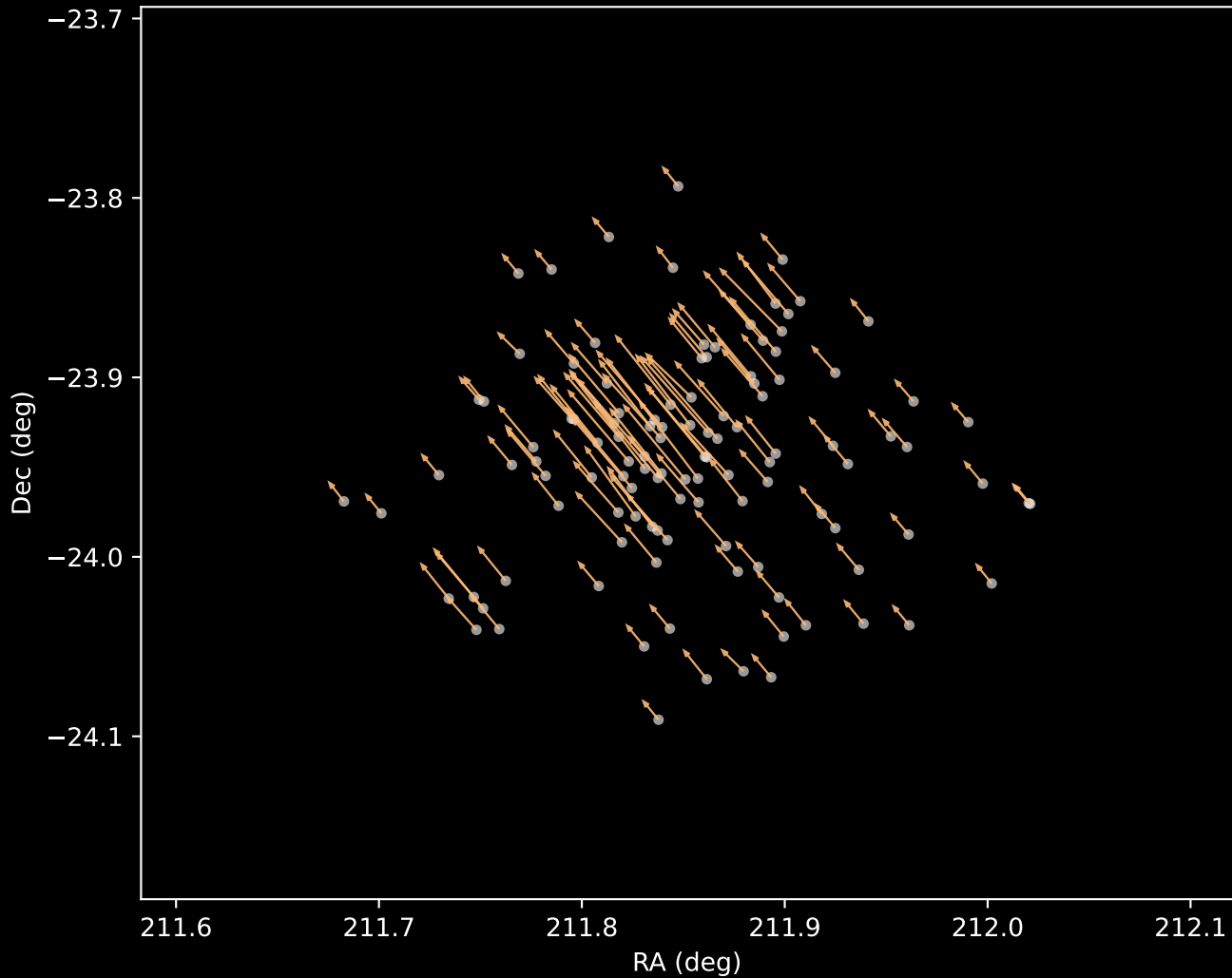
Gaia DR3 Cluster 3 Proper Motion Vectors (n=115)
