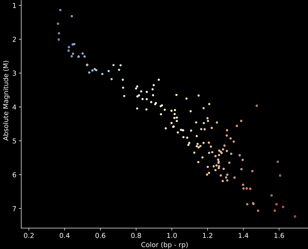
Gaia Cluster: [Trumpler_7] Stars (n= 152) Hertzsprung-Russel Diagram
