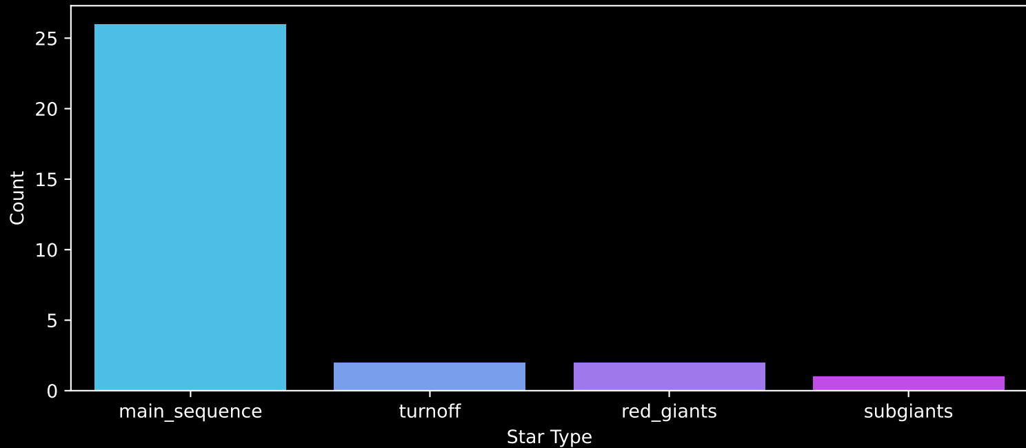
Gaia Cluster: [Turner_5] Count plot of Star Type
