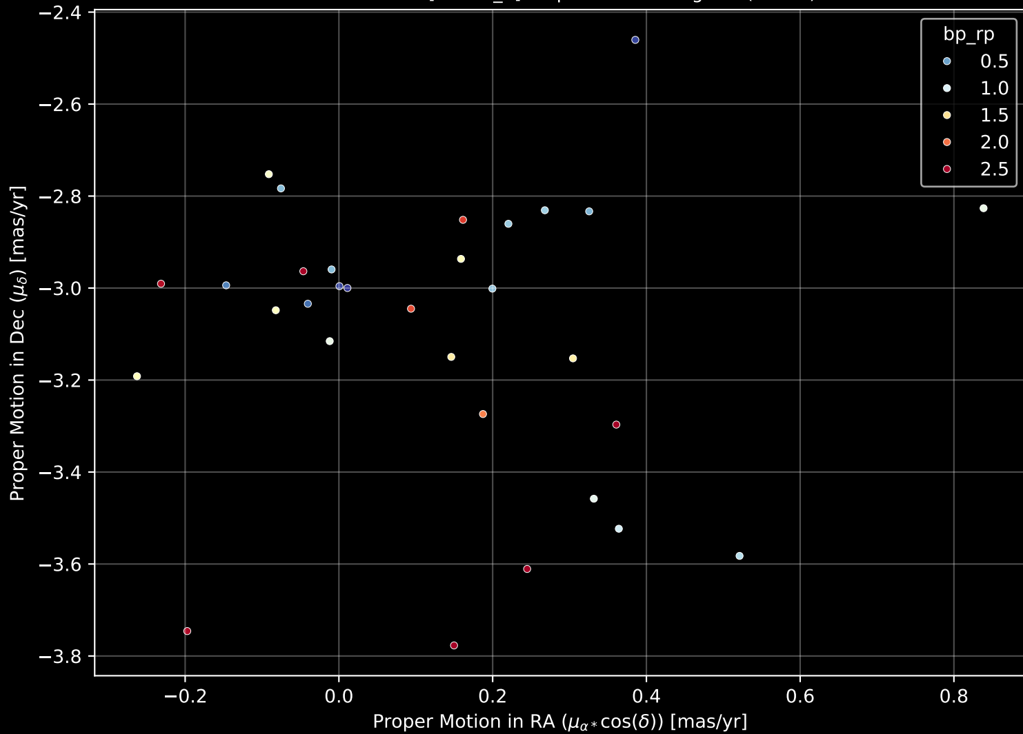
Gaia Cluster: [Turner_5] Proper Motion Diagram (n= 31)
