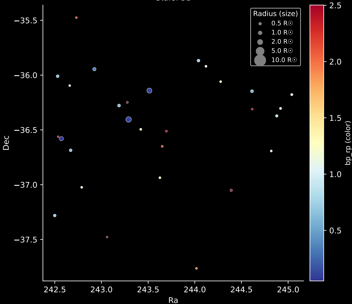
Gaia Cluster: [Turner_5] Stars: 31
