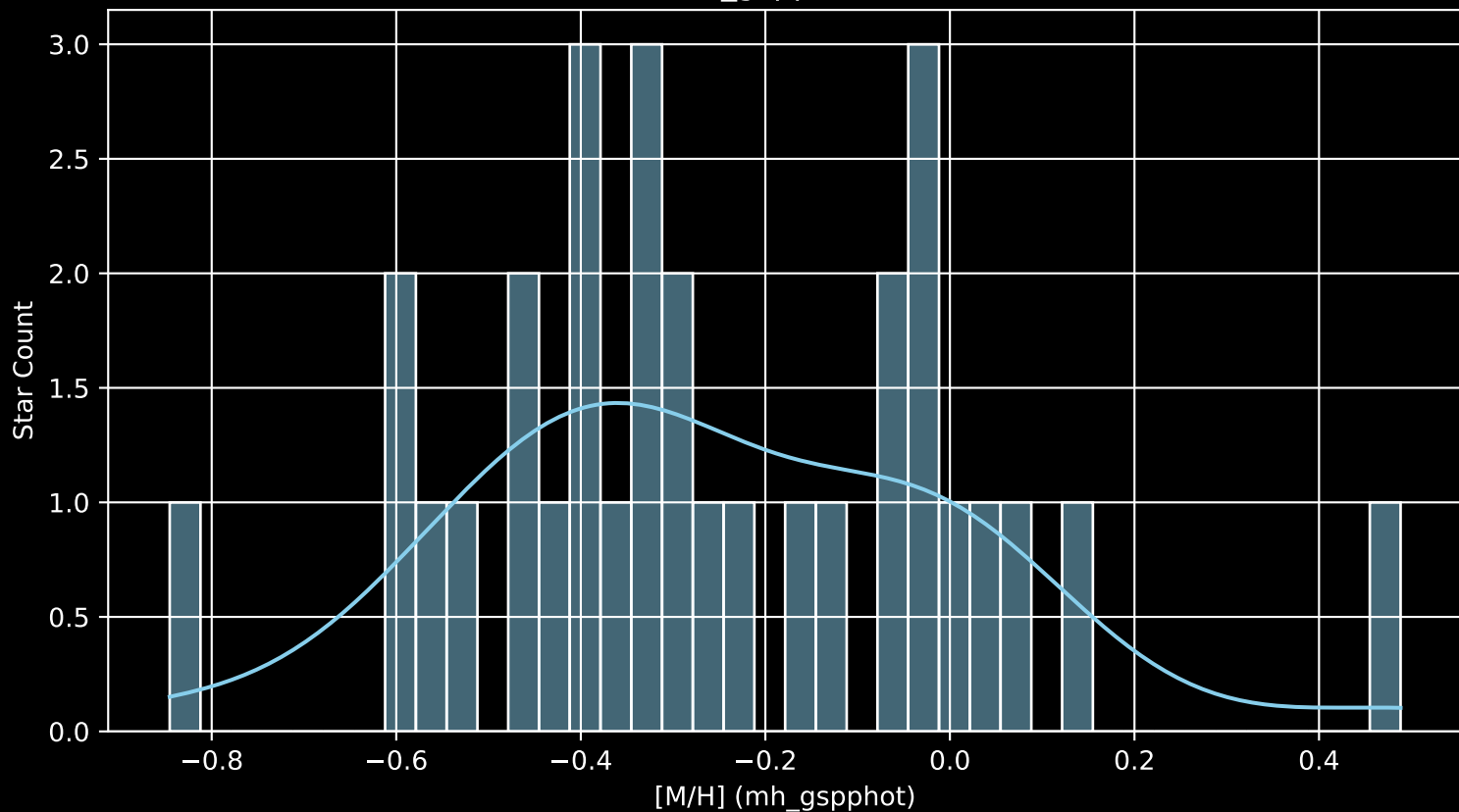
Gaia Cluster: [Turner_5 [M/H] (mh_gspphot) (n= 31)
