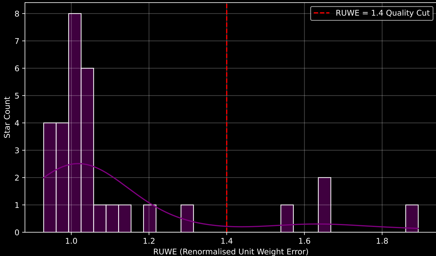
Gaia Cluster: [Turner_5] RUWE Distribution (n= 31)
