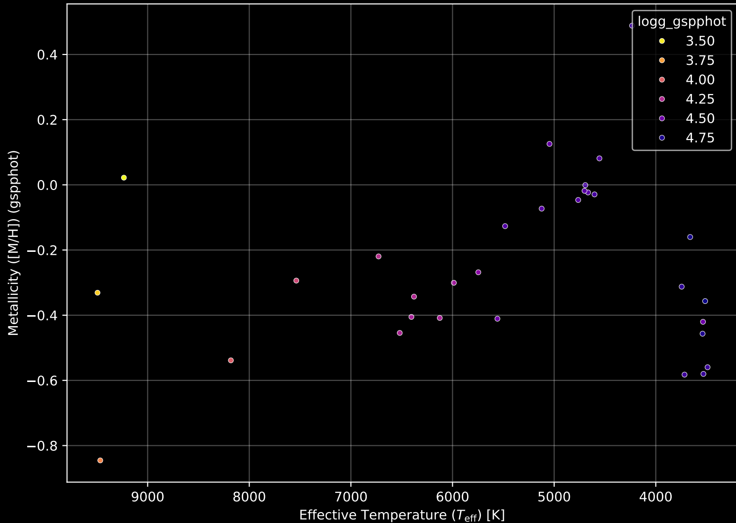
Gaia Cluster: [Turner_5] Stellar Population Parameters (n= 31)
