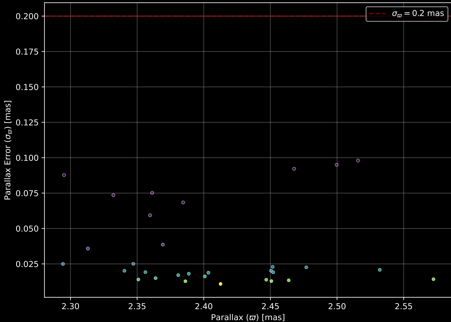
Gaia Cluster: [Turner_5] Parallax Quality (n= 31)
