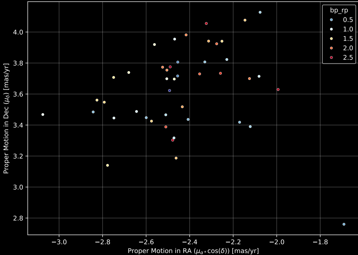
Gaia Cluster: [UBC_1] Proper Motion Diagram (n= 45)
