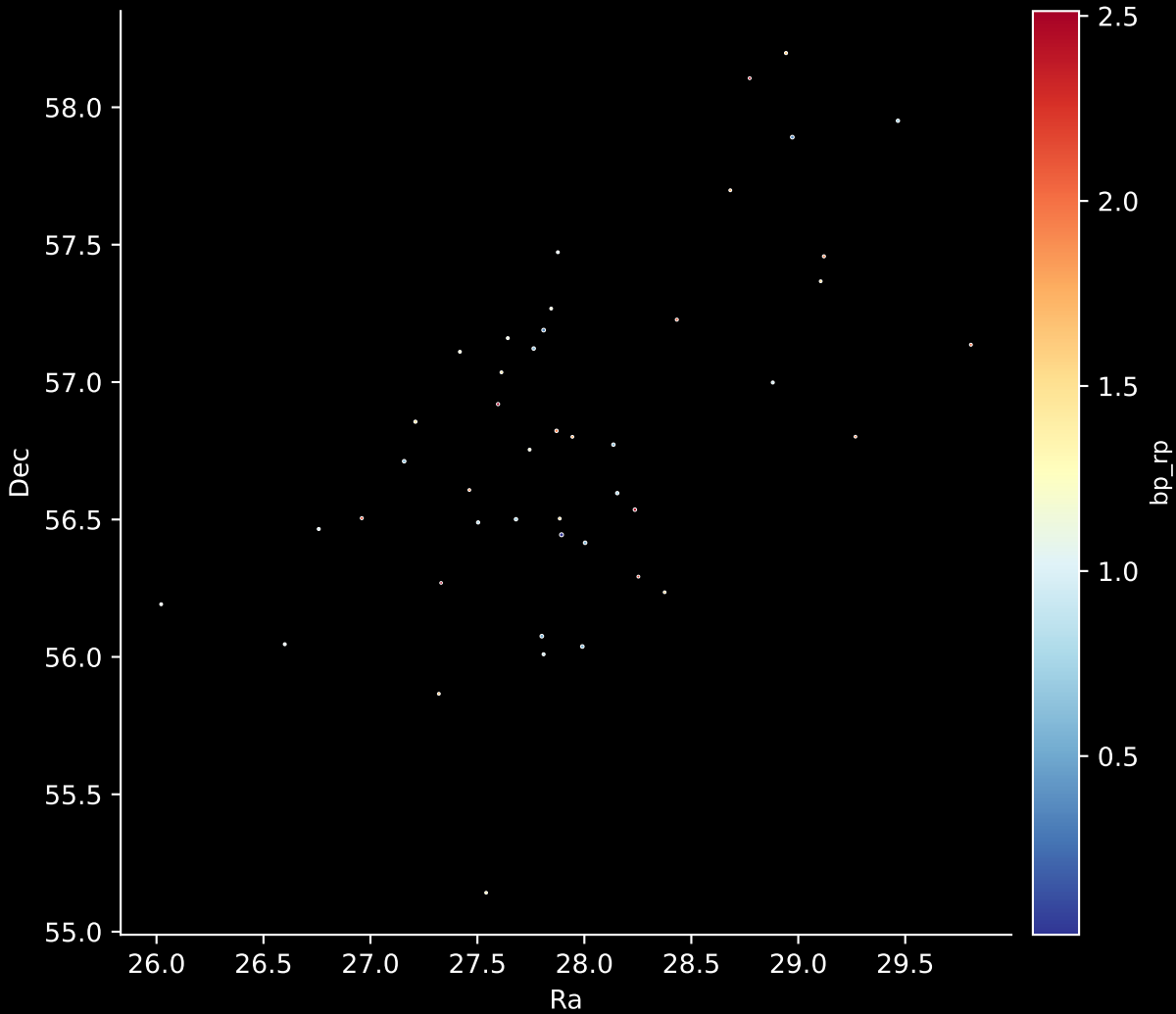
Gaia Cluster: [UBC_1] Stars: 45
