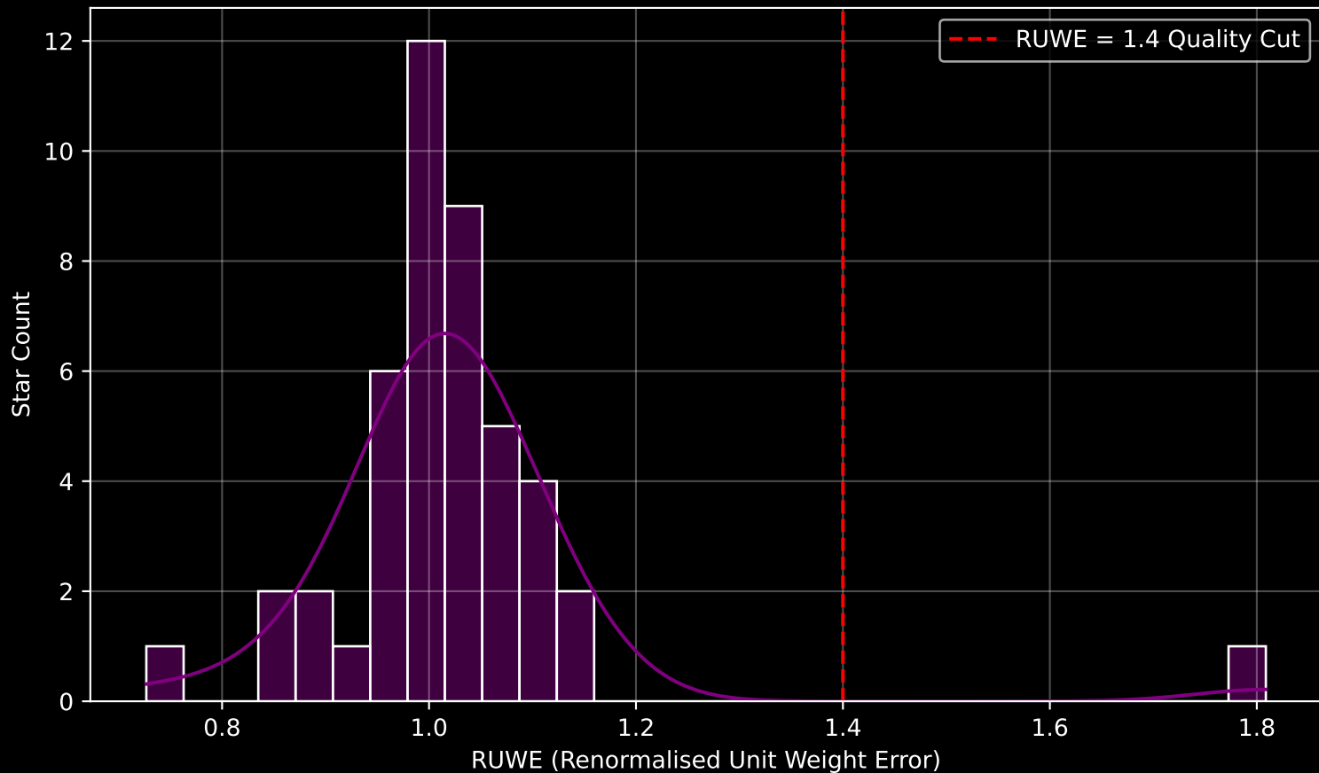
Gaia Cluster: [UBC_1] RUWE Distribution (n= 45)
