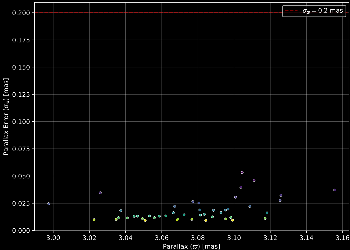
Gaia Cluster: [UBC_1] Parallax Quality (n= 45)
