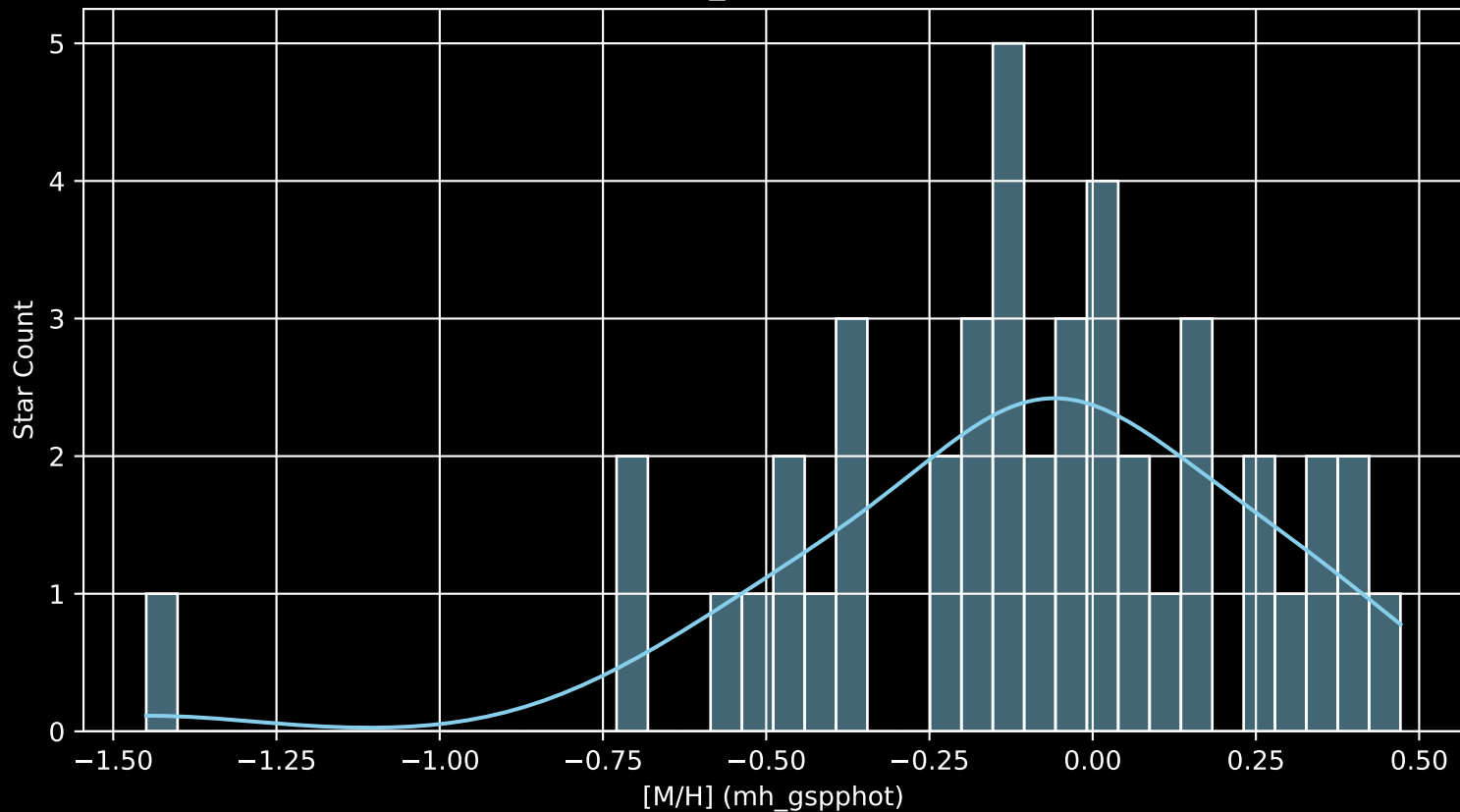
Gaia Cluster: [UBC_1 [M/H] (mh_gspphot) (n= 44)
