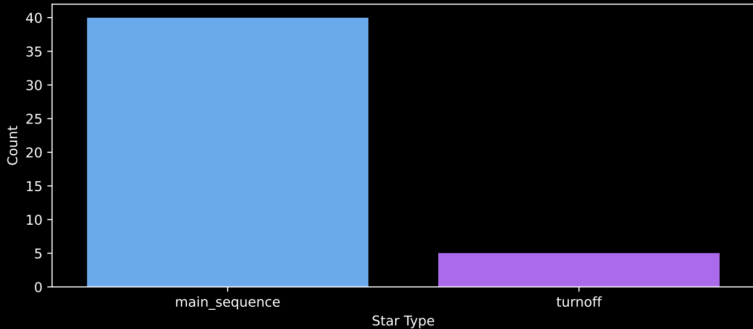
Gaia Cluster: [UBC_1] Count plot of Star Type
