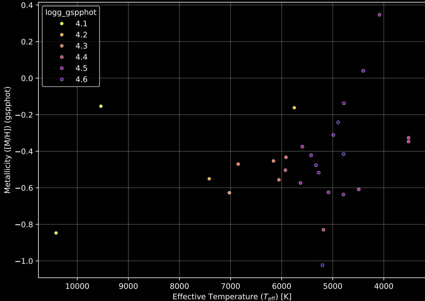
Gaia Cluster: [UBC_11] Stellar Population Parameters (n= 28)
