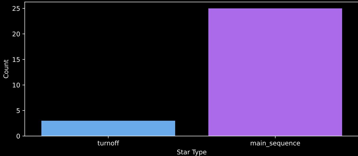
Gaia Cluster: [UBC_11] Count plot of Star Type
