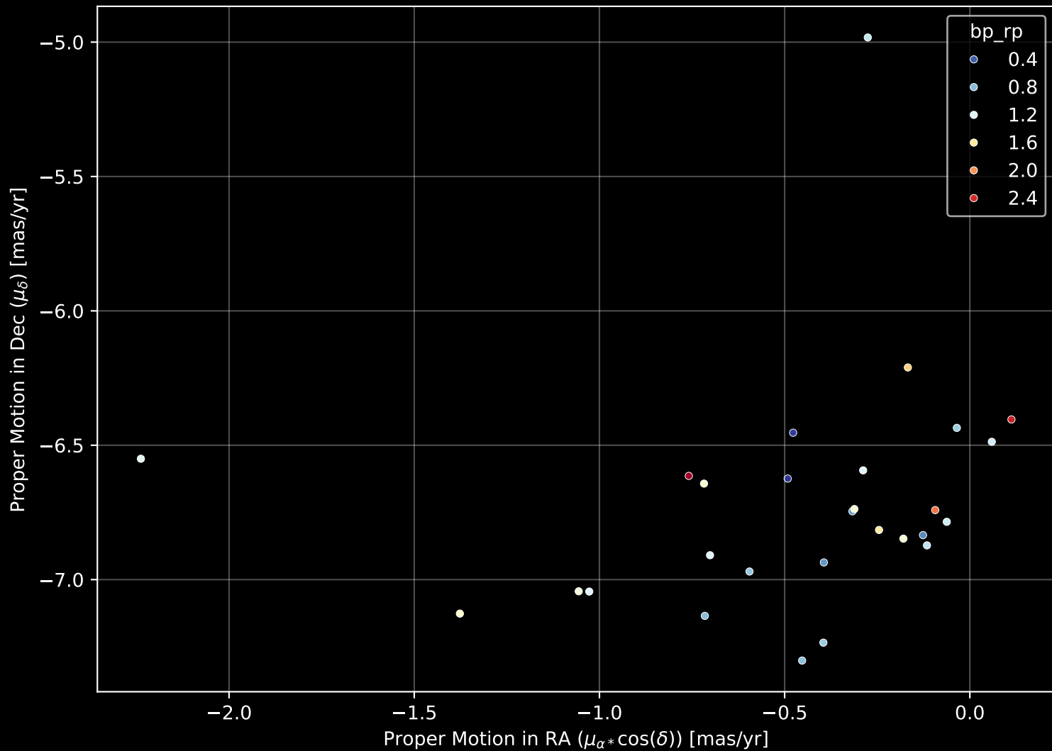
Gaia Cluster: [UBC_11] Proper Motion Diagram (n= 28)
