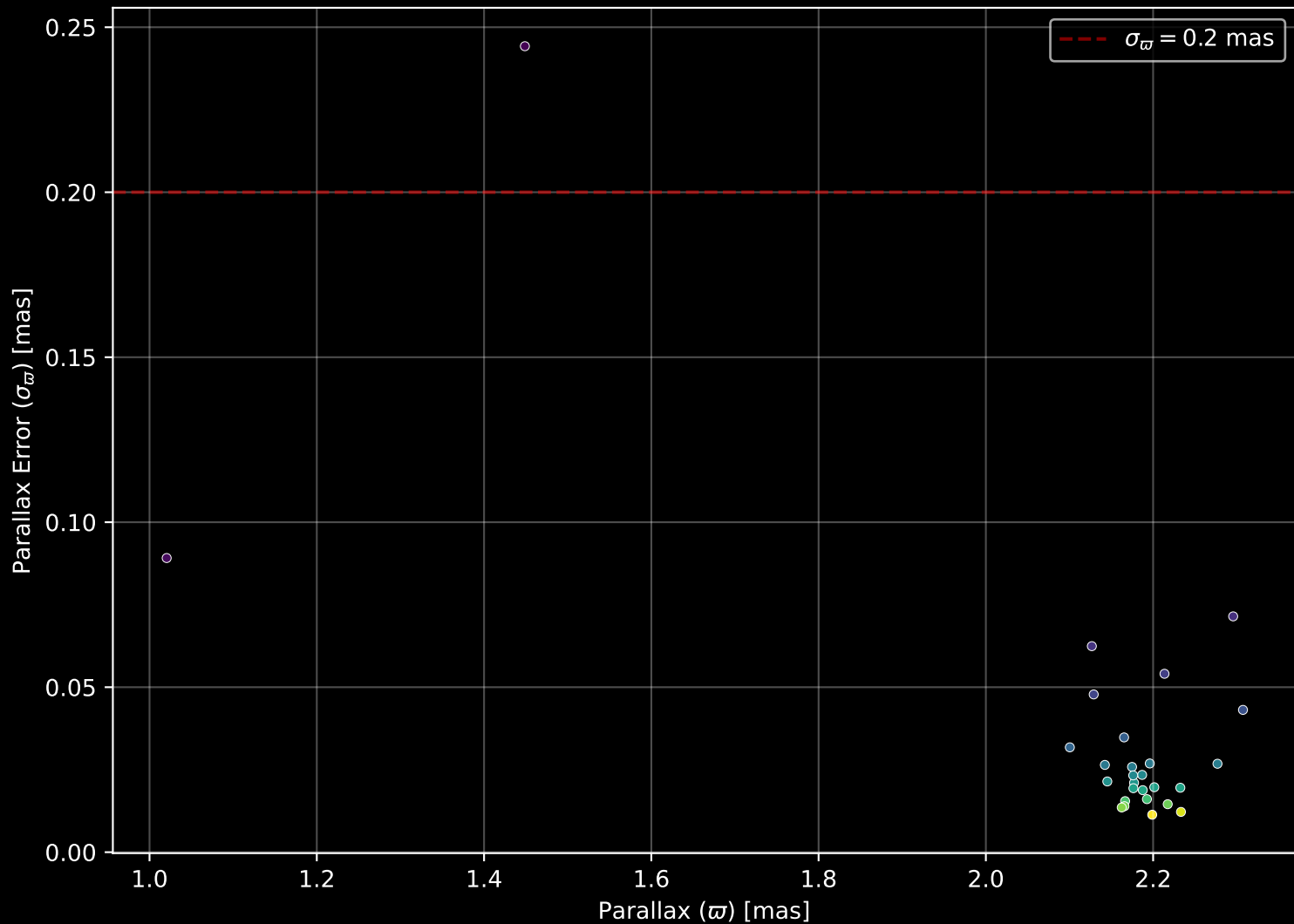
Gaia Cluster: [UBC_11] Parallax Quality (n= 28)
