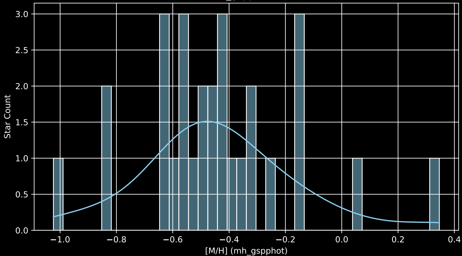
Gaia Cluster: [UBC_11 [M/H] (mh_gspphot) ( \bar{n}=28 )
