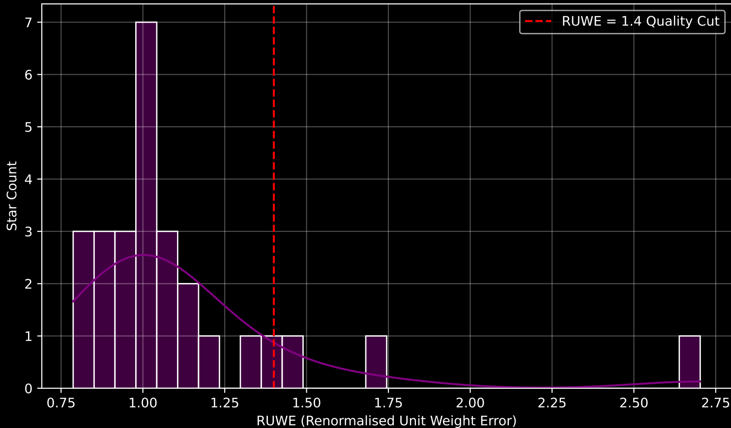
Gaia Cluster: [UBC_11] RUWE Distribution (n= 27)
