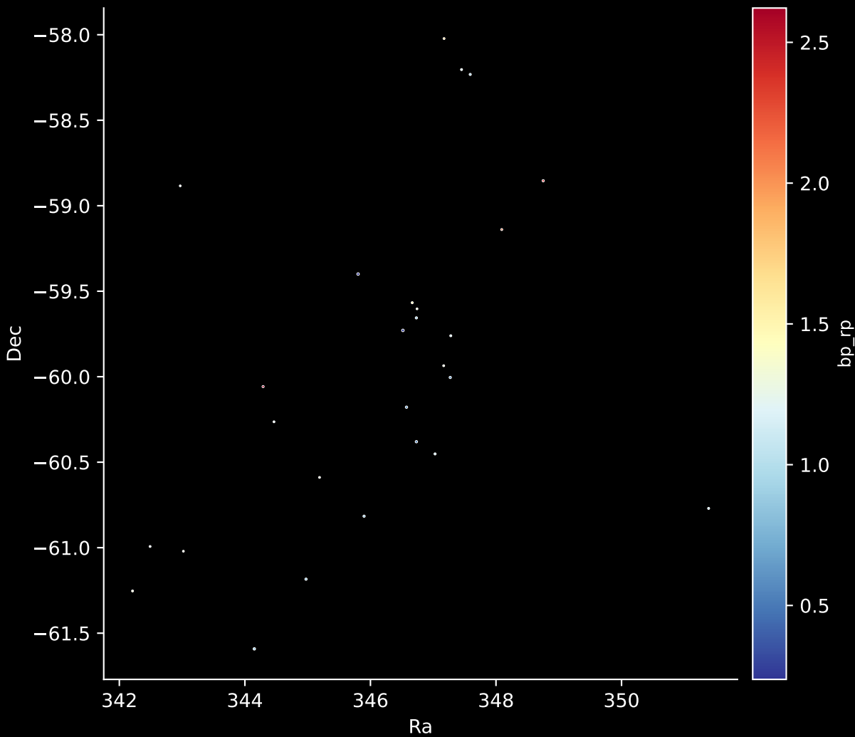
Gaia Cluster: [UBC_11] Stars: 28
