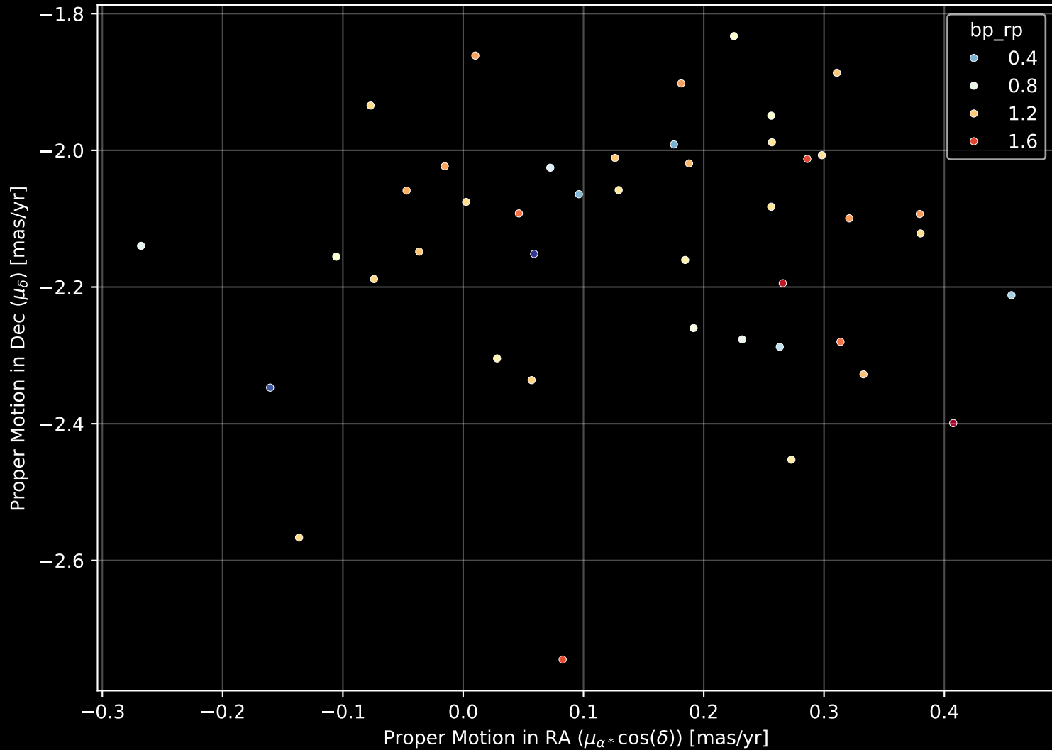
Gaia Cluster: [UBC_14] Proper Motion Diagram (n= 43)
