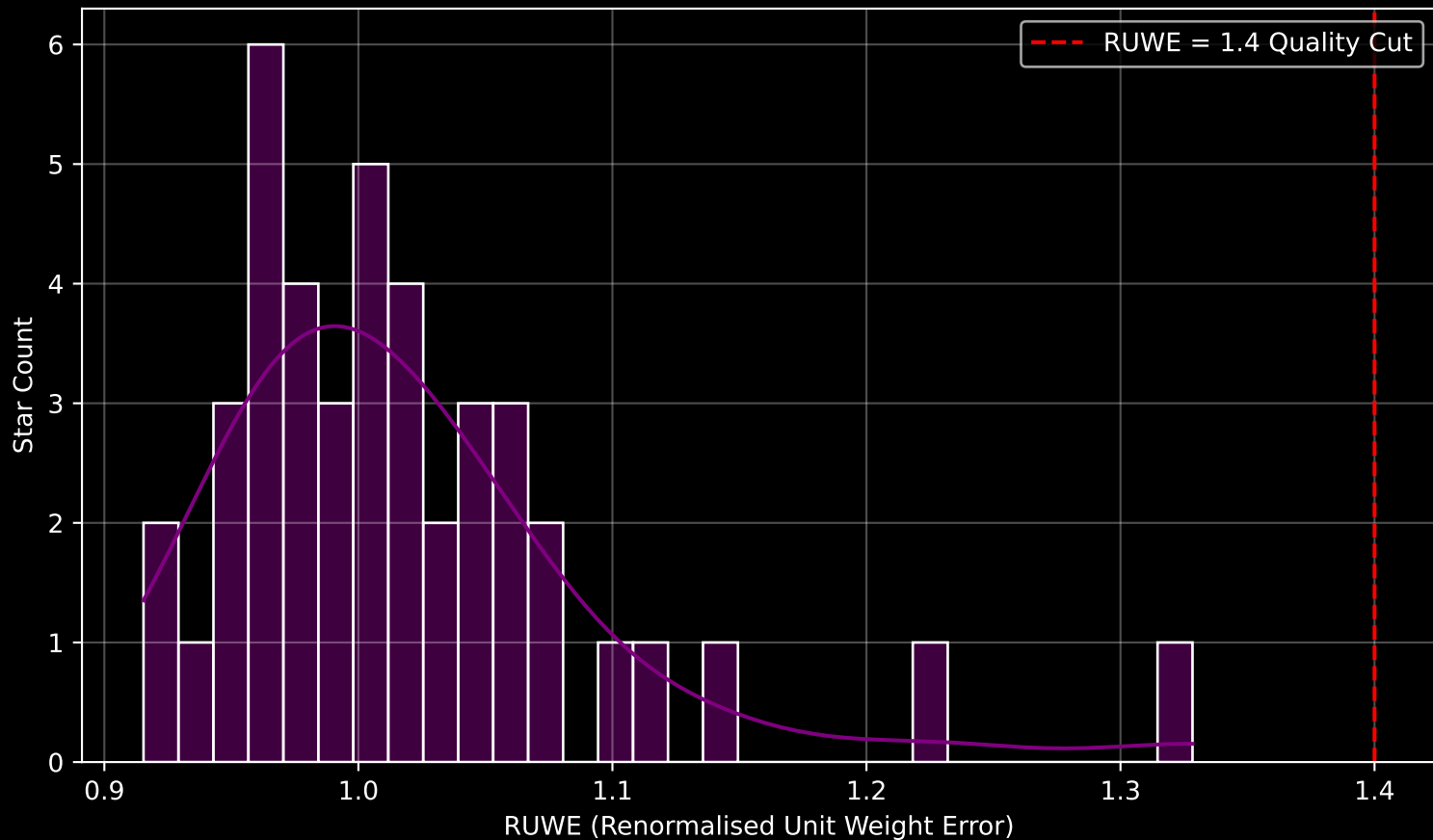
Gaia Cluster: [UBC_14] RUWE Distribution (n= 43)
