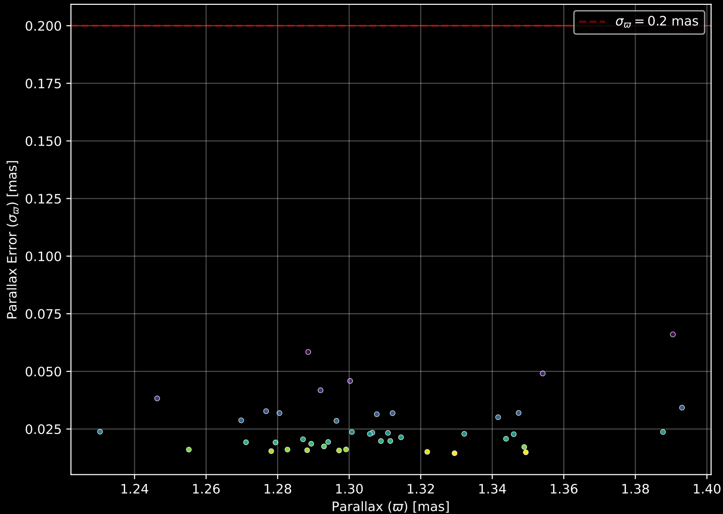
Gaia Cluster: [UBC_14] Parallax Quality (n= 43)
