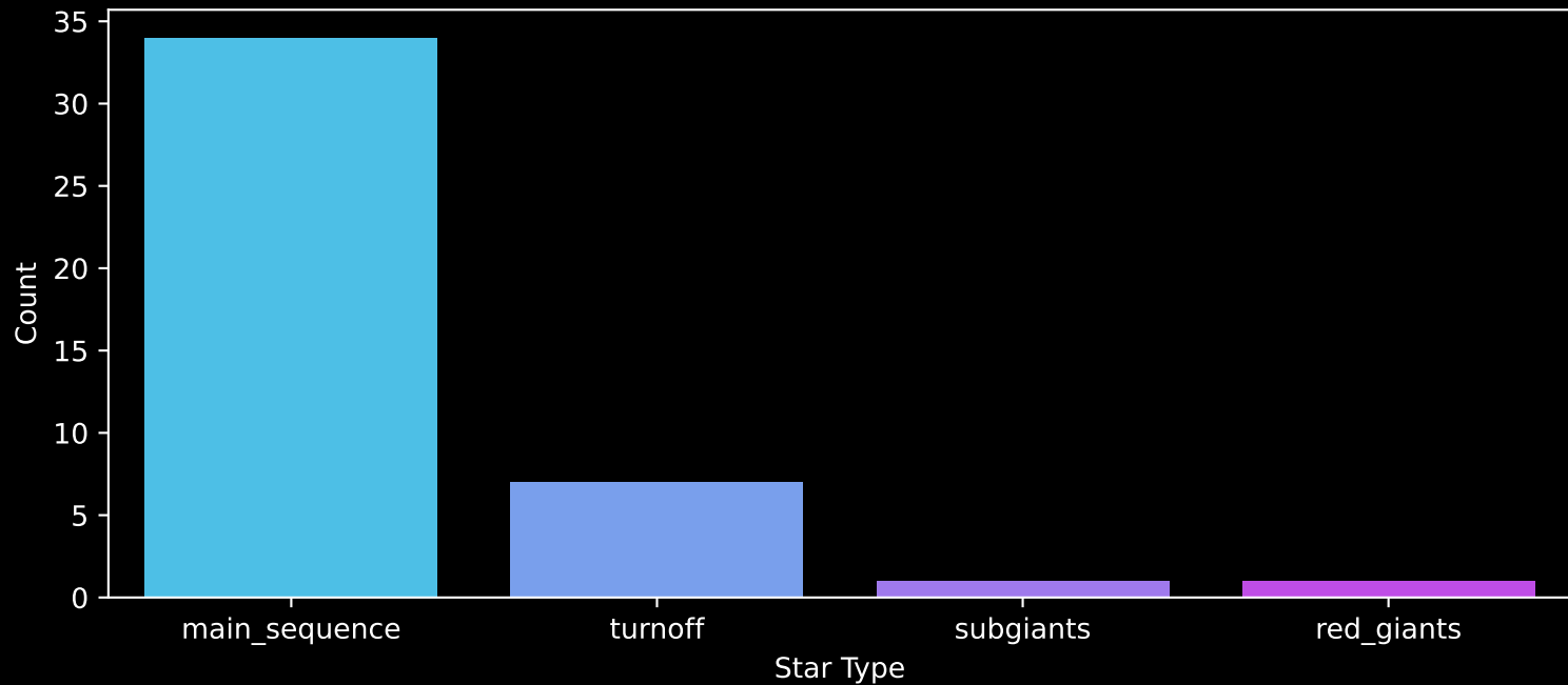
Gaia Cluster: [UBC_14] Count plot of Star Type
