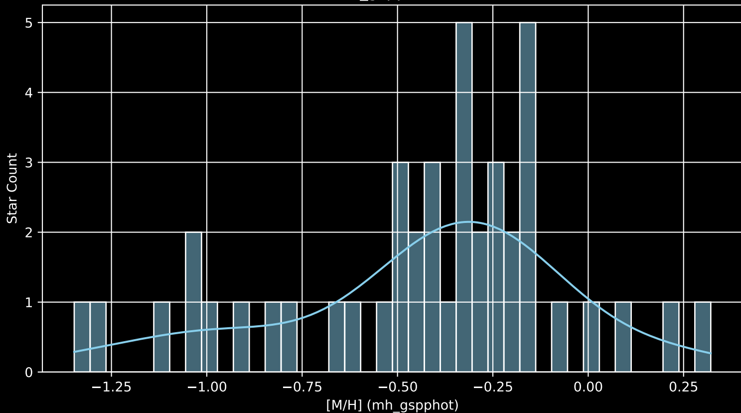
Gaia Cluster: [UBC_14 [M/H] (mh_gspphot) (n= 43)
