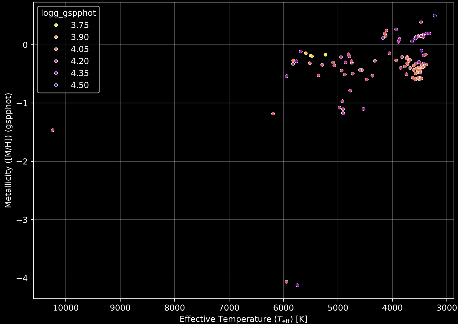
Gaia Cluster: [UBC_17a] Stellar Population Parameters (n= 120)
