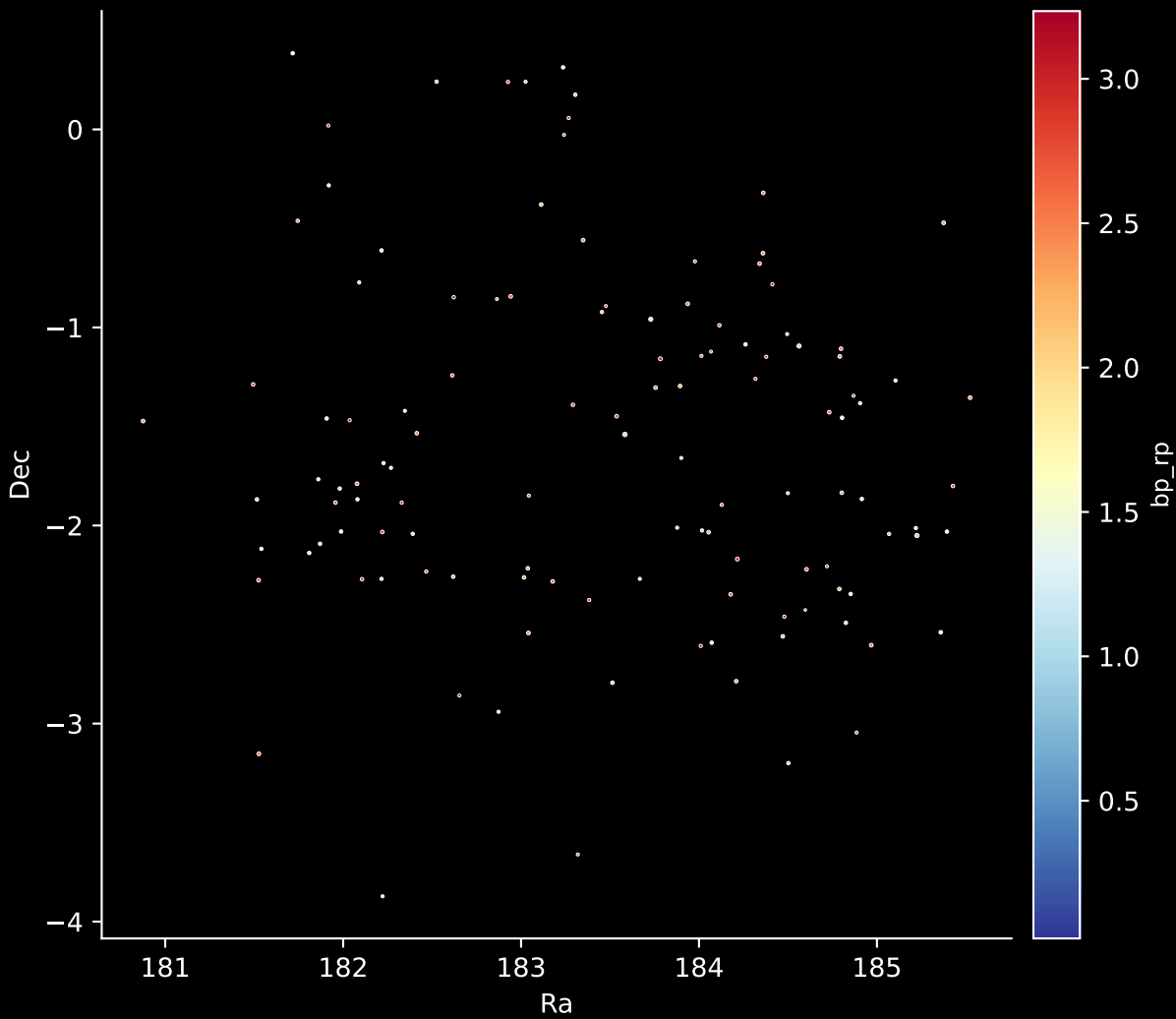
Gaia Cluster: [UBC_17a] Stars: 120
