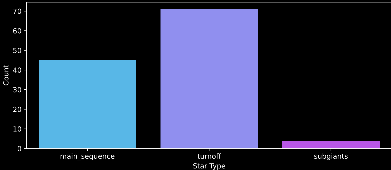
Gaia Cluster: [UBC_17a] Count plot of Star Type
