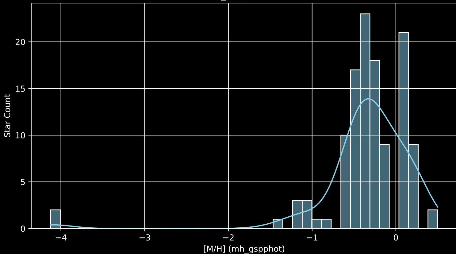
Gaia Cluster: [UBC_17a [M/H] (mh_gspphot) (n= 120)
