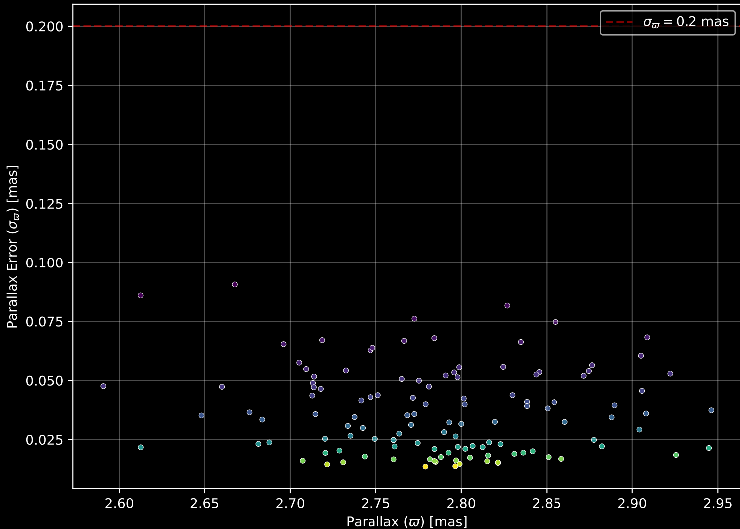
Gaia Cluster: [UBC_17a] Parallax Quality (n= 120)
