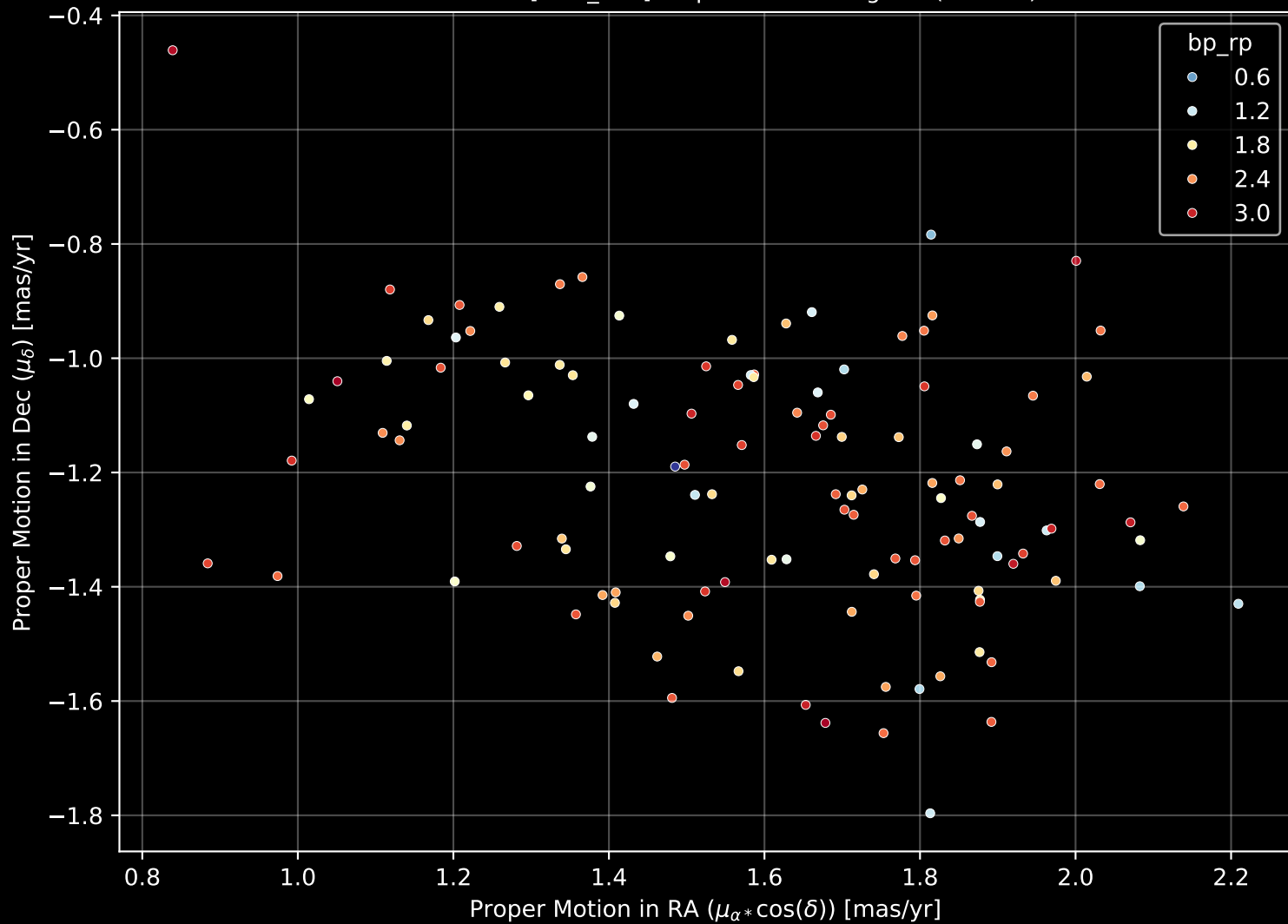
Gaia Cluster: [UBC_17a] Proper Motion Diagram (n= 120)
