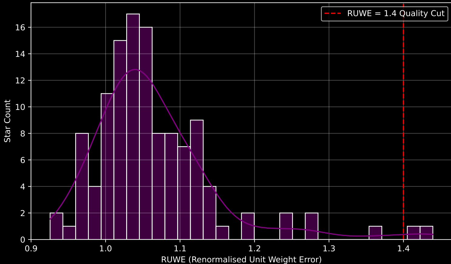
Gaia Cluster: [UBC_17a] RUWE Distribution (n= 120)
