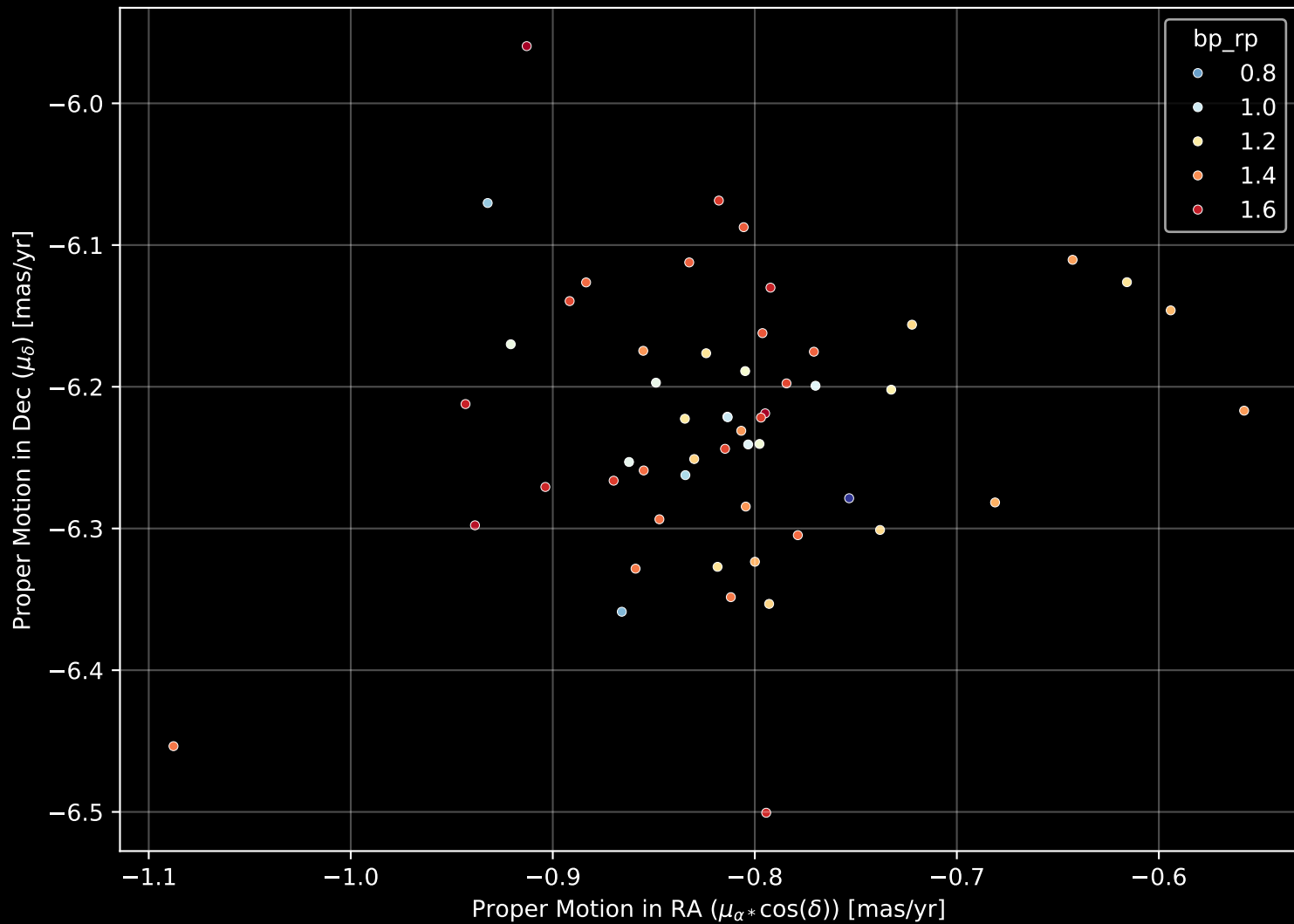
Gaia Cluster: [UBC_27] Proper Motion Diagram (n= 54)
