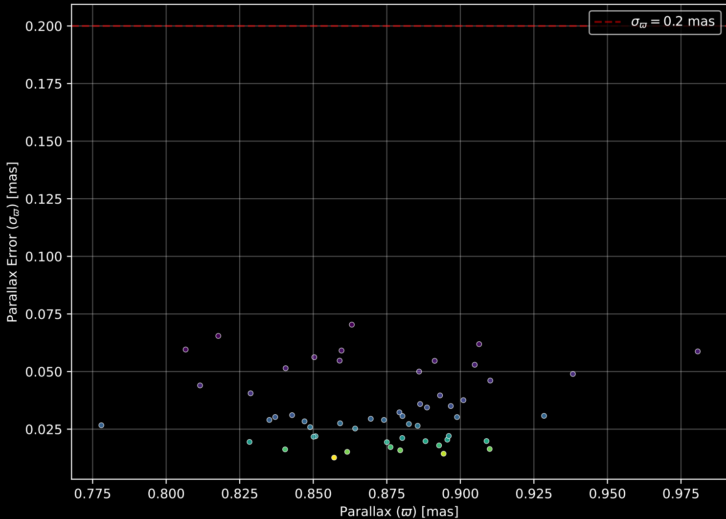
Gaia Cluster: [UBC_27] Parallax Quality (n= 54)
