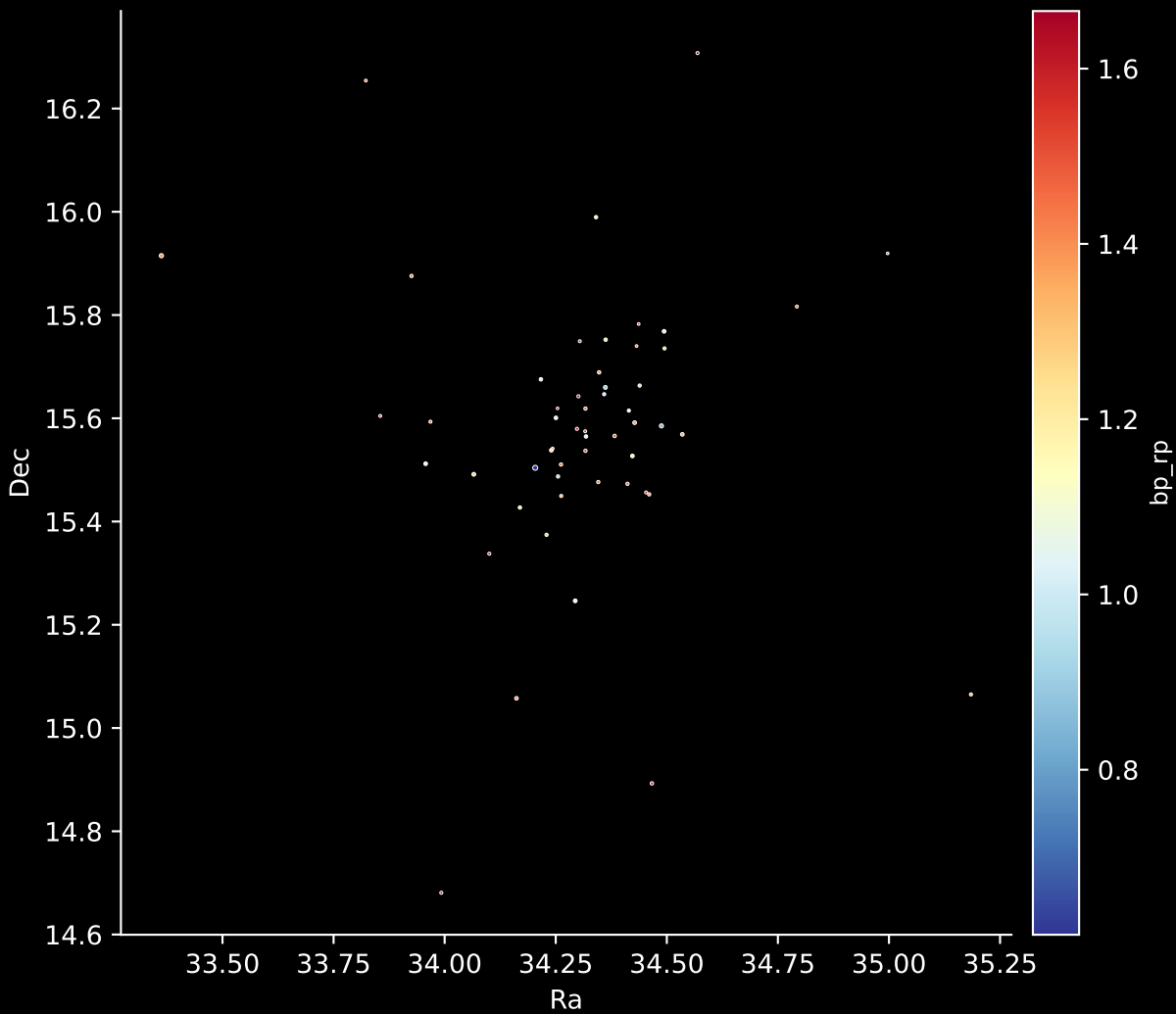
Gaia Cluster: [UBC_27] Stars: 54
