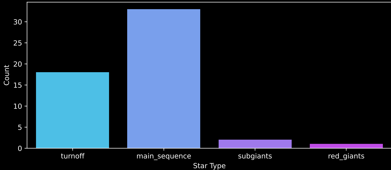
Gaia Cluster: [UBC_27] Count plot of Star Type
