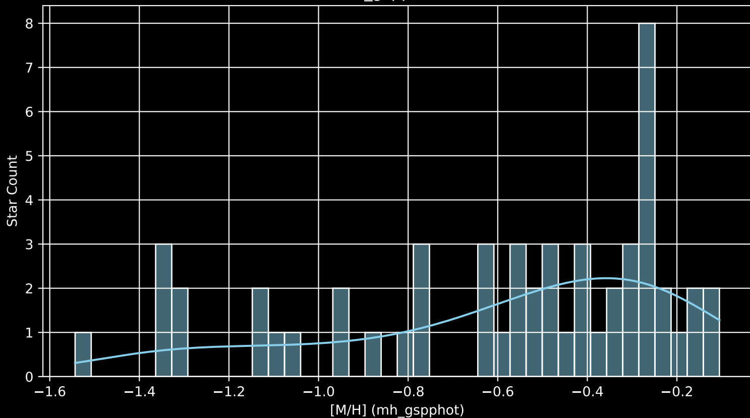
Gaia Cluster: [UBC_27 [M/H] (mh_gspphot) (n= 54)
