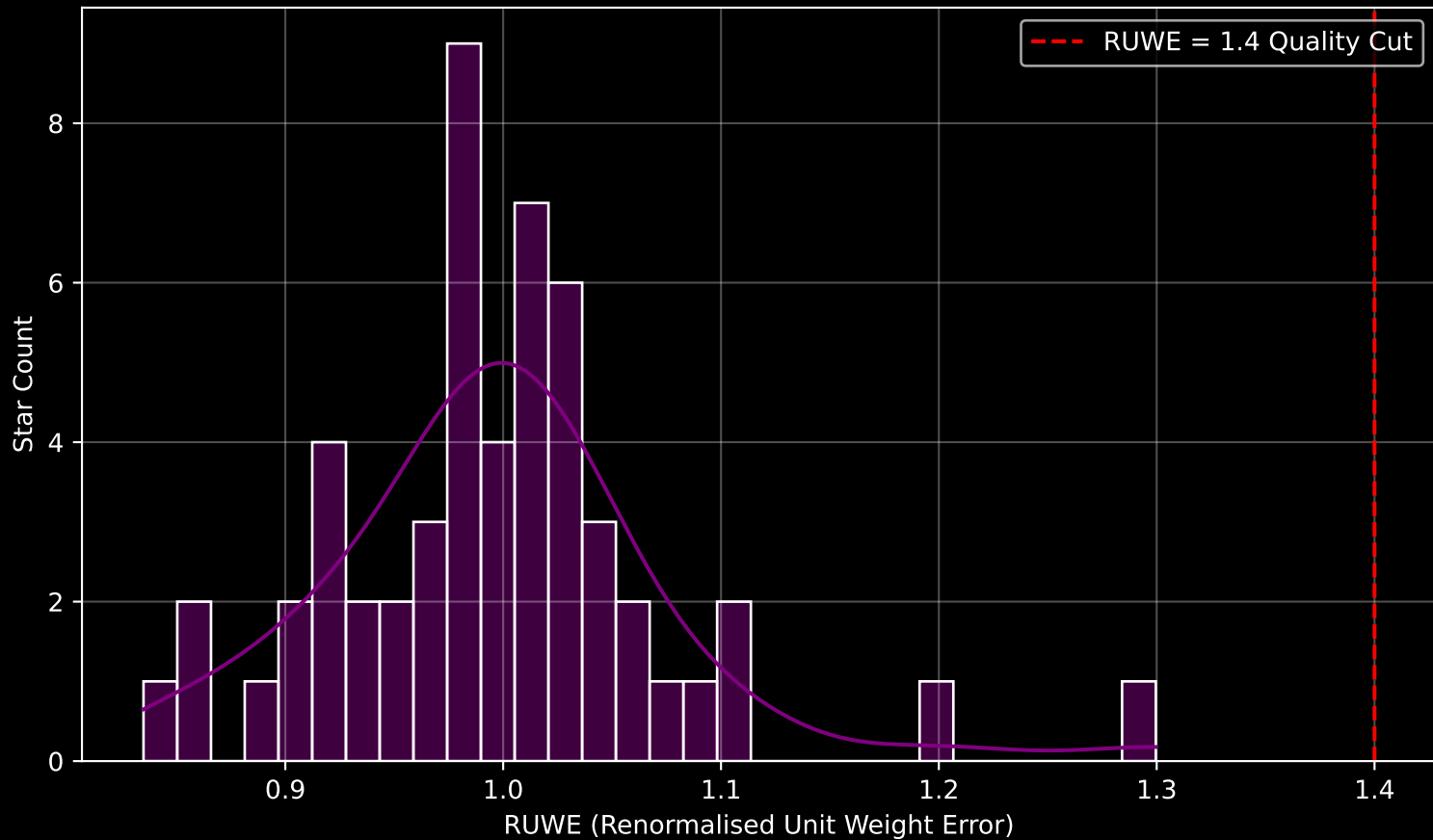
Gaia Cluster: [UBC_27] RUWE Distribution (n= 54)
