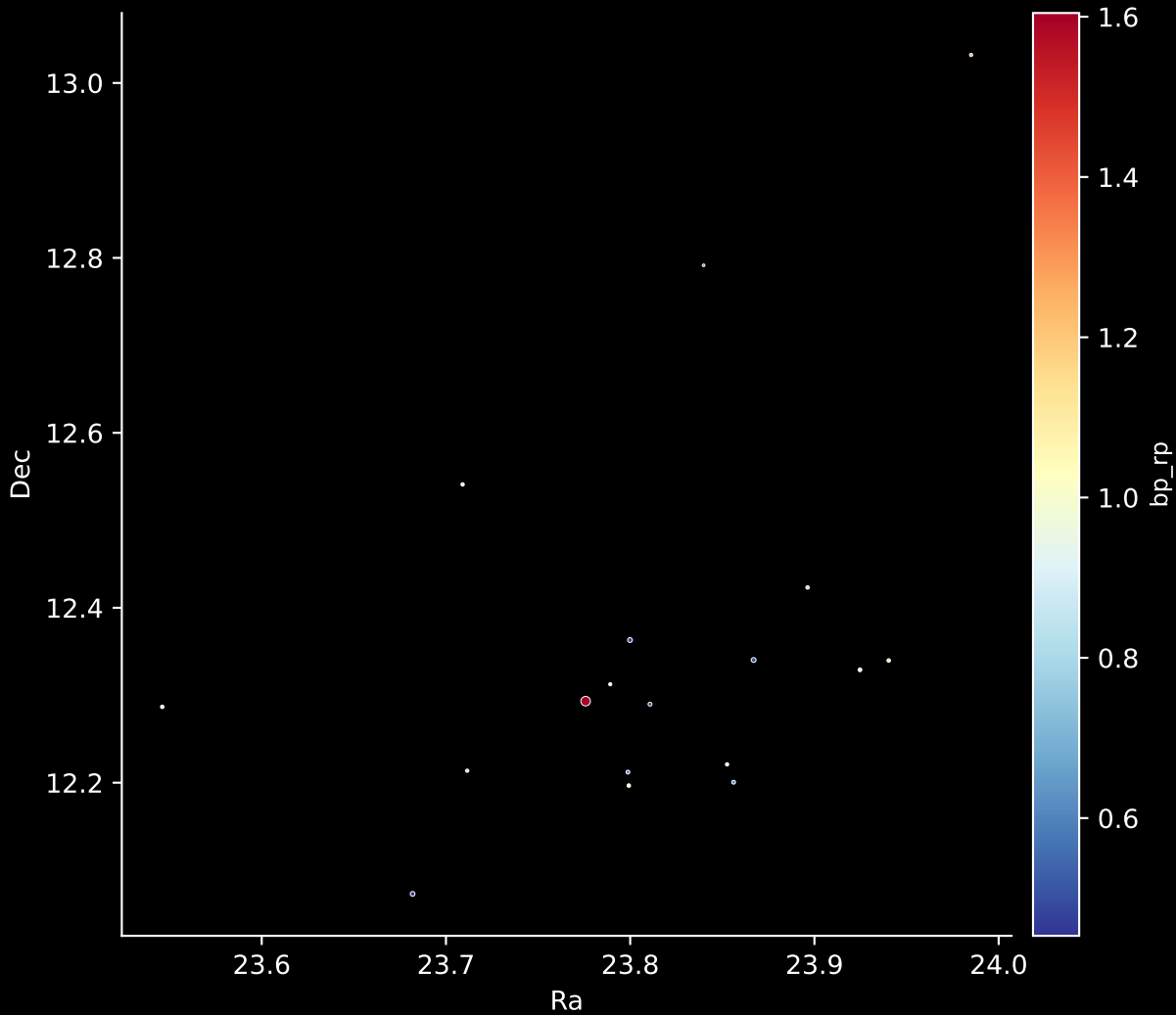
Gaia Cluster: [UBC_3] Stars: 18
