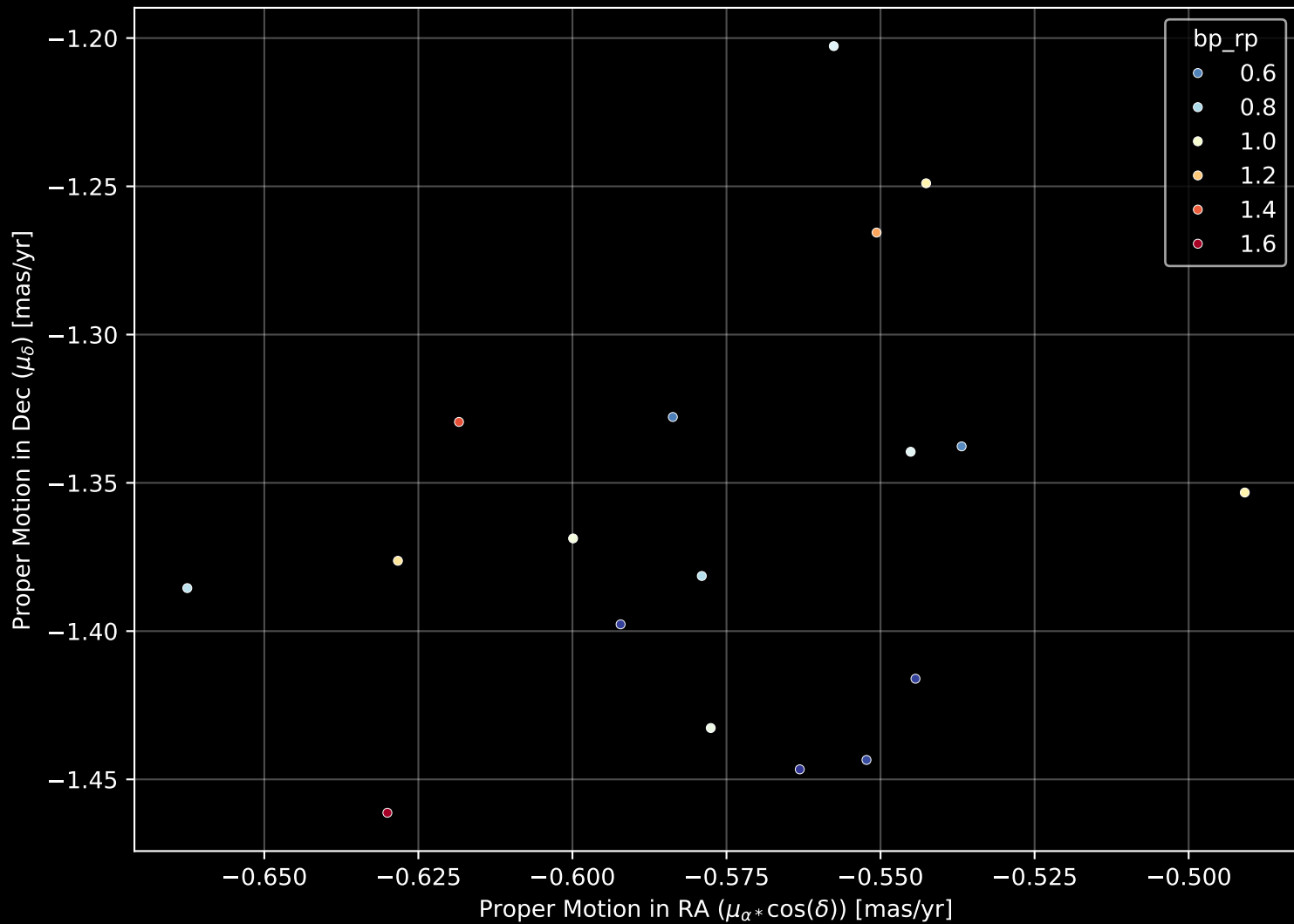
Gaia Cluster: [UBC_3] Proper Motion Diagram (n= 18)
