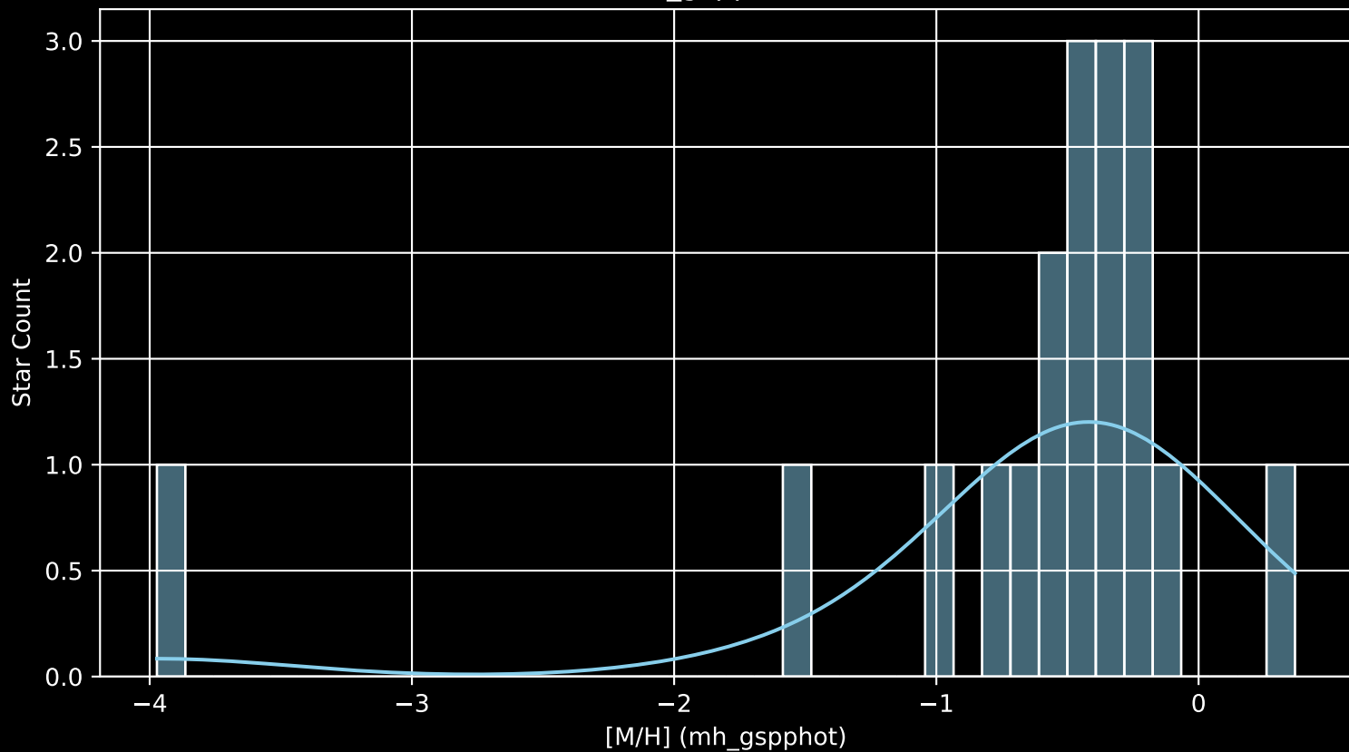
Gaia Cluster: [UBC_3 [M/H] (mh_gspphot) (n= 18)
