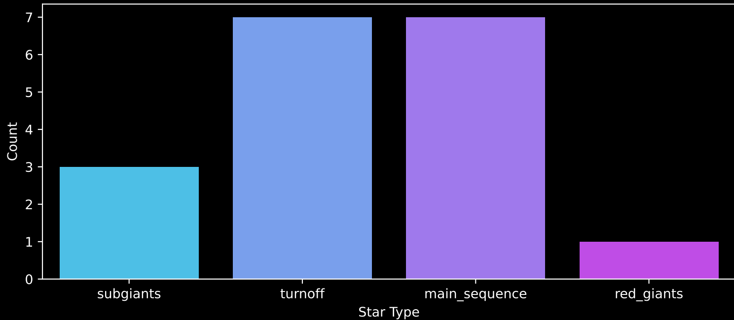
Gaia Cluster: [UBC_3] Count plot of Star Type
