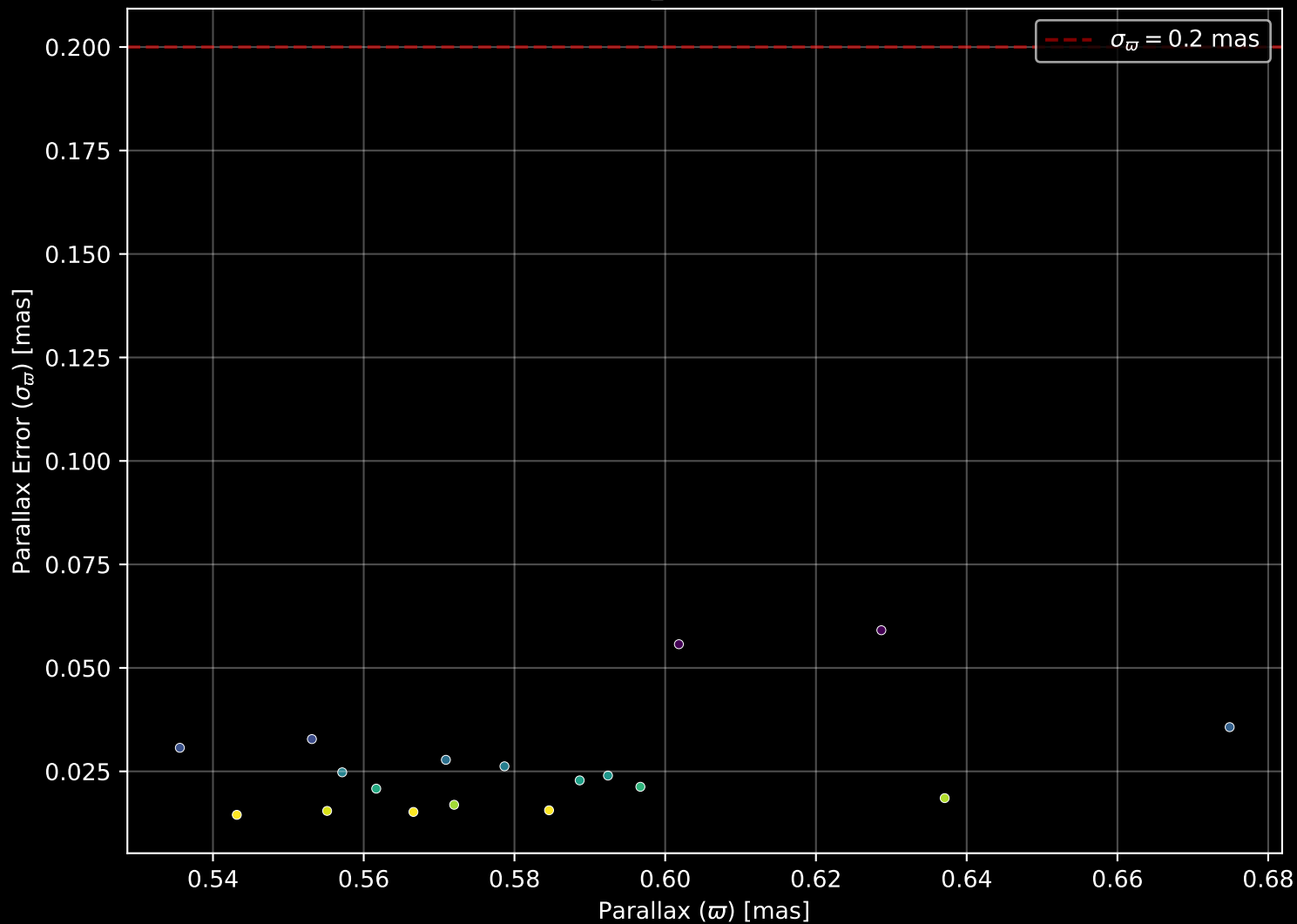
Gaia Cluster: [UBC_3] Parallax Quality (n= 18)
