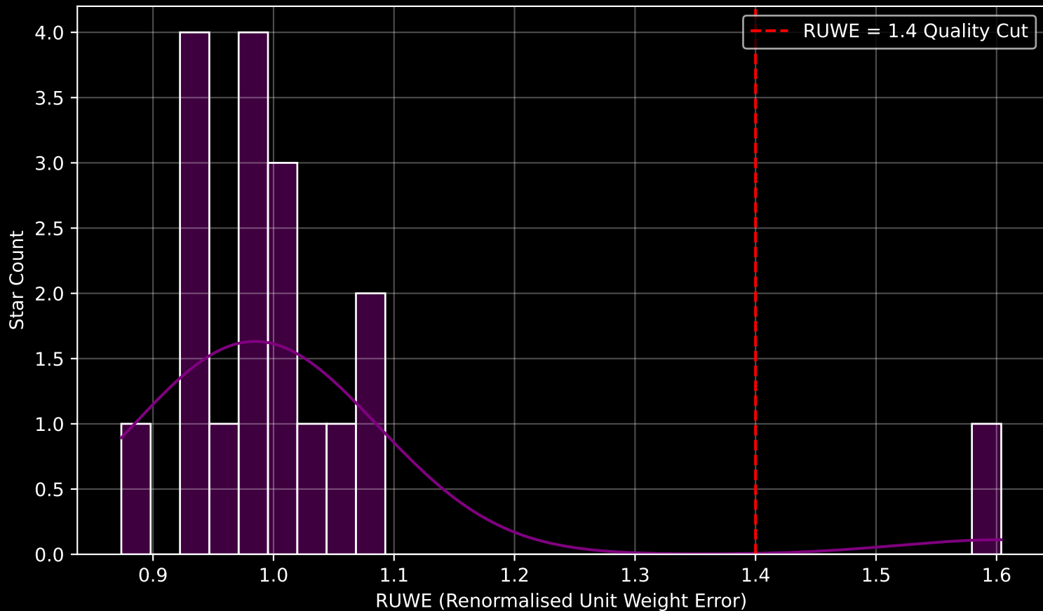
Gaia Cluster: [UBC_3] RUWE Distribution (n= 18)
