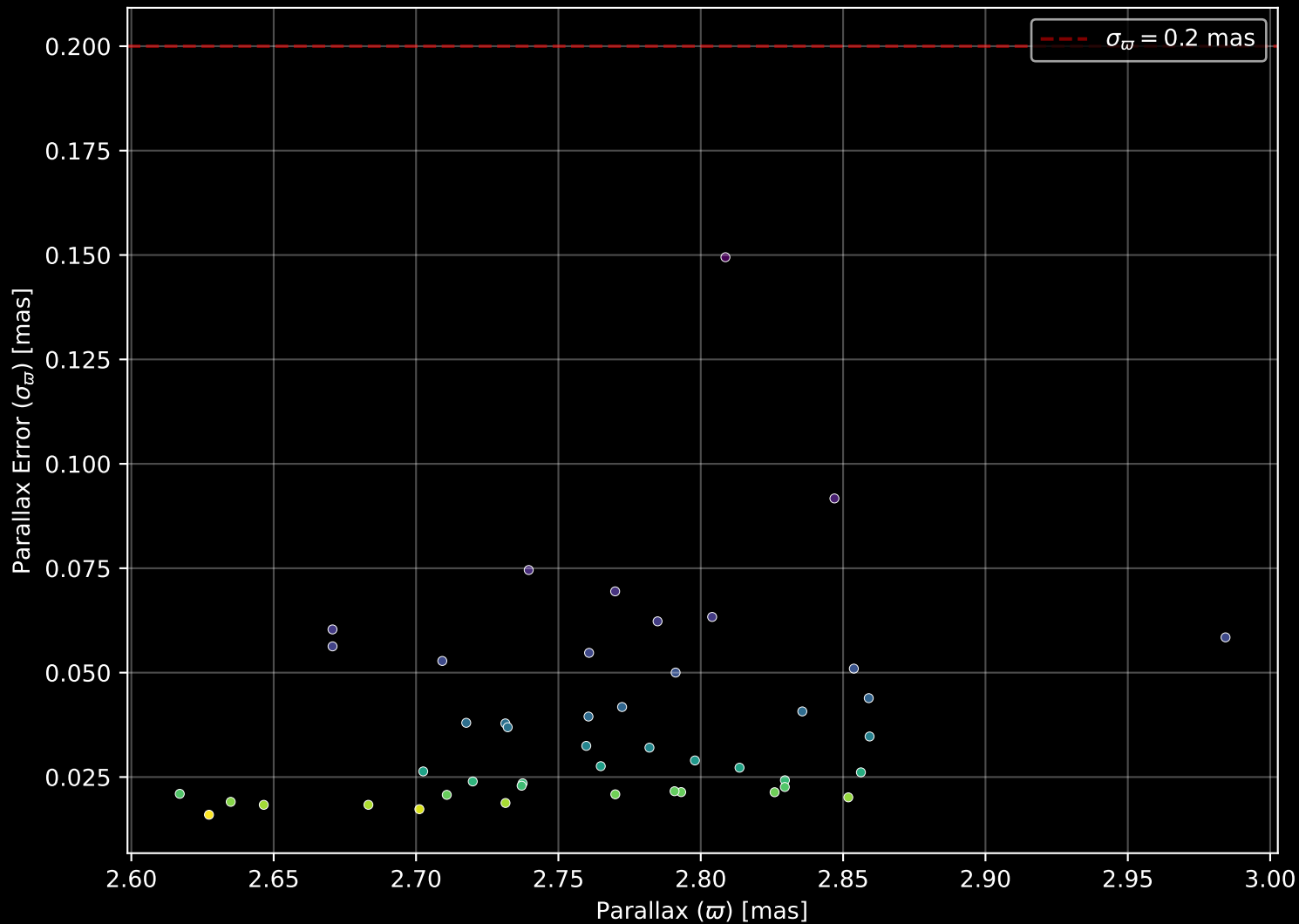
Gaia Cluster: [UBC_31] Parallax Quality (n= 46)
