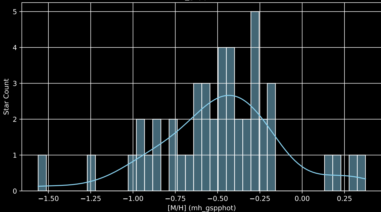
Gaia Cluster: [UBC_31 [M/H] (mh_gspphot) (n= 46)
