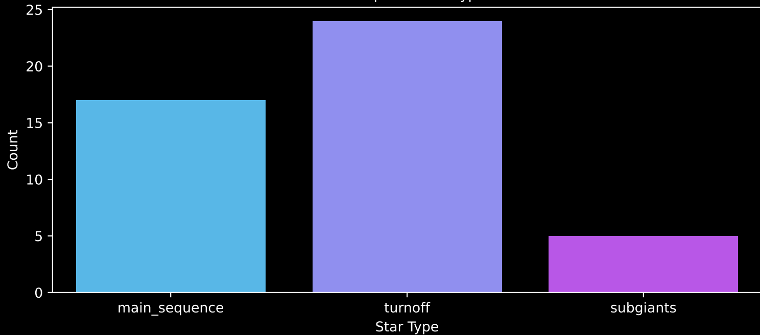
Gaia Cluster: [UBC_31] Count plot of Star Type
