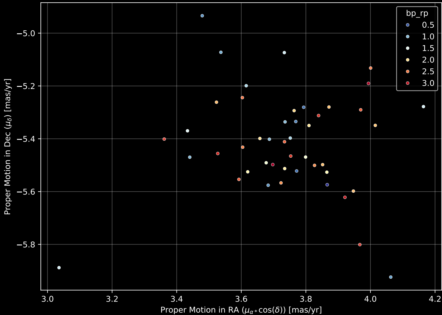
Gaia Cluster: [UBC_31] Proper Motion Diagram (n= 46)
