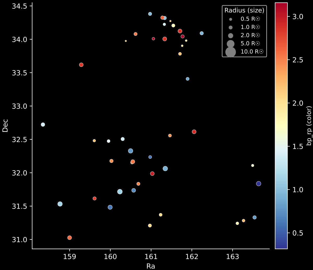
Gaia Cluster: [UBC_31] Stars: 46
