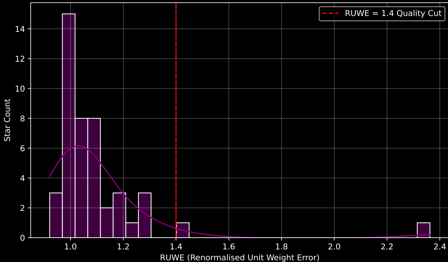
Gaia Cluster: [UBC_31] RUWE Distribution (n= 45)
