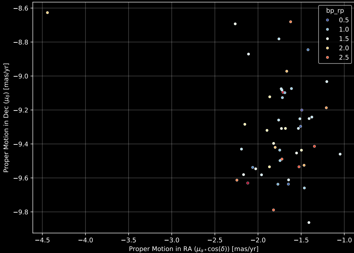
Gaia Cluster: [UBC_32] Proper Motion Diagram (n= 52)
