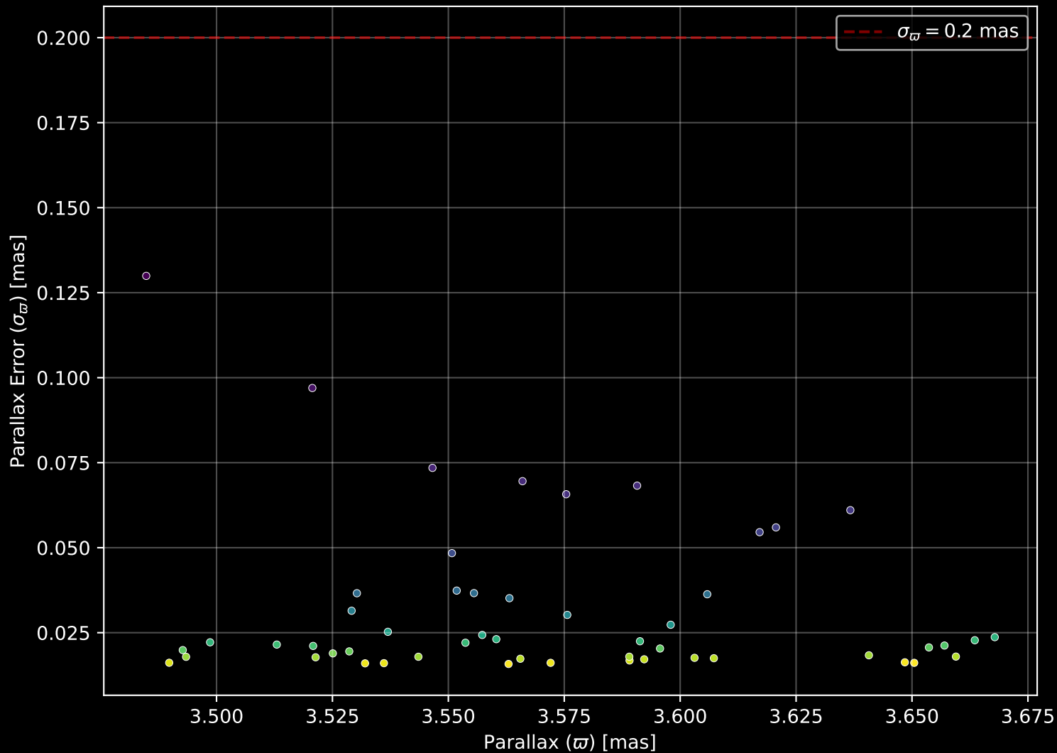
Gaia Cluster: [UBC_32] Parallax Quality (n= 52)
