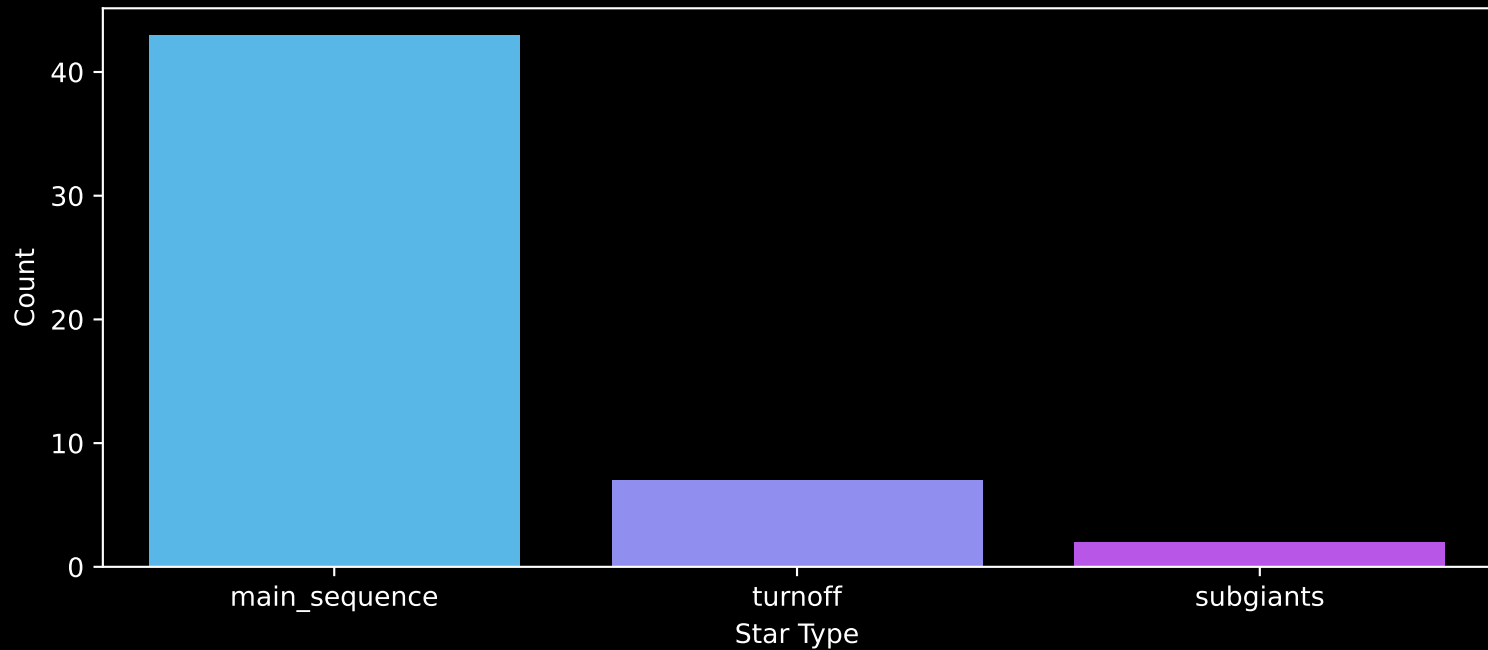
Gaia Cluster: [UBC_32] Count plot of Star Type
