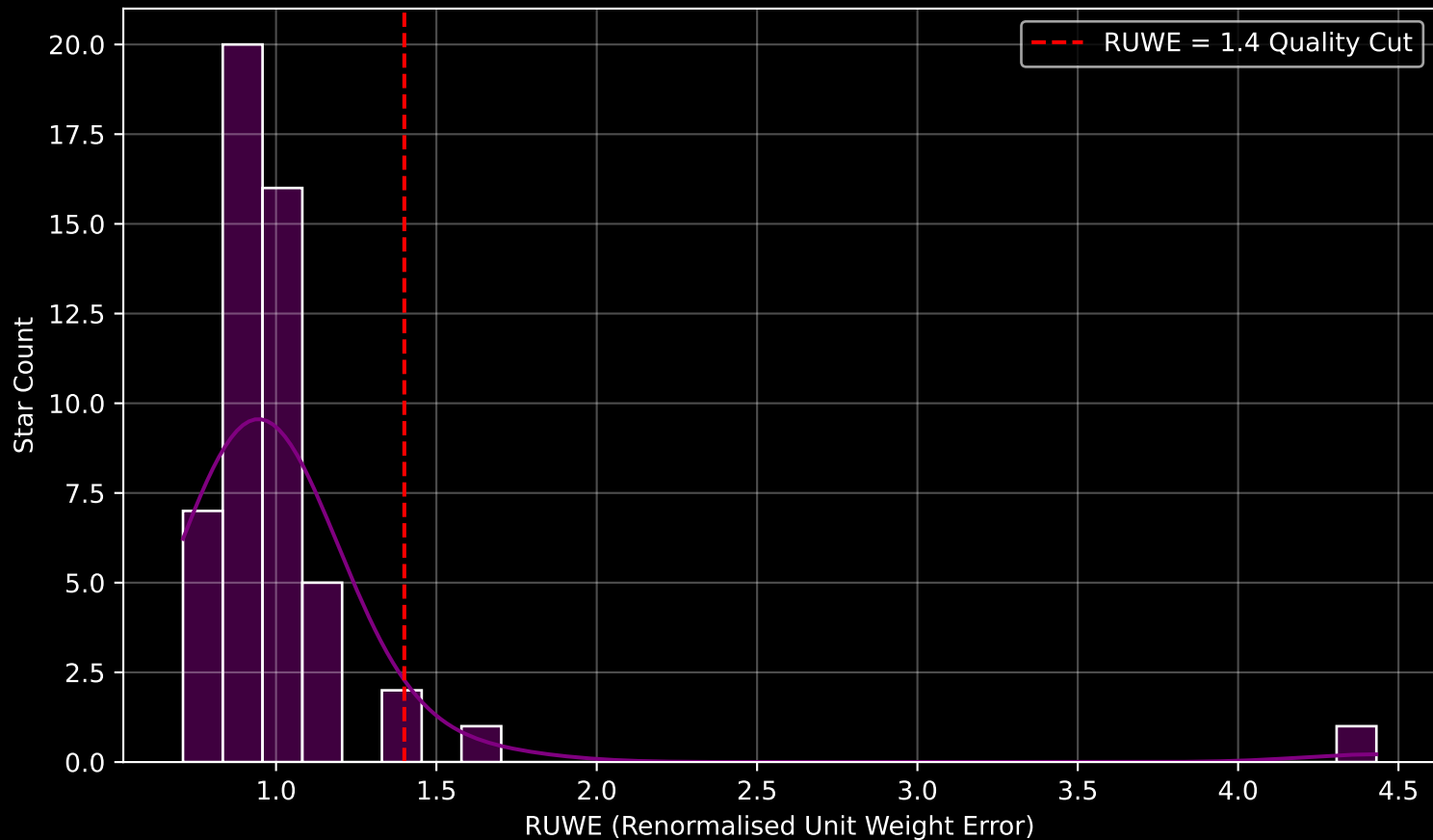
Gaia Cluster: [UBC_32] RUWE Distribution (n= 52)
