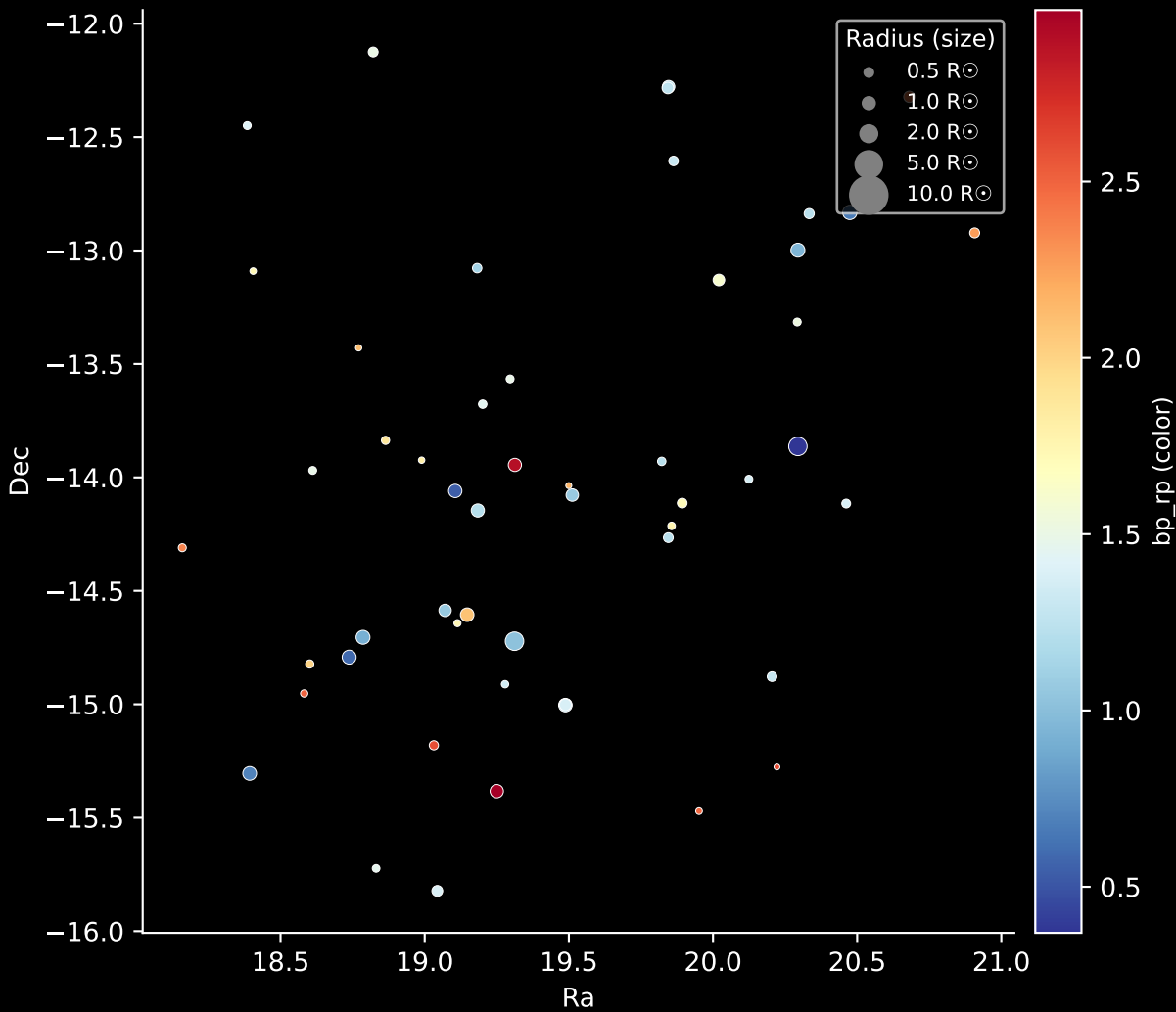
Gaia Cluster: [UBC_32] Stars: 52
