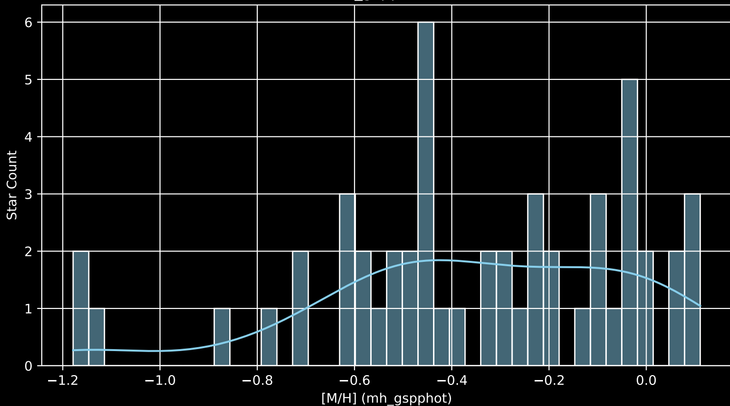
Gaia Cluster: [UBC_32 [M/H] (mh_gspphot) (n= 52)
