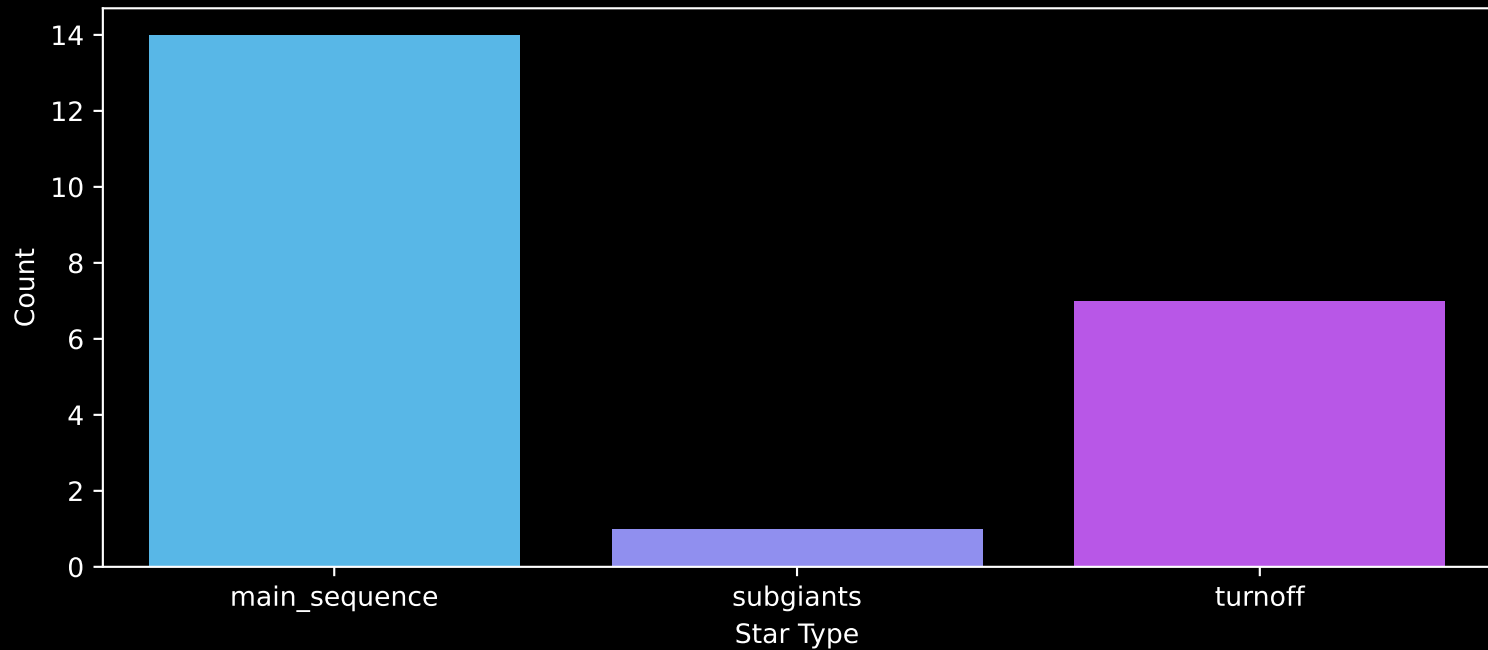
Gaia Cluster: [UBC_36] Count plot of Star Type
