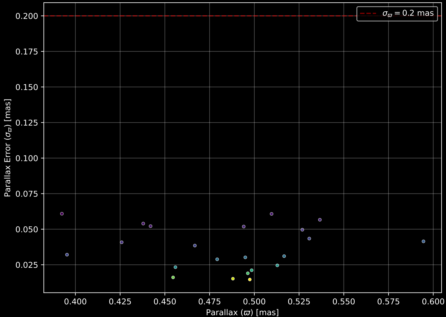
Gaia Cluster: [UBC_36] Parallax Quality (n= 22)
