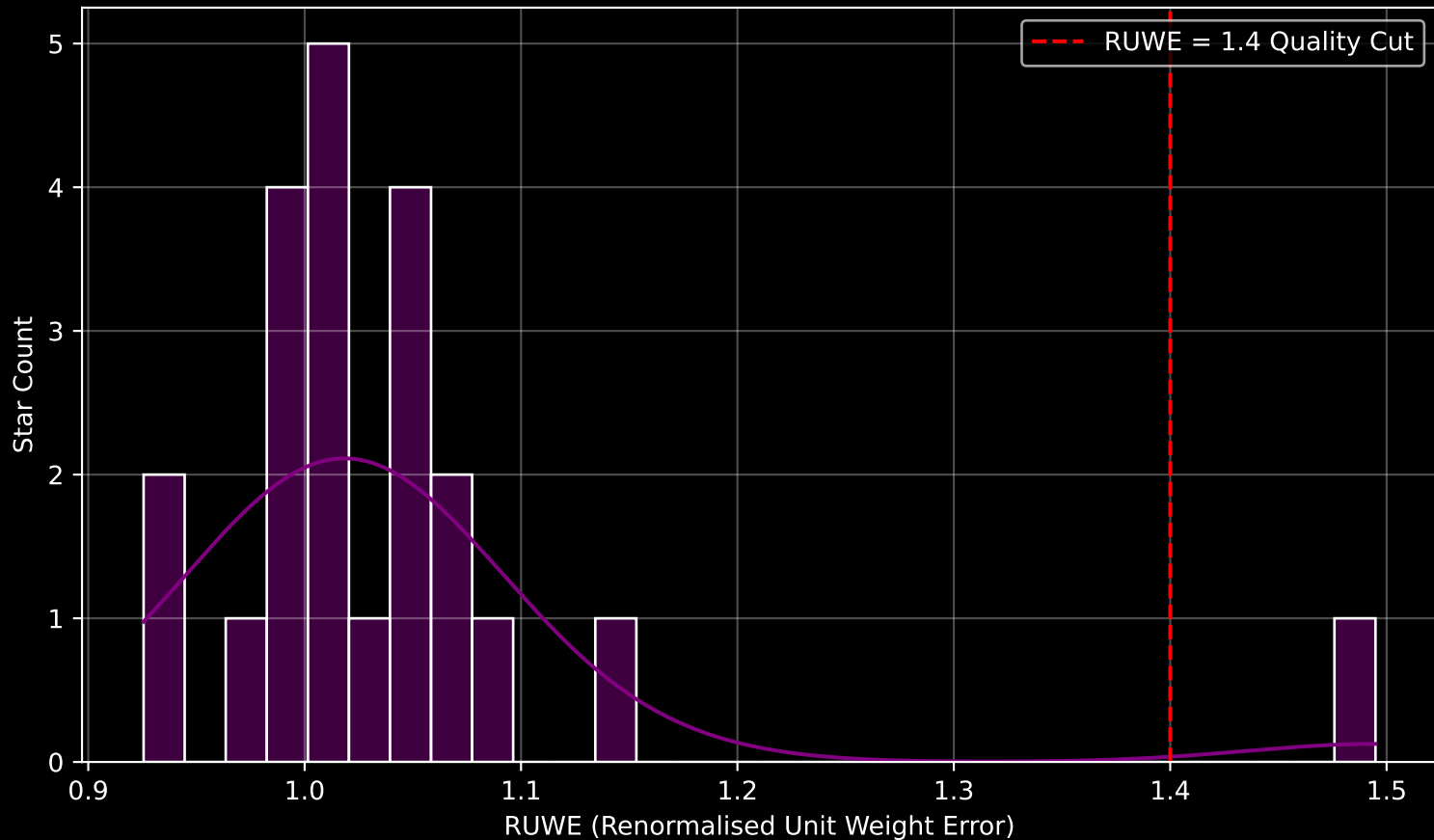
Gaia Cluster: [UBC_36] RUWE Distribution (n= 22)
