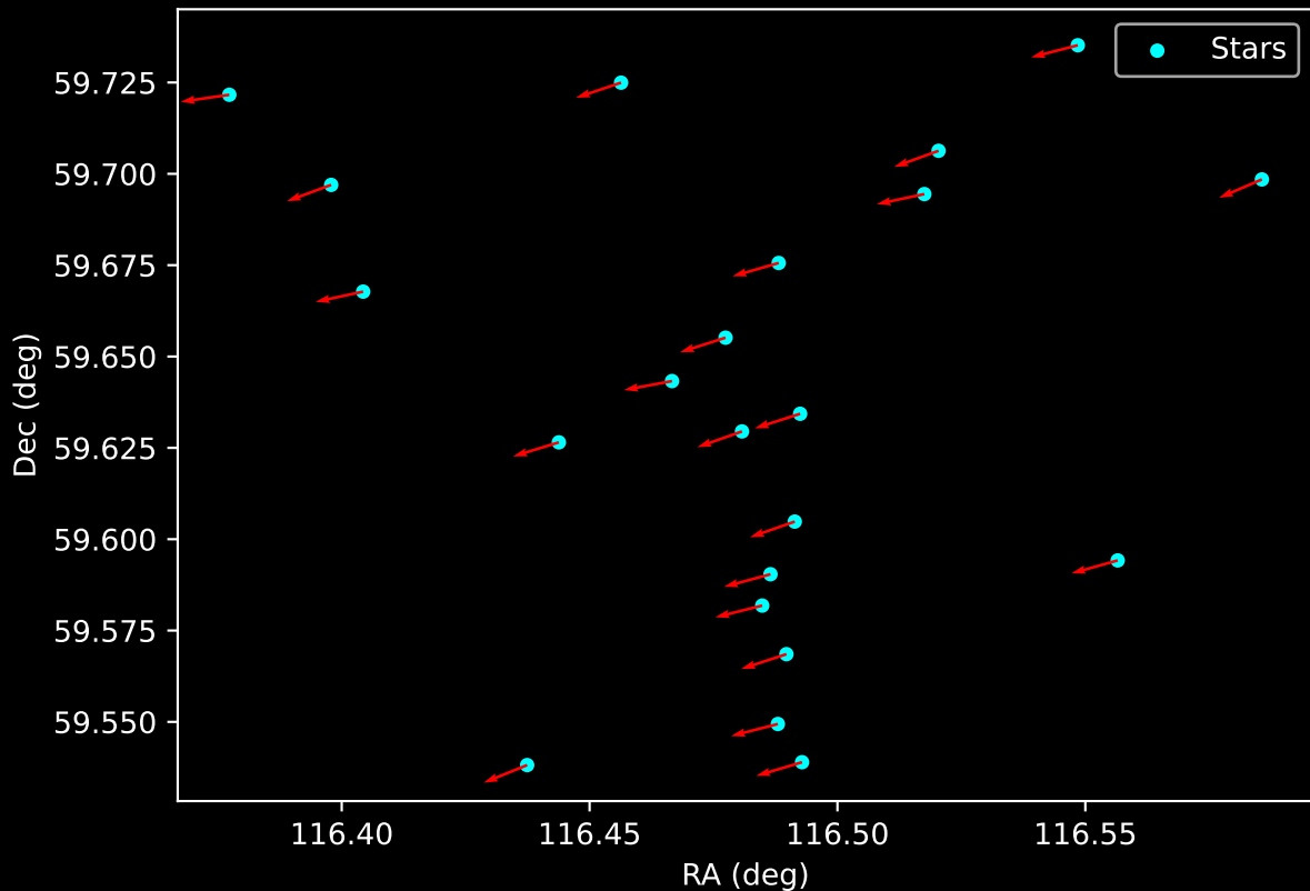
Gaia Cluster: [UBC_36] Proper Motion Vectors for Gaia Star Field (n= 22)
