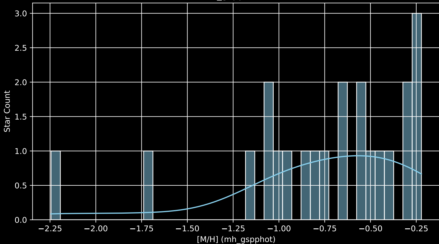
Gaia Cluster: [UBC_36 [M/H] (mh_gspphot) (n= 22)
