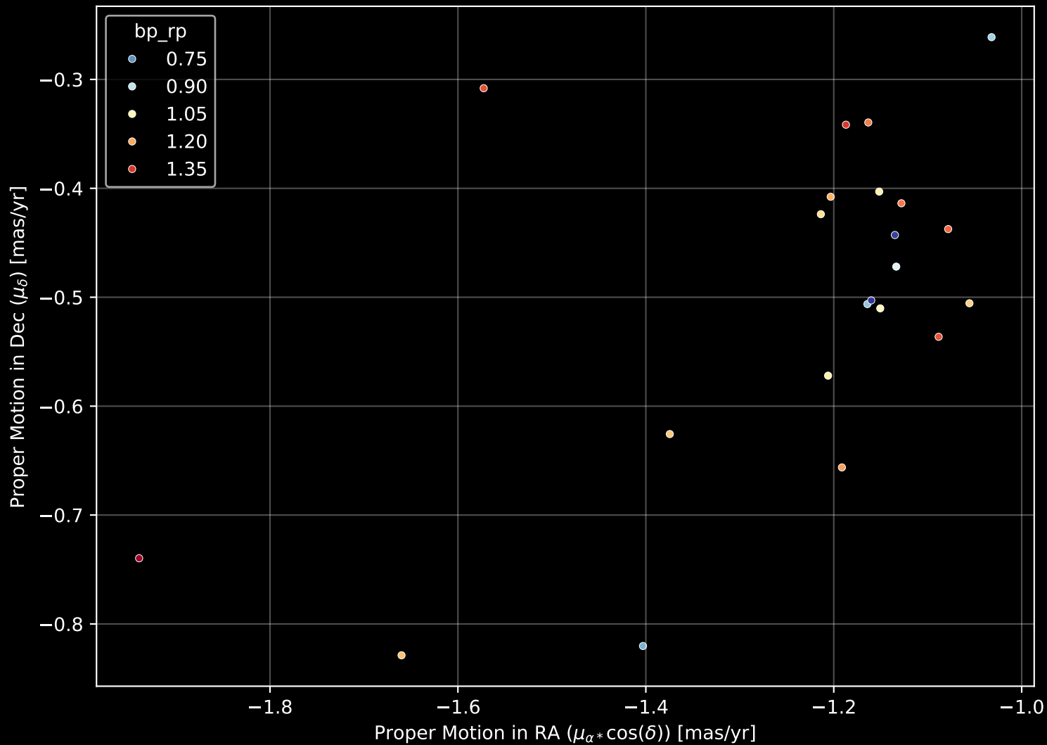
Gaia Cluster: [UBC_36] Proper Motion Diagram (n= 22)
