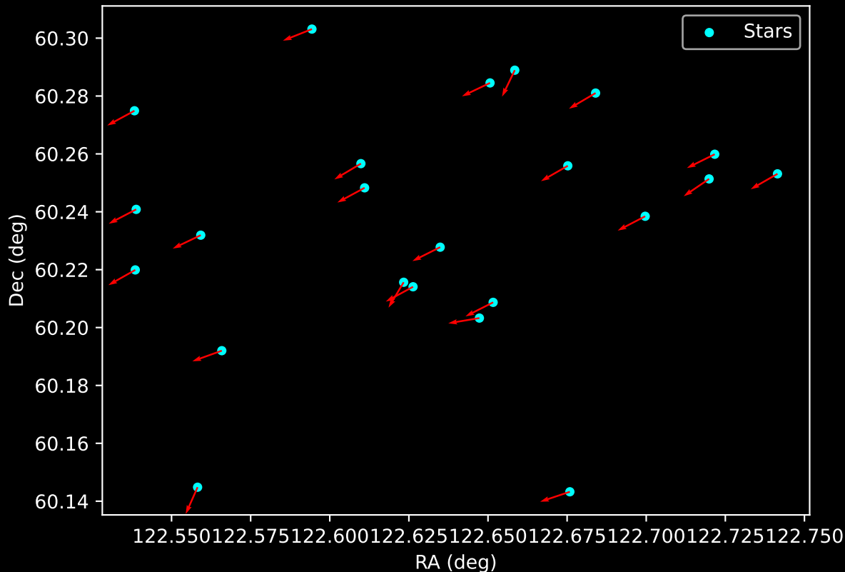
Gaia Cluster: [UBC_40] Proper Motion Vectors for Gaia Star Field (n= 23)
