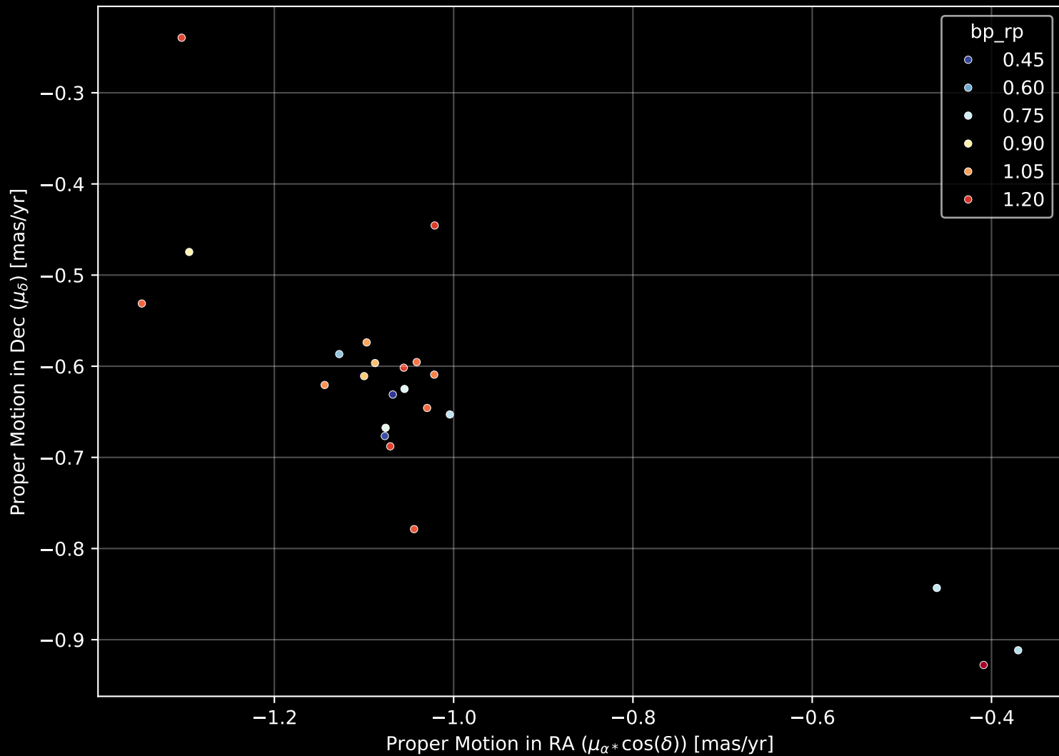
Gaia Cluster: [UBC_40] Proper Motion Diagram (n= 23)
