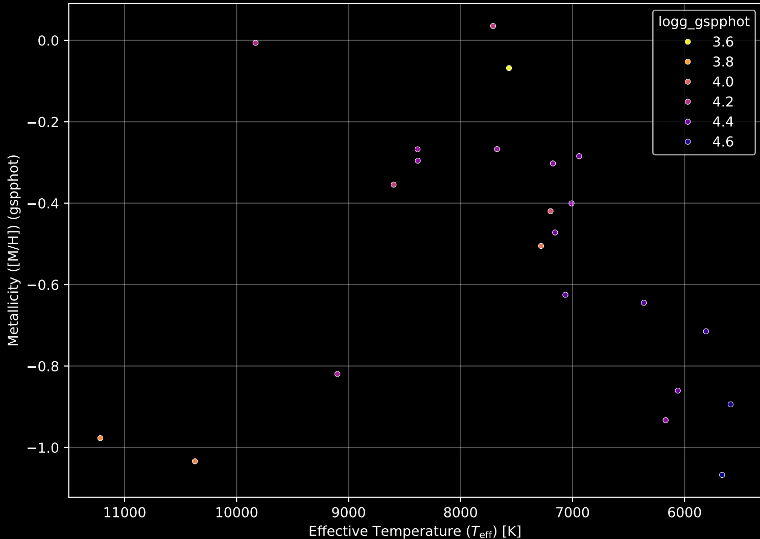
Gaia Cluster: [UBC_40] Stellar Population Parameters (n= 23)
