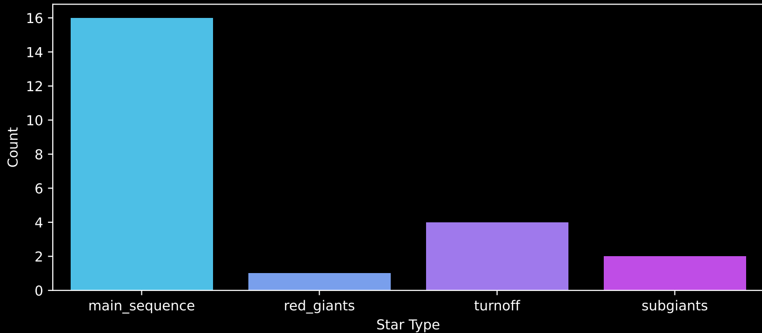
Gaia Cluster: [UBC_40] Count plot of Star Type
