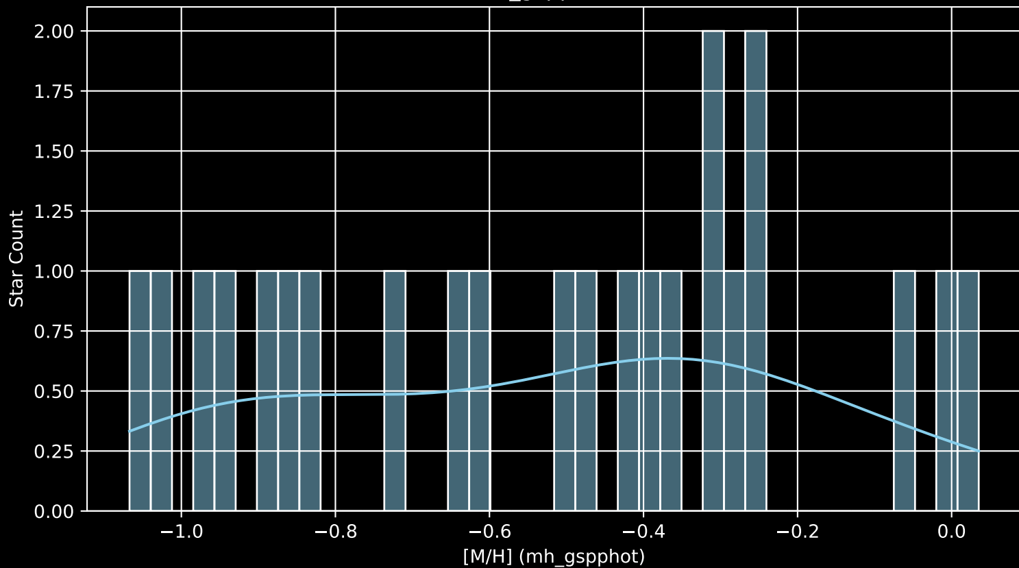
Gaia Cluster: [UBC_40 [M/H] (mh_gspphot) ( \bar{n}=23 )
