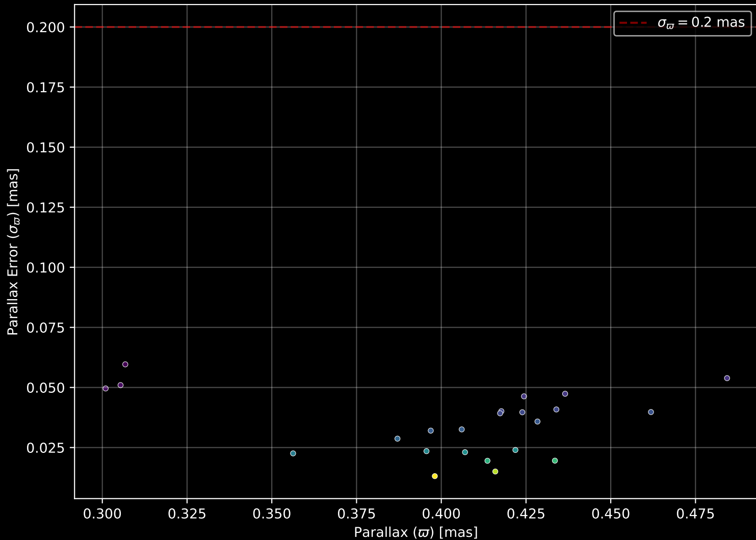
Gaia Cluster: [UBC_40] Parallax Quality (n= 23)
