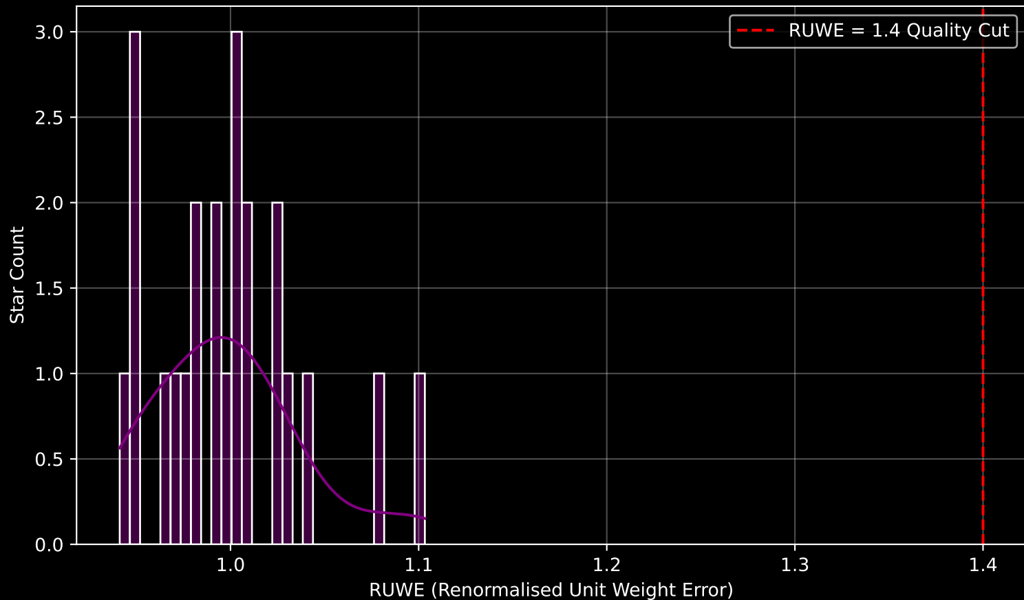
Gaia Cluster: [UBC_40] RUWE Distribution (n= 23)
