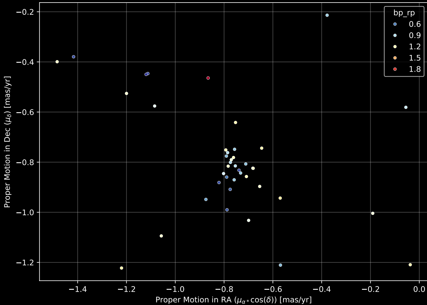
Gaia Cluster: [UBC_41] Proper Motion Diagram (n= 41)
