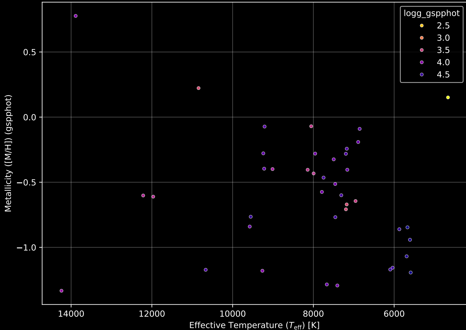
Gaia Cluster: [UBC_41] Stellar Population Parameters (n= 41)
