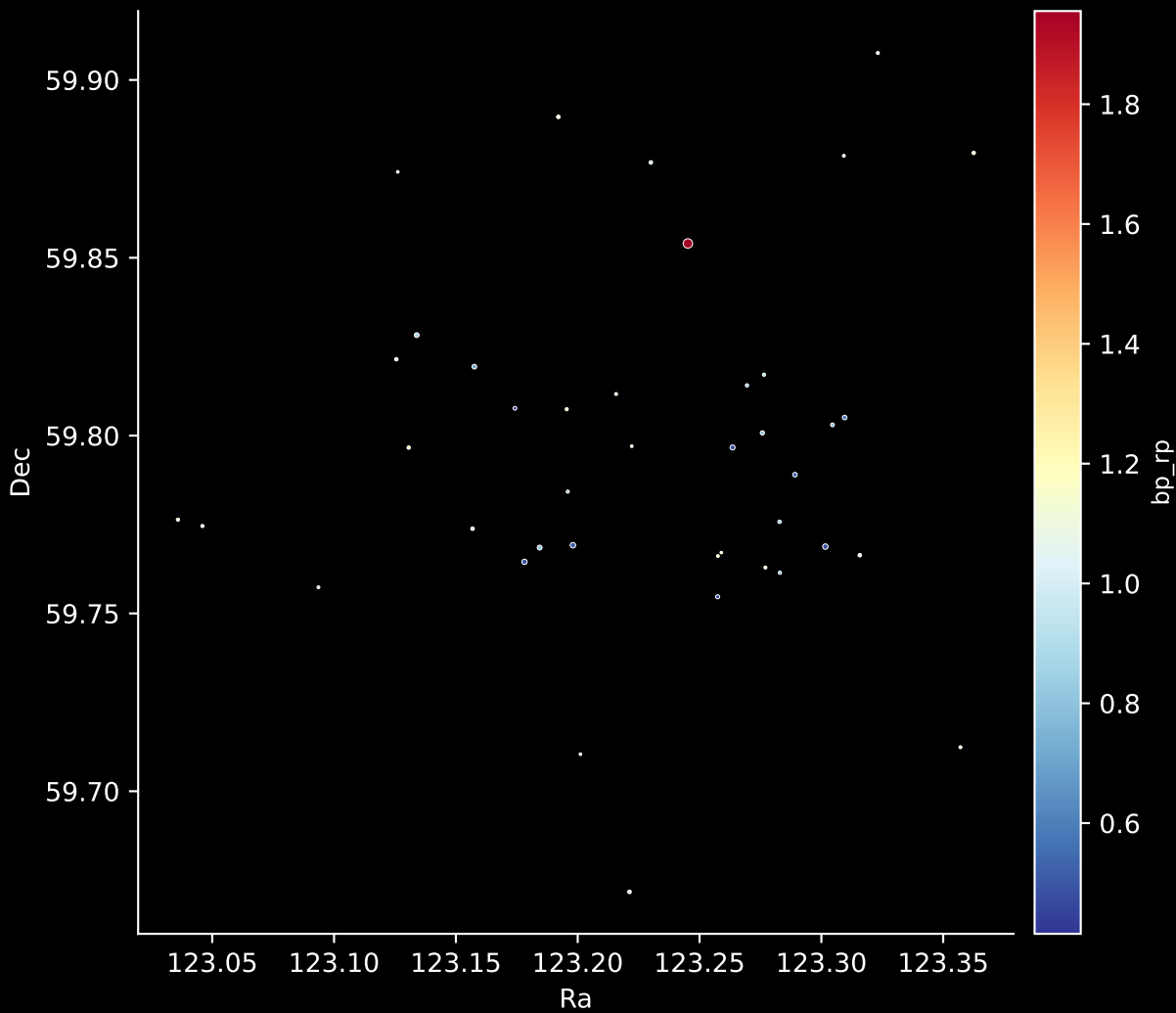
Gaia Cluster: [UBC_41] Stars: 41
