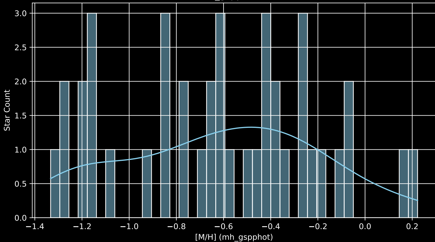
Gaia Cluster: [UBC_41 [M/H] (mh_gspphot) ( n = 40 )
