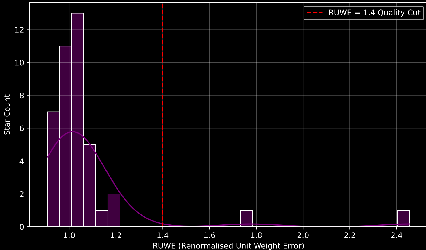
Gaia Cluster: [UBC_41] RUWE Distribution (n= 41)
