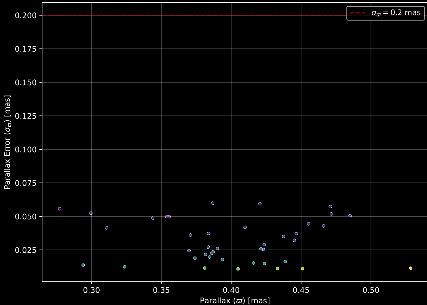
Gaia Cluster: [UBC_41] Parallax Quality (n= 41)
