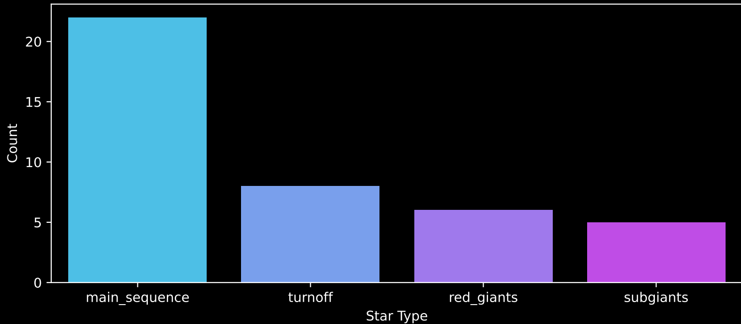
Gaia Cluster: [UBC_41] Count plot of Star Type
