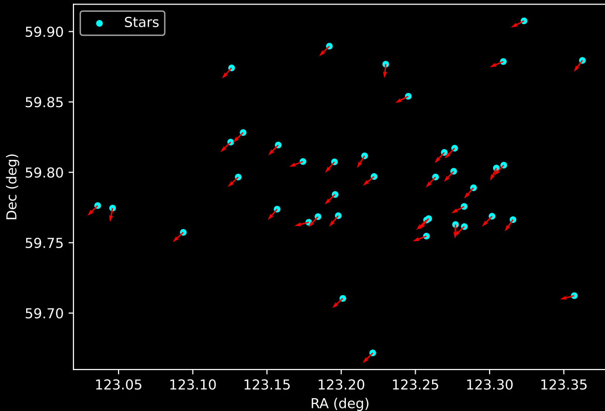
Gaia Cluster: [UBC_41] Proper Motion Vectors for Gaia Star Field (n= 41)
