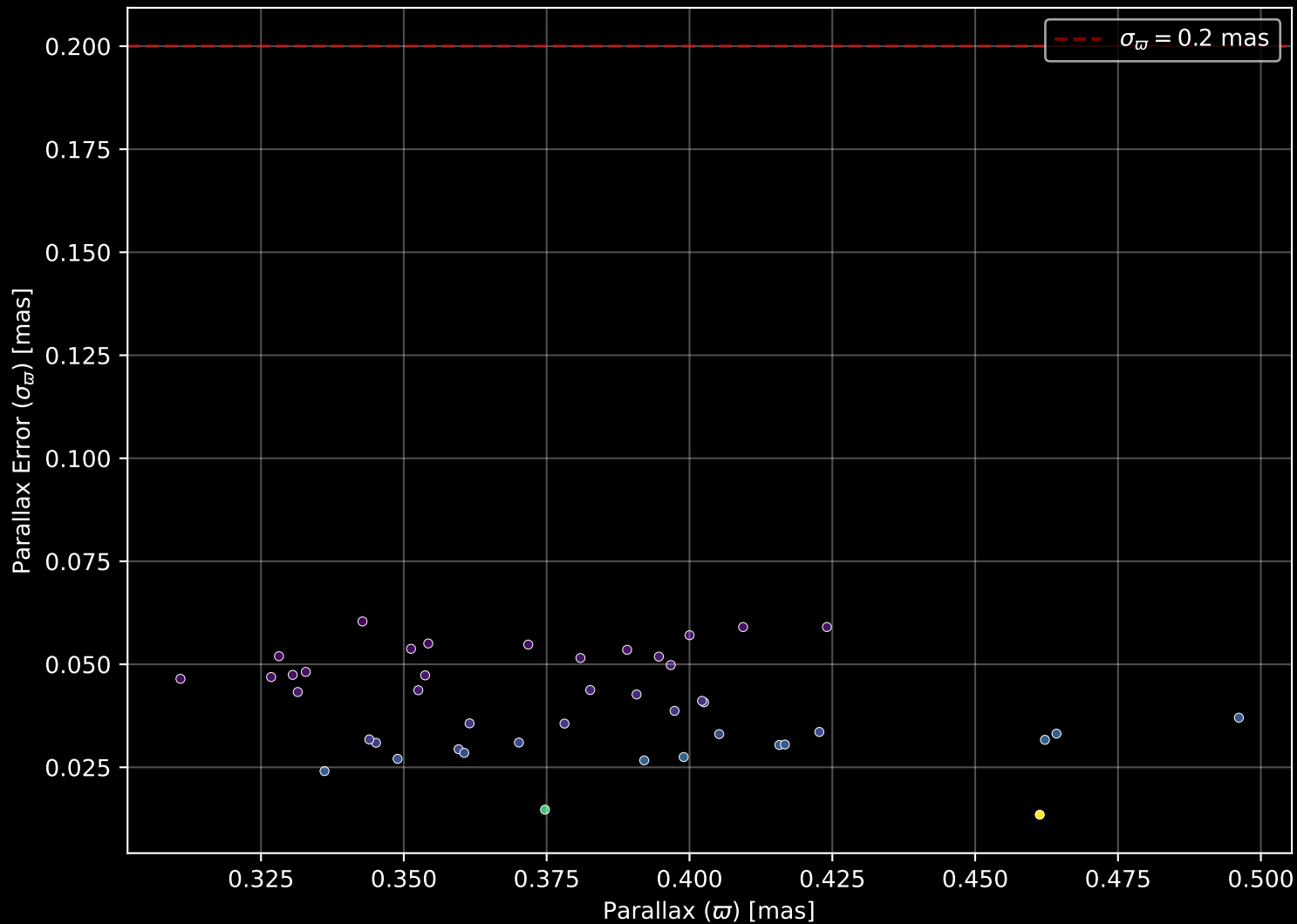
Gaia Cluster: [UBC_49] Parallax Quality (n= 44)
