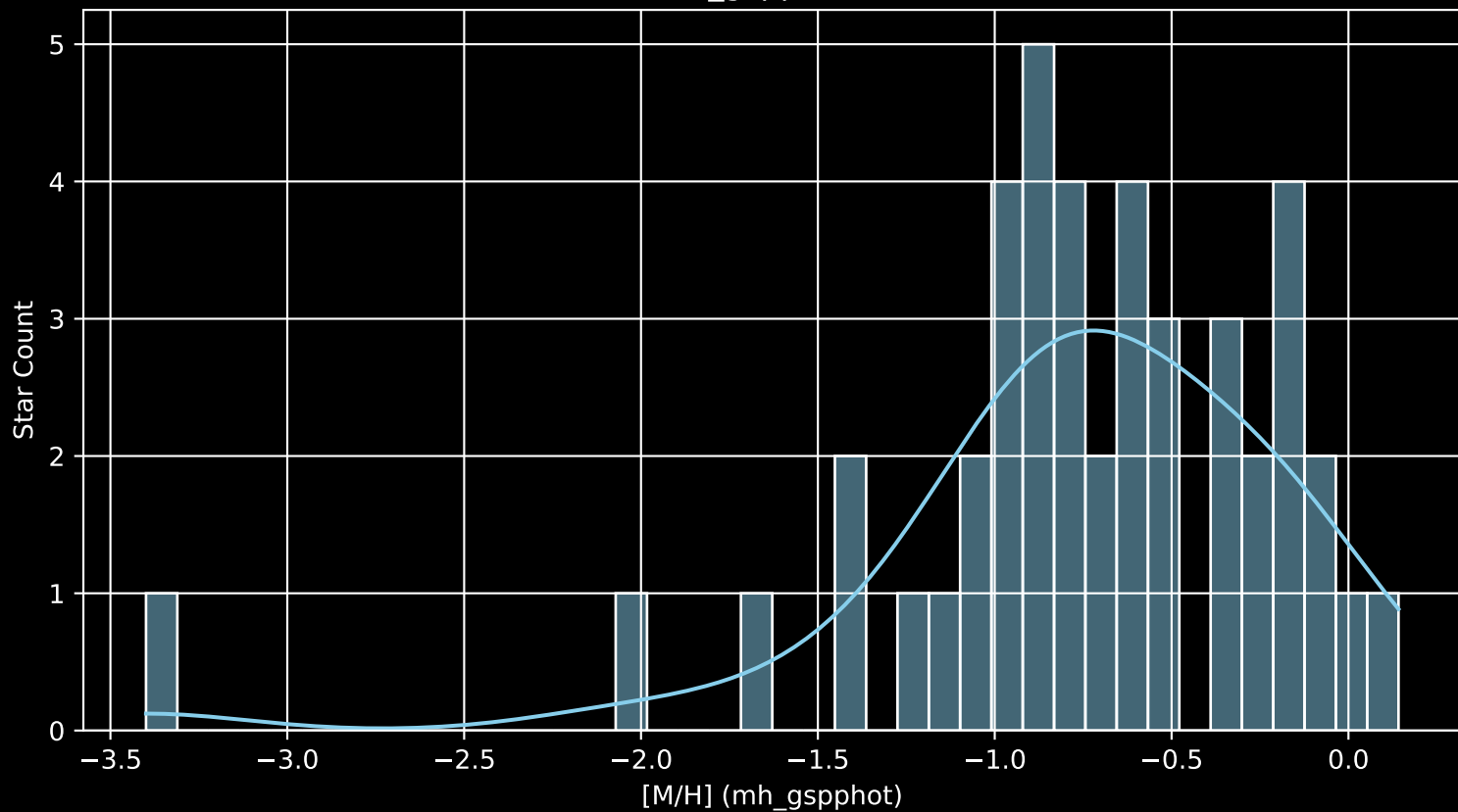
Gaia Cluster: [UBC_49 [M/H] (mh_gspphot) ( \bar{n}=44 )
