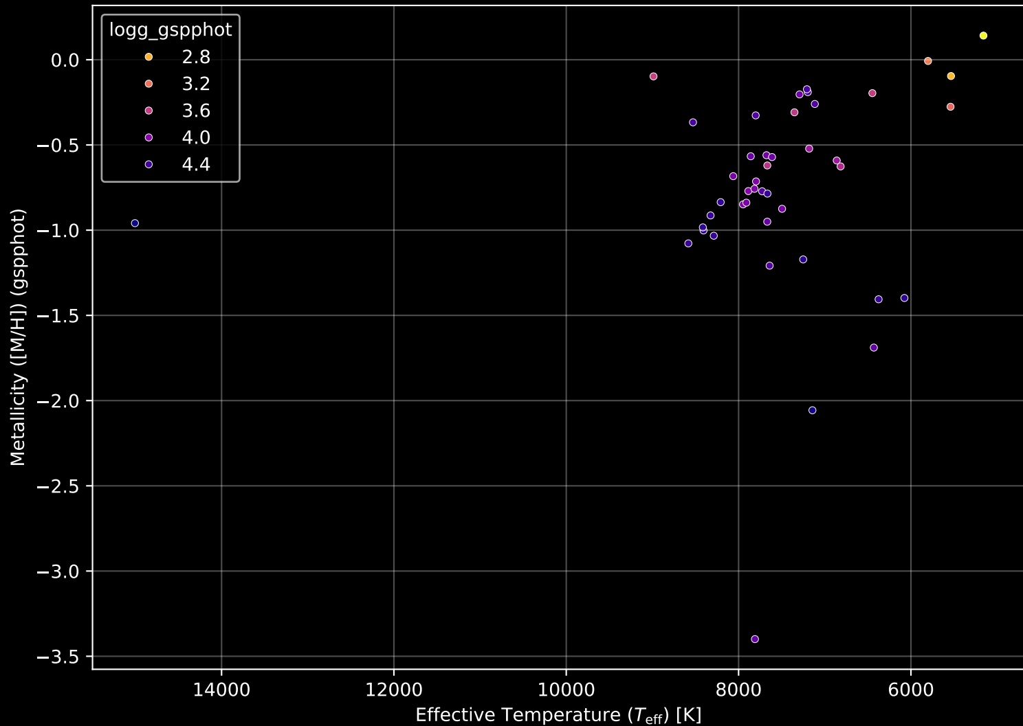
Gaia Cluster: [UBC_49] Stellar Population Parameters (n= 44)
