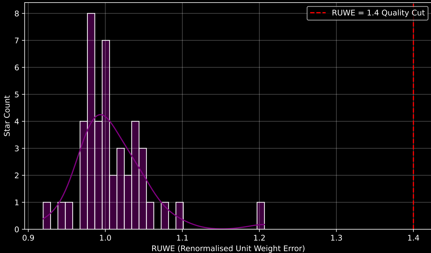
Gaia Cluster: [UBC_49] RUWE Distribution (n= 44)
