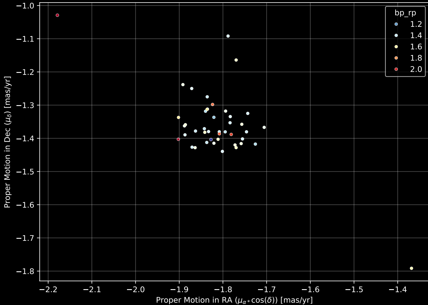
Gaia Cluster: [UBC_49] Proper Motion Diagram (n= 44)
