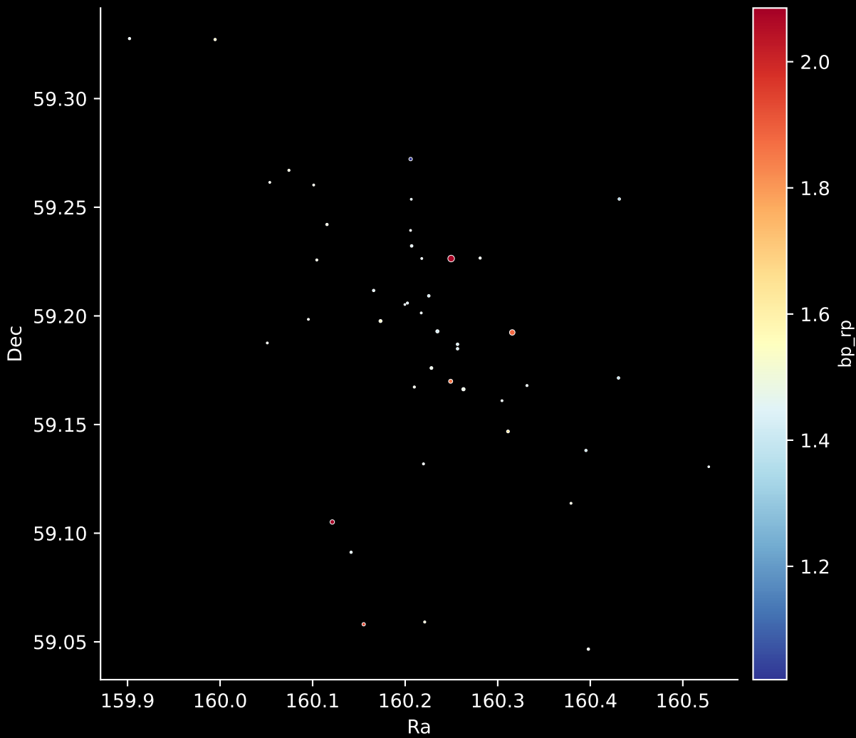
Gaia Cluster: [UBC_49] Stars: 44
