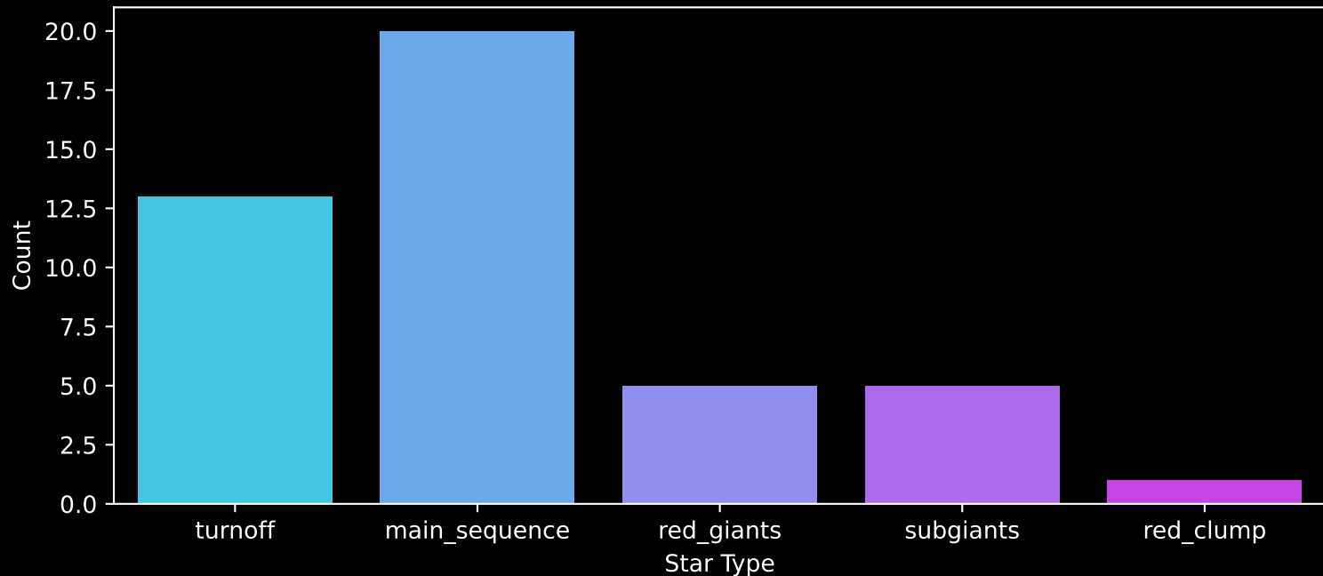
Gaia Cluster: [UBC_49] Count plot of Star Type
