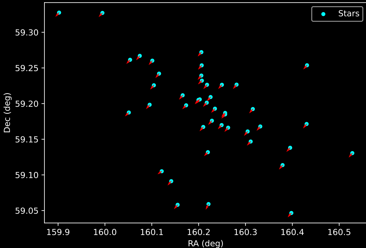
Gaia Cluster: [UBC_49] Proper Motion Vectors for Gaia Star Field (n= 44)
