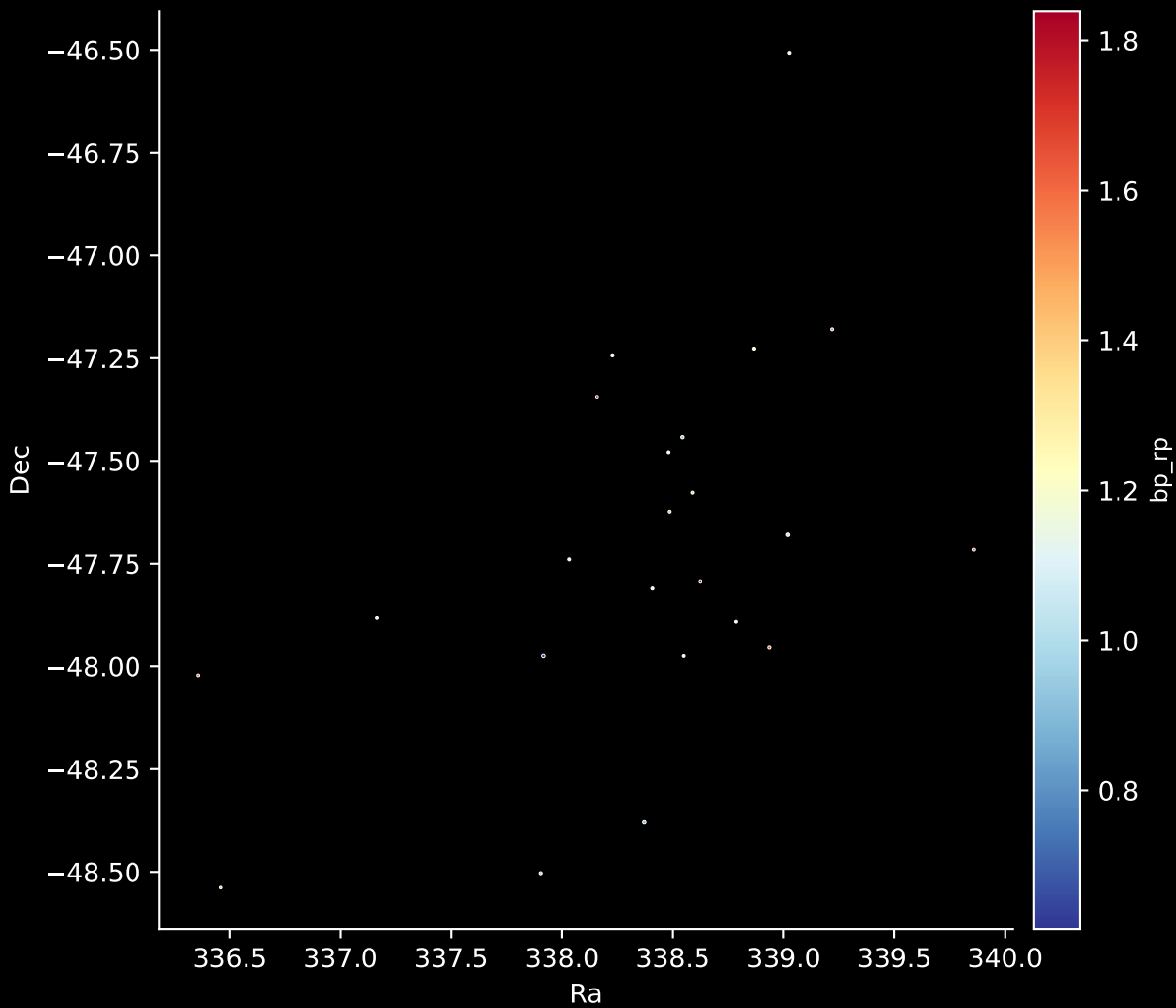
Gaia Cluster: [UBC_5] Stars: 23
