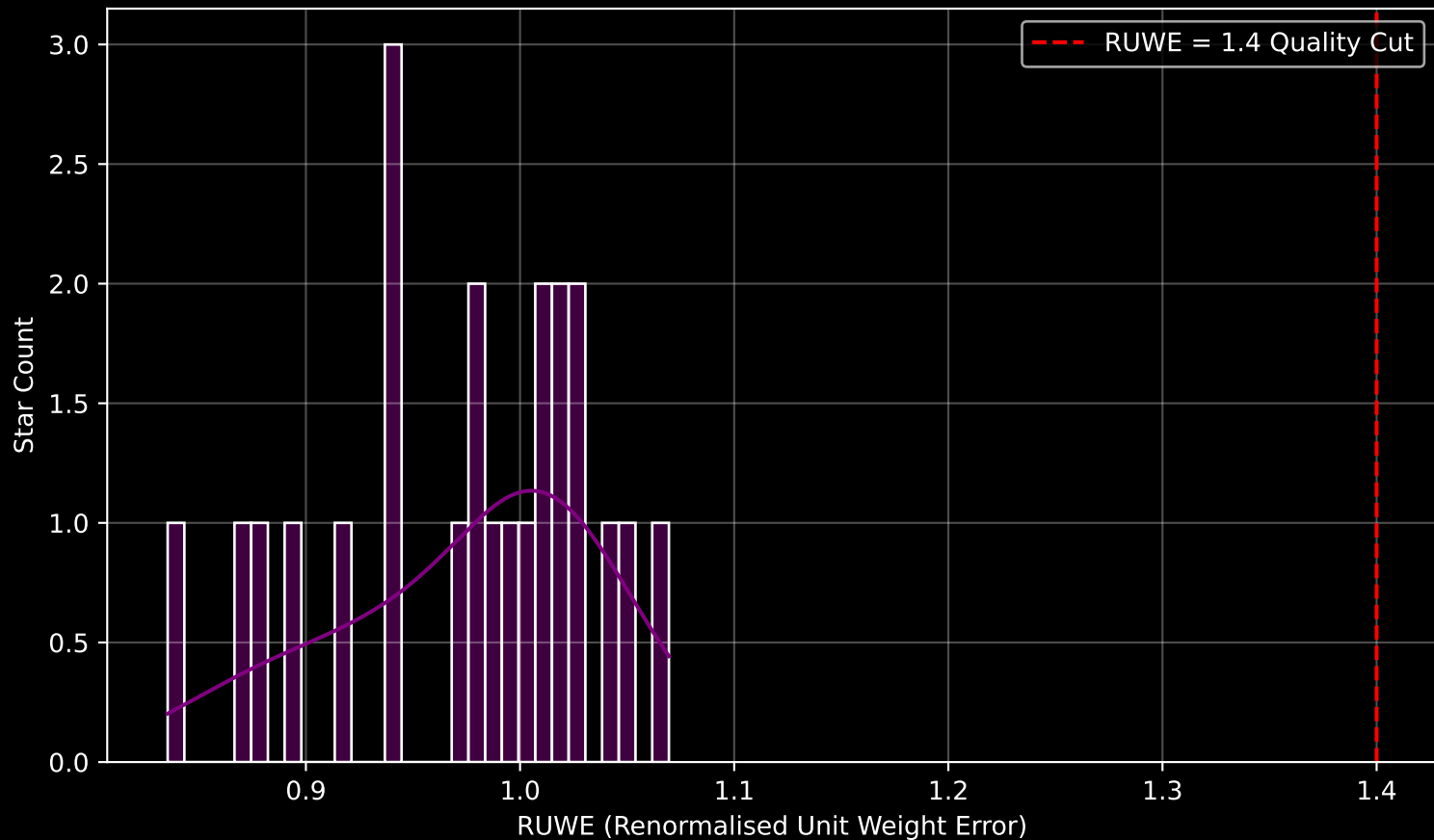
Gaia Cluster: [UBC_5] RUWE Distribution (n= 23)
