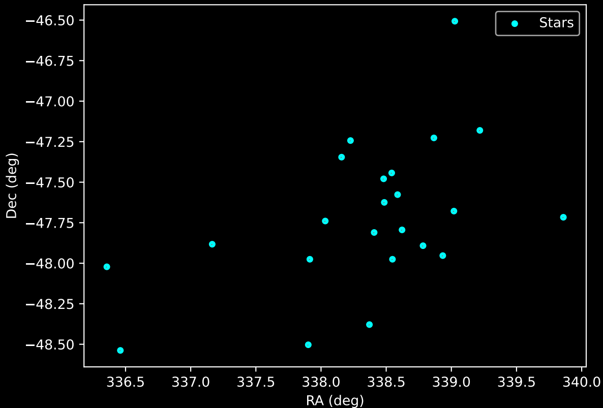
Gaia Cluster: [UBC_5] Proper Motion Vectors for Gaia Star Field (n= 23)
