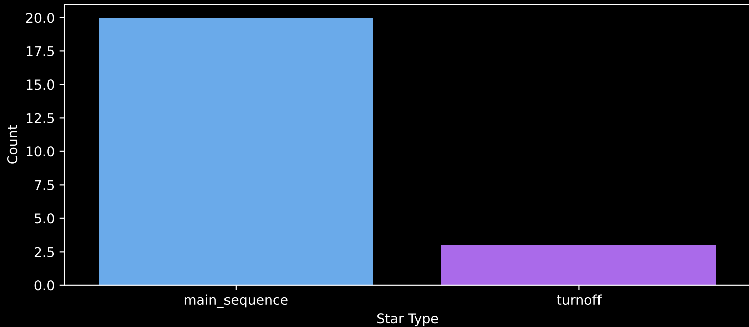
Gaia Cluster: [UBC_5] Count plot of Star Type
