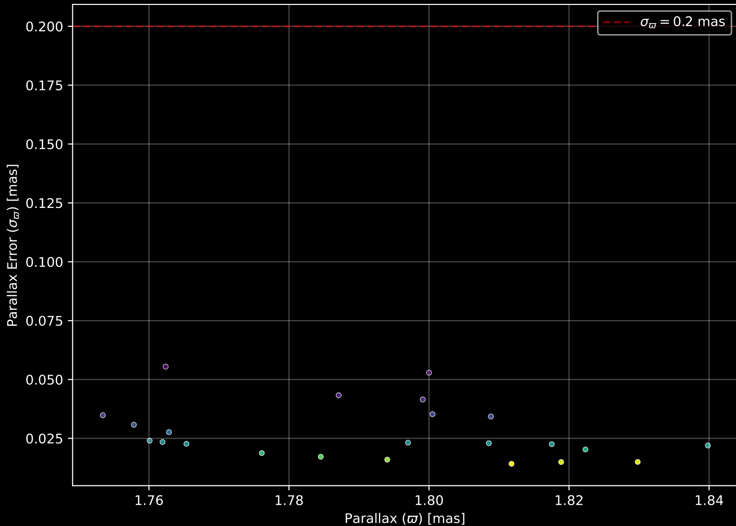
Gaia Cluster: [UBC_5] Parallax Quality (n= 23)
