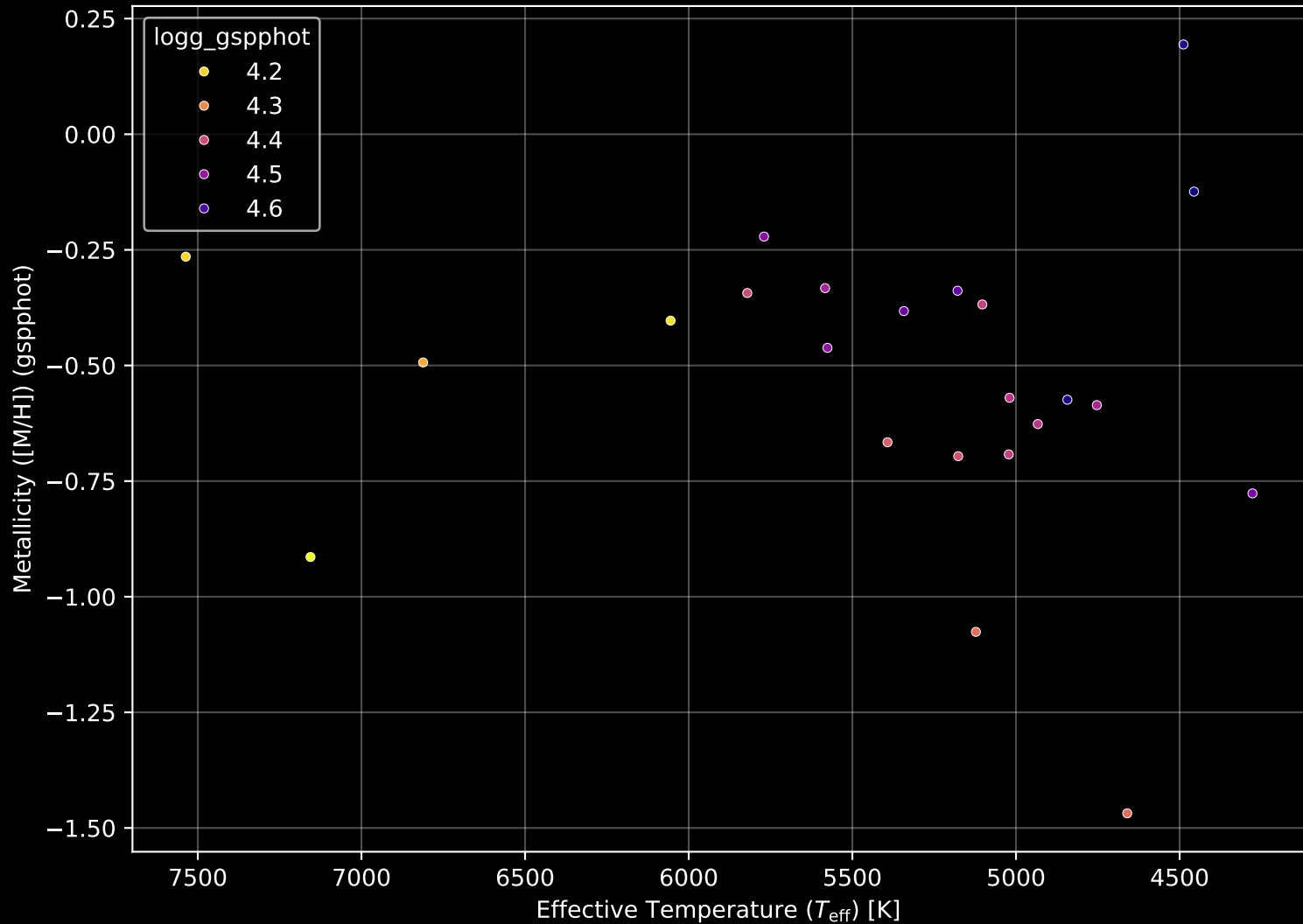
Gaia Cluster: [UBC_5] Stellar Population Parameters (n= 23)
