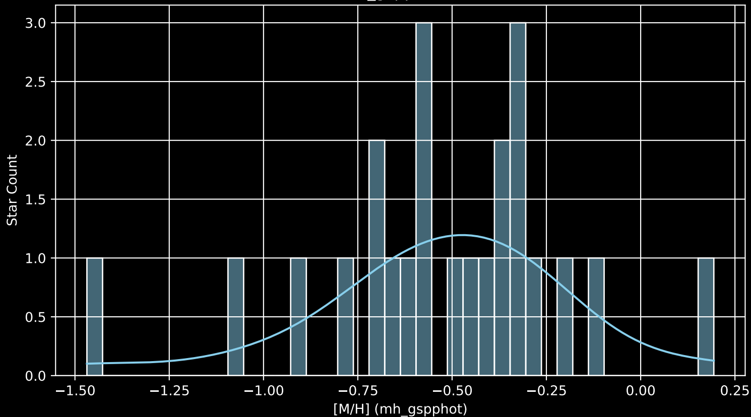
Gaia Cluster: [UBC_5 [M/H] (mh_gspphot) (n= 23)
