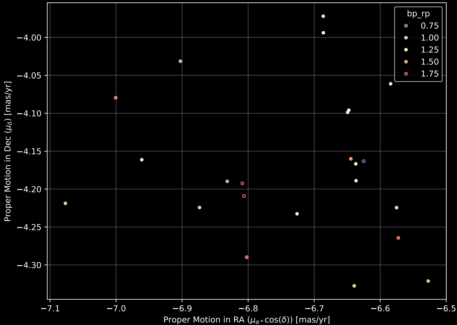
Gaia Cluster: [UBC 5] Proper Motion Diagram (n= 23)
